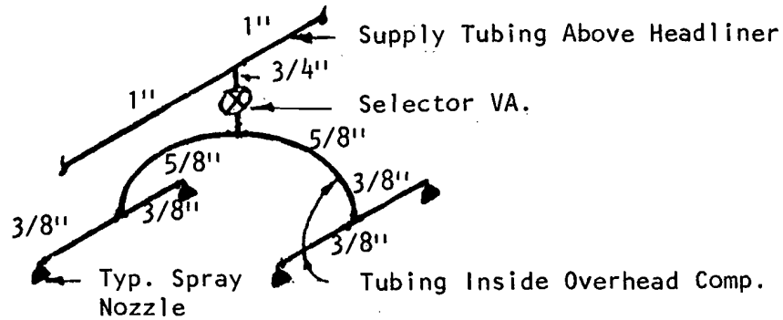
NOZZLE AND TUBING SCHEMATIC
