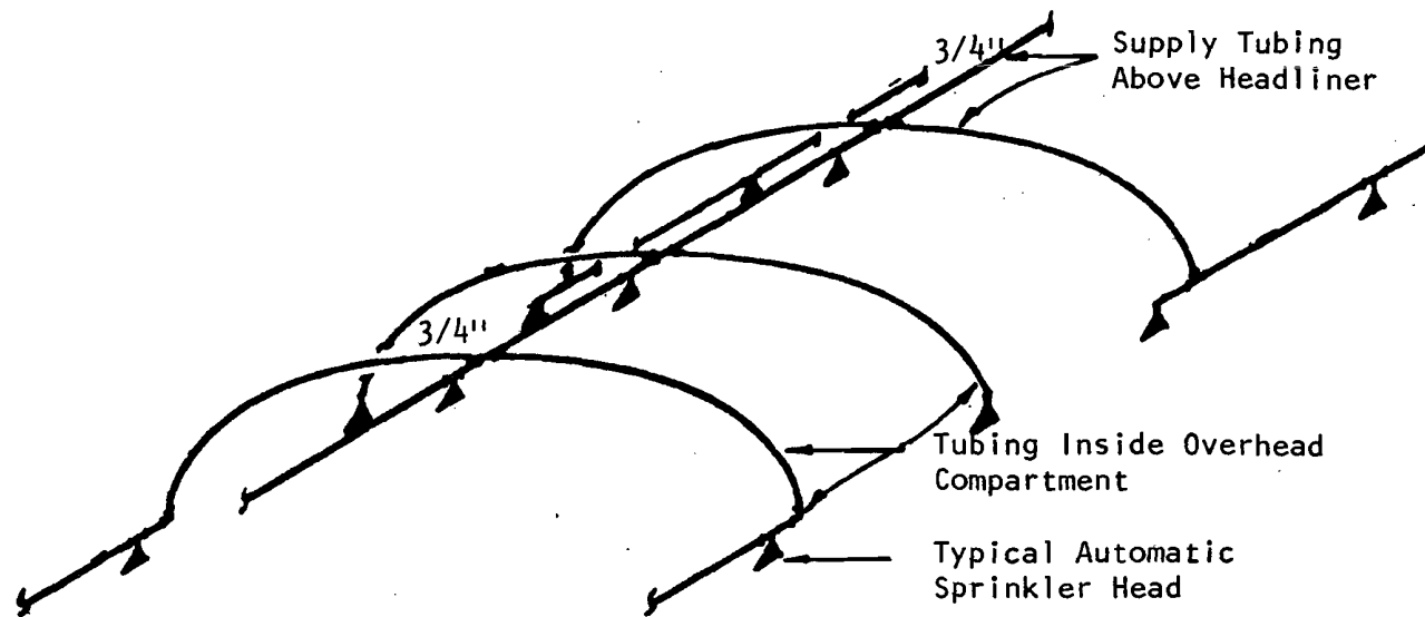
AUTOMATIC SPRINKLER AND PIPING SCHEMATIC
