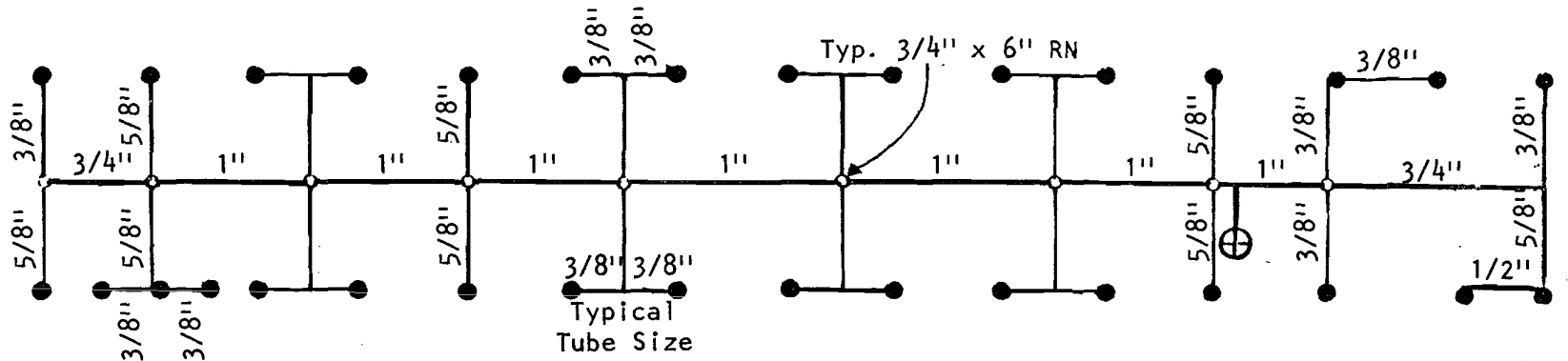
NOZZLE AND TUBING PLAN
