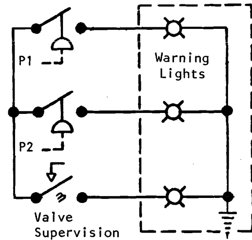
Detail "C" - Electrical Supervision
