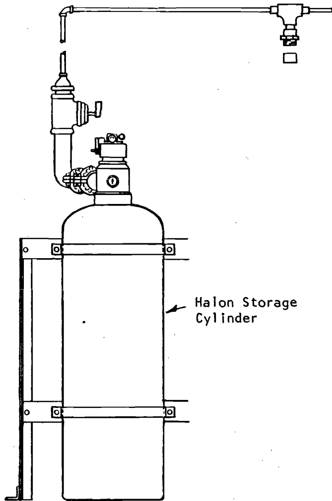
Detail "A" Schematic Typical Halon Supply
