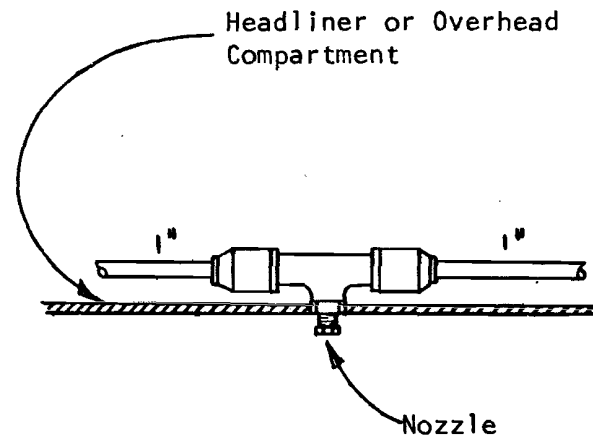
Detail "B" Schematic Typical Nozzle Head Installation
