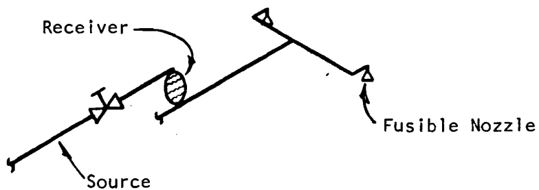
Detail "A" Typical Nozzle and Piping Schematic
