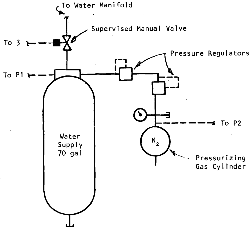
Detail "A" - Typical 70 gal Water Supply
