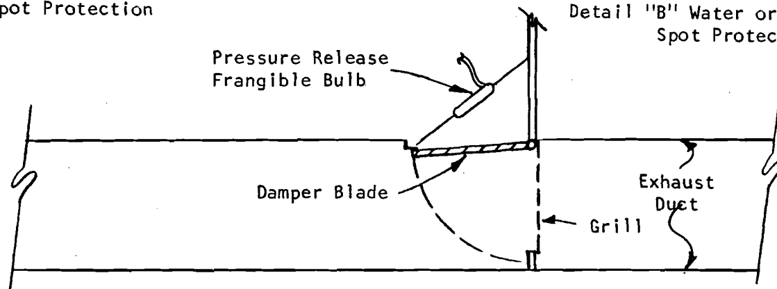
Detail "C" Typical Damper Installation In Lavatory Exhaust (Schematic Only)
