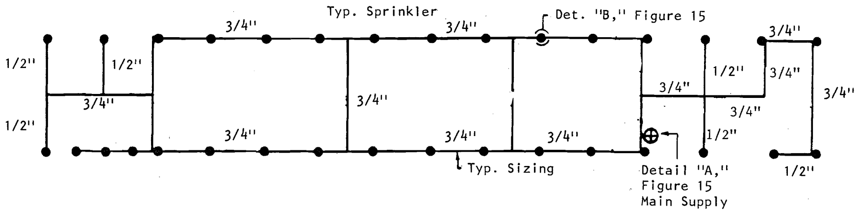
AUTOMATIC SPRINKLER AND TUBING PLAN
