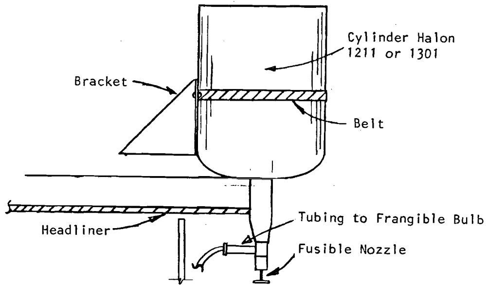
Detail "A" Halon Spot Protection
