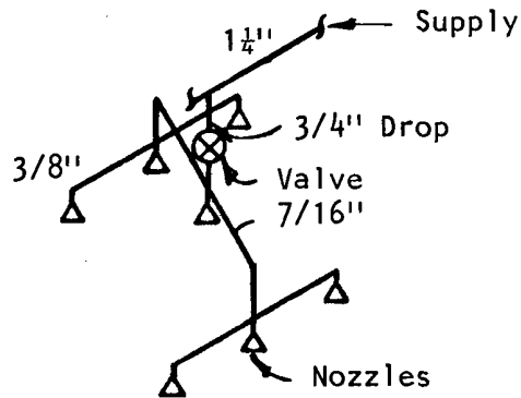
Detail "A," Typical Nozzle and Piping Schematic
