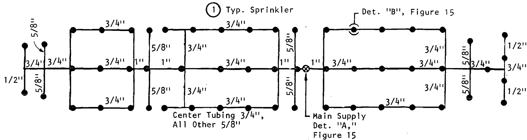
AUTOMATIC SPRINKLER AND TUBING PLAN
