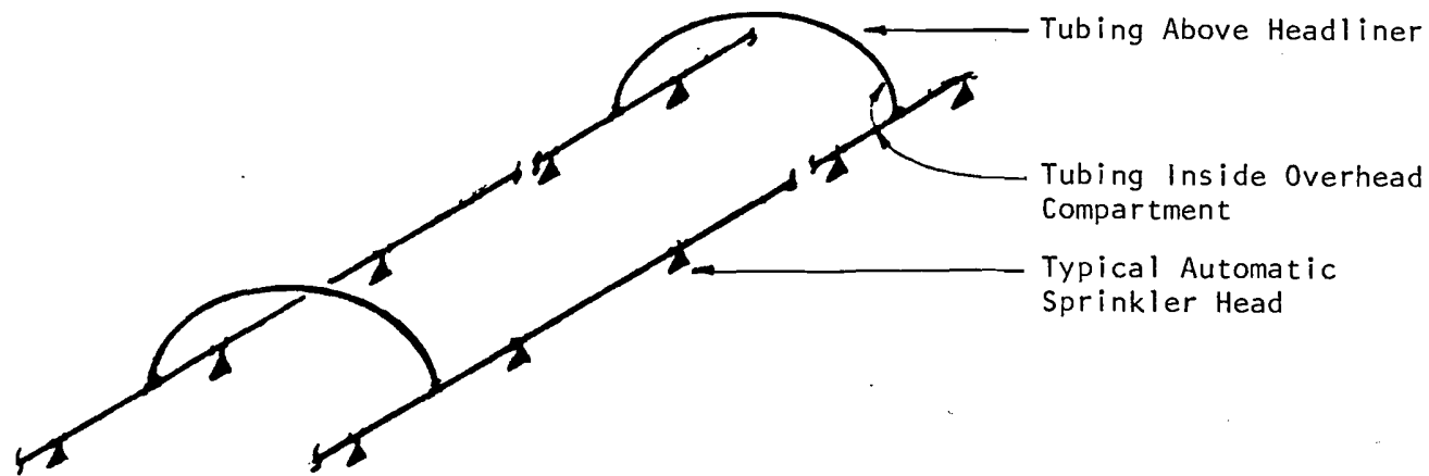
SPRINKLER AND TUBING SCHEMATIC
