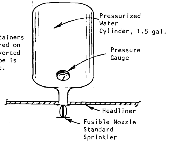
Detail "B" Water or Water/AFFF Spot Protection
