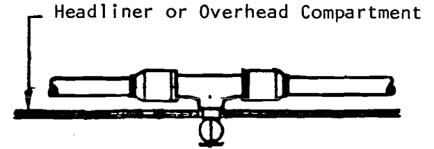
Detail "B" - Typical Sprinkler Head Installation
