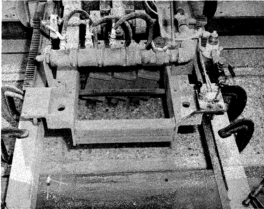
FIGURE 7. MACHINE FOR INSTALLING REFLEX-PERCUSSIVE GROOVES IN THE TEST SECTIONS
