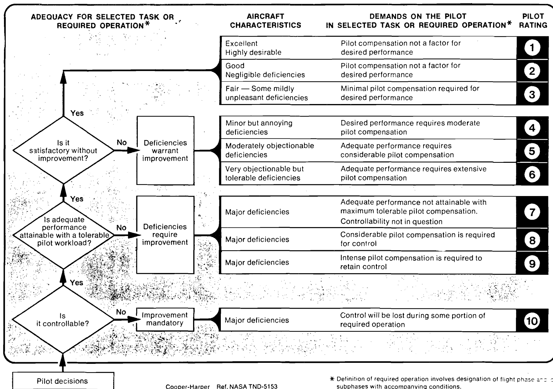
Figure 1a. Cooper-Harper Pilot Rating Scale (Reference 7)
