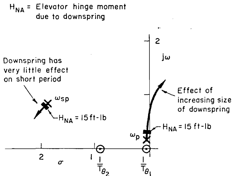
Figure 11. Effect of Increasing Downspring on the Phugoid Mode
