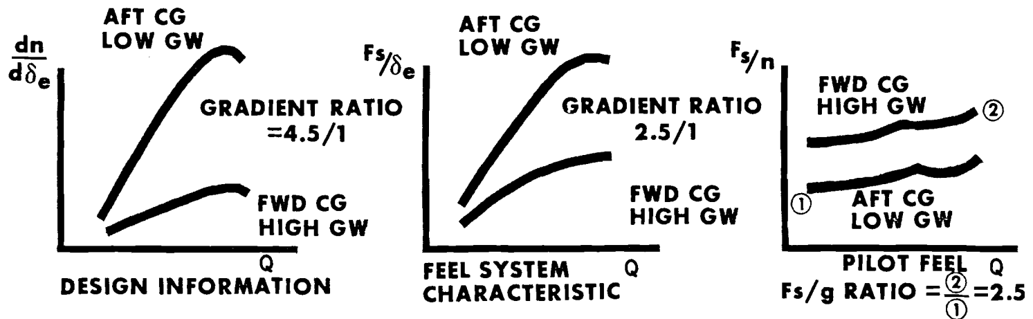
Figure 20. The 727 Feel System; and Empirical CG Computer System (From Reference 28)
