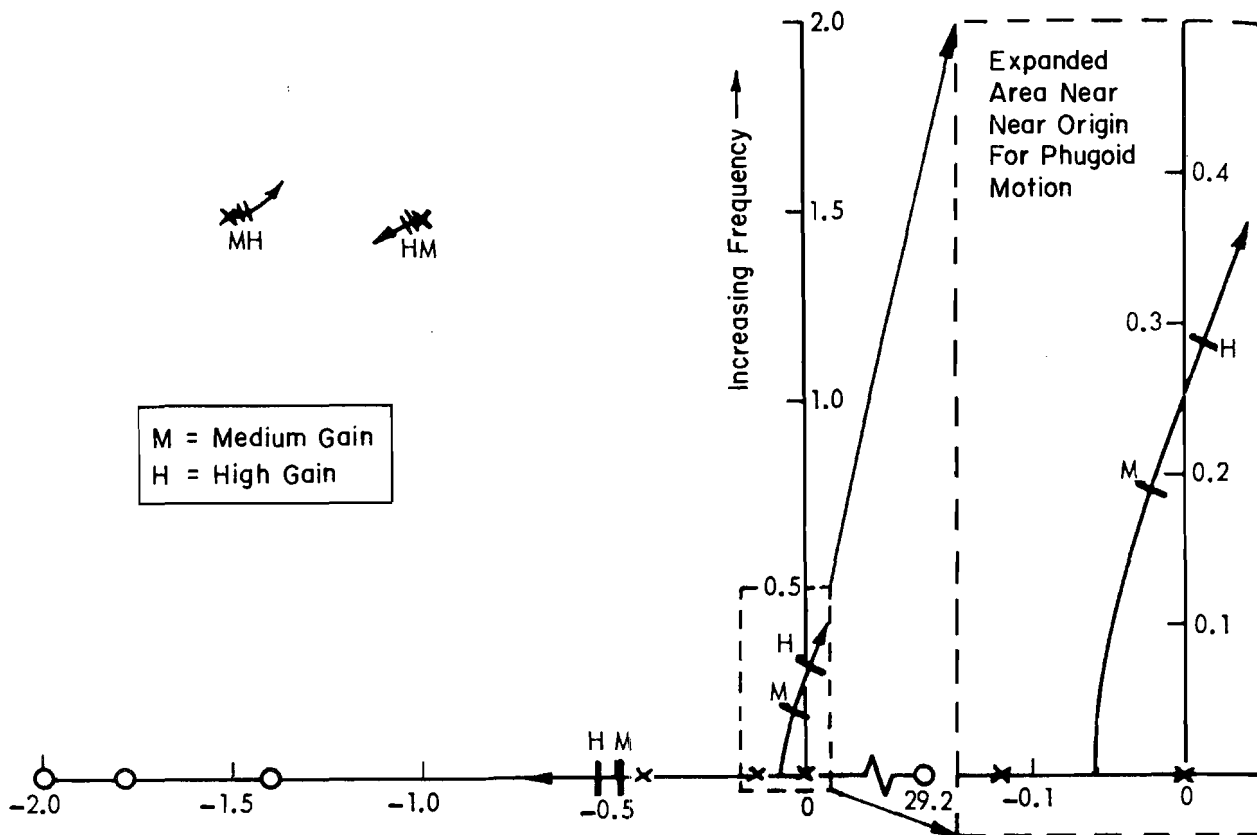
a) Root locus showing the effect of increasing stick force/speed gradient ( u \rightarrow \delta_e gain) on phugoid mode.
