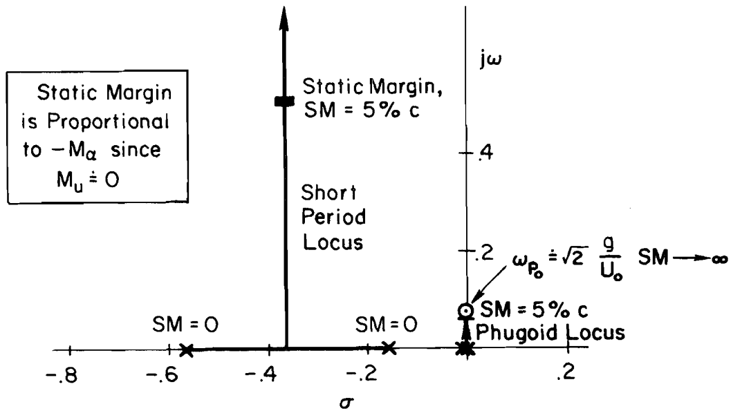
a) Root Loci For Stable Static Margin Variation ( M_\alpha < 0 )
