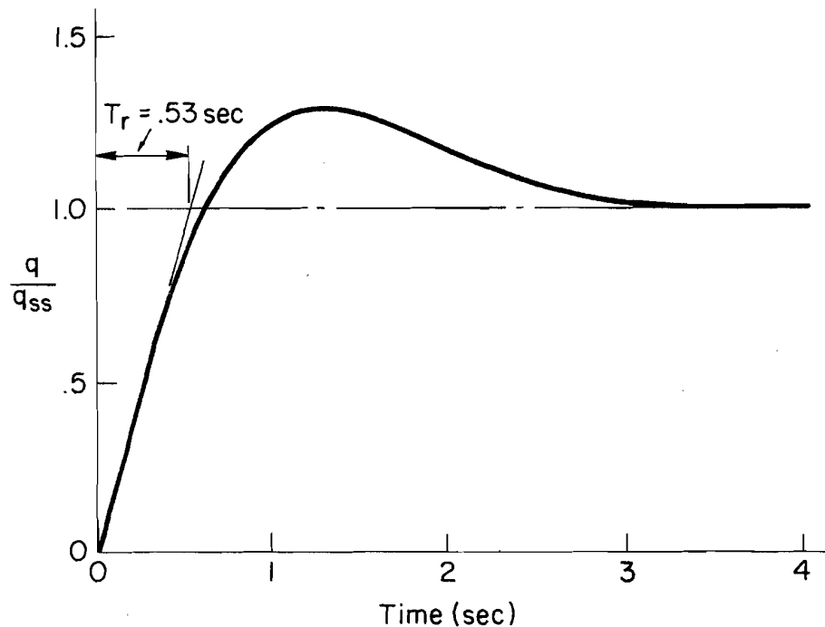
Figure 17. Pitch Rate Response to Step Pitch Rate Command for the Augmented Aircraft in Cruise Flight
