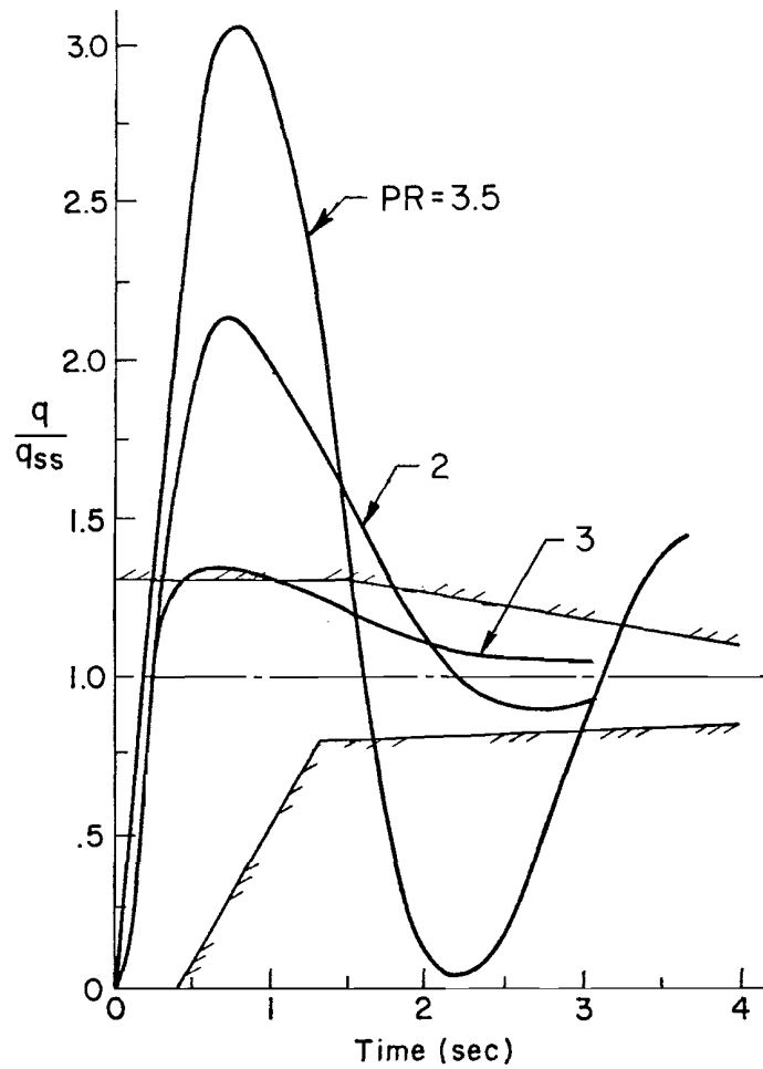
a) Good Conventional Configurations Which do not Meet Exemplary Pitch Rate Requirement
