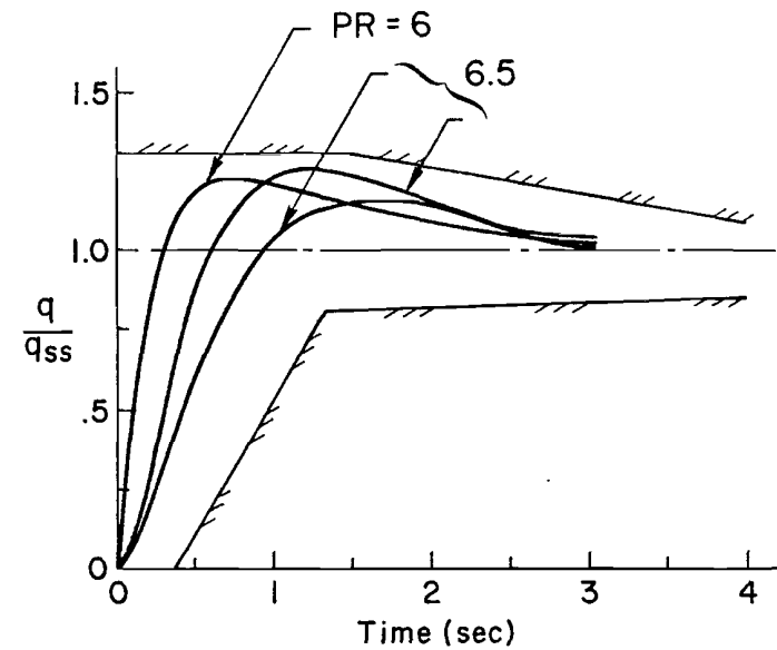
b) Poor Conventional Configurations Which Satisfy the Exemplary Pitch Rate Requirement
