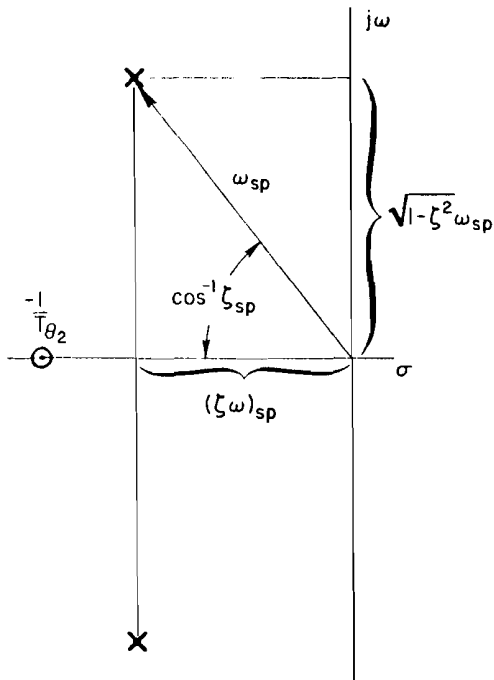
a) s -Plane Root Plot for q/\delta
