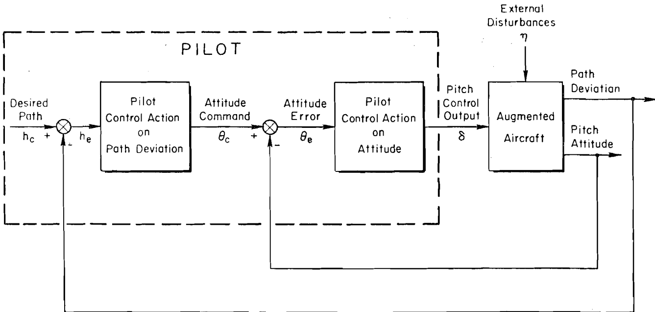
Figure 4. Closed-Loop Pilot-Aircraft System for Precision Path Control
