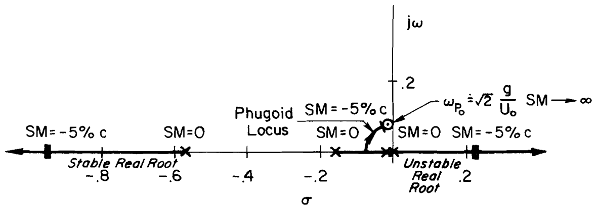
b) Root Loci For Unstable Static Margin Variation ( M_\alpha > 0 )
