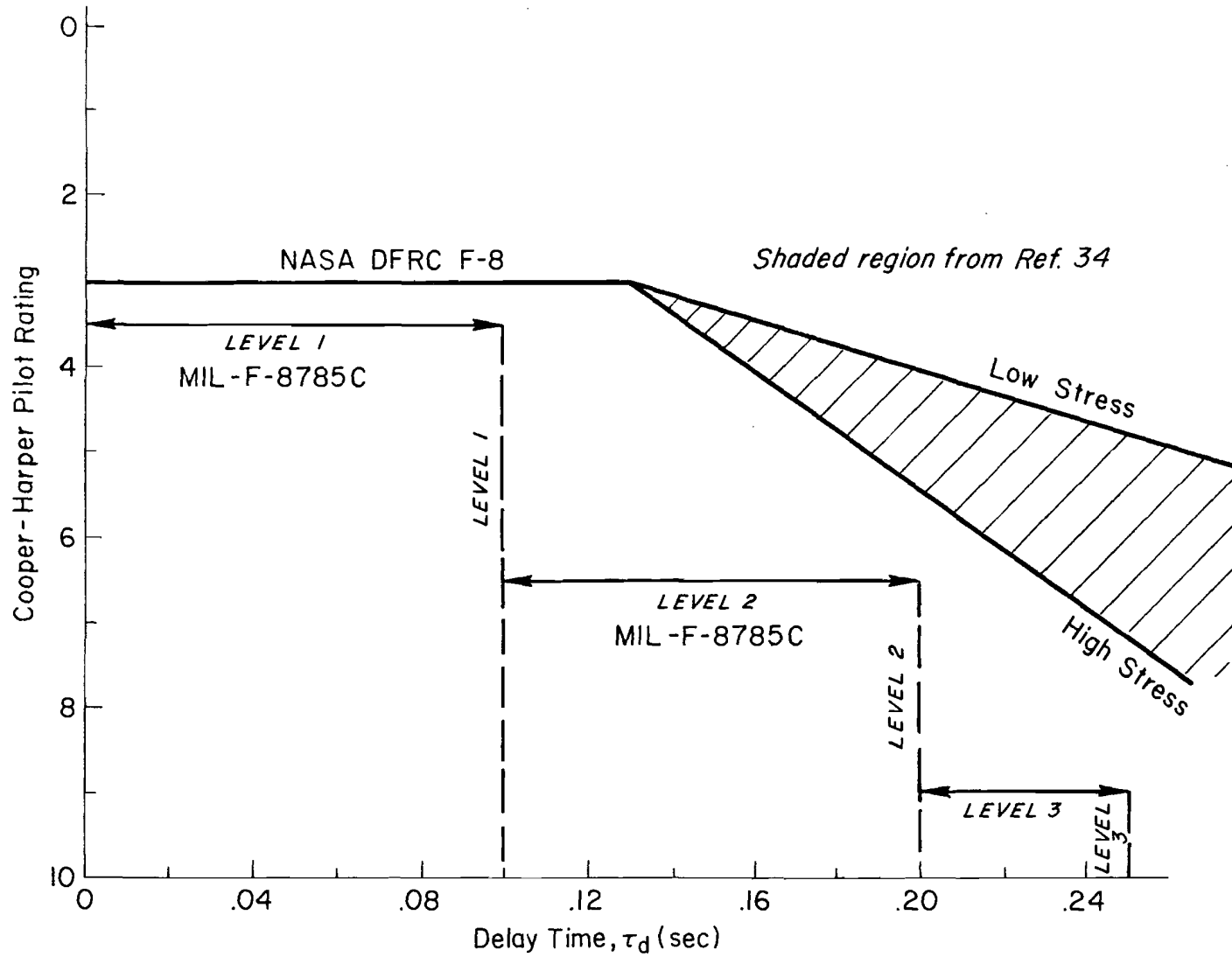
Figure 25. Comparison of MIL-F-8785C Time Delay Requirements with Data from Ref. 34
