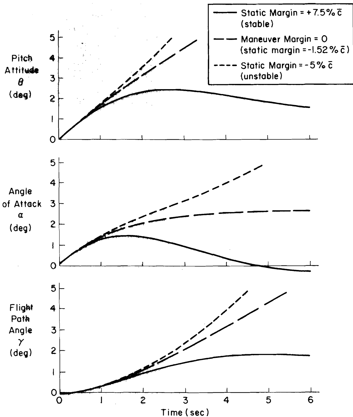
Figure 11. Generic RSS Transport Short-Period Motions for Cruise Conditions ( M = 0.74 , h = 38,000 ft); Input \delta_H = -1 deg/sec Impulse
