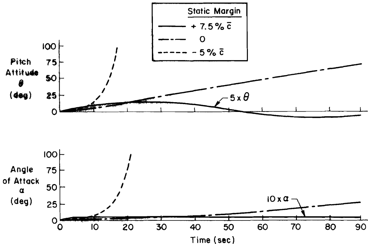
Figure 12. Generic RSS Transport Three-Degree-of-Freedom Responses for Cruise ( M = 0.74 , h = 38,000 ft); Input \delta_H = -1/10 deg Step
