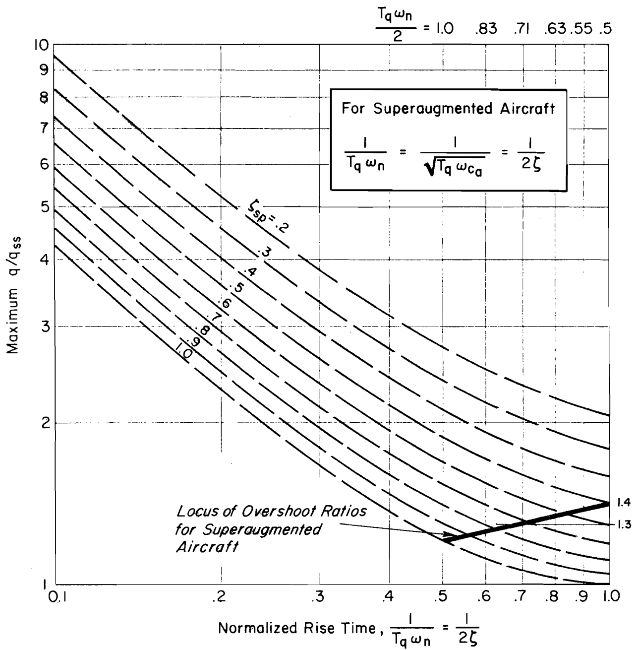
Figure 18. Maximum Pitch Rate Overshoot Variation for Superaugmented Aircraft
