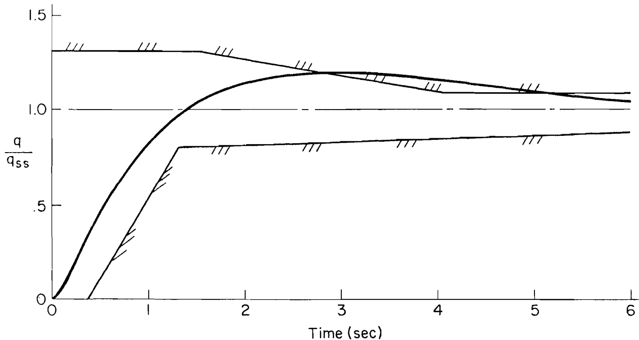
Figure 23. A Simulated Superaugmented Airplane Response for Approach and Landing (Ref. 29); 1/T_{\theta 2} = 0.53 \text{ sec}^{-1} , 1/T_q = 1 \text{ sec}^{-1}
