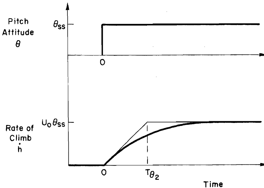
Figure 7. Path Rate Response to Attitude Change
