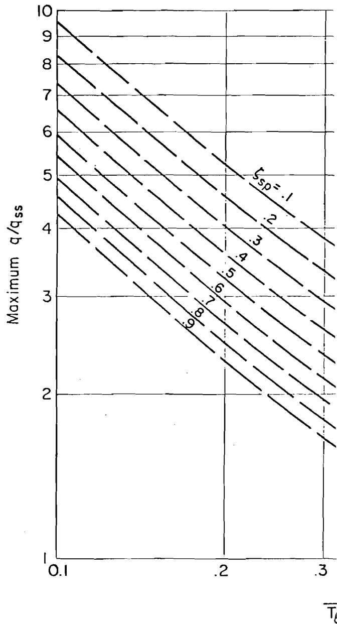
Figure 14. Pitch Overshoot Variation Conventional Aircraft (General)
