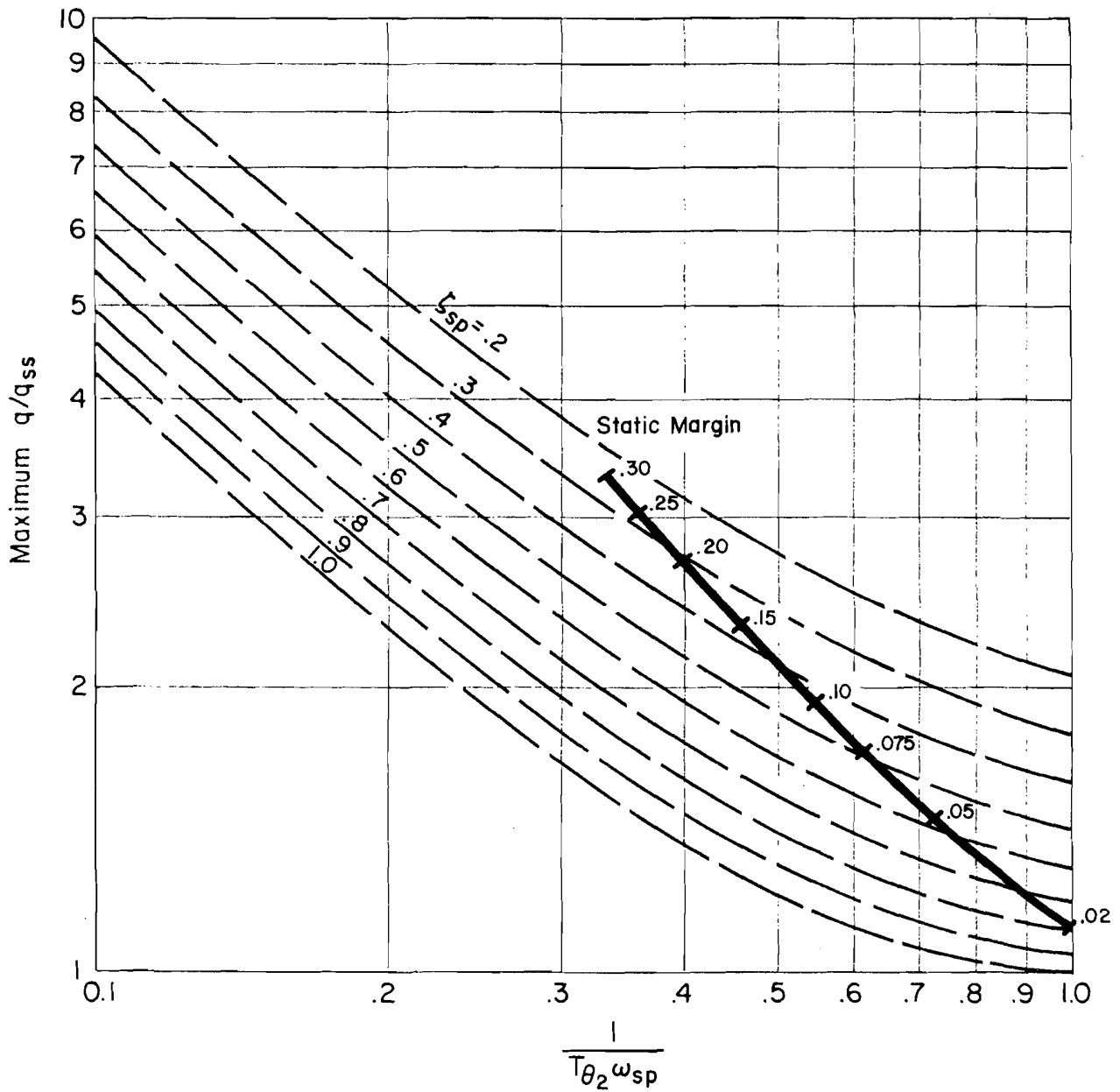
Figure 14. Pitch Overshoot Variation with Static Margin for Conventional Aircraft (Generic Aircraft in Cruise)
