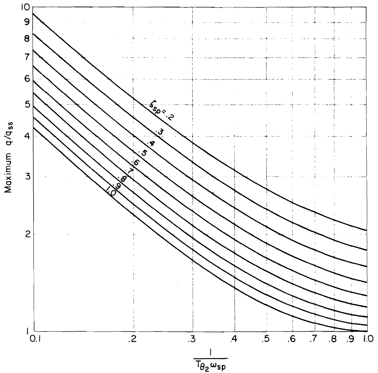
Figure 9. Maximum Pitch Rate Overshoot for Step Control Input
