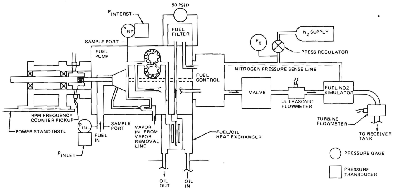
FIGURE 44. ENGINE FUEL SCHEMATIC TEST
