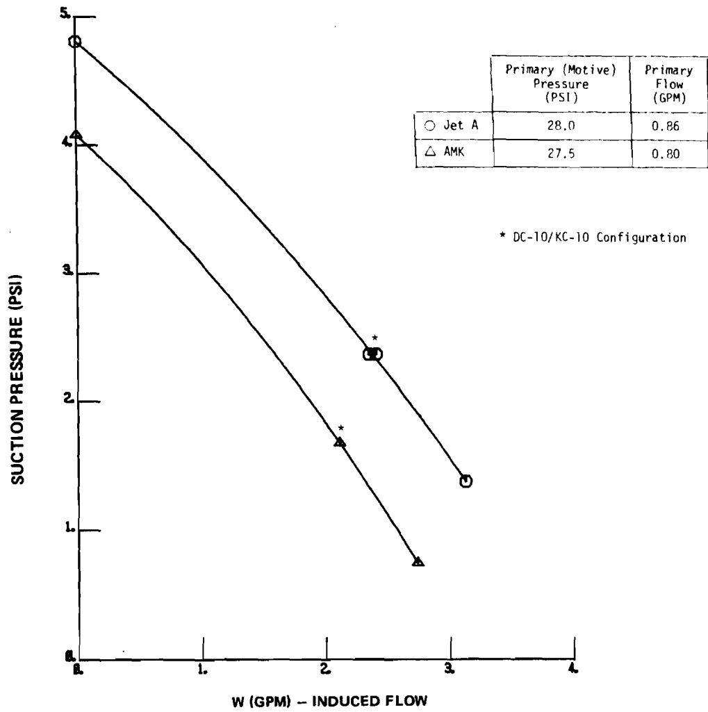
FIGURE 16. SCAVENGE JET PUMP PERFORMANCE
