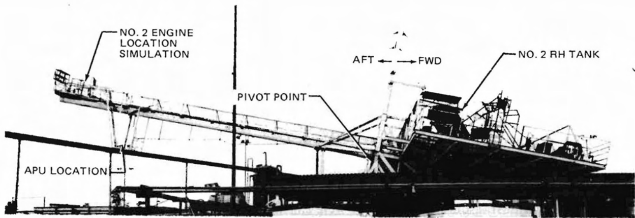
FIGURE 41. FUEL FEED TEST RIG, ELEVATION VIEW
