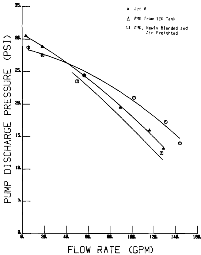
FIGURE 27. BOOST PUMP PERFORMANCE, CONFIGURATION 2
