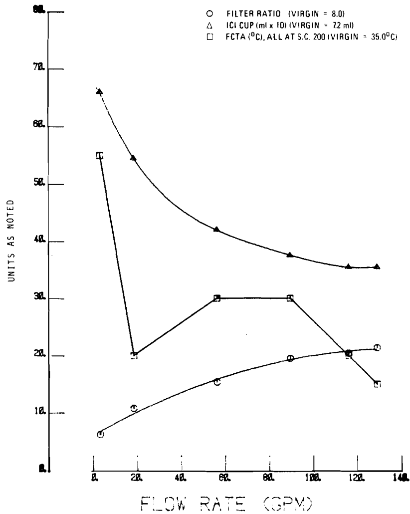
FIGURE 28. 12K AMK FUEL QUALITY, CONFIGURATION 2
