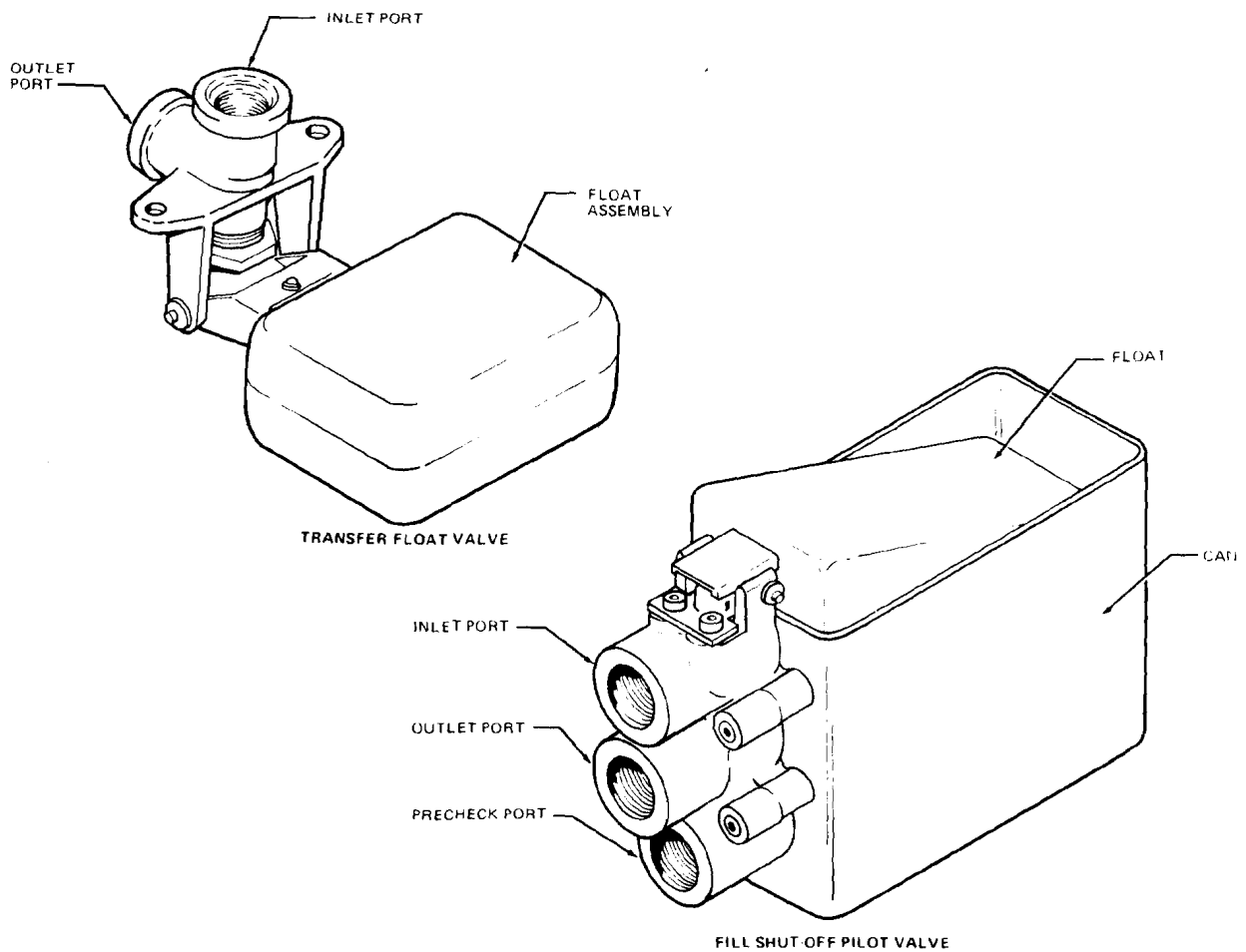
FIGURE 5. FLOAT VALVES
