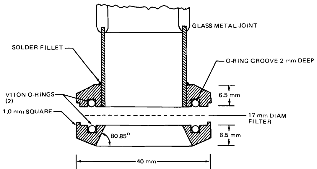
FIGURE A1. DESCRIPTION OF FILTER SCREEN ASSEMBLY
