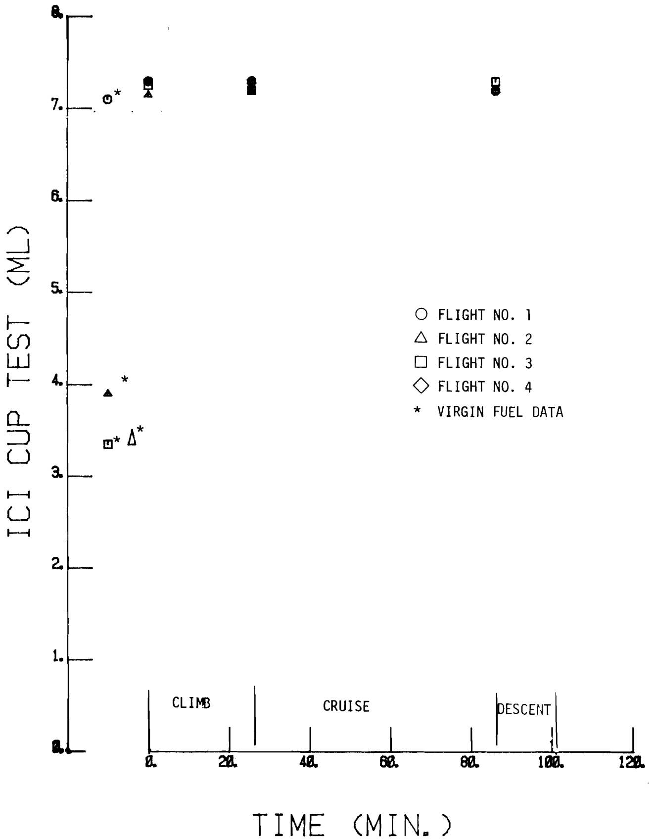
FIGURE 58. ENGINE INTERSTAGE, ICI CUP TEST
