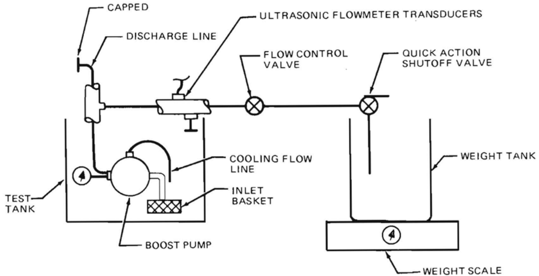
FIGURE 46. ULTRASONIC FLOWMETER CALIBRATION SETUP
