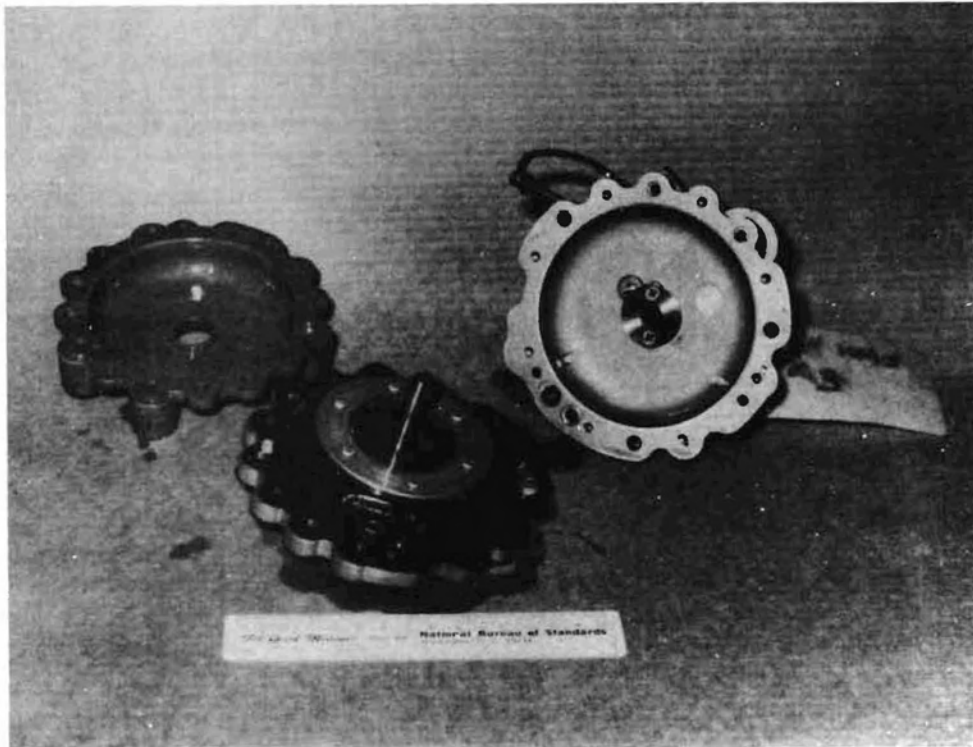
FIGURE 37. DISASSEMBLED FILL VALVE CONTROLLER
