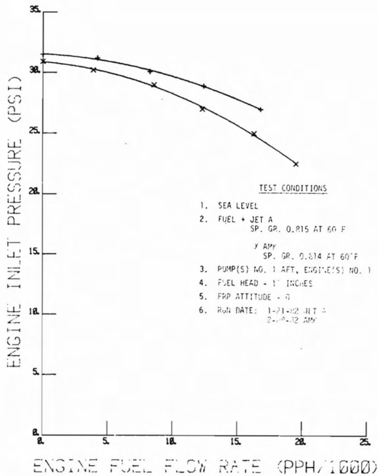
FIGURE 48. FUEL FEED SYSTEM PERFORMANCE – TANK BOOST PUMP OPERATING
