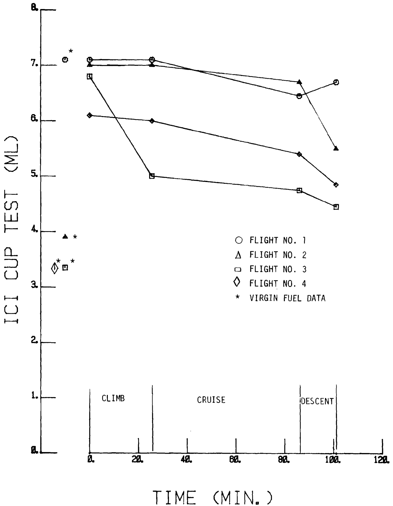
FIGURE 52. TANK AMK, ICI CUP TEST
