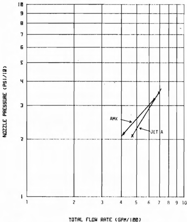
FIGURE 36. DC-10 FILL SYSTEM PERFORMANCE, SINGLE NOZZLE FILLING NO. 1 TANK
