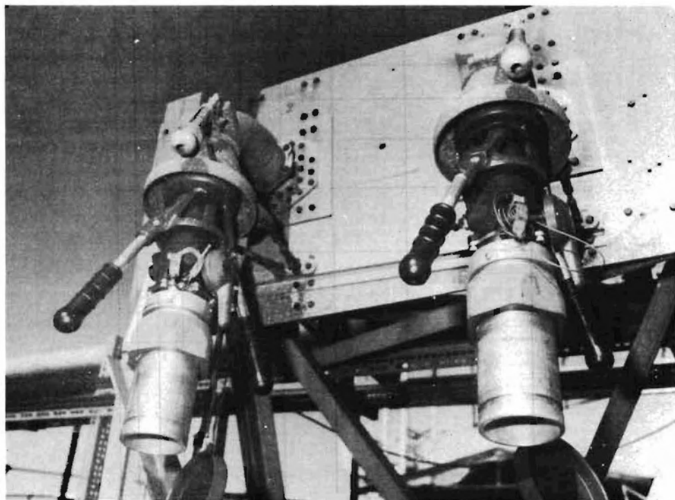
FIGURE 35. ADAPTERS AND FUEL NOZZLE ASSEMBLIES
