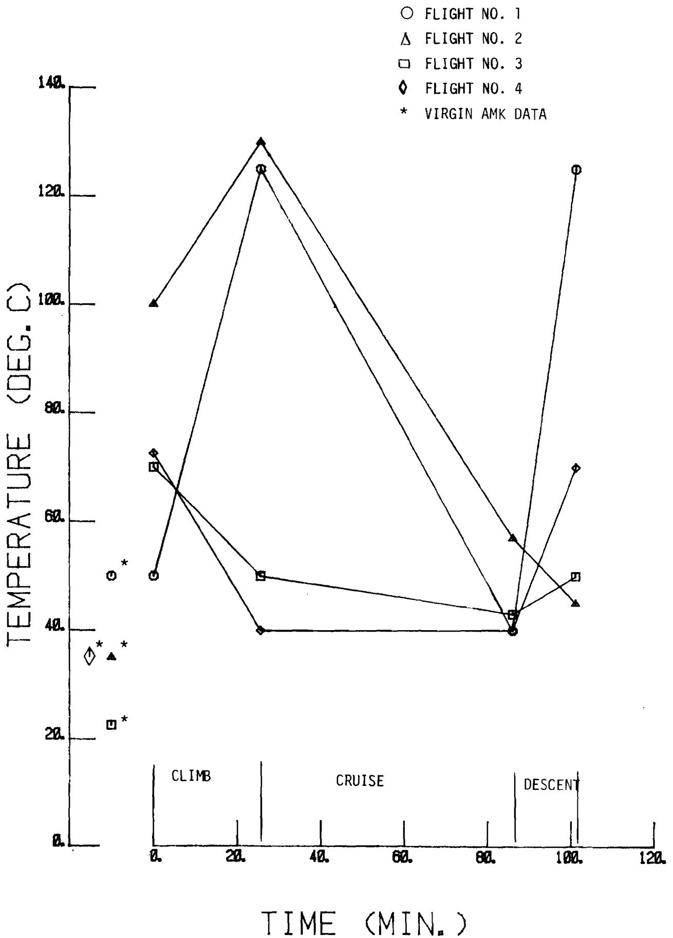
FIGURE 53. TANK AMK, FCTA TEMPERATURE
