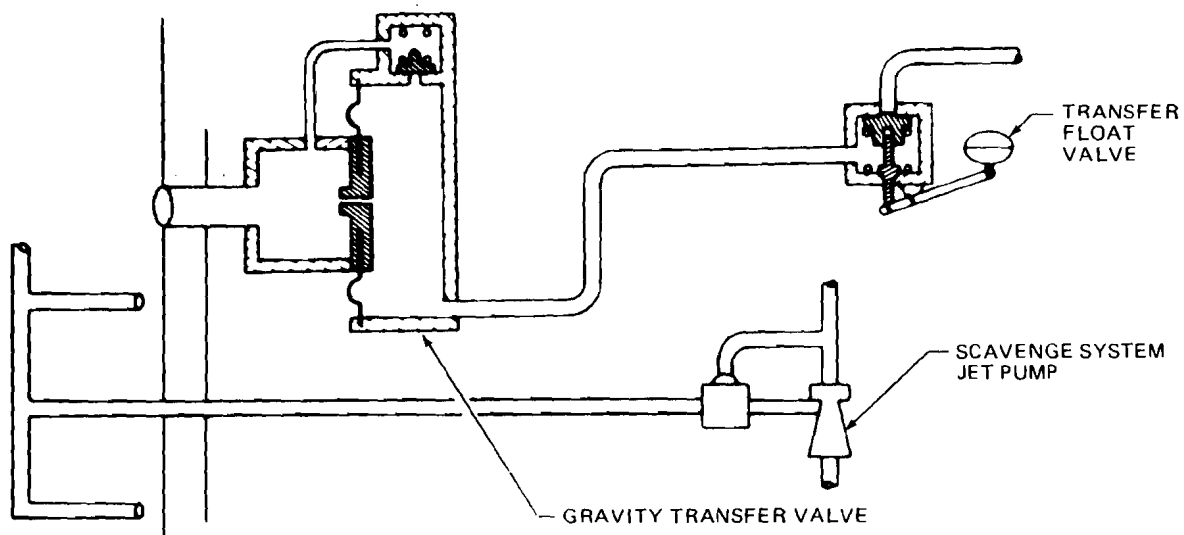
FIGURE 7. OUTBOARD COMPARTMENT GRAVITY TRANSFER AND SCAVENGE SYSTEMS
