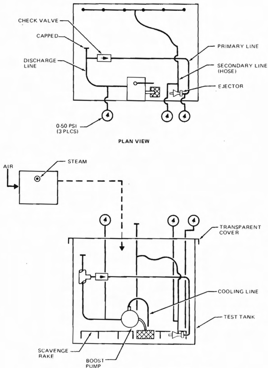
FIGURE 29. WATER TEST SCHEMATIC
