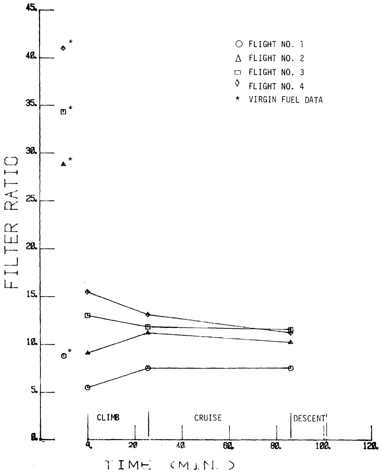
FIGURE 54. ENGINE INLET, FILTER RATIO
