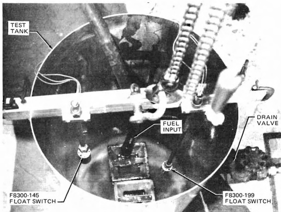
FIGURE 13. FLOAT SWITCH TEST SETUP
