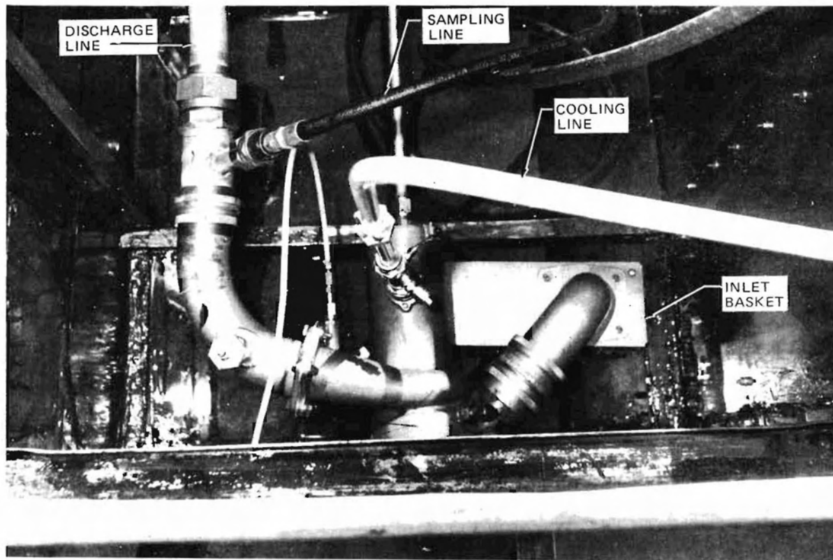
FIGURE 22. CONFIGURATION 2, BOOST PUMP TEST
