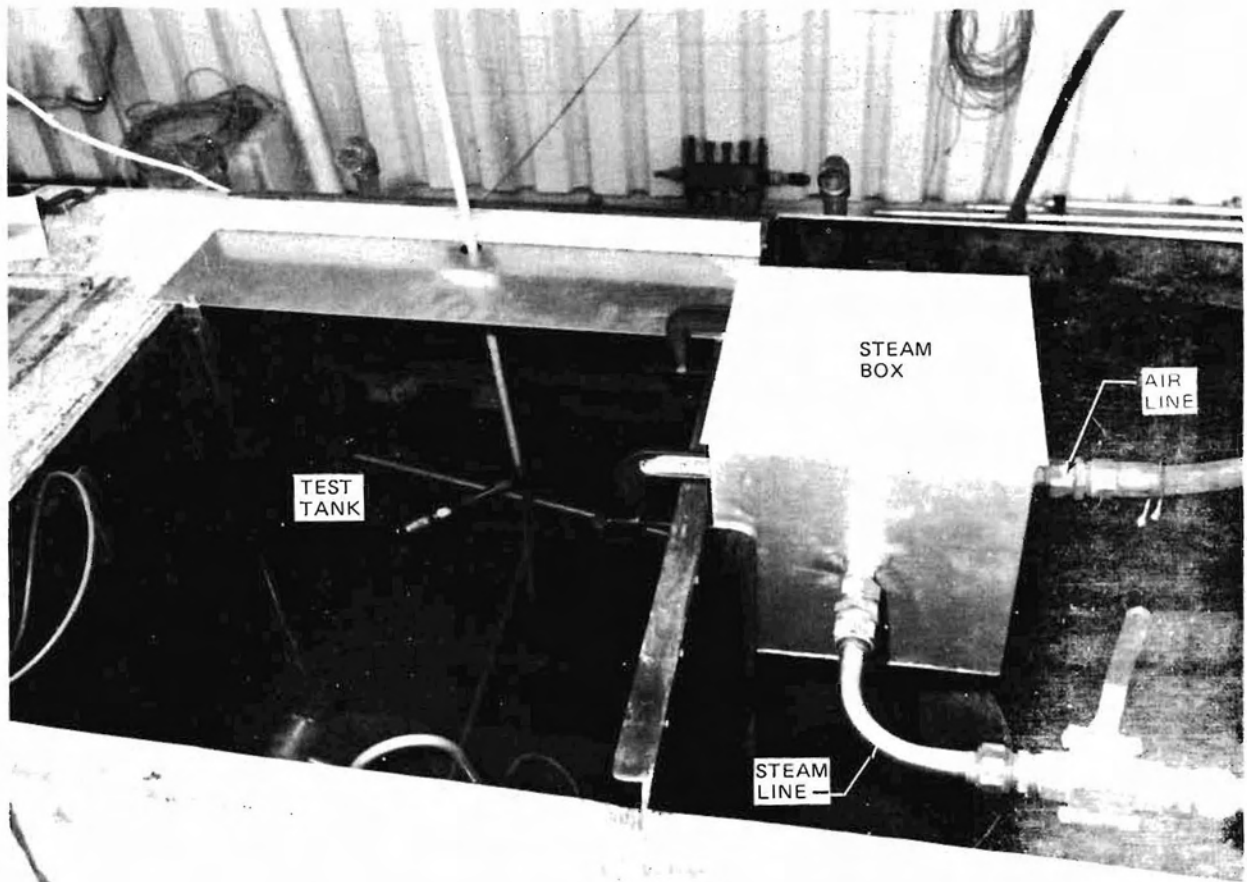
FIGURE 31. TEST TANK AND STEAM BOX, WATER TEST
