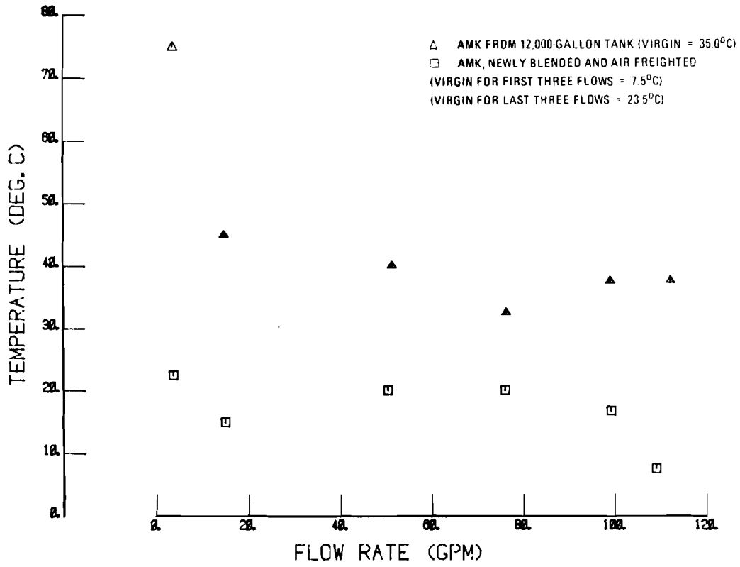
FIGURE 26. FCTA TEMPERATURE, CONFIGURATION 1
