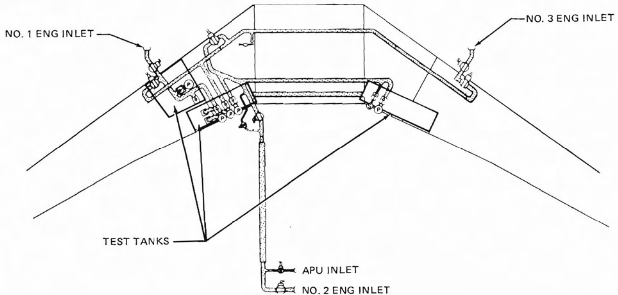
FIGURE 42. DC-10 FUEL FEED SYSTEM SIMULATOR
