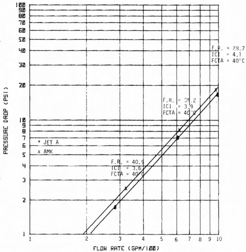
FIGURE 62. KC-10 AERIAL REFUELING NOZZLE/RECEPTACLE TEST
