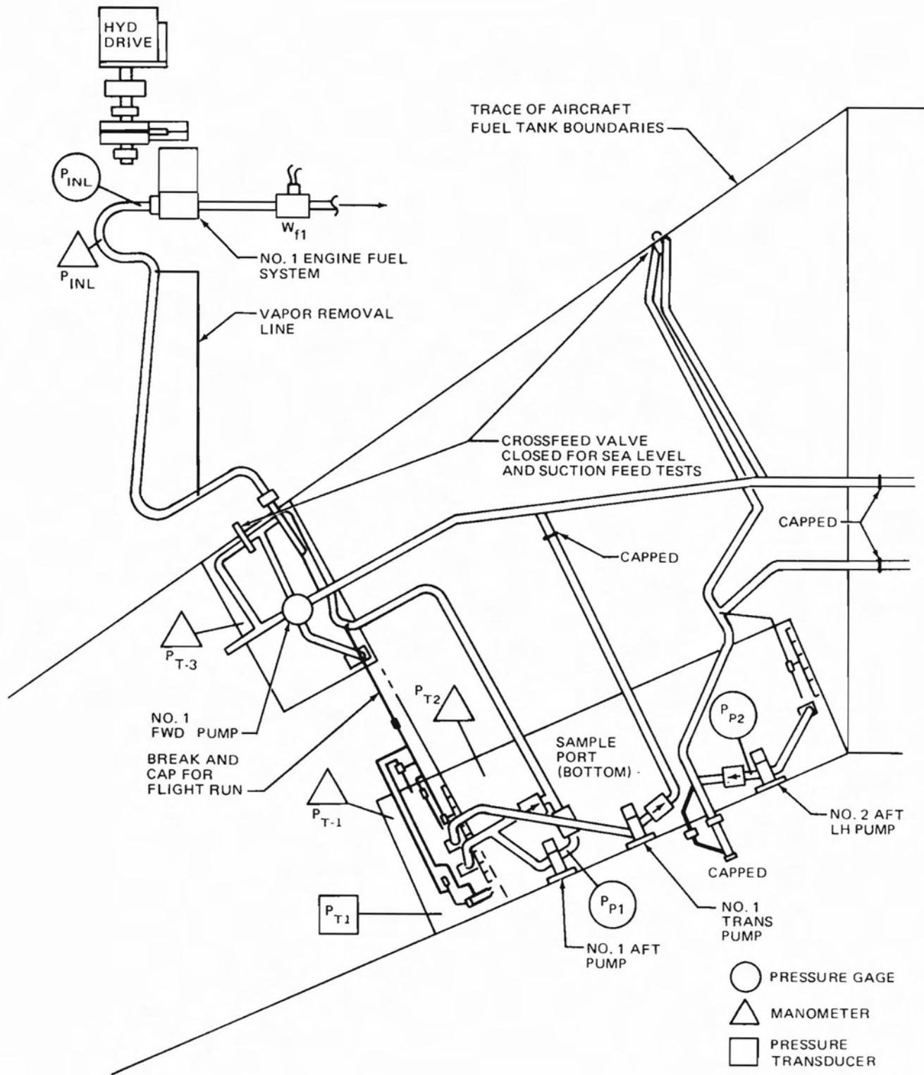
FIGURE 43. FUEL FEED SYSTEM TEST SCHEMATIC – PLAN VIEW
