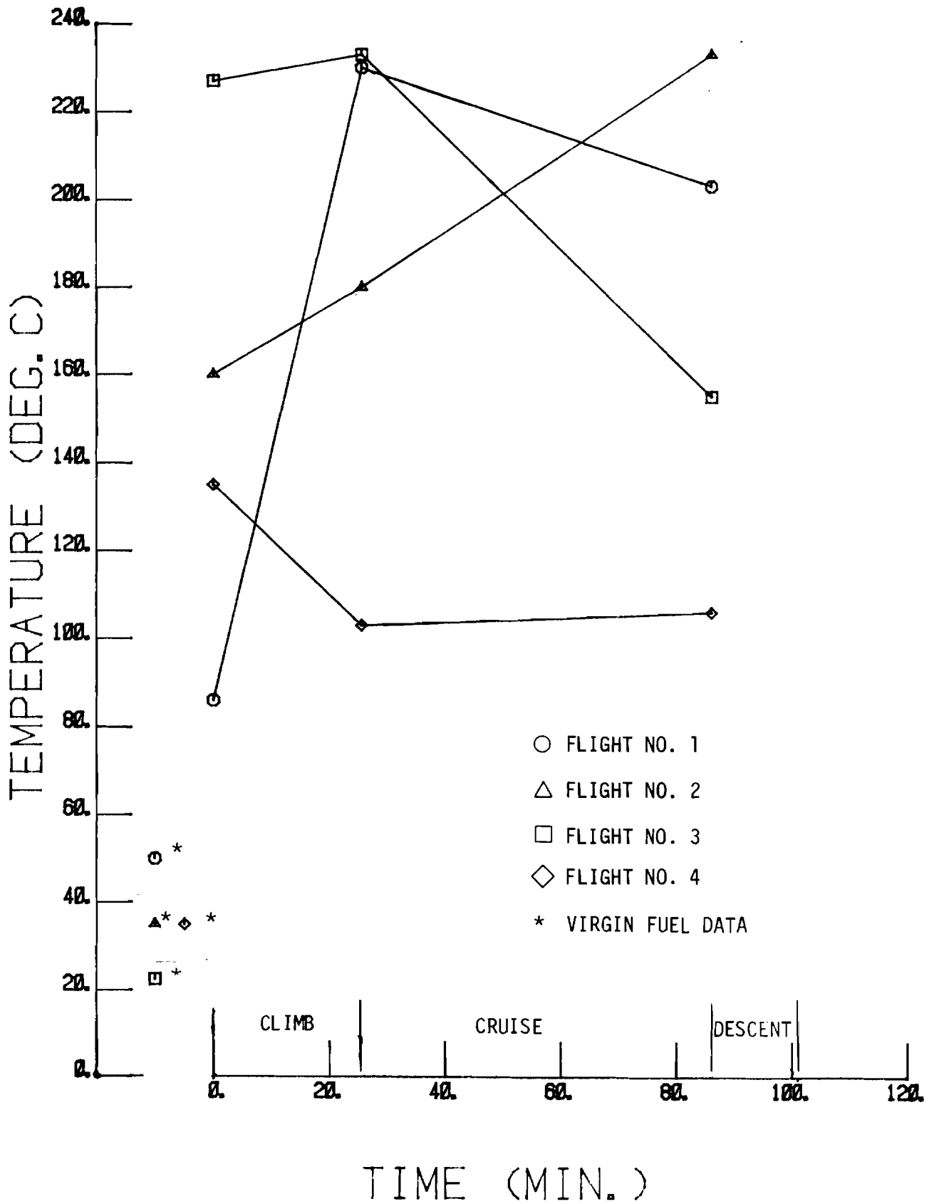
FIGURE 59. ENGINE INTERSTAGE, FCTA TEMPERATURE
