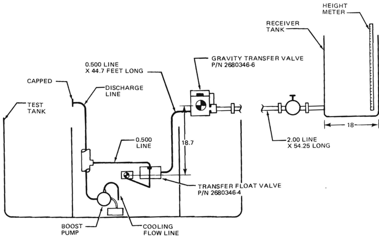
FIGURE 18. TRANSFER VALVE TEST SCHEMATIC
