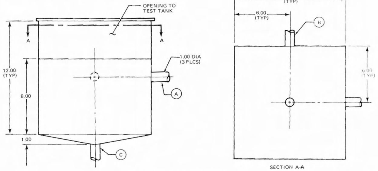
FIGURE 30. STEAM BOX, WATER TEST
