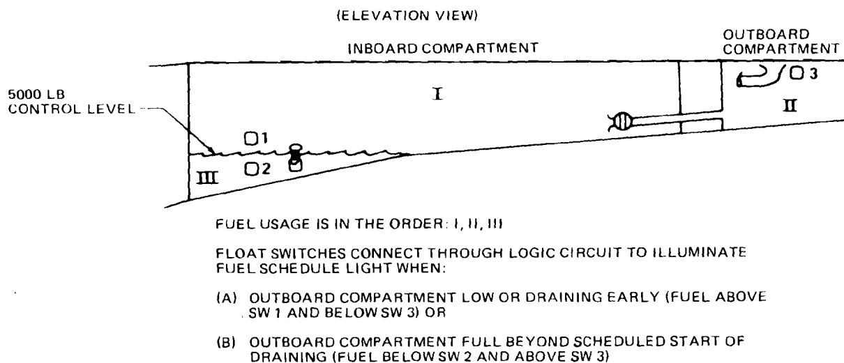
FIGURE 3. OUTBOARD MAIN FUEL TANK, FUEL USAGE SCHEDULE
