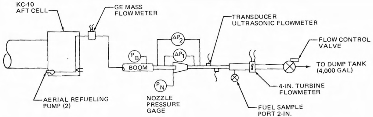
FIGURE 60. KC-10 AERIAL REFUELING NOZZLE/RECEPTACLE TEST SCHEMATIC
