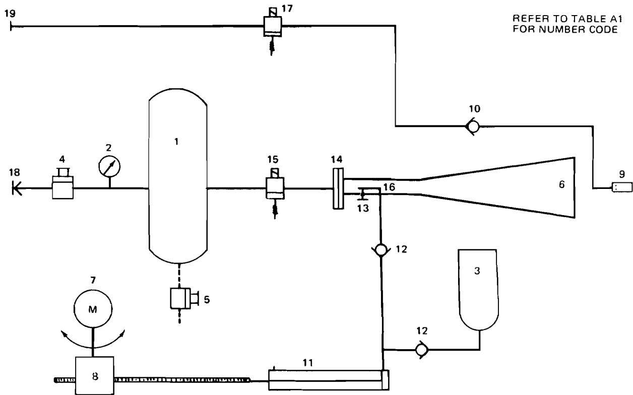
FIGURE A2. FLAMMABILITY COMPARISON TEST APPARATUS (FCTA) SCHEMATIC
