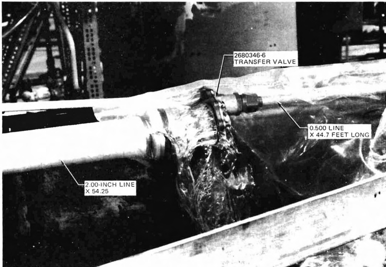
FIGURE 19. GRAVITY TRANSFER VALVE, GRAVITY FLOW
