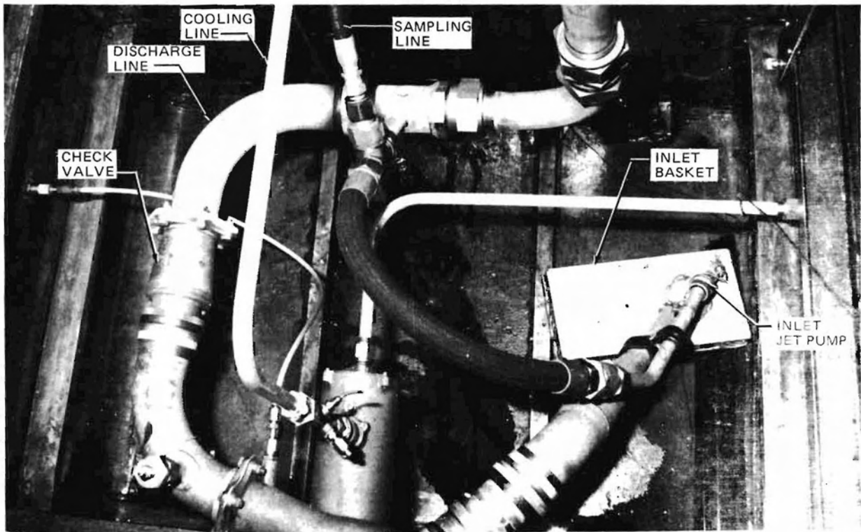
FIGURE 21. CONFIGURATION 1, BOOST PUMP TEST
