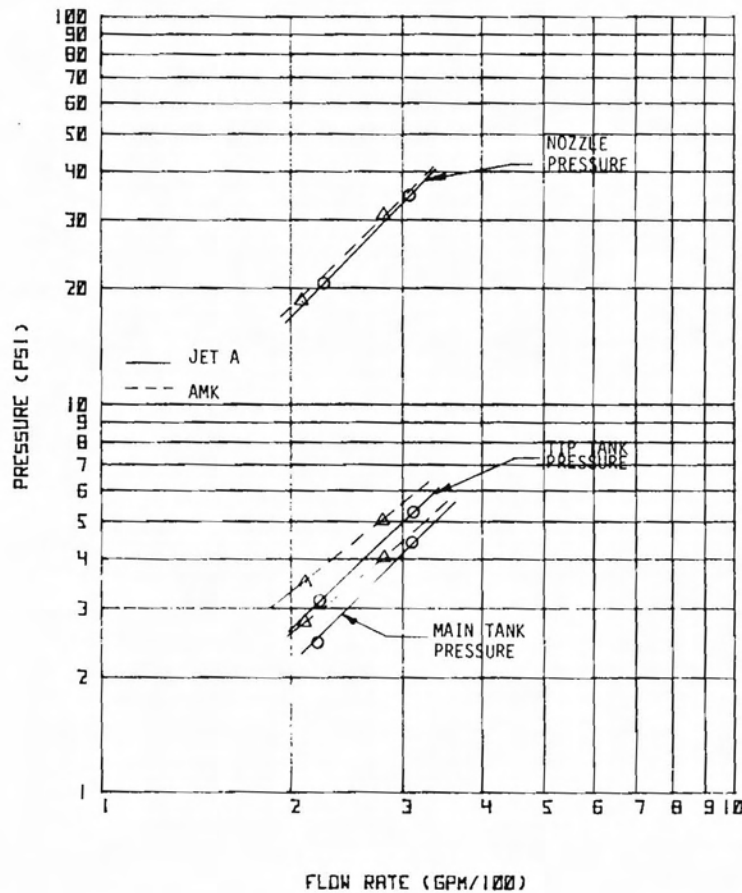
FIGURE 40. VENT SYSTEM PERFORMANCE USING SINGLE FUELING NOZZLE
