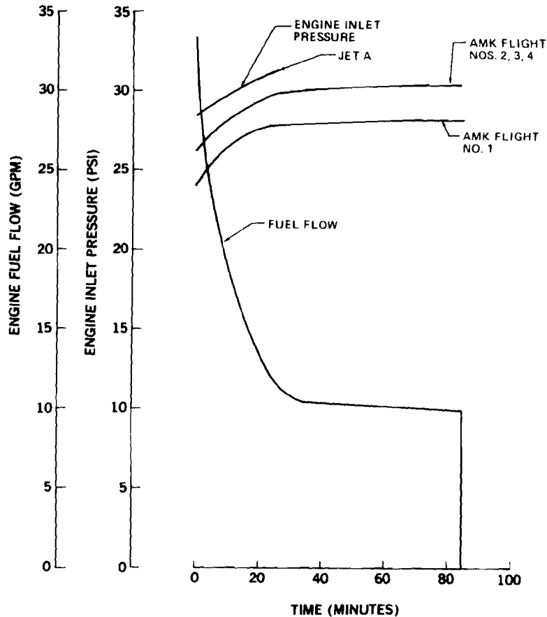
FIGURE 50. FUEL FLOW CHARACTERISTICS DURING SIMULATED FLIGHTS
