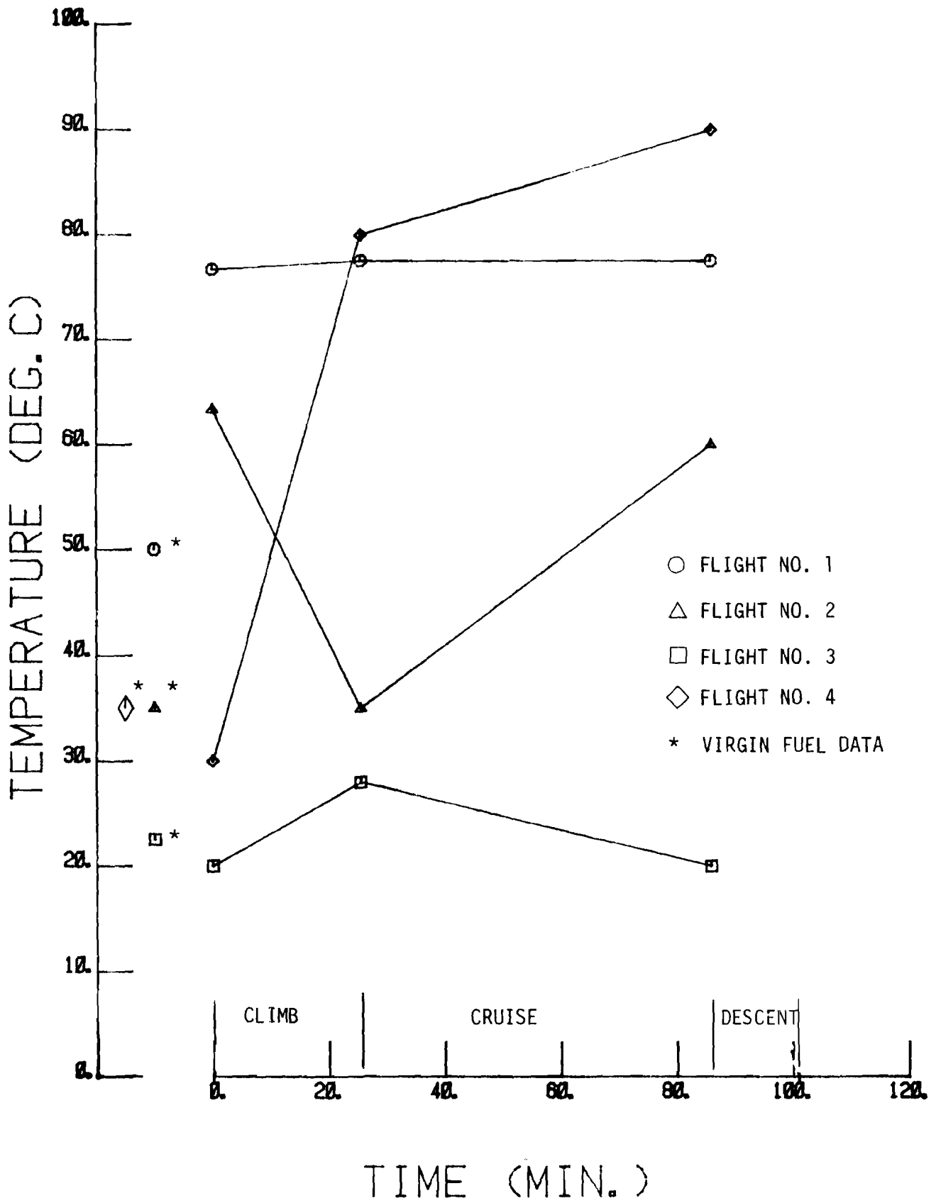
FIGURE 56. ENGINE INLET, FCTA TEMPERATURE
