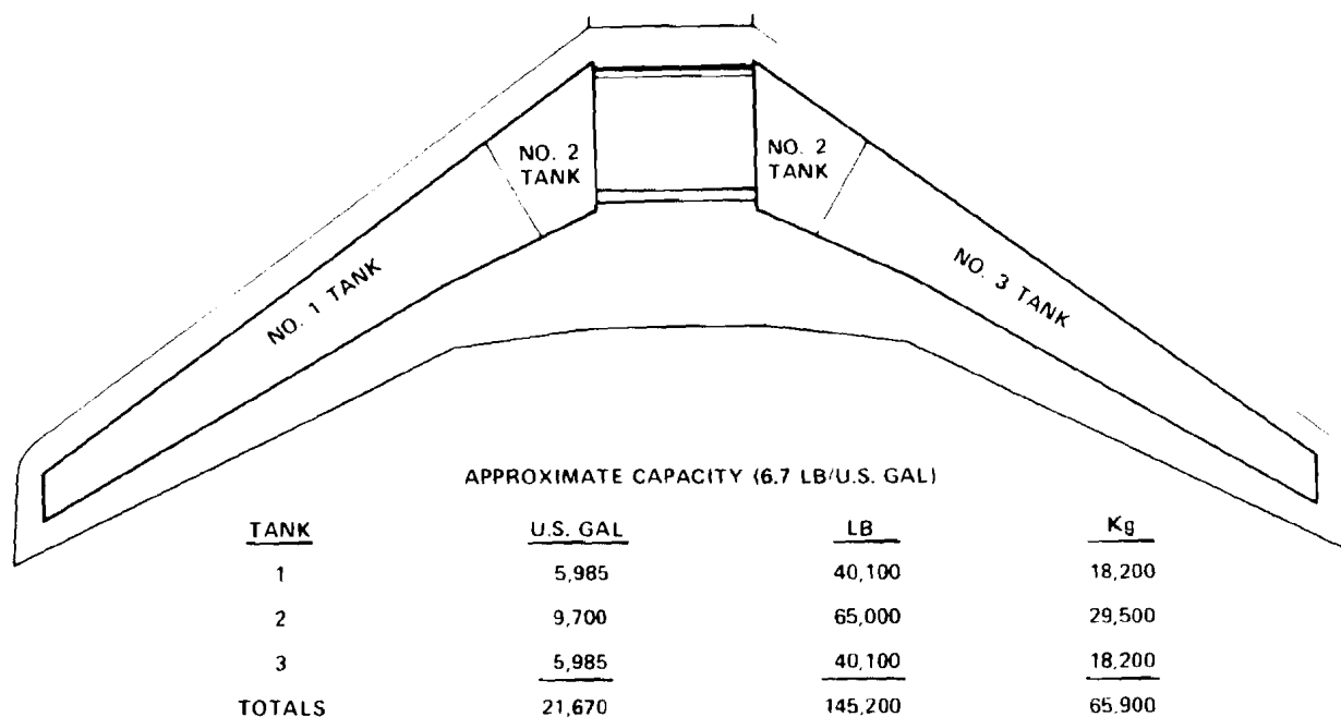
FIGURE 2. FUEL TANKAGE – DC-10 SERIES 10
