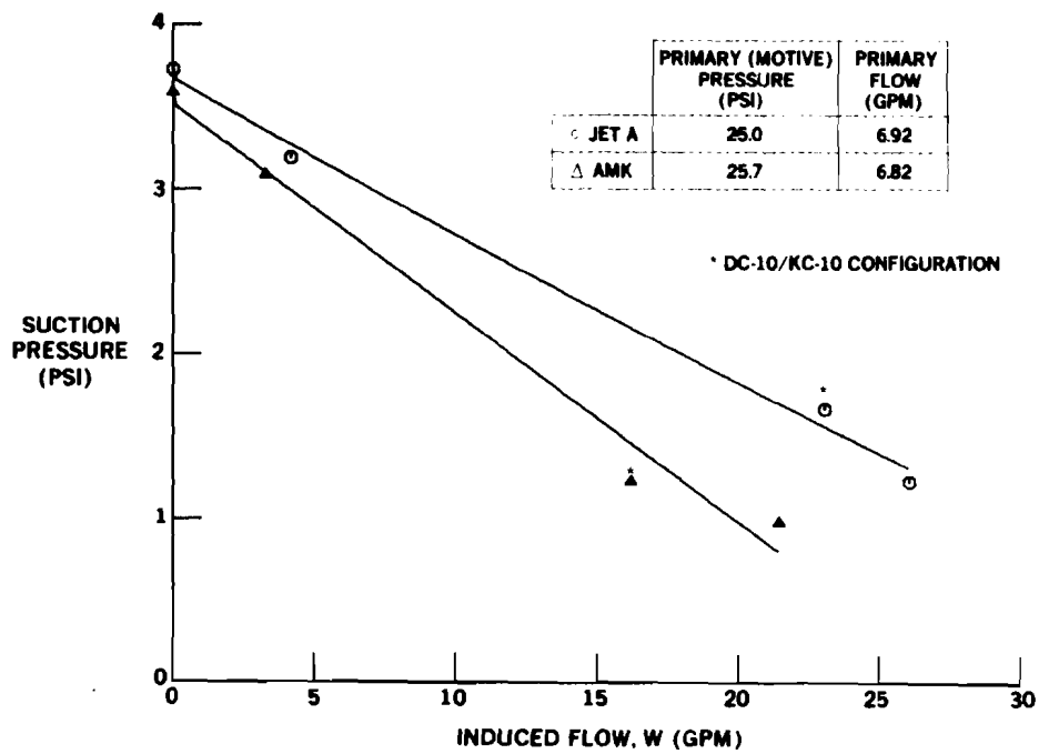
FIGURE 17. TRANSFER JET PUMP PERFORMANCE
