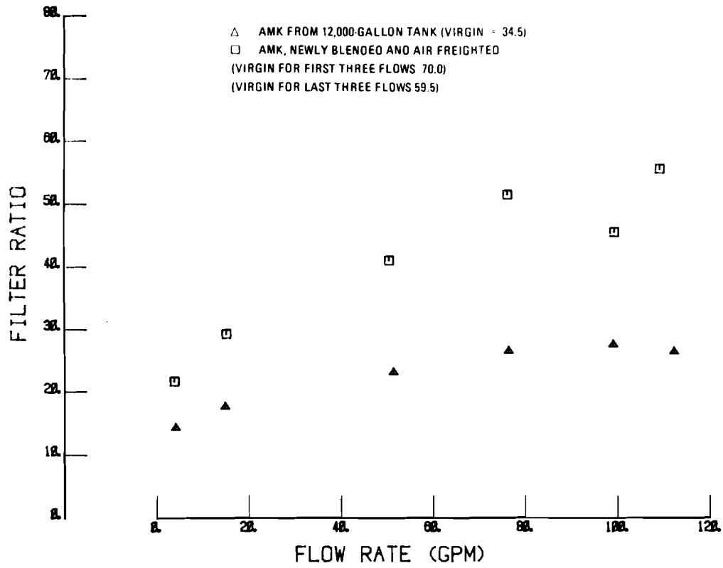
FIGURE 24. FILTER RATIO, CONFIGURATION 1
