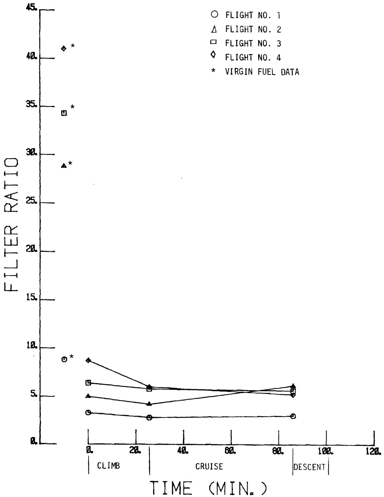
FIGURE 57. ENGINE INTERSTAGE, FILTER RATIO
