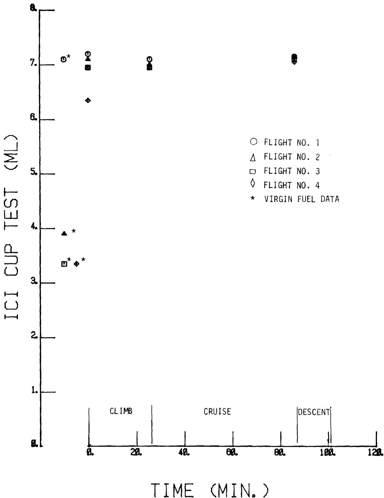
FIGURE 55. ENGINE INLET, ICI CUP TEST
