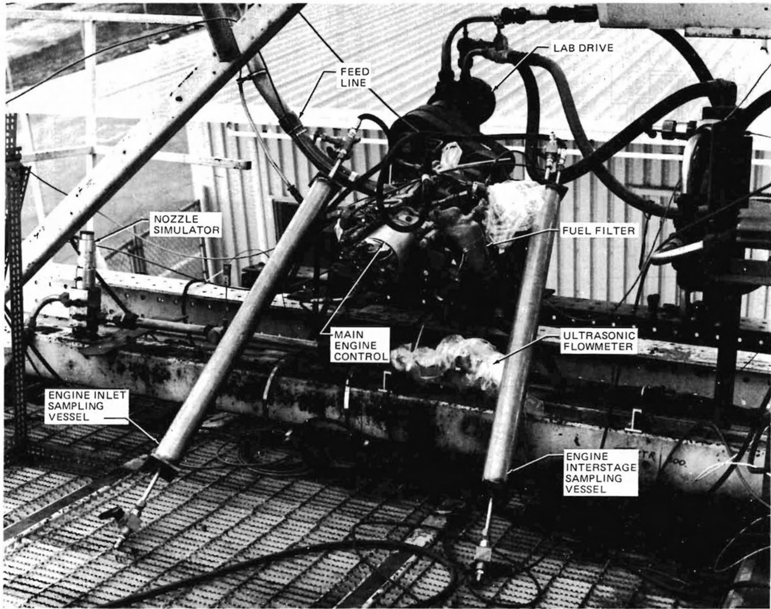
FIGURE 45. SAMPLING AT ENGINE INLET AND INTERSTAGE
