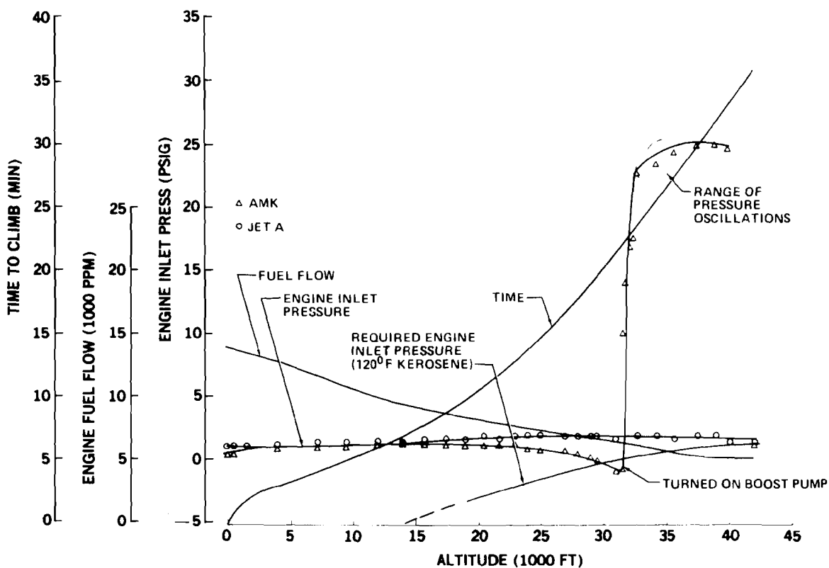
FIGURE 49. SUCTION FEED CLIMB TEST
