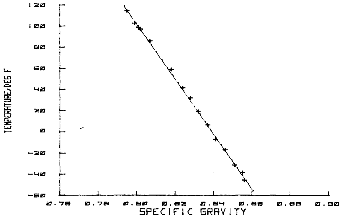
FIGURE B1. AMK, SPECIFIC GRAVITY VERSUS TEMPERATURE
