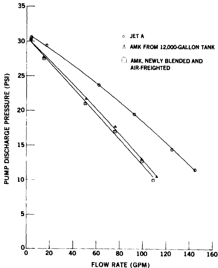
FIGURE 23. BOOST PUMP PERFORMANCE, CONFIGURATION 1.
