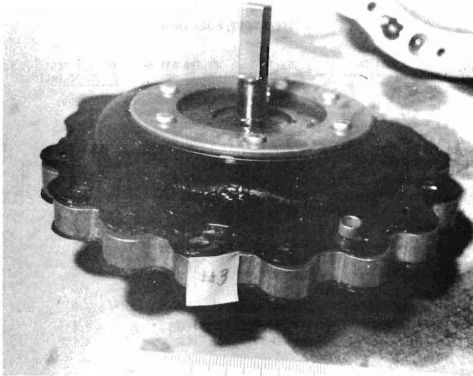
FIGURE 38. GEL FORMATION ON CONTROLLER DIAPHRAGM
