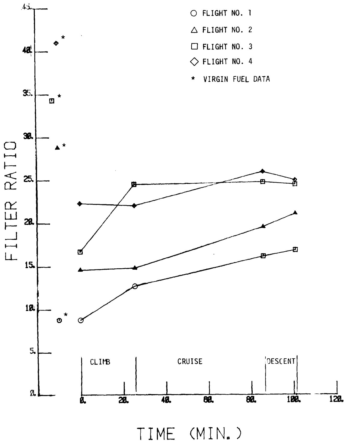
FIGURE 51. TANK AMK, FILTER RATIO
