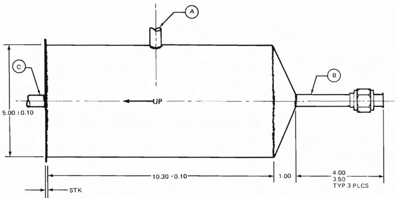
FIGURE 12. SAMPLING VESSEL
