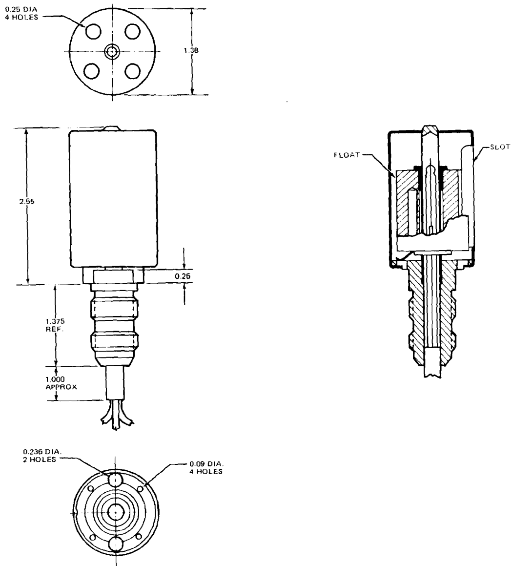
FIGURE 4. FLOAT SWITCH
