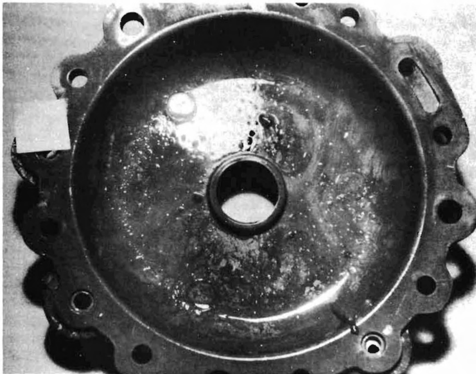
FIGURE 39. GEL GLOBULES ON CONTROLLER HOUSING
