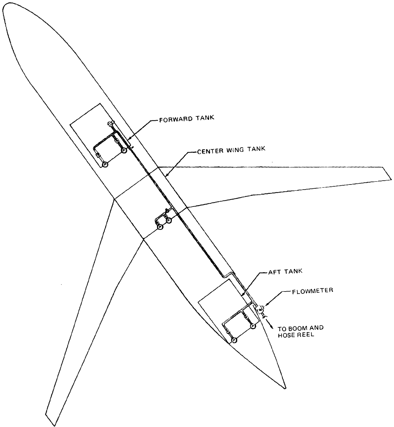
FIGURE 11. KC-10 AERIAL REFUELING
