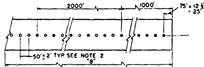
DETAIL "B"
