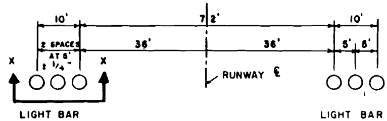
DETAIL A
