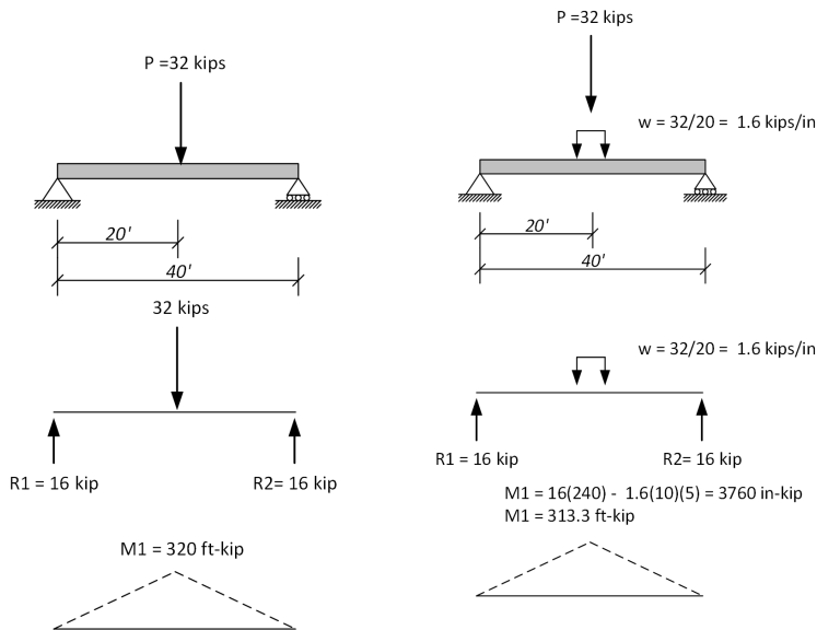
Figure 4.3 Statics check
