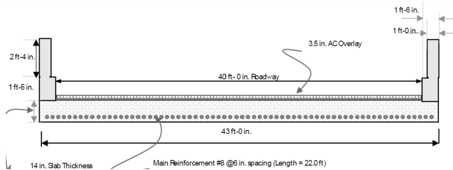
Figure 20. AASHTO MBE Example A7 Cross Section
