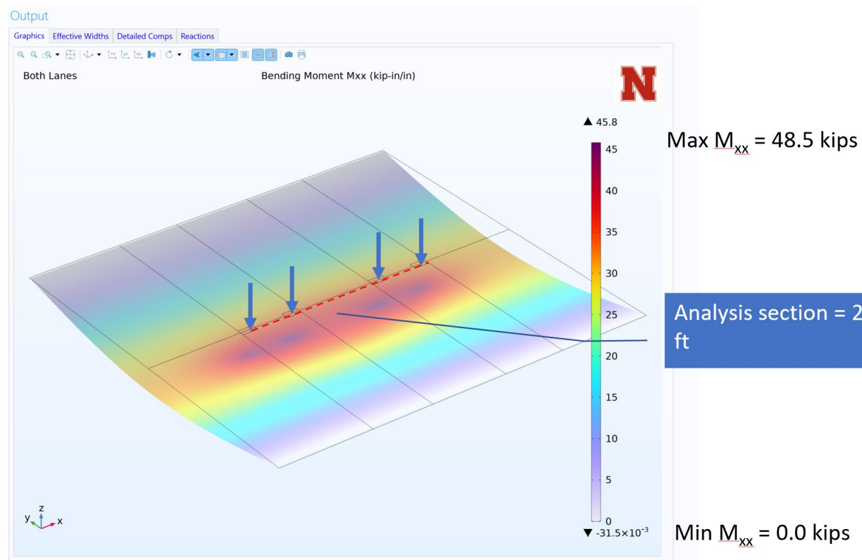
Figure 4.17 Load position and bending moments
