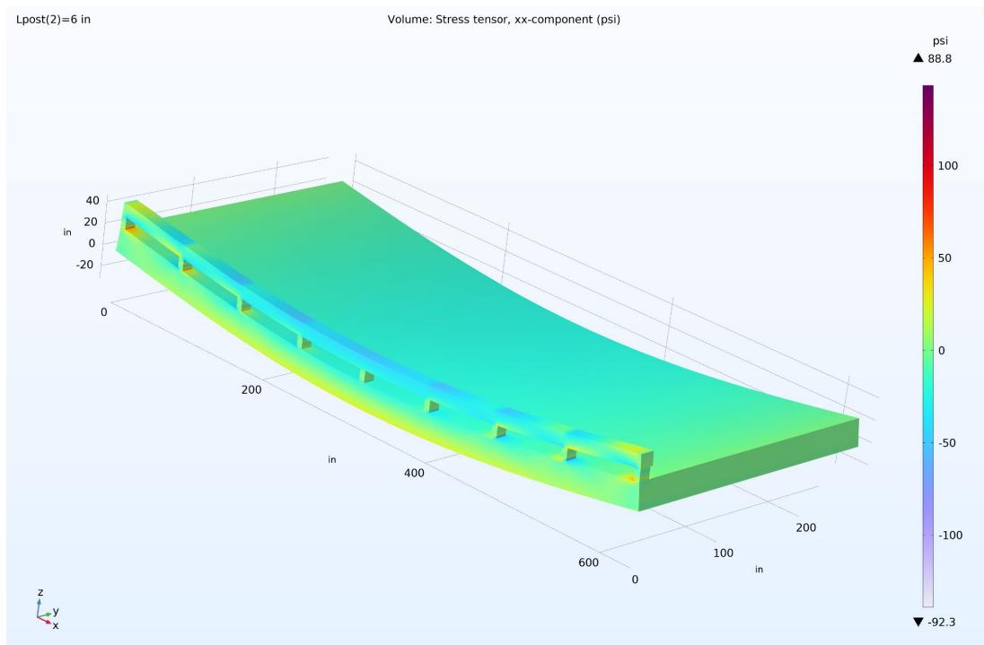
Figure 6.7 Local Post Stresses (6-in post)
