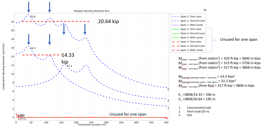
Figure 4.7 Bending moments plotted across the transverse section near the edge
