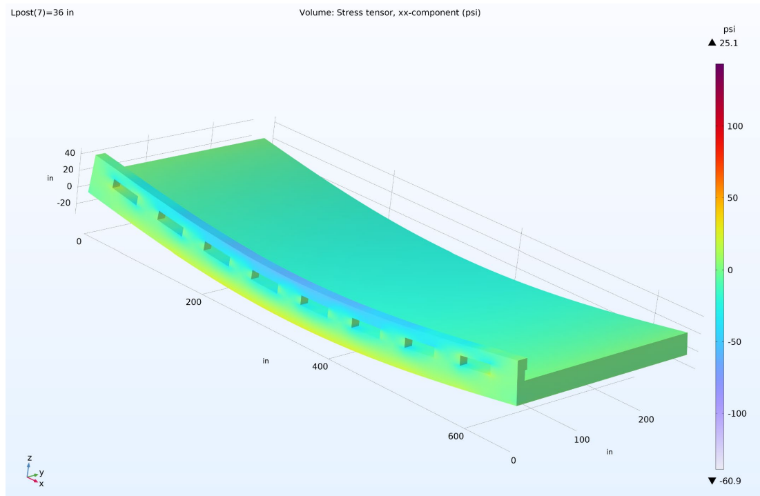
Figure 6.12 Normal Stress in the Longitudinal Direction (36-in post)
