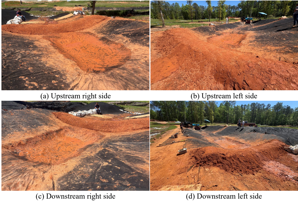
Figure 4.9: Temporary Earth Check
