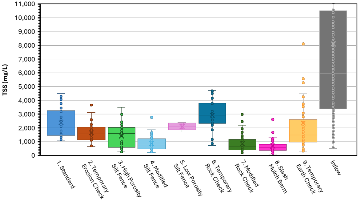
Figure 4.13: Downstream TSS per Installation
