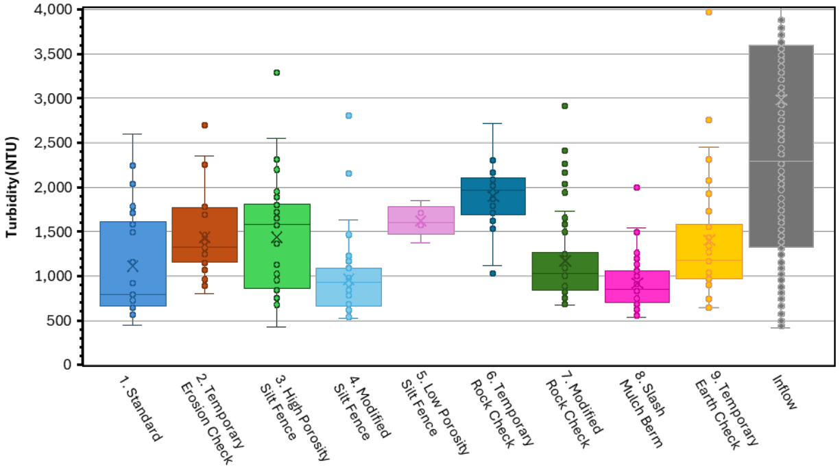
Figure 4.14: Downstream Turbidity per Installation
