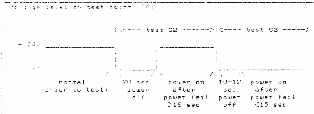
Fig. A3 Results of POWER UP RESET/RELAY DRIVER TEST
