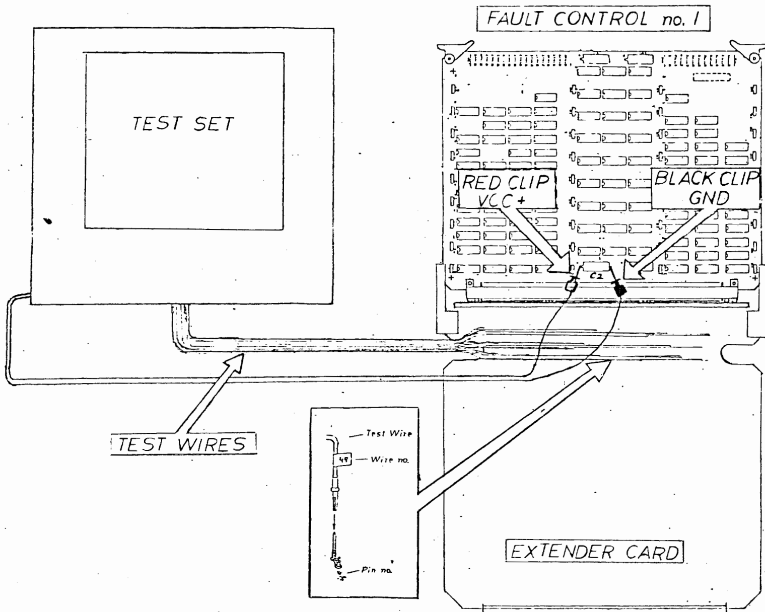
Figure A1 - Fault Control #1 Test Set Layout.
