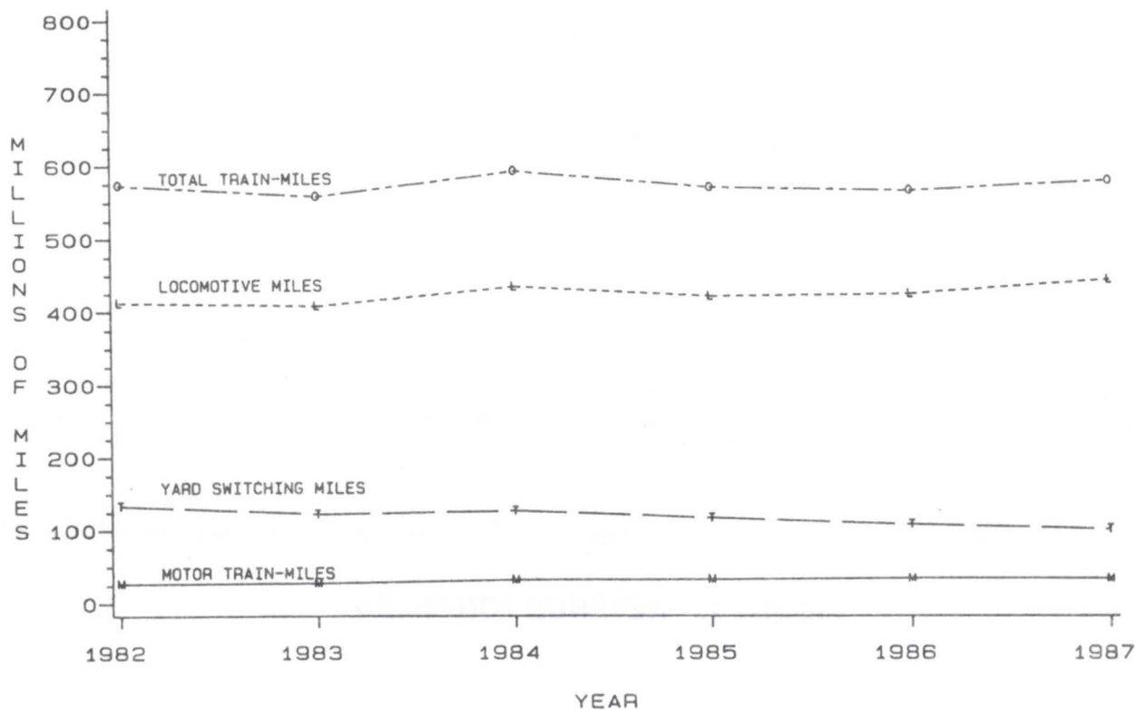
FIGURE 1. RAILROAD TRAIN-MILES
