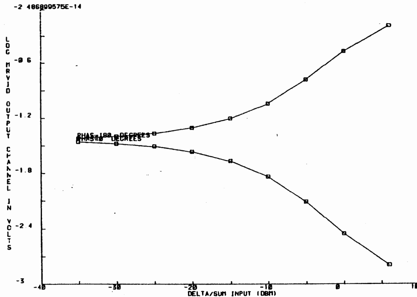
FIGURE 3B LOG MRVID OUTPUT CHANNEL VS INPUT D/S RATIO & PHASE
