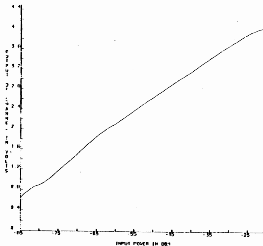
FIGURE 2. SUM LOG AMPLIFIER OUTPUT (3/26/62)
