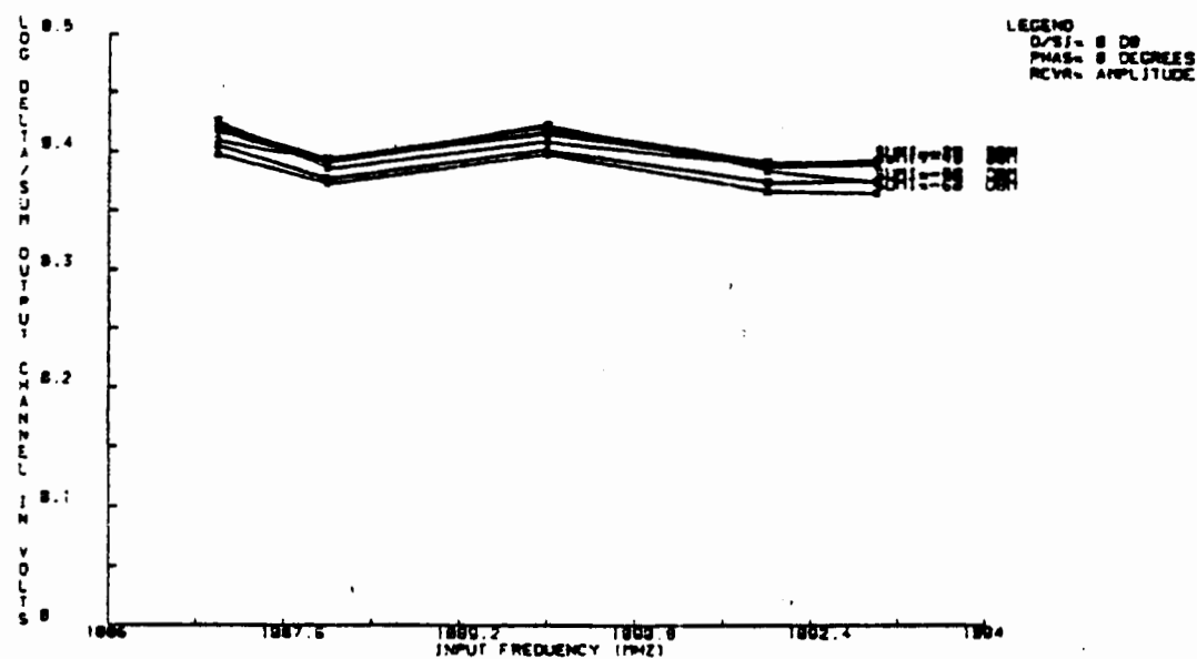
FIGURE 2 LOG DELTA/SUM OUTPUT CHANNEL VS INPUT FREQUENCY & SUM
