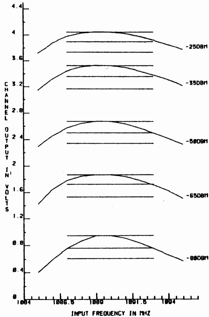
FIGURE 1.2 DELTA LOG AMPLIFIER BANDPASS AT DIFFERENT INPUT RF LEVELS
