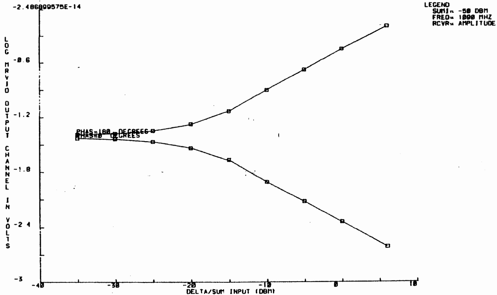
FIGURE 3A. LOG MRVID OUTPUT CHANNEL VS INPUT D/S RATIO & PHASE
