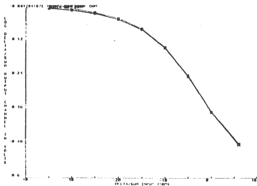
FIGURE B LOG DELTA/SUM OUTPUT CHANNEL VS INPUT D/S RATIO & SUM
