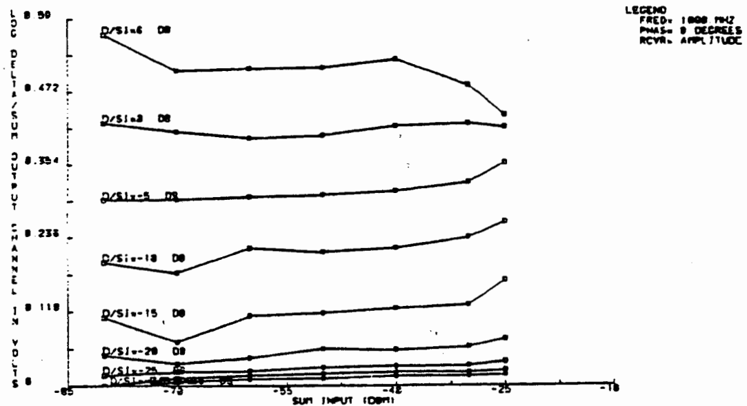
FIGURE B. LDC DELTA/SUM OUTPUT CHANNEL VS INPUT SUM & D/S RATIO
