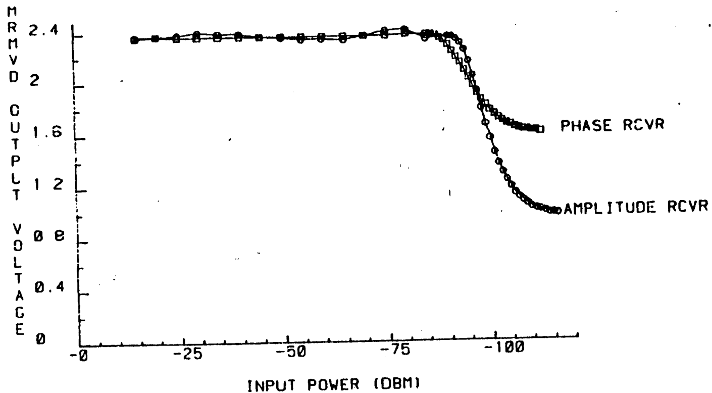
FIGURE 12. PHASE AND AMPLITUDE MONOPULSE VIDEO VS INPUT POWER
