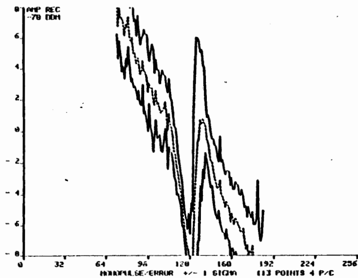
FIGURE 21. AMPLITUDE RECEIVER LOW POWER ERROR
