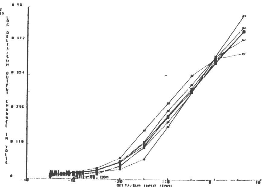
FIGURE C LOG DELTA/SUM OUTPUT CHANNEL VS INPUT D/S RATIO & SUM
