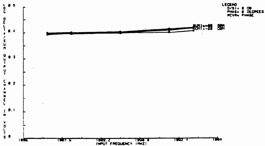
FIGURE 1 LOG DELTA/SUM OUTPUT CHANNEL VS INPUT FREQUENCY & SUM
