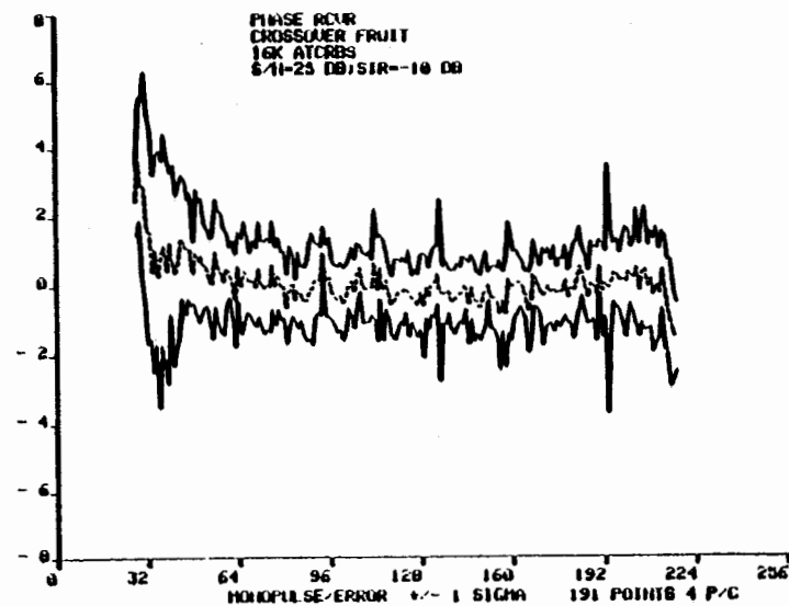
FIGURE. 26 INTERFERENCE EFFECTS
