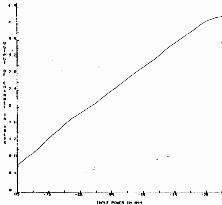
FIGURE 1. DELTA LOG AMPLIFIER OUTPUT (3/23/62)
