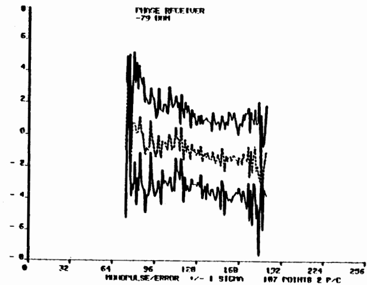
FIGURE 20. PHASE RECEIVER LOW POWER ERROR
