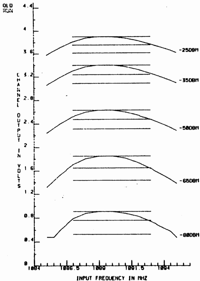
FIGURE 1.1 SUM LOG AMPLIFIER BANDPASS AT DIFFERENT INPUT RF LEVELS
