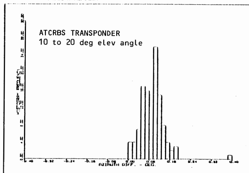
AMPLITUDE RECEIVER FLIGHT TEST AZIMUTH RESIDUAL HISTOGRAMS FIGURE 24
