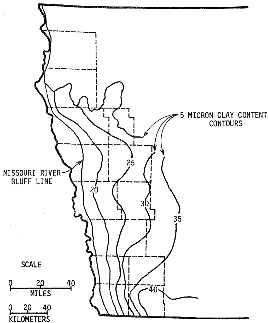
Fig. 4. Geographic distribution of 5 micron clay (in percent) contours in loess of western Iowa. After Dahl et al. (1958).
