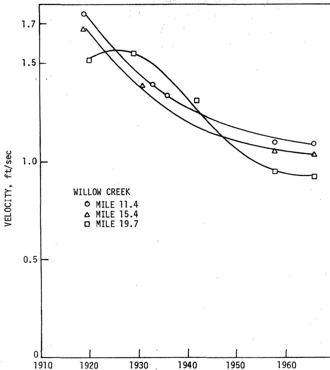
Fig. 18. Velocity variation with time for 3 sections of the Willow Creek.
