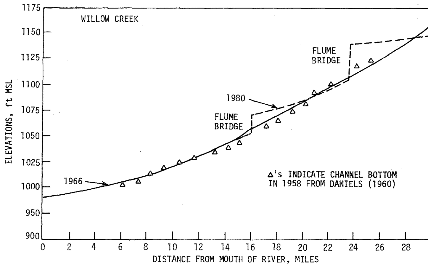
Fig. 11. Longitudinal profiles of Willow Creek 1958, 1966, and 1980.
