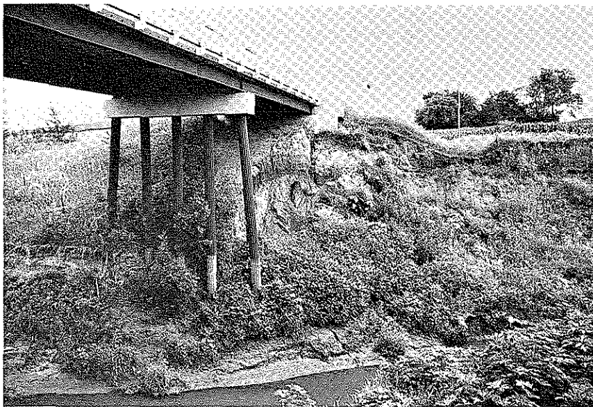
Plate 3. Channel degradation has exposed portions of these piles. Former ground level is indicated by the top of the light-colored portion at bottom of piles. Note also the soil pulling away from the abutment.
