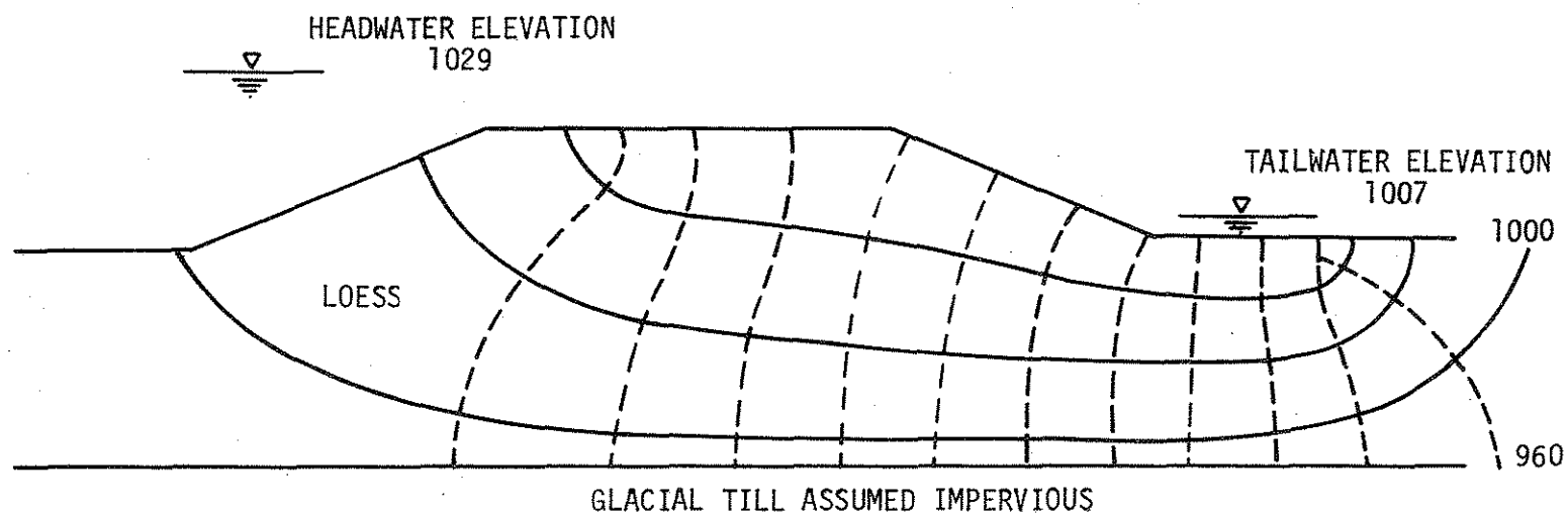
Fig. 22. Flow net beneath structure for Flume No. 2.
