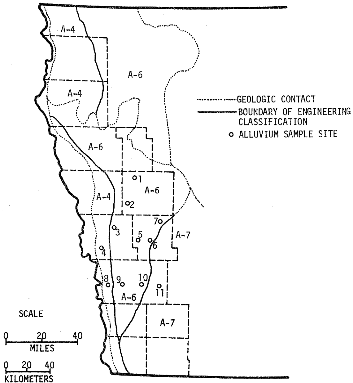
Fig. 5. Engineering classification of loess in western Iowa. After Hansen et al. (1959) and location of alluvium sample sites.
