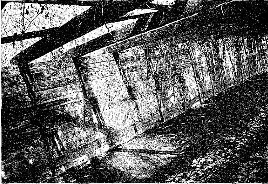
Plate 13. Flume of the original flume bridge in Fremont County. Note wood sidewalls and floor, cross braces on top, and absence of piles in the interior of the flume.
