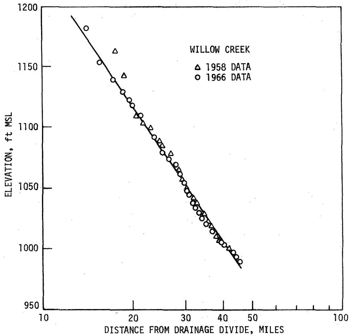
Fig. 19. Longitudinal profile of Willow Creek on semilog plot.
