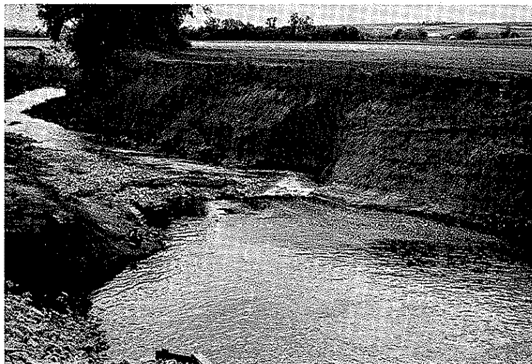
Plate 17. Scour hole at stilling basin downstream from flume bridge. Note how deflection of channel is causing lateral erosion.
