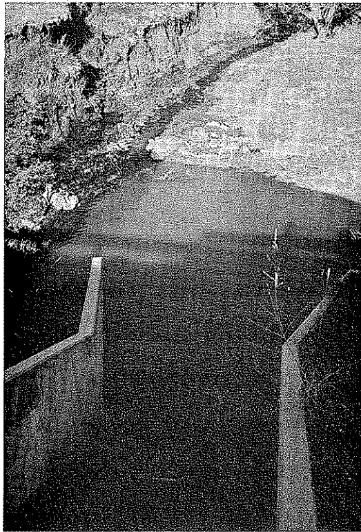
Plate 18. Undissipated energy on the downstream side of this box culvert having an IDOT flume outlet resulted in erosion of a scour hole and bank instability.
