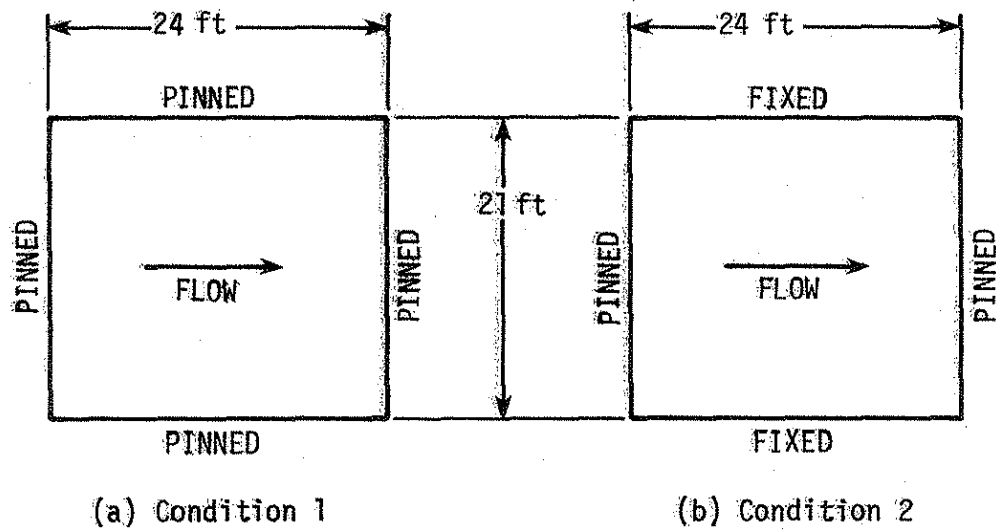
Fig. 26. Plan view of stilling basin with assumed edge conditions-- Flume No. 2.
