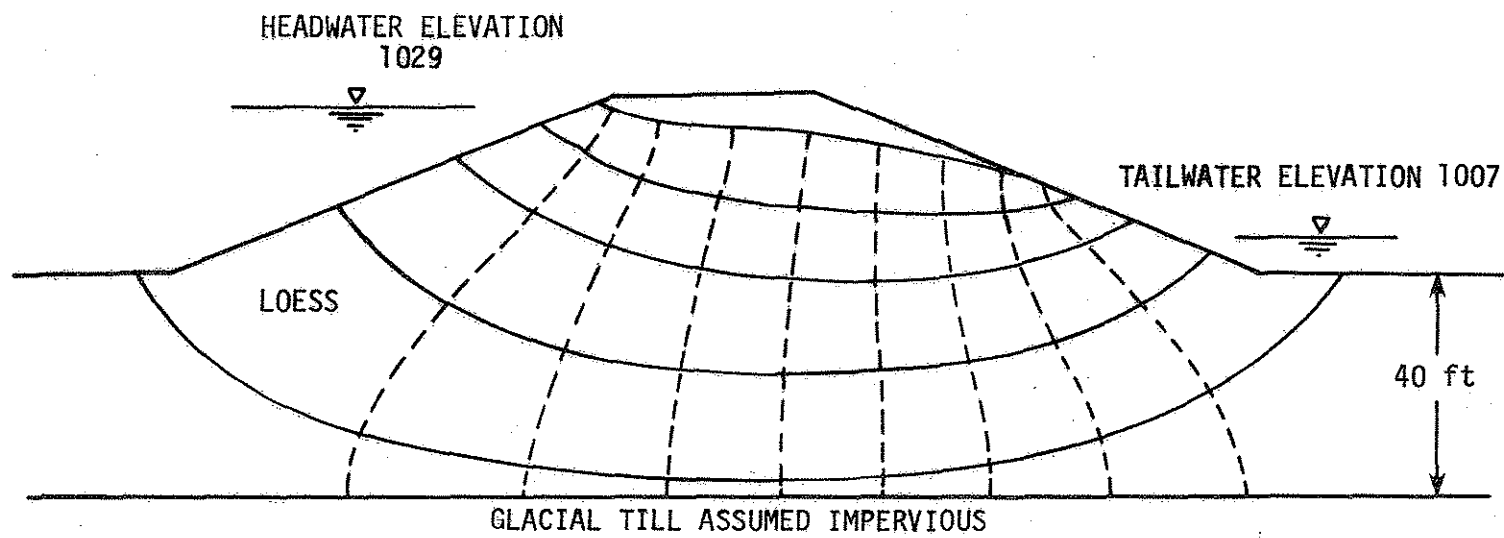
Fig. 24. Flow net through embankment adjacent to structure for Flume No. 2.
