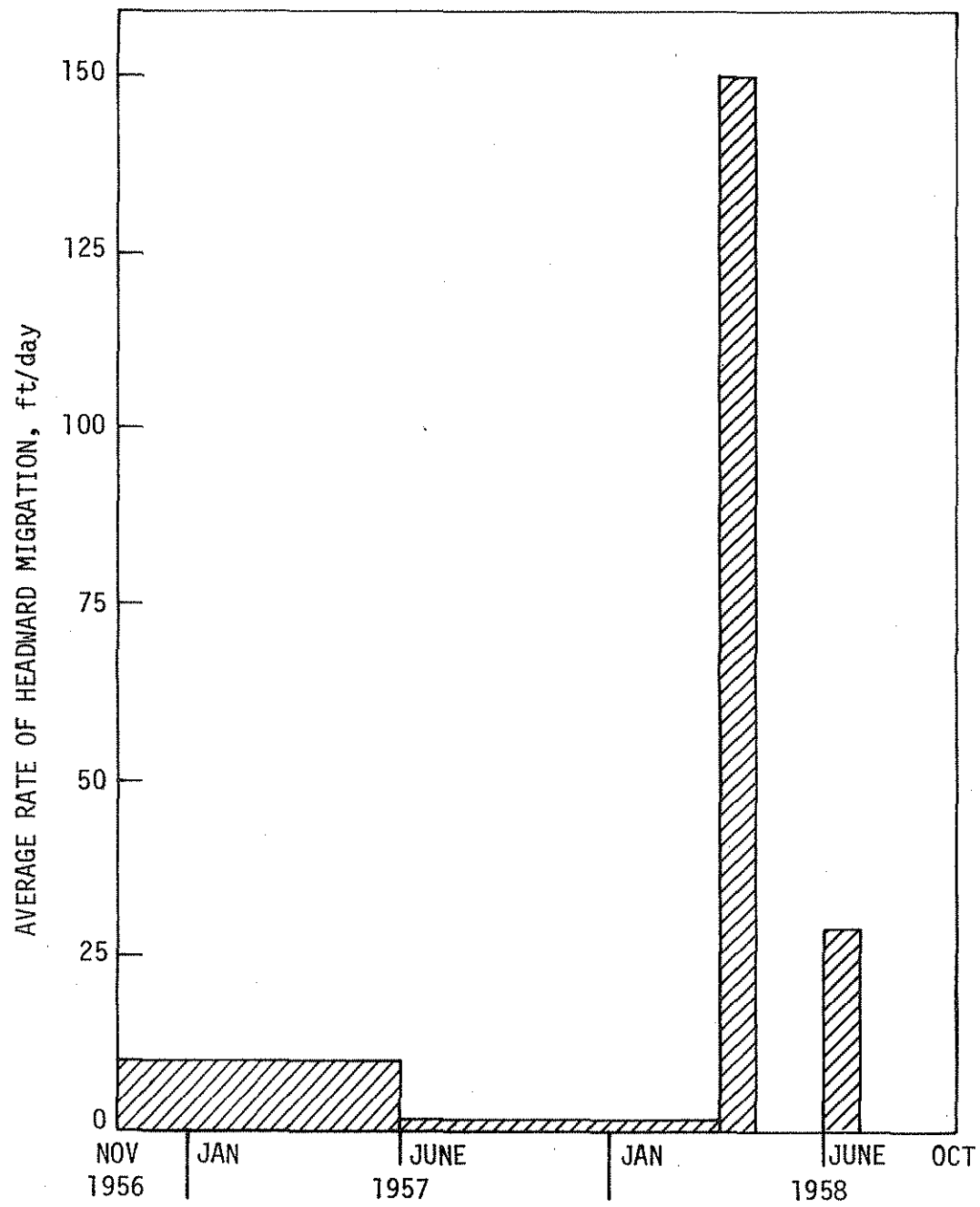
Fig. 13. Average Rate of knickpoint migration on Willow Creek. Plotted from data reported by Daniels (1960).
