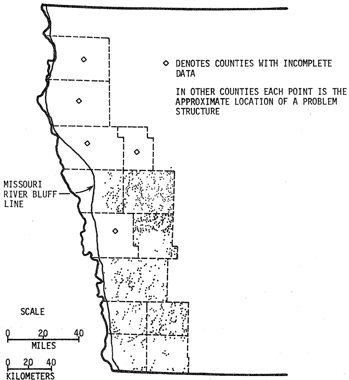
Fig. 16. Location of problem structures as determined by data from Iowa DOT bridge inventory.
