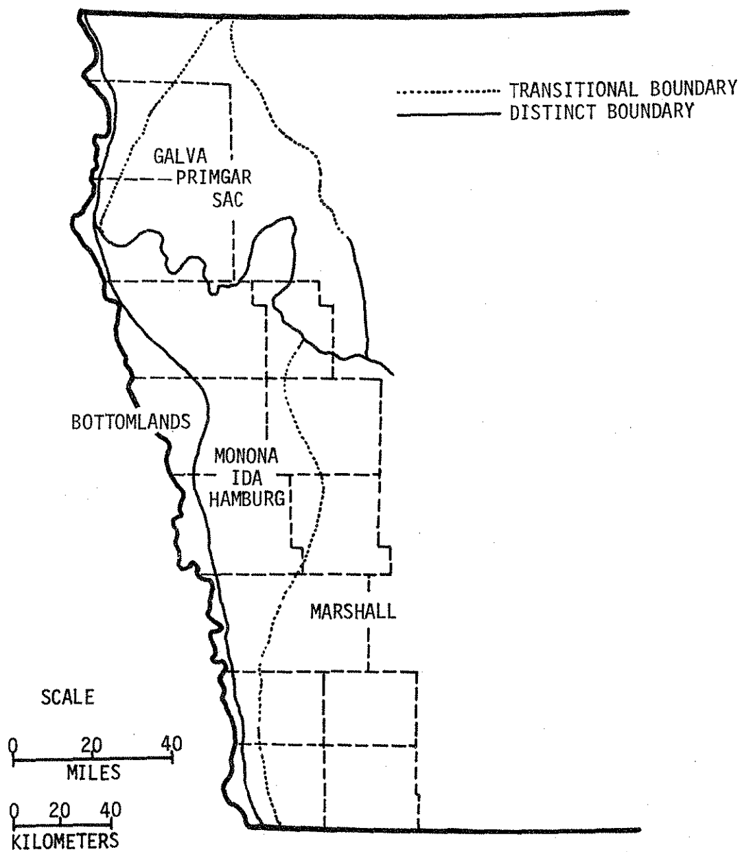
Fig. 6. Principal soil associations in western Iowa. After Simonson et al. (1952).
