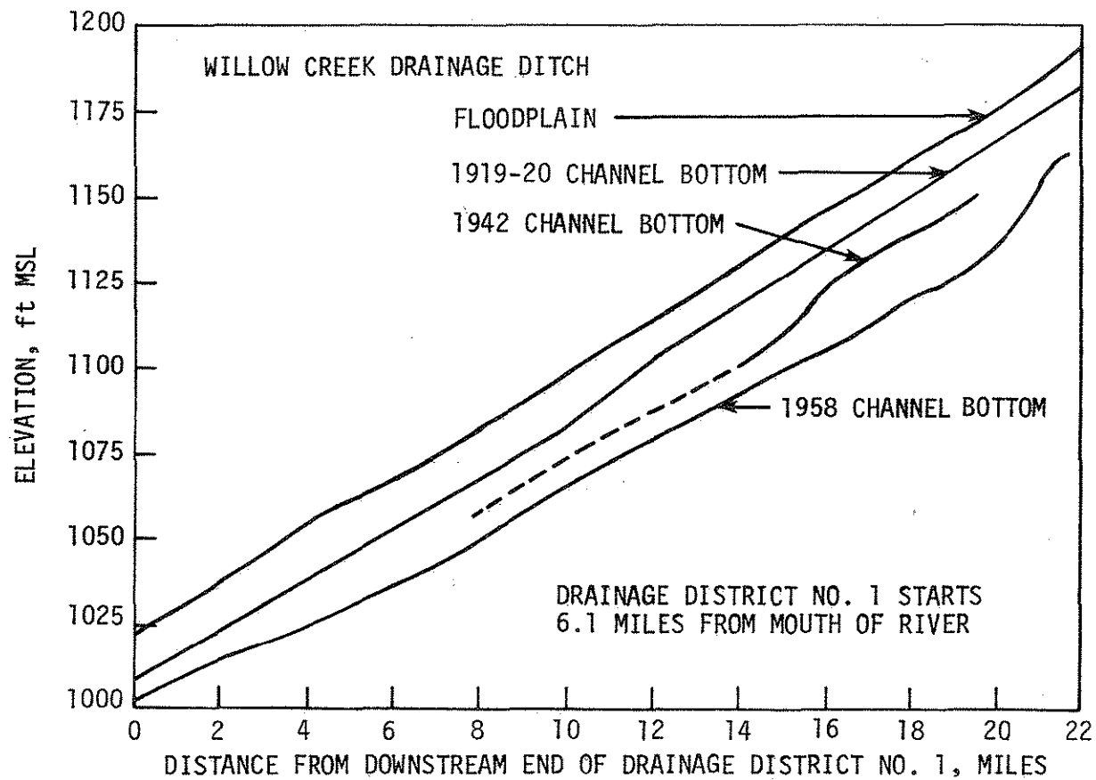
Fig. 10. Longitudinal profile of Willow drainage ditch in Drainage Districts 1 and 2. After Daniels (1960).
