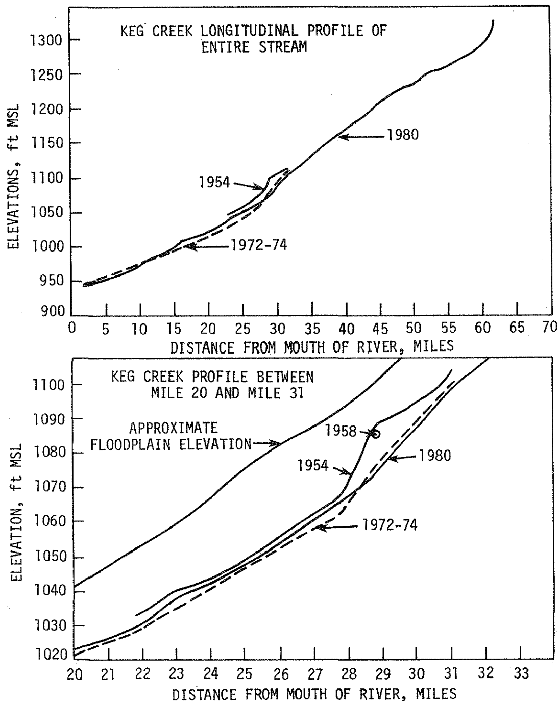
Fig. 12. Longitudinal profile of Keg Creek.
