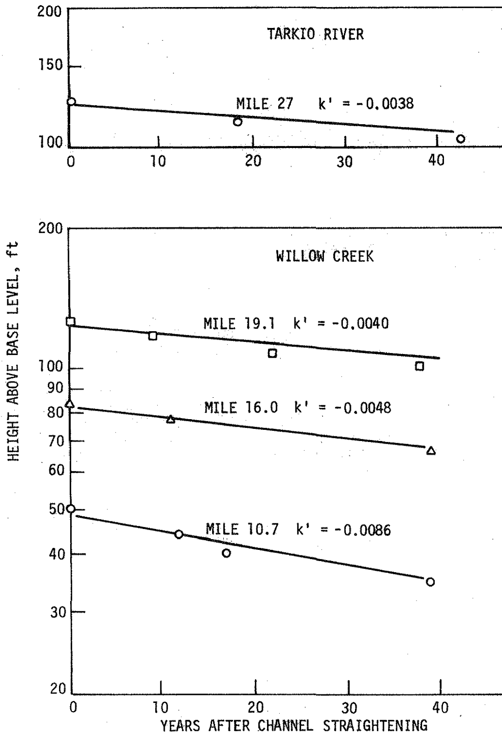
Fig. 20. Time versus log height above base level for reaches of Willow and Tarkio Rivers.
