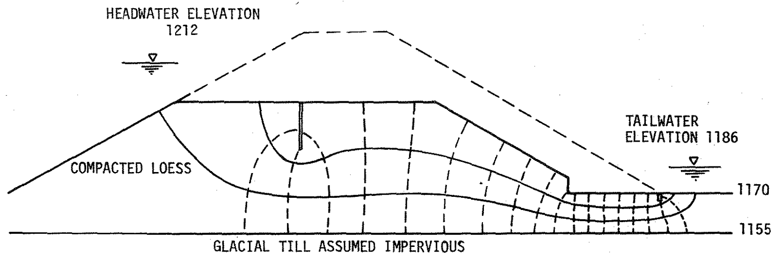
Fig. 23. Flow net beneath structure for Flume No. 3.
