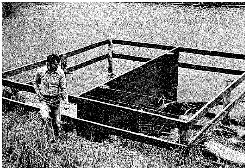
Plate 10. An SCS-type drop inlet for a grade stabilization structure. Note baffle plate to disrupt vortices and trash rack.
