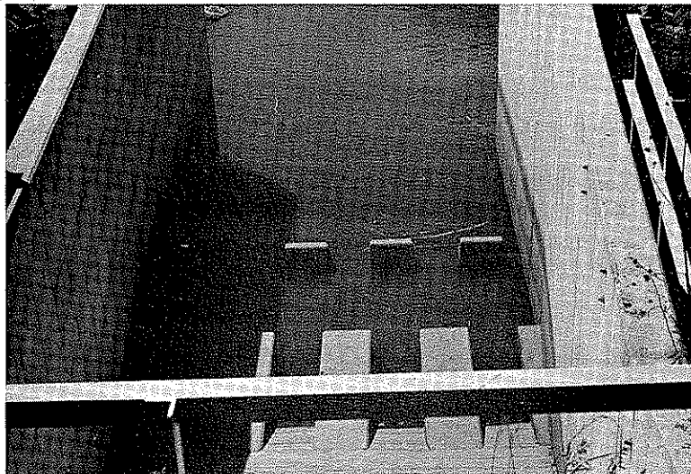
Plate 19. Chutes and baffle blocks for energy dissipation on downstream side of box-culvert type of grade stabilization structure.
