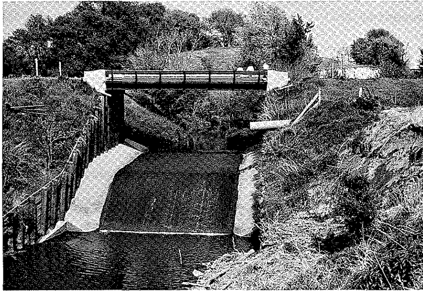
Plate 7. Flume bridge in Fremont County. Note wood piles inside the flume.
