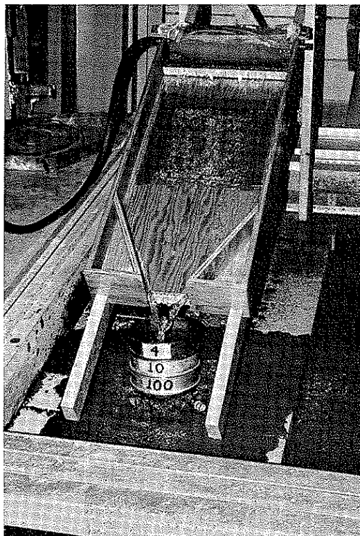
Plate 12. Erosion flume used in cement stabilization study.
