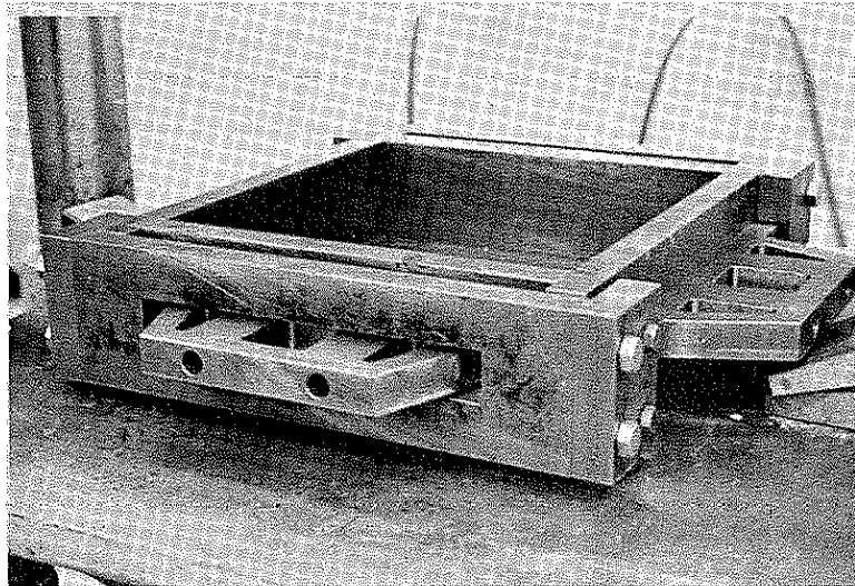
Plate 11. Mold used for preparing soil-cement specimens for erosion tests.
