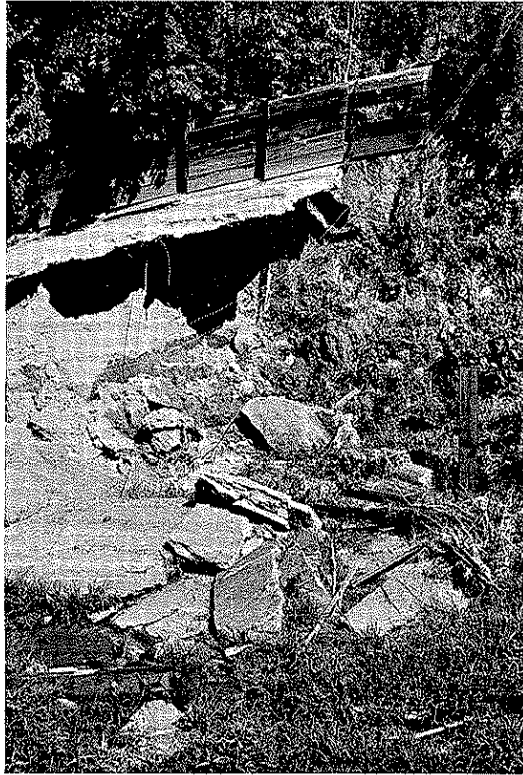
Plate 16. The remainder of the concrete floor and timber sidewalls of a flume which has failed, probably through piping.
