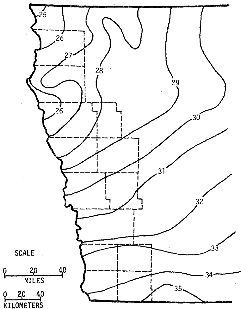
Fig. 8. Normal amounts of annual precipitation in inches. From U.S. Geological Survey (1978).
