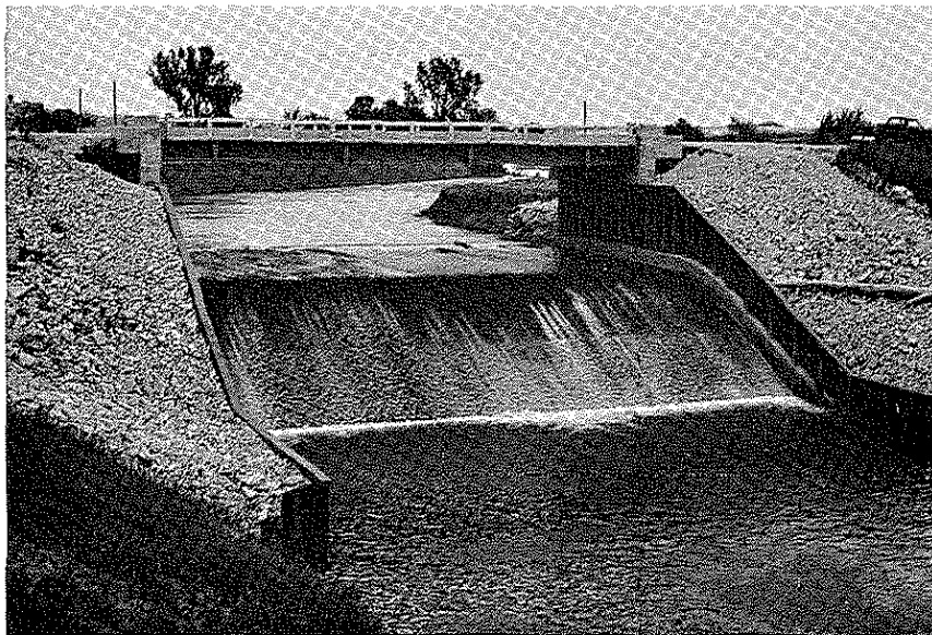
Plate 14. Recently built flume bridge in Harrison County. Note the use of steel piles in the sidewalls and bridge alignment relative to stream channel.
