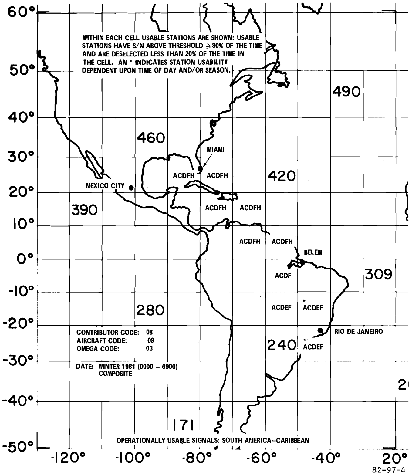
FIGURE 4. OPERATIONALLY USABLE SIGNALS: SOUTH AMERICA-CARIBBEAN, WINTER 1980-1981
