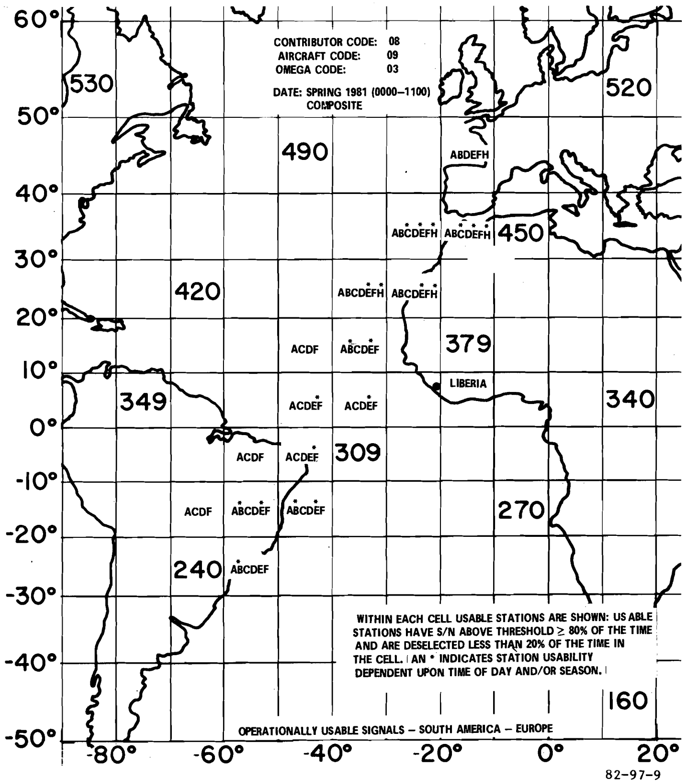
FIGURE 9. OPERATIONALLY USABLE SIGNALS: SOUTH AMERICA-EUROPE, SPRING 1981 (000-0100 GMT)
