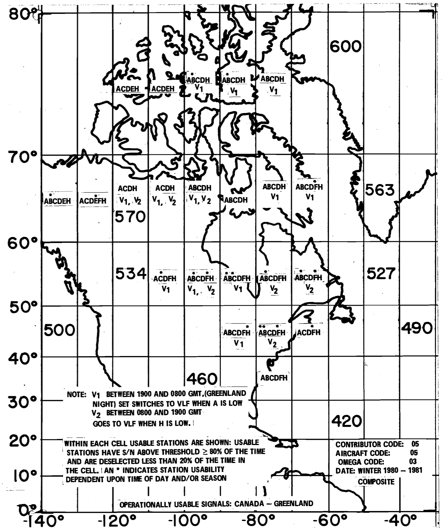
FIGURE 12. OPERATIONALLY USABLE SIGNALS: CANADA-GREENLAND, WINTER 1981
