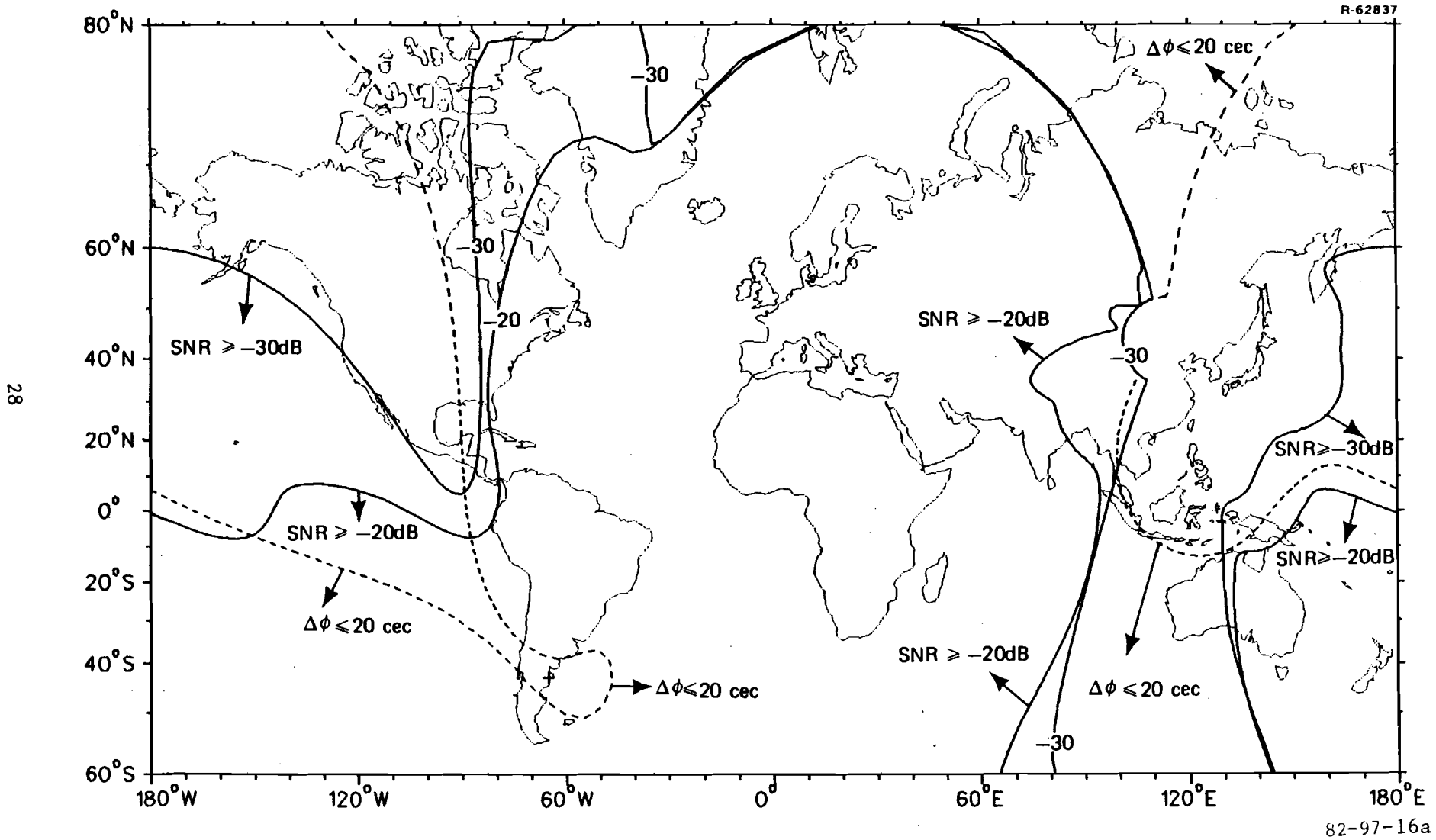
FIGURE 16. OMEGA SIGNAL COVERAGE PREDICTION DIAGRAM ARGENTINA (F) (MAY 0600 - 1800 GMT) (SHEET 1 OF 2)
