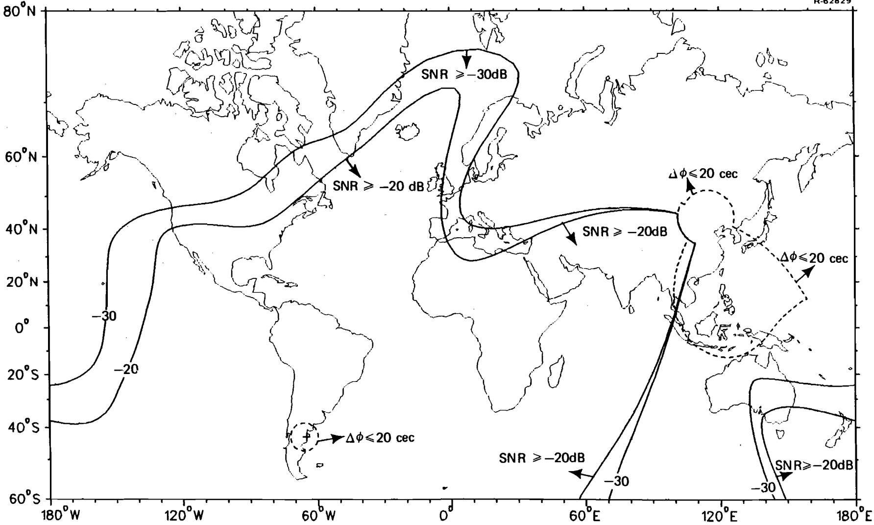
FIGURE 16. OMEGA SIGNAL COVERAGE PREDICTION DIAGRAM ARGENTINA (F) (MAY 0600 - 1800 GMT) (SHEET 2 OF 2)
