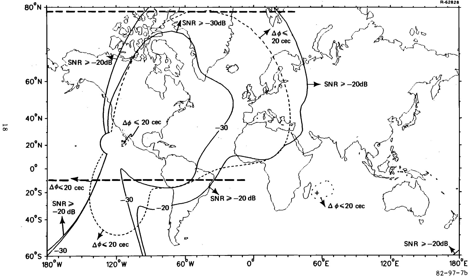
FIGURE 7. OMEGA SIGNAL COVERAGE PREDICTION DIAGRAM LA REUNION (E) (SHEET 2 OF 3)
