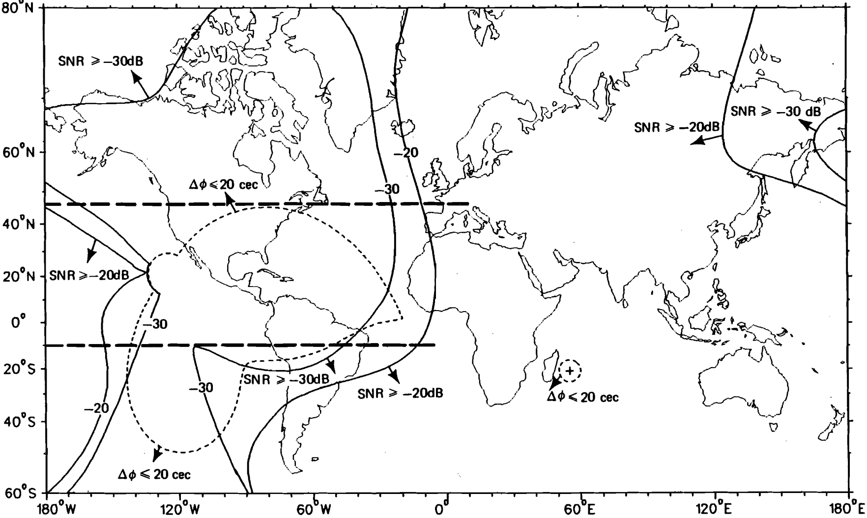
FIGURE 7. OMEGA SIGNAL COVERAGE PREDICTION DIAGRAM LA REUNION (E) (SHEET 1 OF 3)
