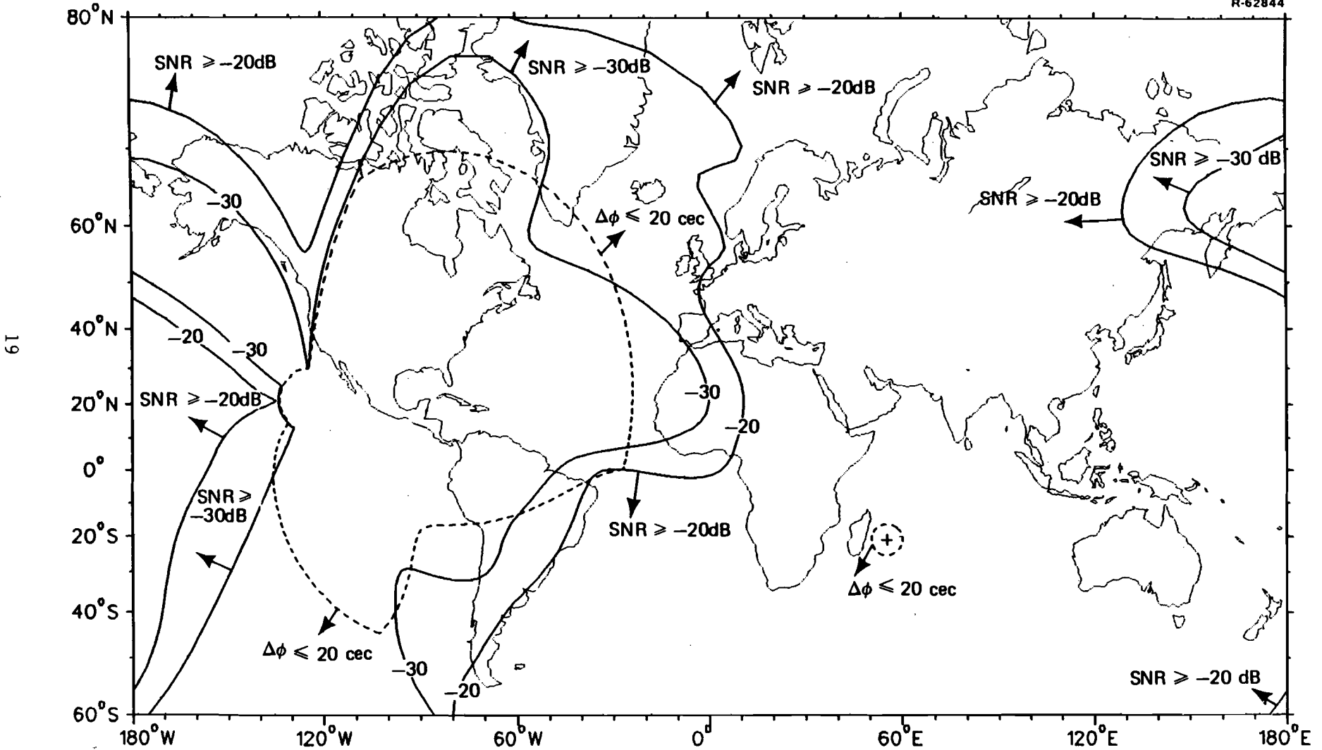
FIGURE 7. OMEGA SIGNAL COVERAGE PREDICTION DIAGRAM LA REUNION (E) (SHEET 3 OF 3)
