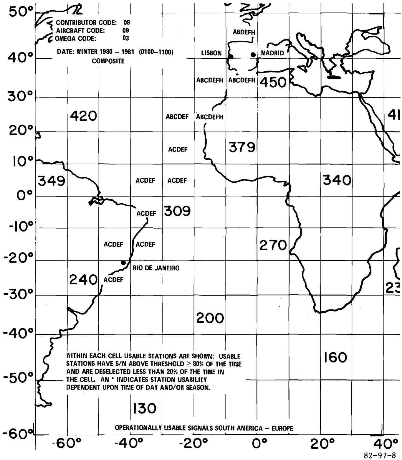
FIGURE 8. OPERATIONALLY USABLE SIGNALS: SOUTH AMERICA-EUROPE, WINTER 1980-1981 (0100-1100 GMT)
