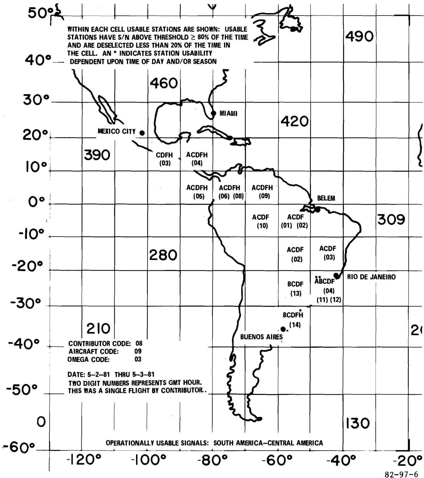
FIGURE 6. OPERATIONALLY USABLE SIGNALS: SOUTH AMERICA-CENTRAL AMERICA, SPRING 1981
