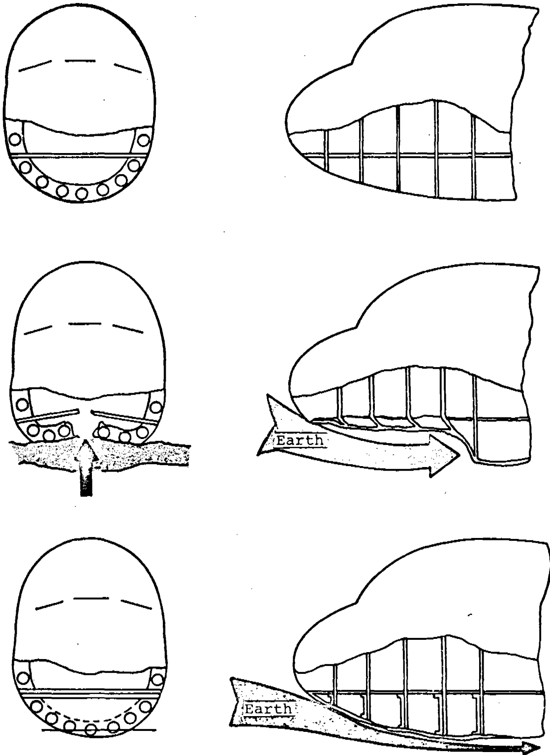
FIGURE E-2: METHOD OF REINFORCING NOSE STRUCTURE TO PROVIDE INCREASED RESISTANCE TO VERTICAL LOADS AND TO REDUCE EARTH SCOOPING (REFERENCE 3, PAGE 125)
