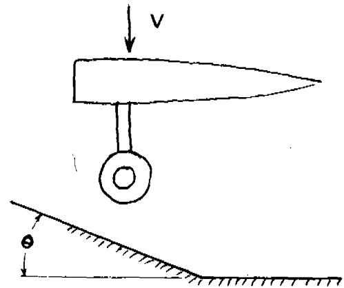
FIGURE D-1 : LANDING GEAR / WING DROP TEST
