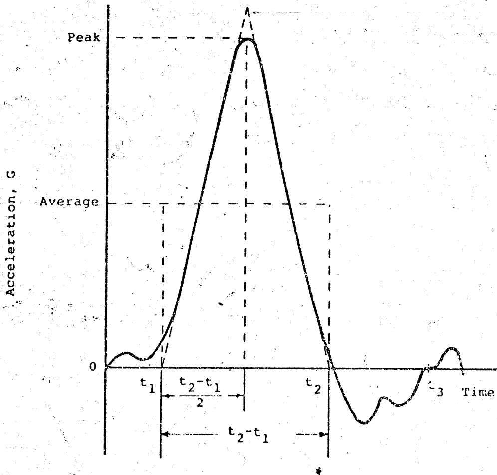
Figure D-3.1 - Typical Aircraft Floor Acceleration Pulse (From Army CSDG)
