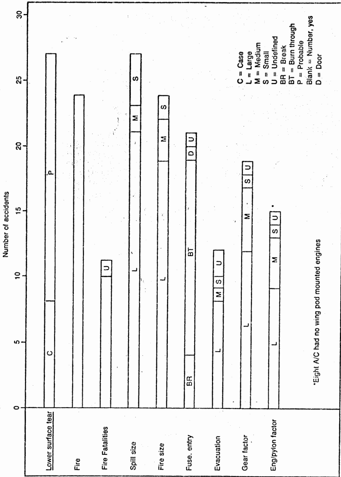
Figure 4.4-Lower Surface Tear
