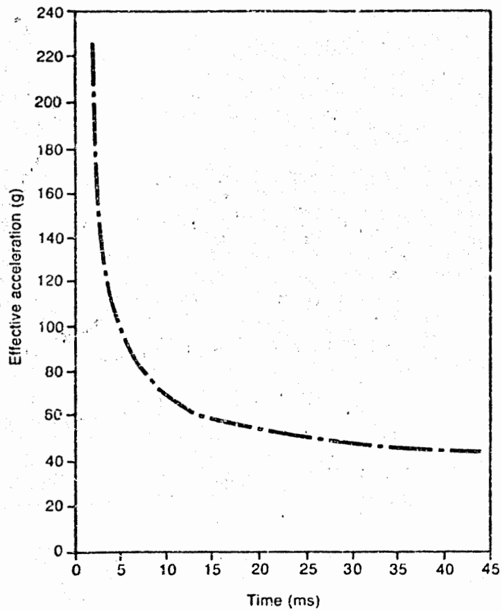
Figure 5.6-Wayne State University Cerebral Concussion Tolerance Curve
