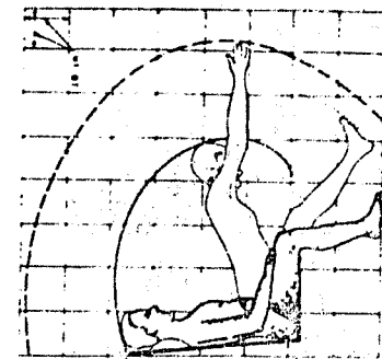
Most exact line for cockpit arrest lines line for loop constraint Lap belt-only extremity strike envelope - side view.
