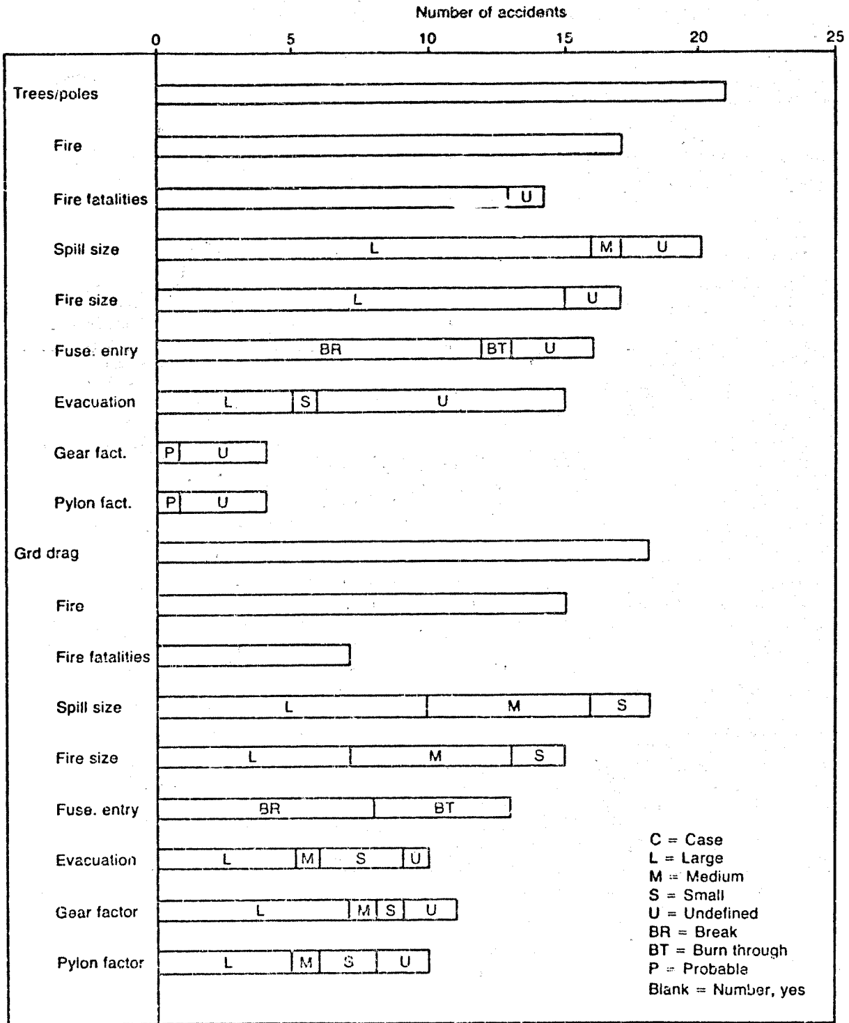
Figure 4.3-Wing Break Assessment
