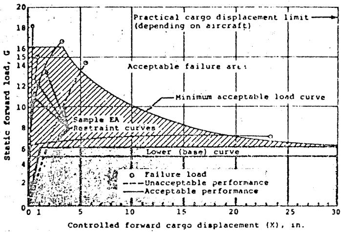
Load-displacement requirements for energy-absorbing cargo restraint systems (forward loading of rotary-wing and fixed-wing aircraft).
