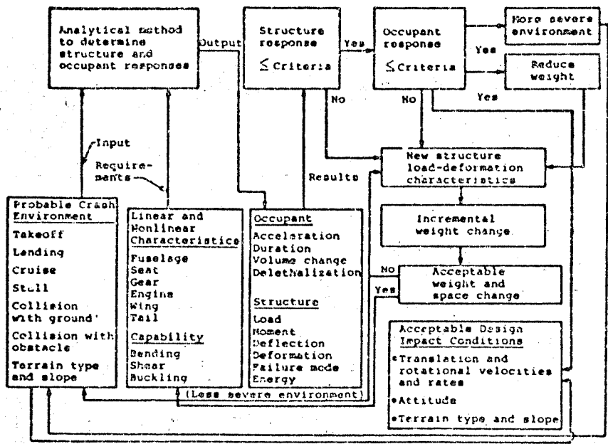
Procedure for evaluation of structural designs with respect to crashworthiness.
