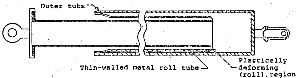
(b) Inversion tube - absorbs energy by inverting a thin-walled tube
