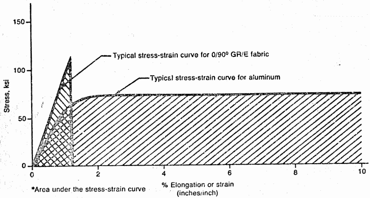
Figure 4.18—Comparison of Apparent Energy Absorbing Characteristics* of Graphite Epoxy Laminate and Aluminum
