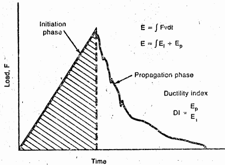
Figure 4.21. - Schematic Representation of Load History in an Impact Test
