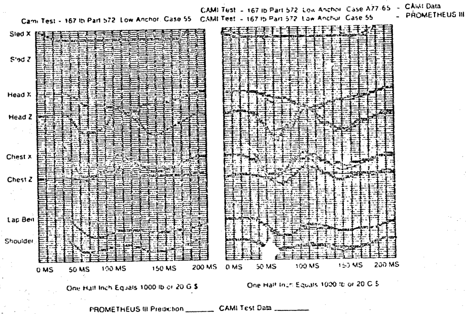
Figure 5.1-PROMETHEUS III Simulations
