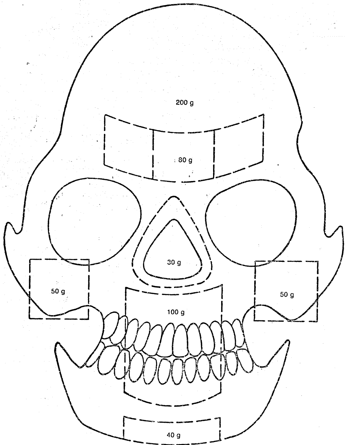
Figure 5.7 - Summary of Maximum Impact Forces on a Padded Deformable Surface
