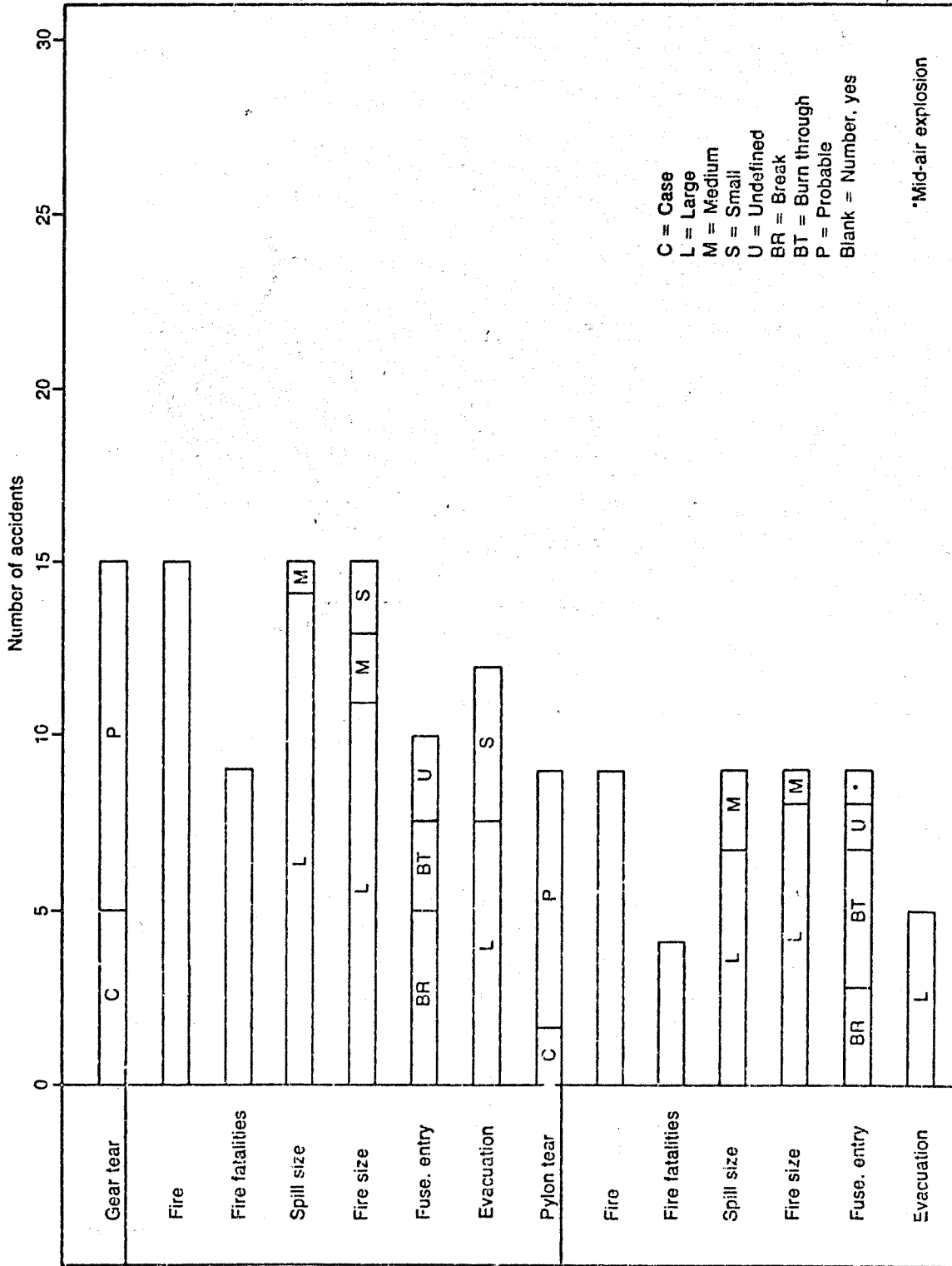
Figure 4.5-Gear/Pylon Wing Box Tear
