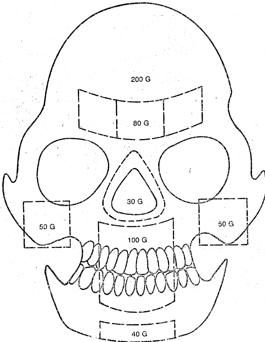
Figure D-5.9 - Summary of Maximum Tolerable Impact Forces on a Padded Deformable Surface (Swearingen, 1965)
