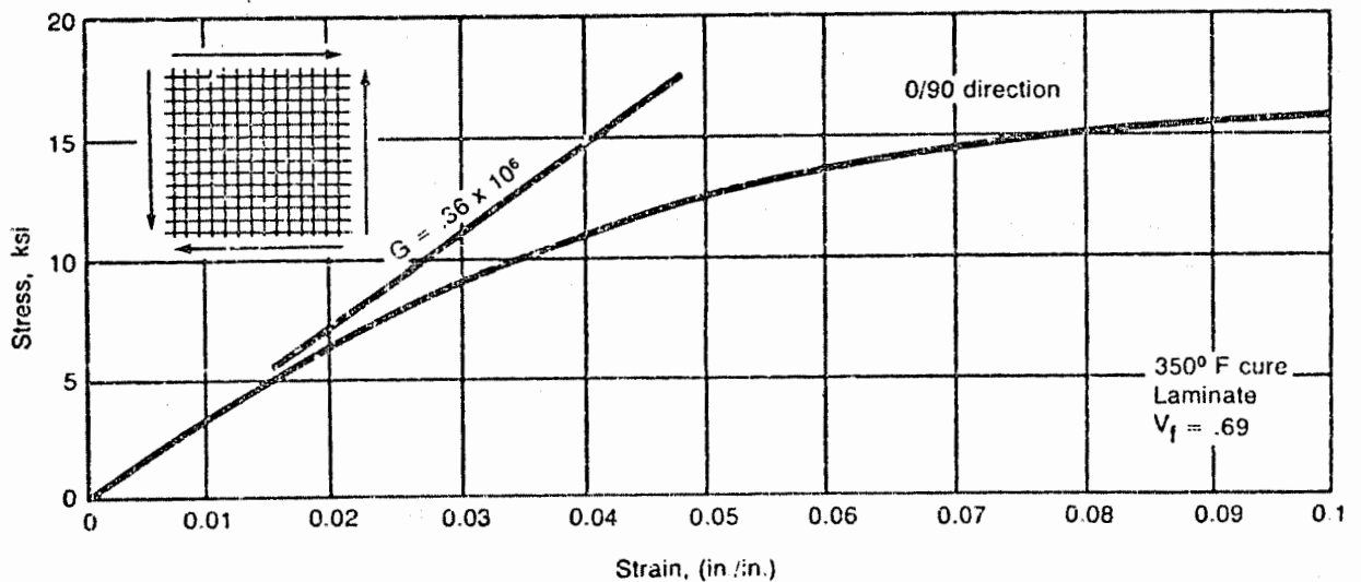
Figure 4.19—Shear Stress-Strain for Kevlar-49/5208 Style 181 Fabric at R.T., Dry
