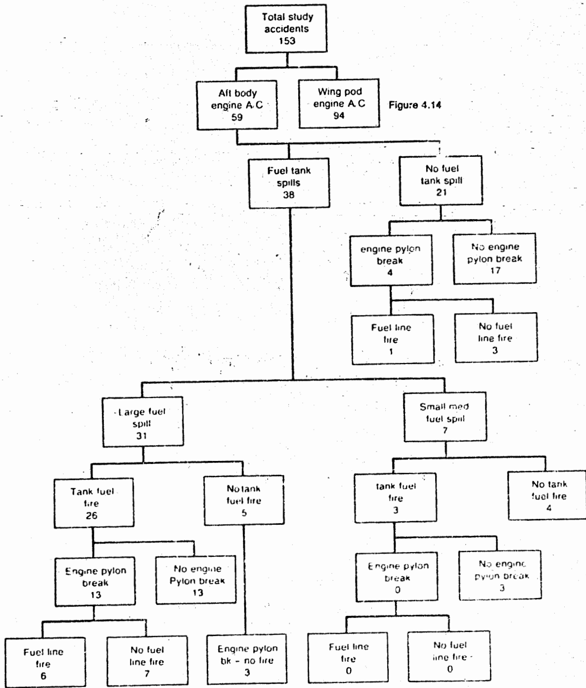
Figure 4.15-Engine/Pylon Separation/Collapse and Fuel Tank Rupture, Aft Body Engined Aircraft
