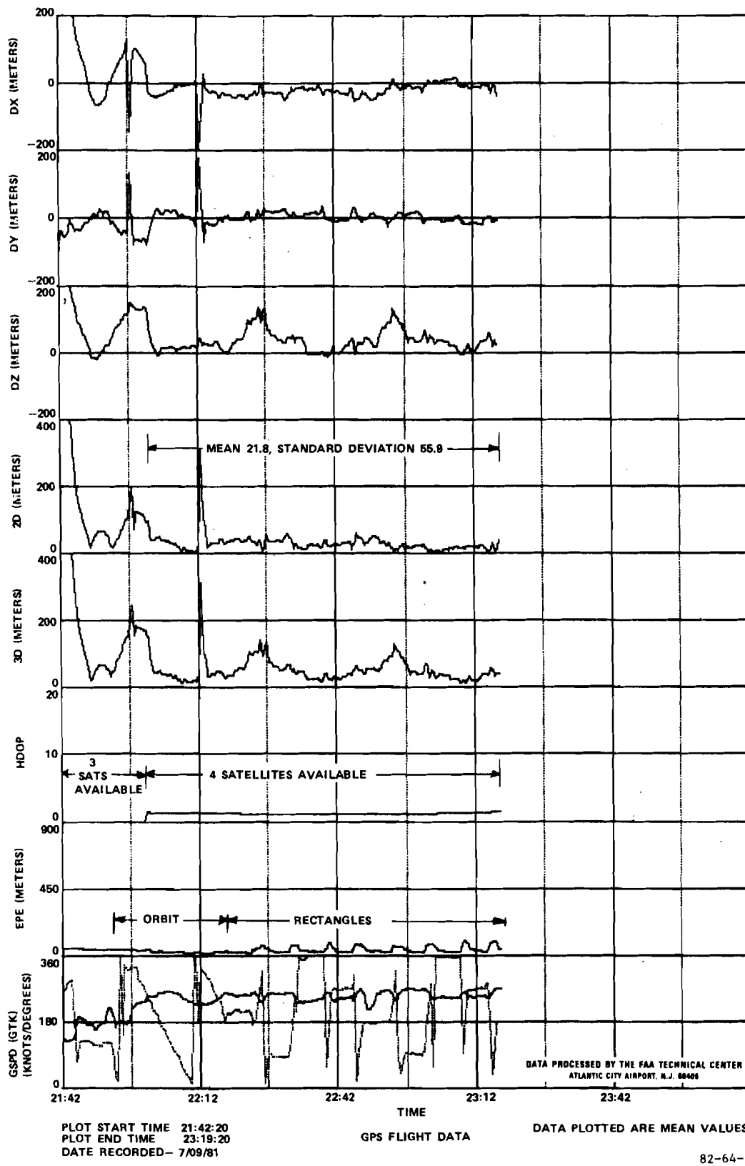
FIGURE 24. DELTA MEAN PLOT FOR JULY 9, 1981
