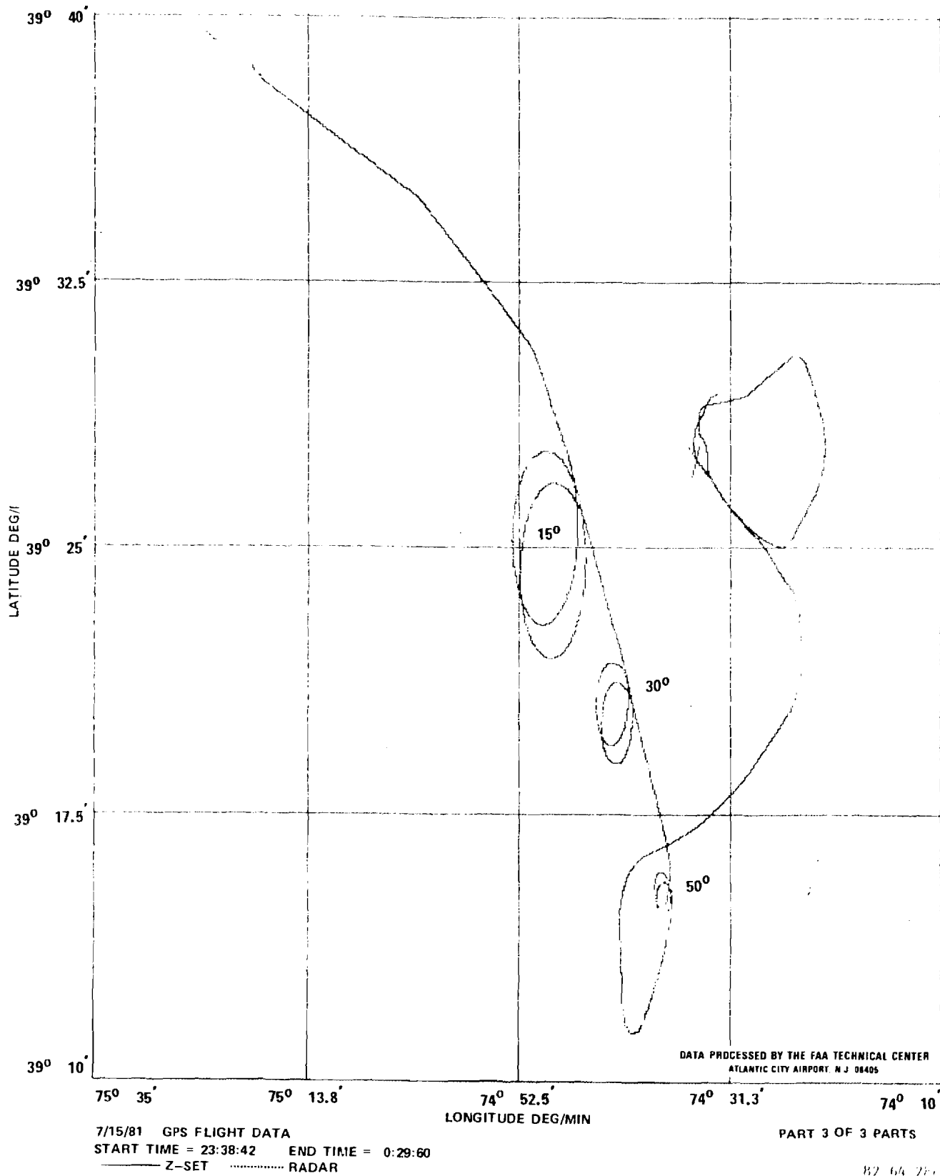
FIGURE 28. GPS AND RADAR DETERMINED FLIGHTPATH OF CONSTANT BANK TURNS (SHEET 3 OF 3)
