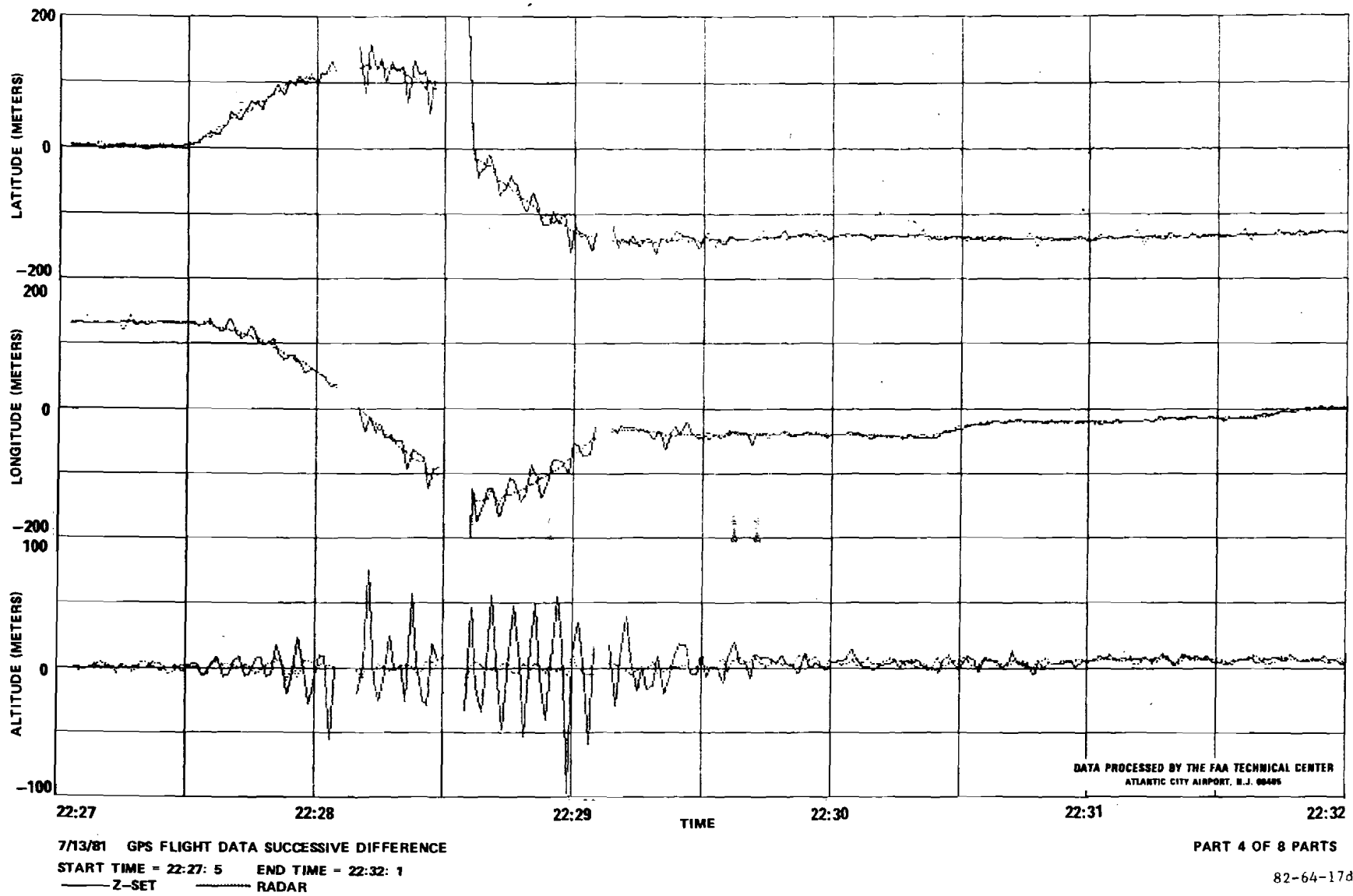
FIGURE 17. SUCCESSIVE DIFFERENCE PLOTS FOR JULY 13, 1981 (SHEET 4 OF 8)
