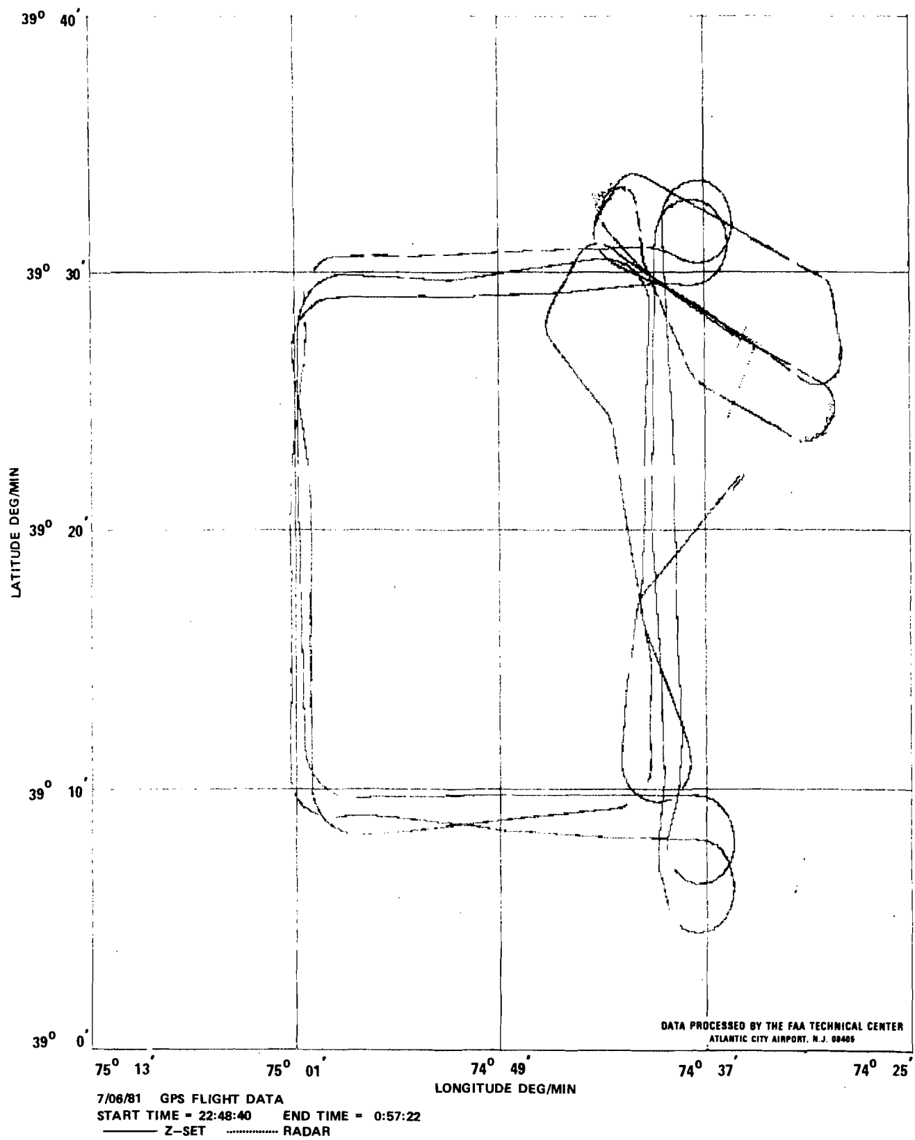
FIGURE 18. GPS AND RADAR FLIGHT RECTANGULAR PATH FOR JULY 6, 1981
