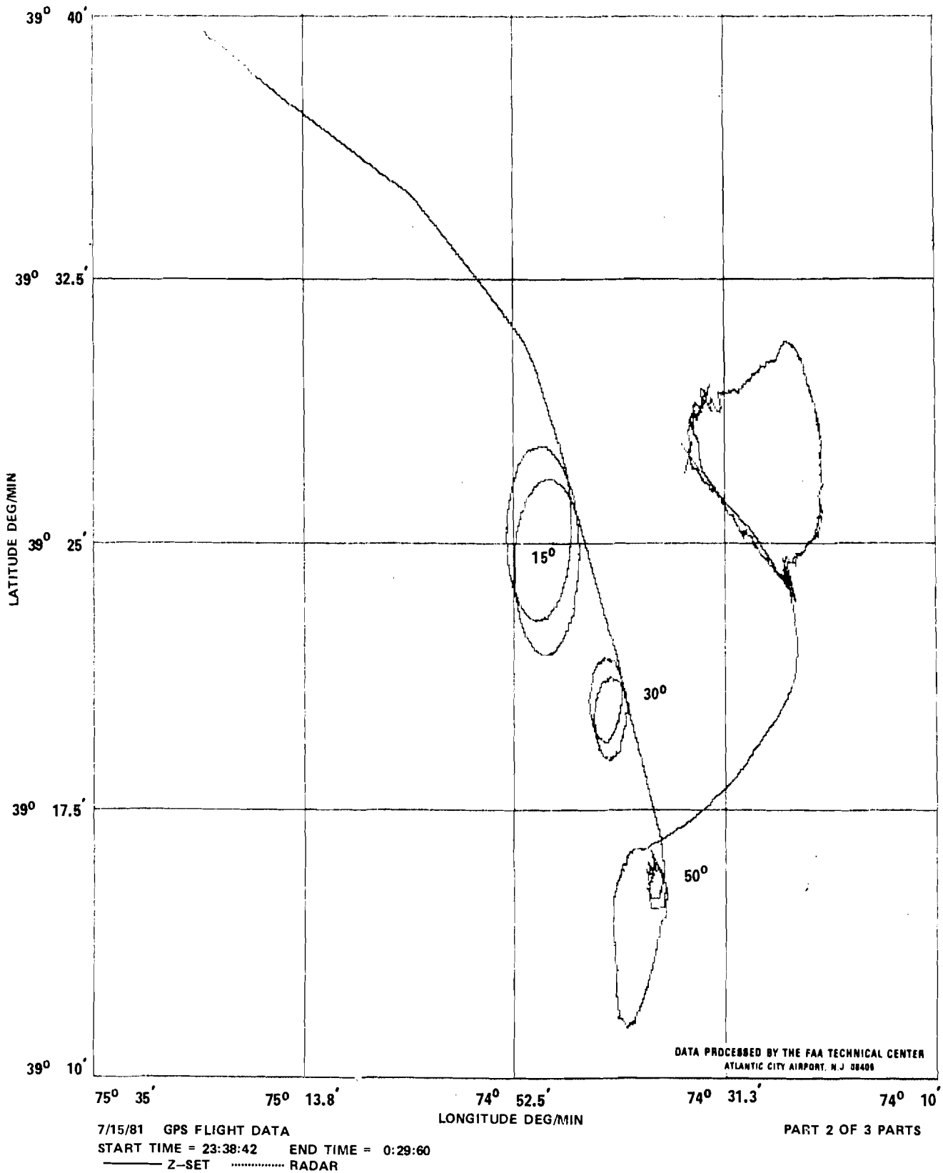
FIGURE 28. GPS AND RADAR DETERMINED FLIGHTPATH OF CONSTANT BANK TURNS (SHEET 2 OF 3)
