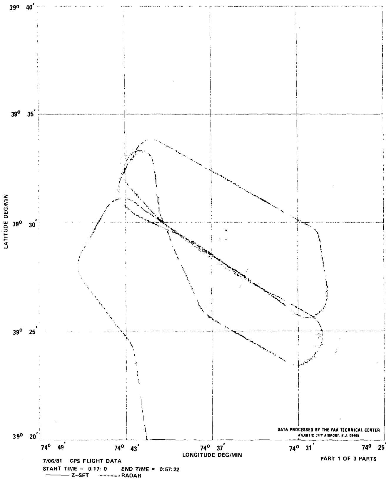
FIGURE 27. GPS AND RADAR DERIVED NONPRECISION FLIGHTPATH ON JULY 6, 1981 (SHEET 1 OF 3)
