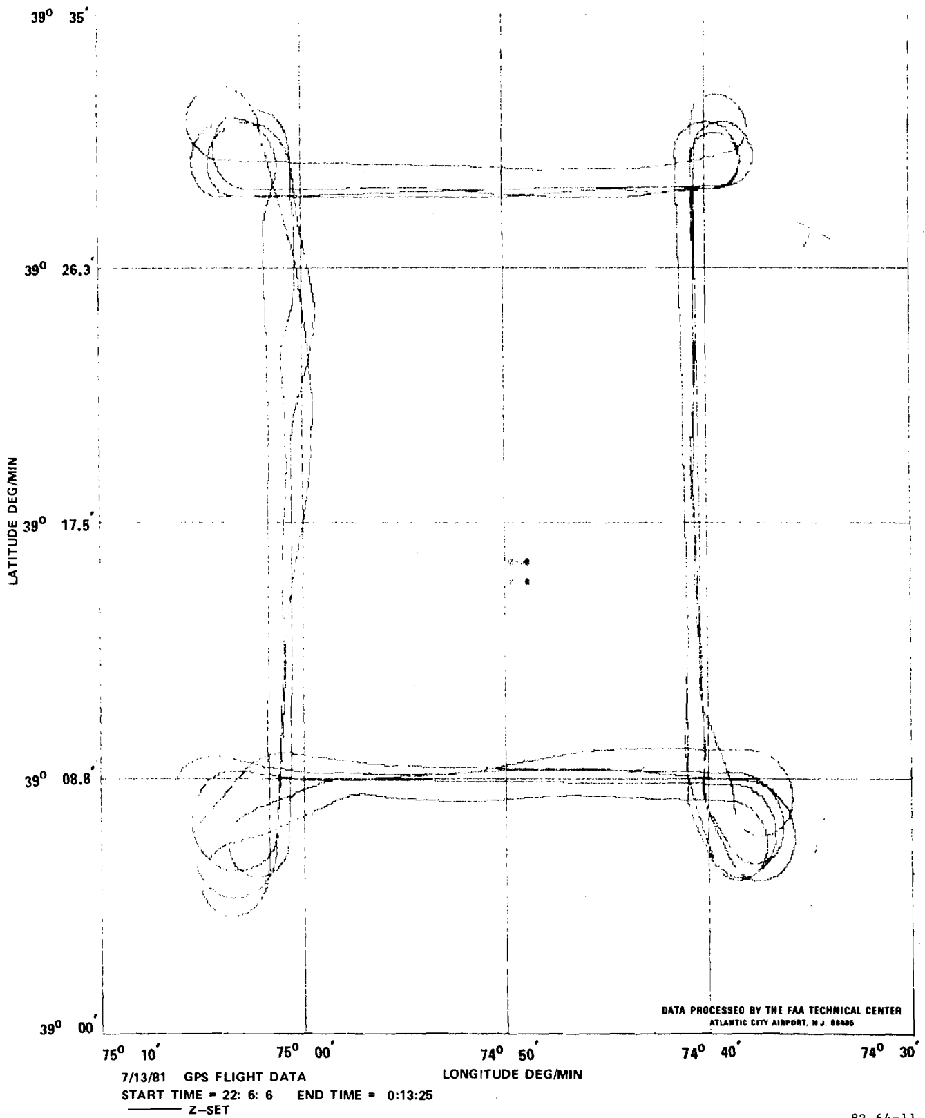
FIGURE 11. GPS DETERMINED FLIGHTPATH ON JULY 13, 1981
