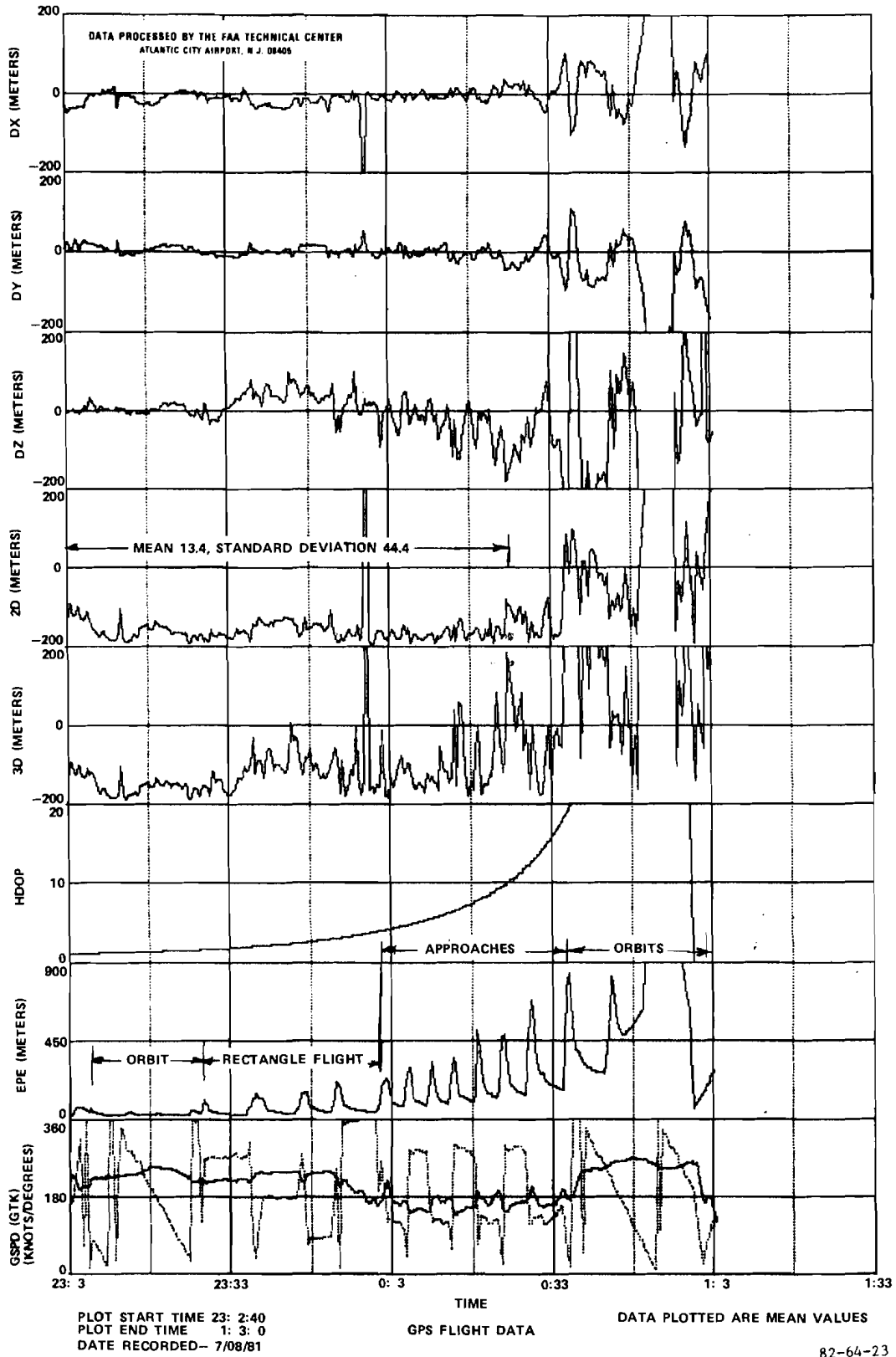
FIGURE 23. DELTA MEAN PLOT FOR JULY 8, 1981
