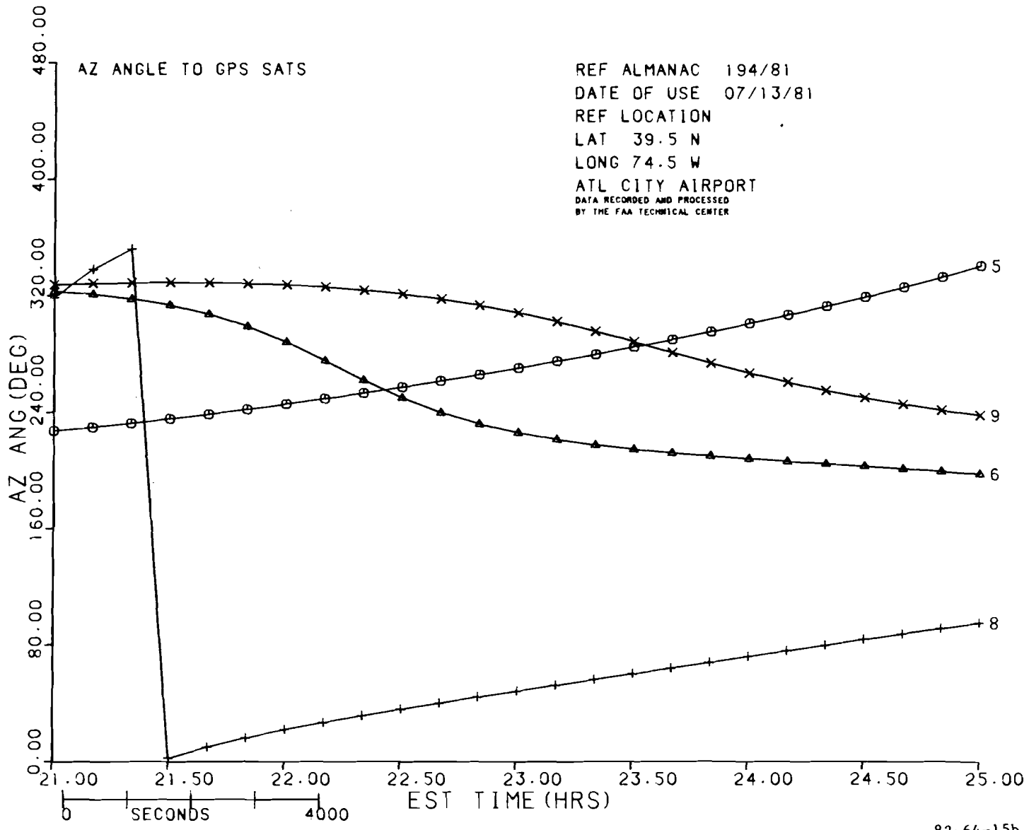
FIGURE 15. SATELLITE PATH PLOT FOR JULY 13, 1981 (SHEET 2 OF 2)
