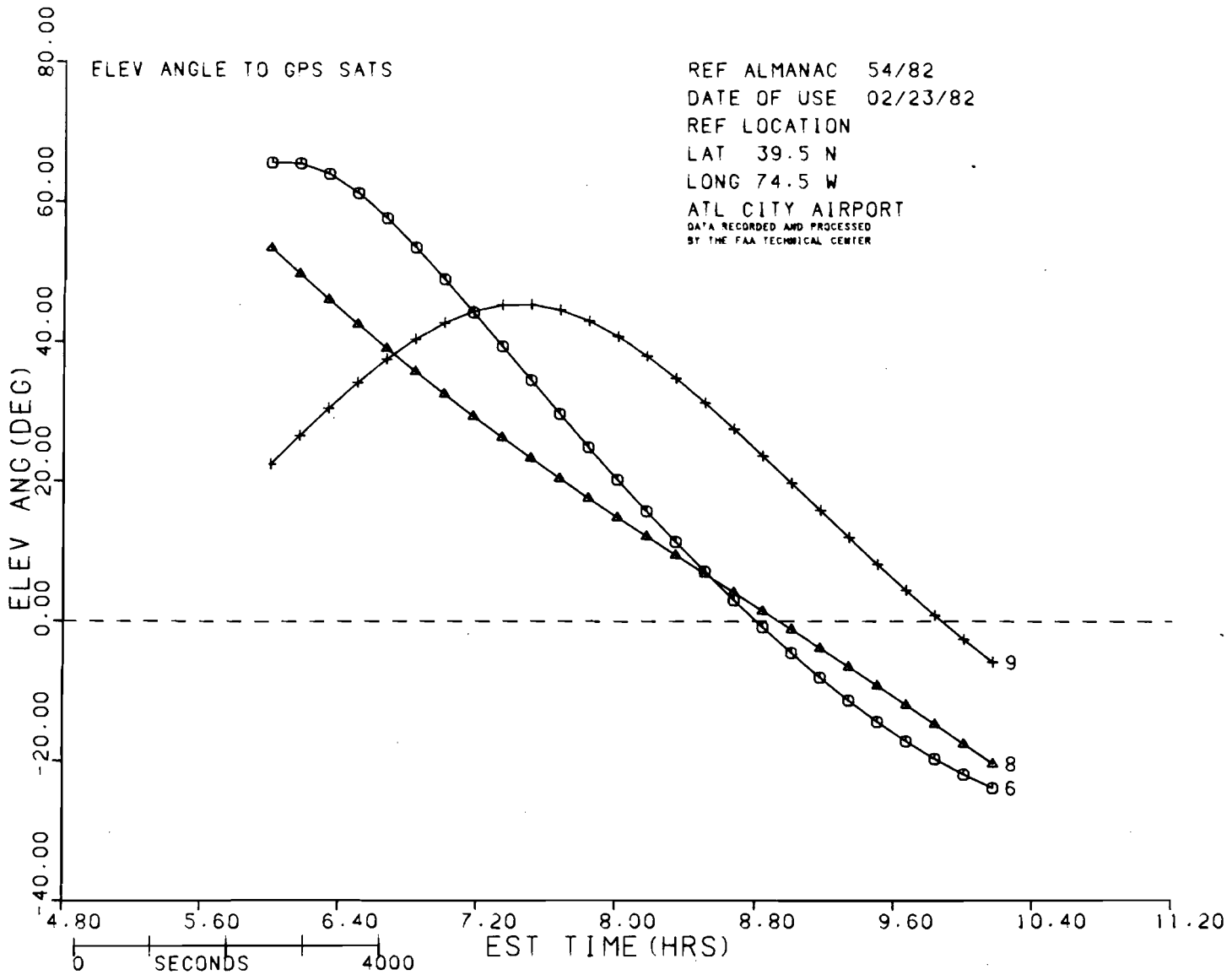
FIGURE 8. SATELLITE PATH PLOT FOR NAVIGATION MODE TEST ON FEBRUARY 23, 1982 (SHEET 1 OF 2)
