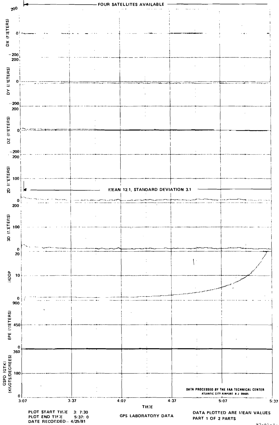
FIGURE 3. DELTA MEAN PLOT FOR CALIBRATION MODE ON APRIL 25, 1981 (SHEET 1 OF 2)
