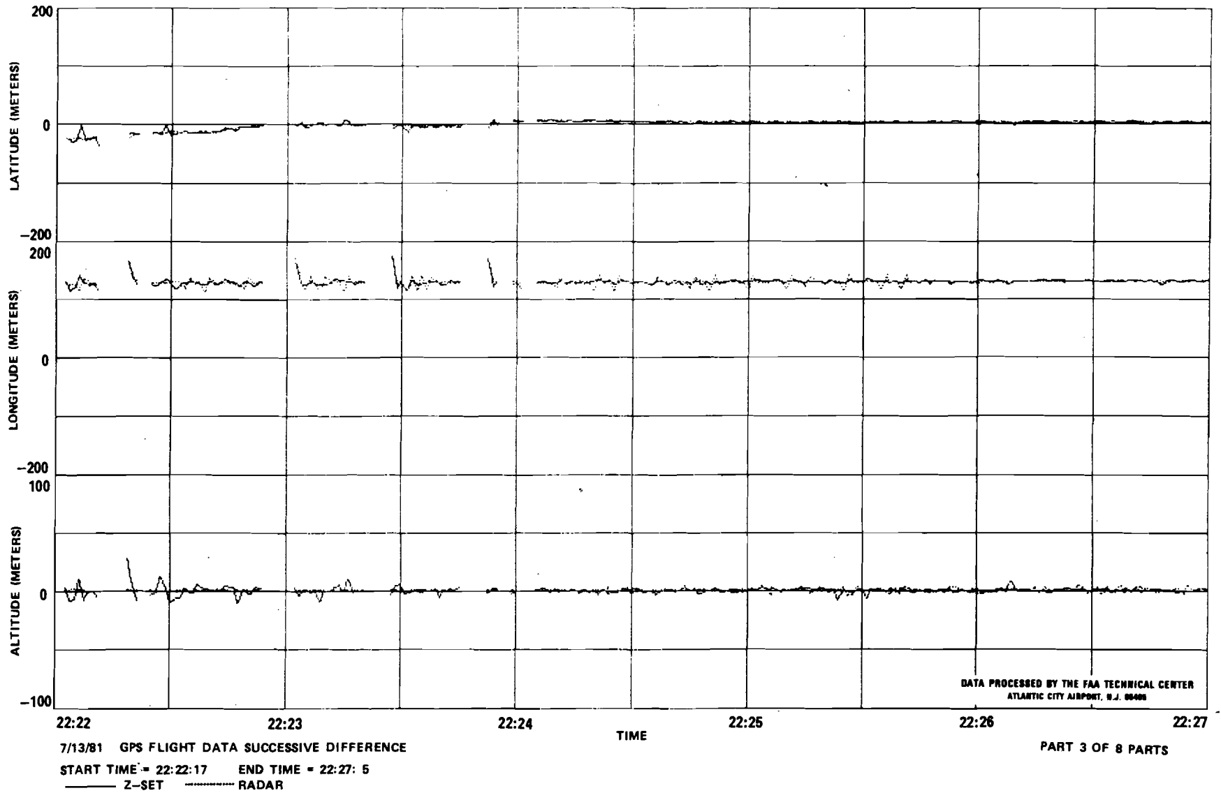
FIGURE 17. SUCCESSIVE DIFFERENCE PLOTS FOR JULY 13, 1981 (SHEET 3 OF 8)
