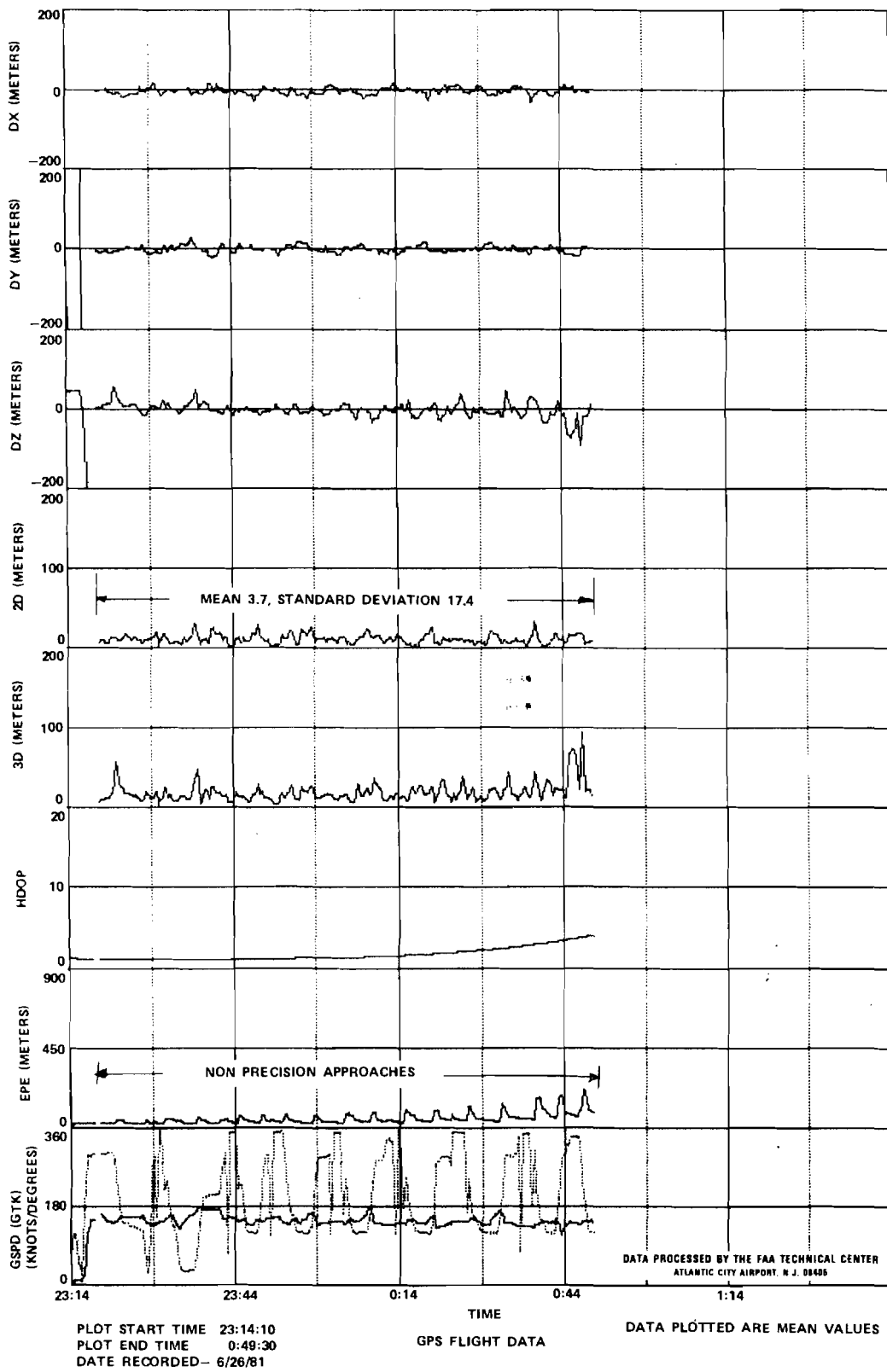
FIGURE 26. DELTA MEAN PLOT FOR JUNE 26, 1981
