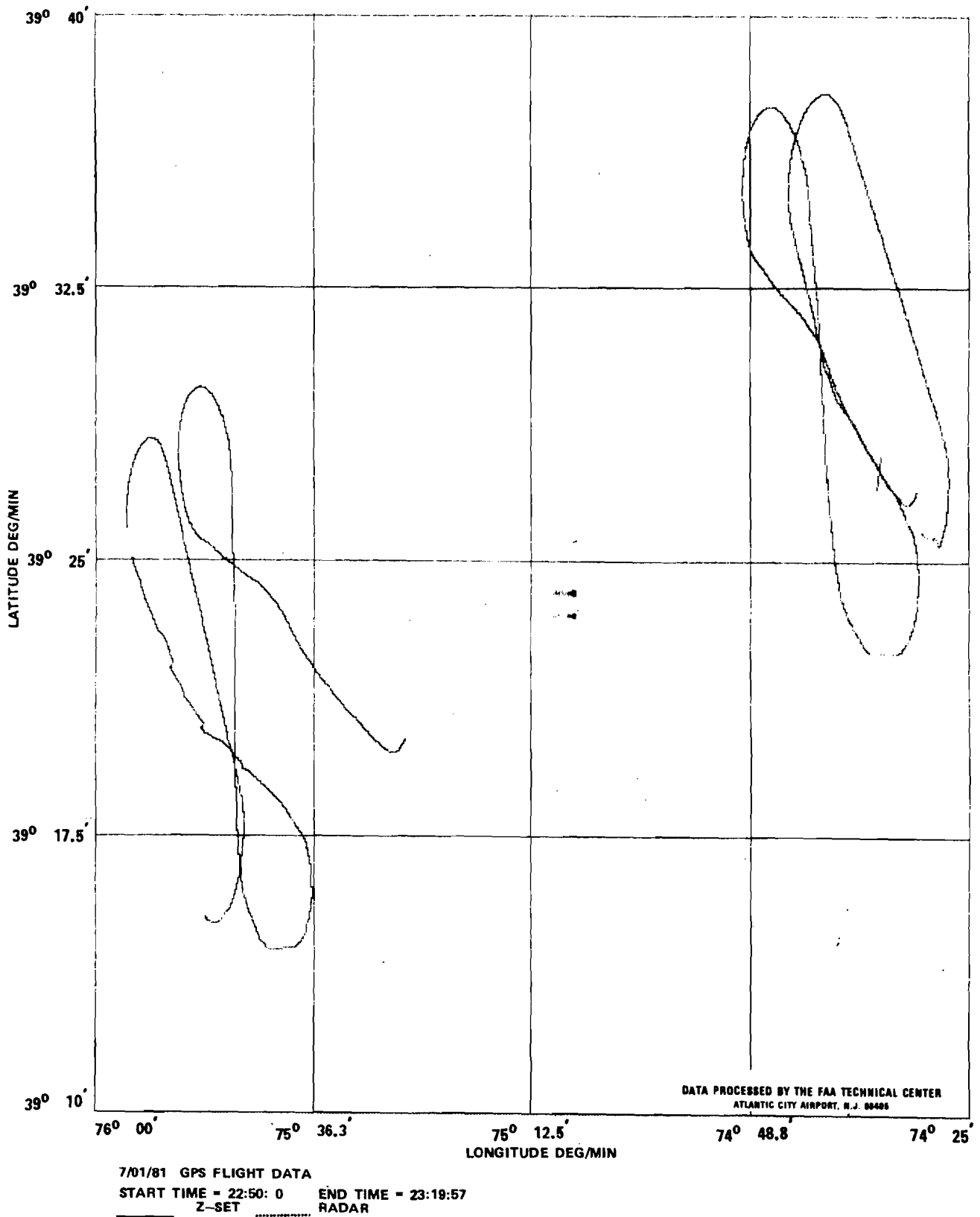
FIGURE 39. GPS AND RADAR DETERMINED FLIGHTPATH DURING Z-SET 4:3 STATUS ON JULY 1, 1981
