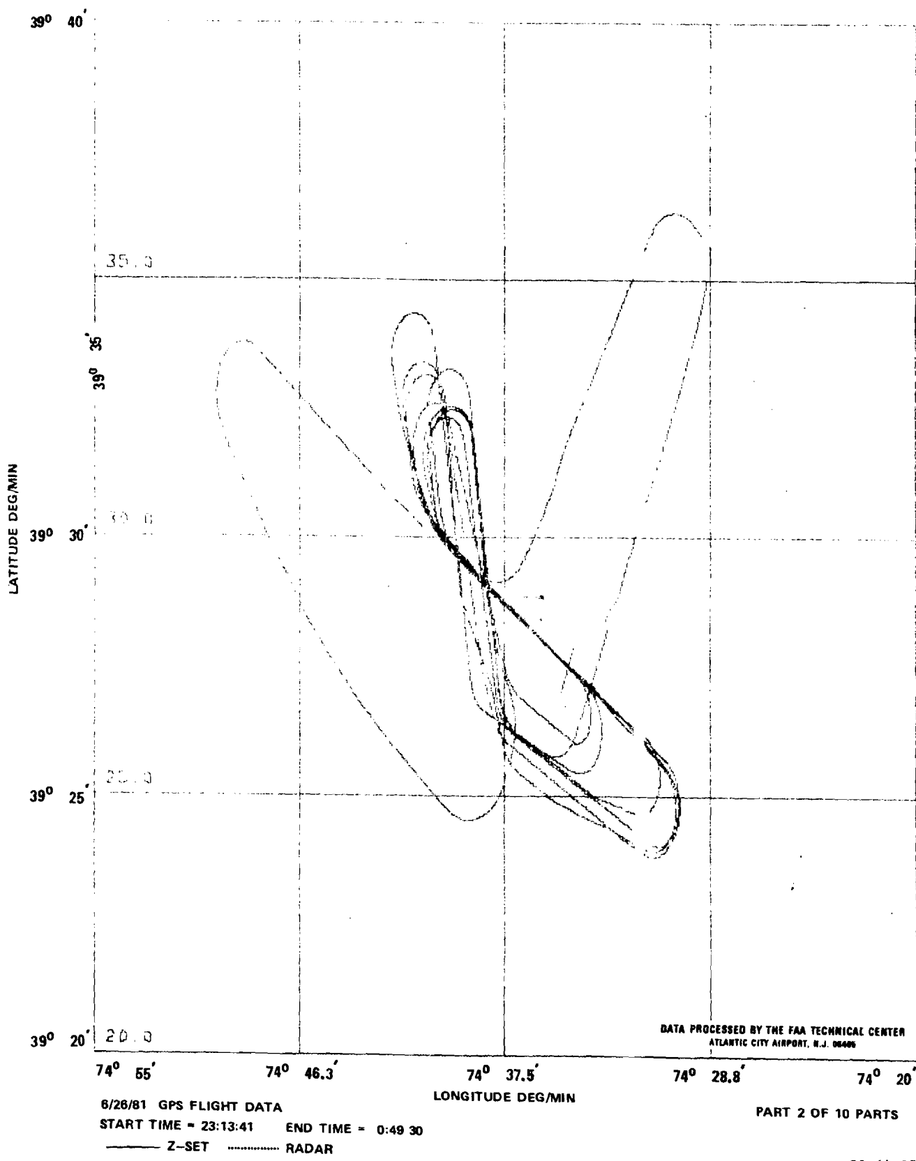
FIGURE 25. GPS AND RADAR DETERMINED NONPRECISION FLIGHTPATH ON JUNE 26, 1981 (SHEET 2 OF 10)
