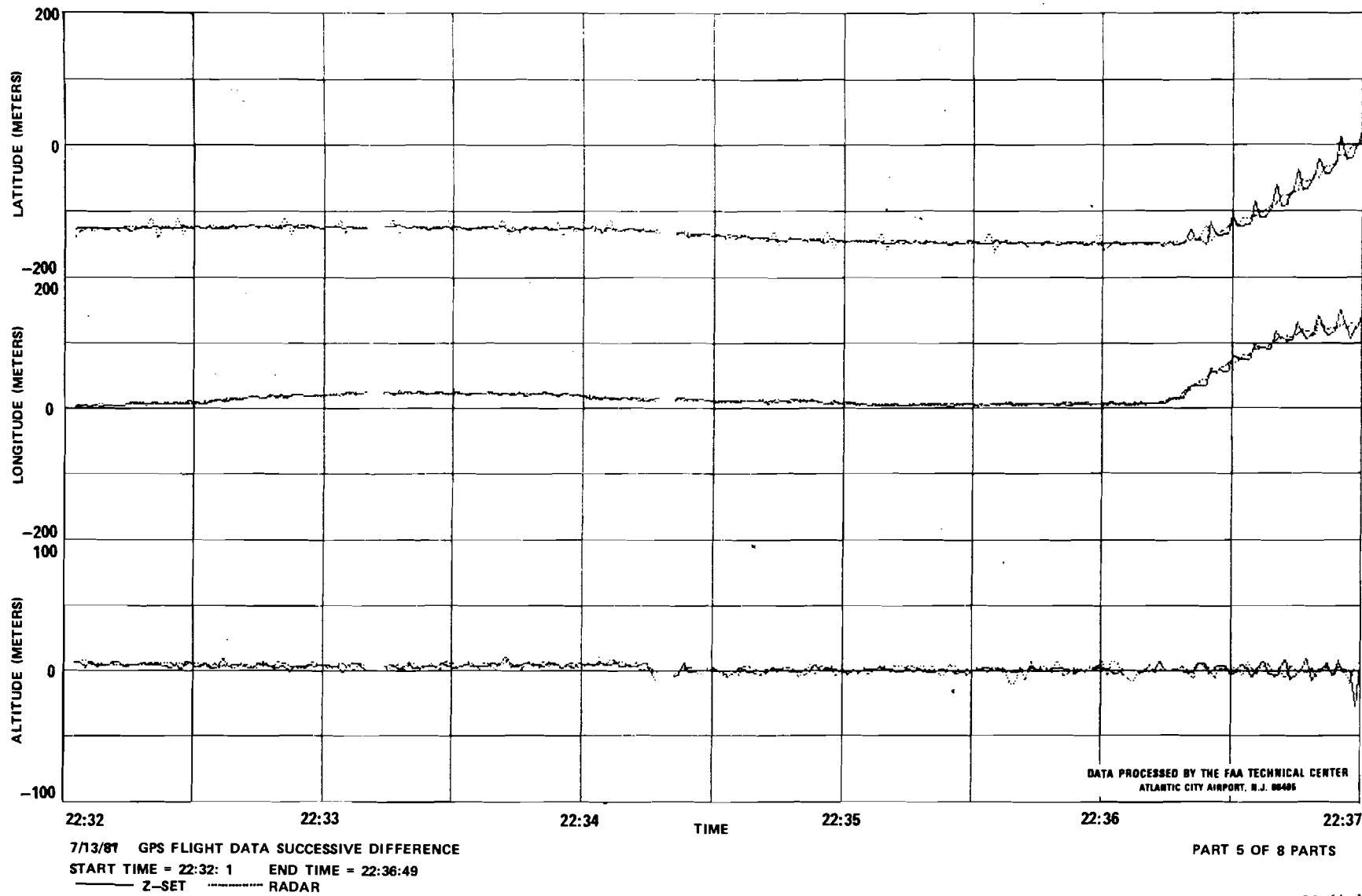
FIGURE 17. SUCCESSIVE DIFFERENCE PLOTS FOR JULY 13, 1981 (SHEET 5 OF 8)
