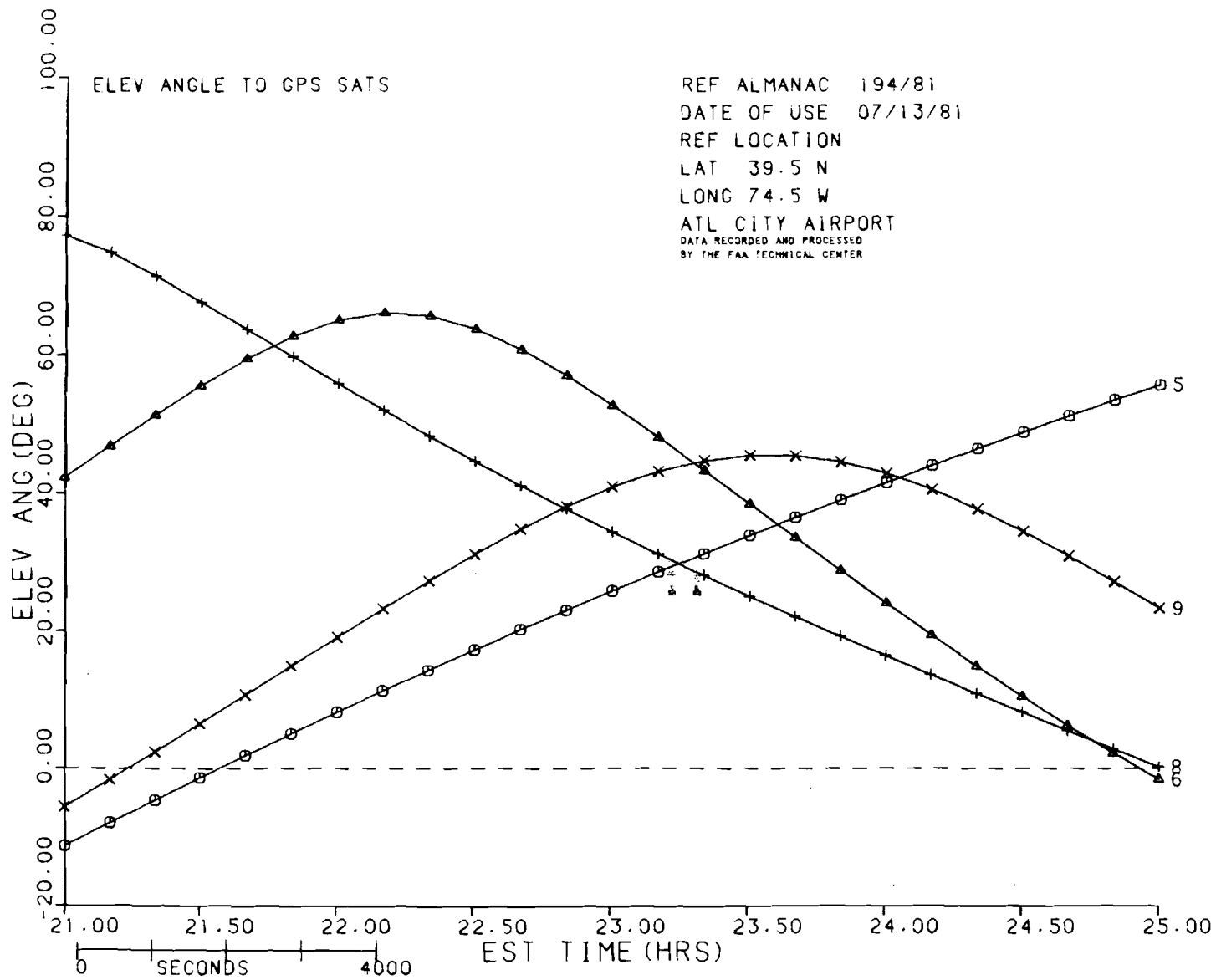
FIGURE 15. SATELLITE PATH PLOT FOR JULY 13, 1981 (SHEET 1 OF 2)
