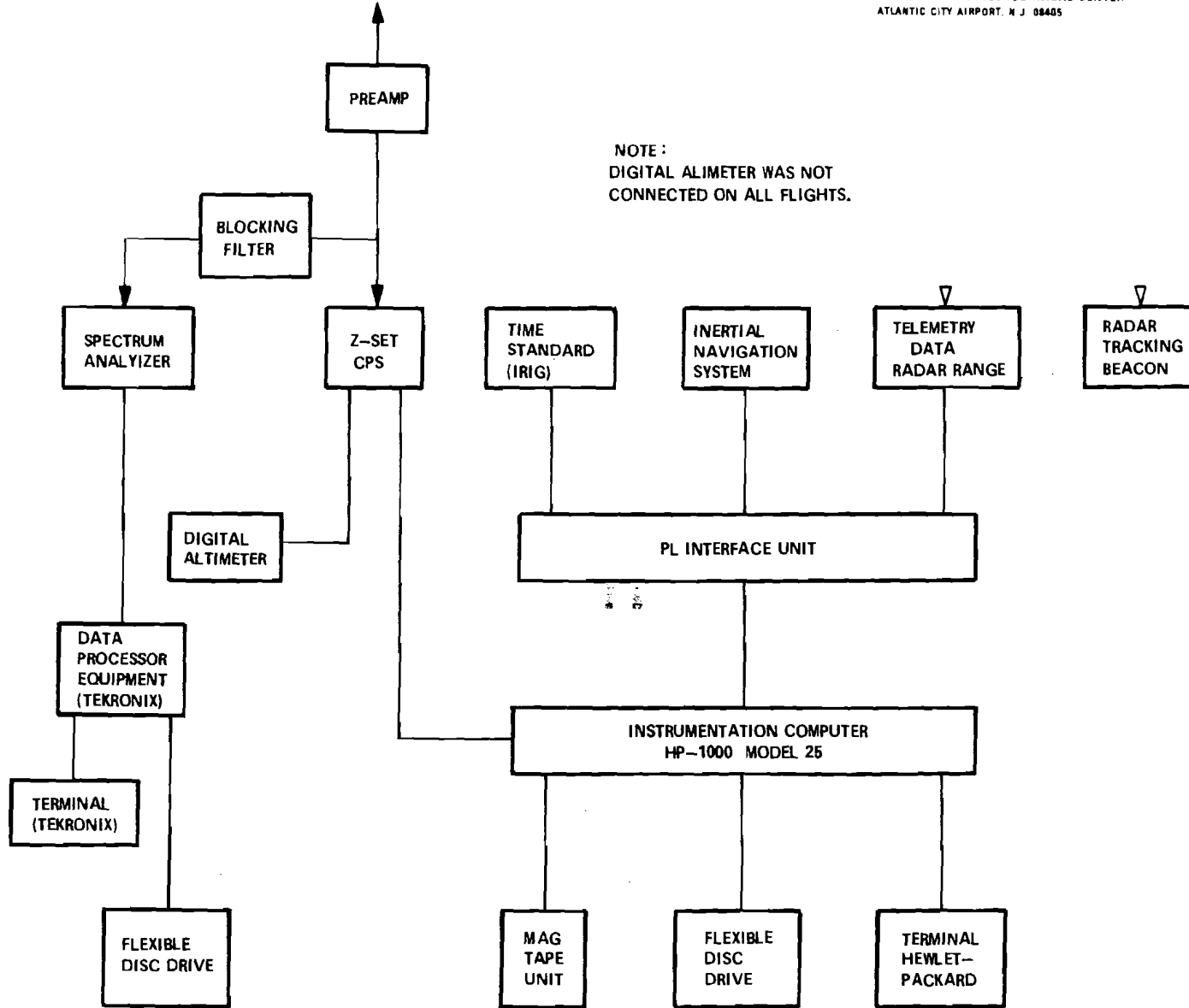
FIGURE 2. AIRBORNE TEST CONFIGURATION
