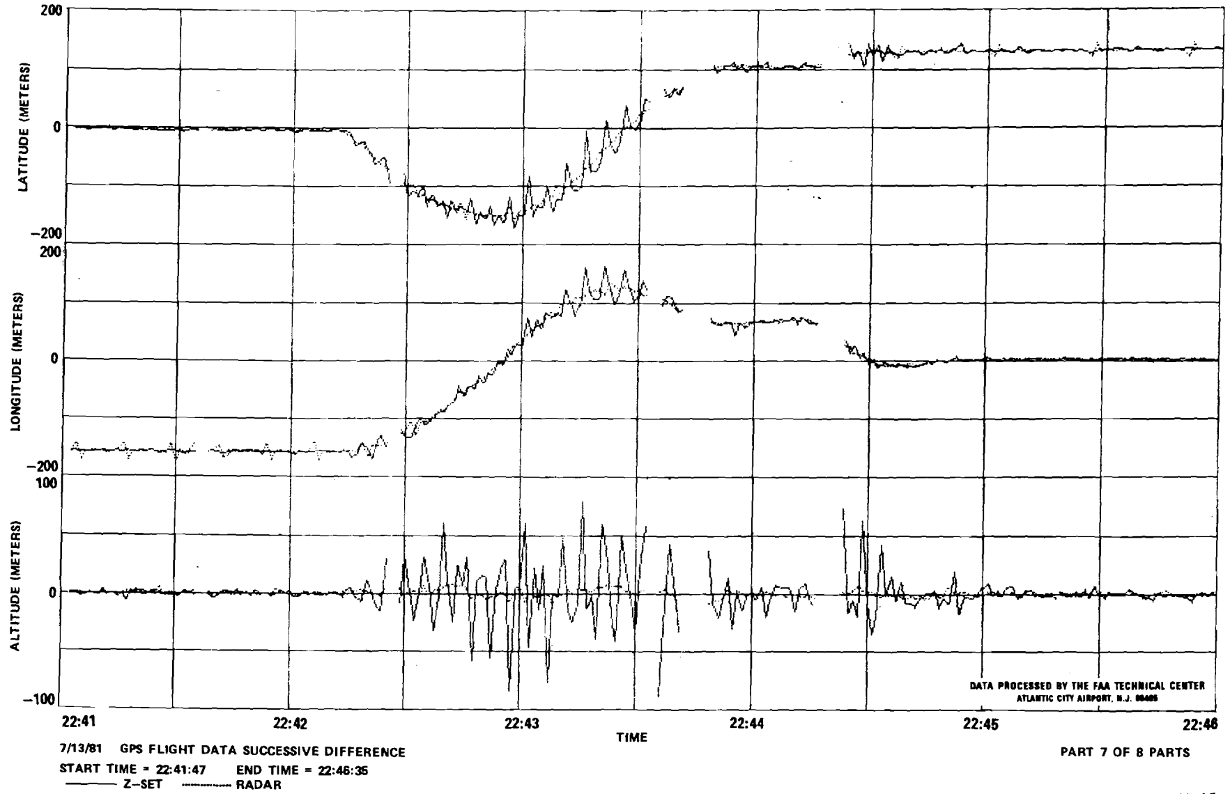
FIGURE 17. SUCCESSIVE DIFFERENCE PLOTS FOR JULY 13, 1981 (SHEET 7 OF 8)
