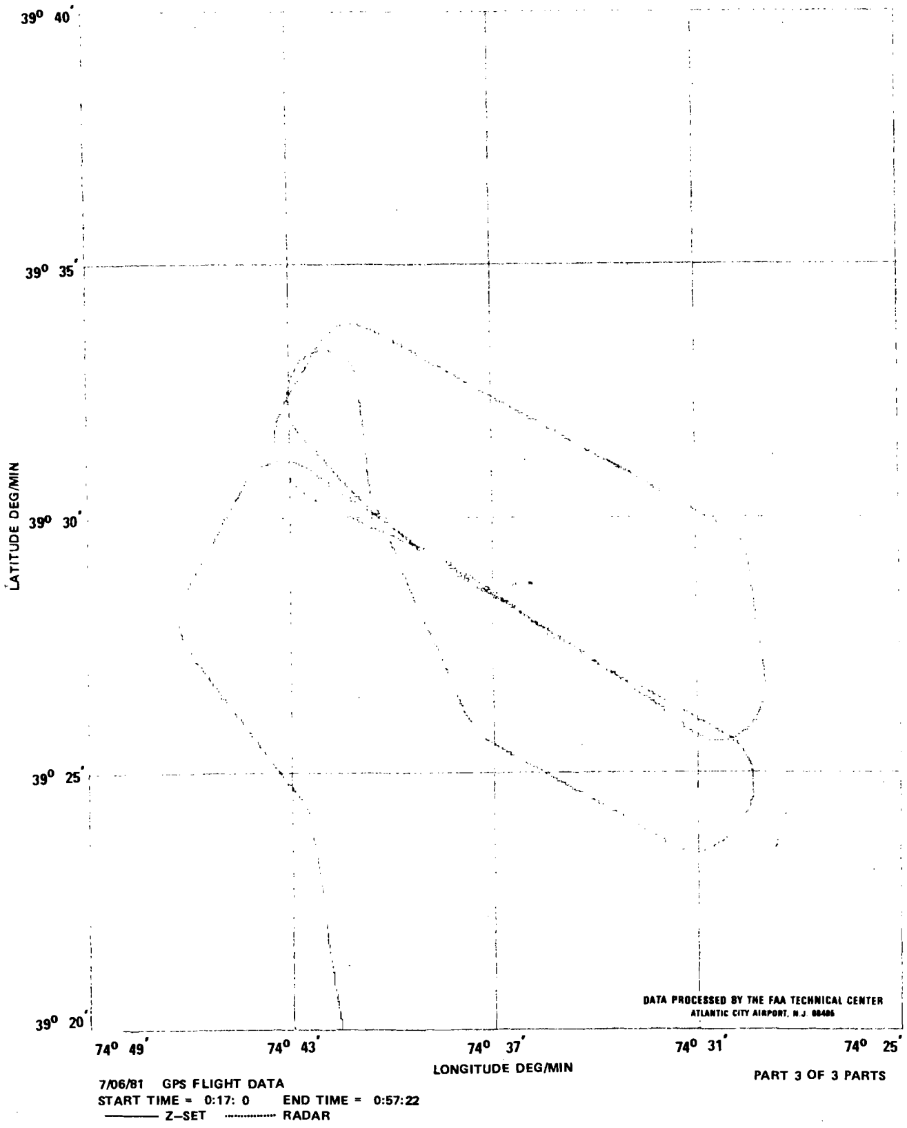
FIGURE 27. GPS AND RADAR DERIVED NONPRECISION FLIGHTPATH ON JULY 6, 1981 (SHEET 3 OF 3)
