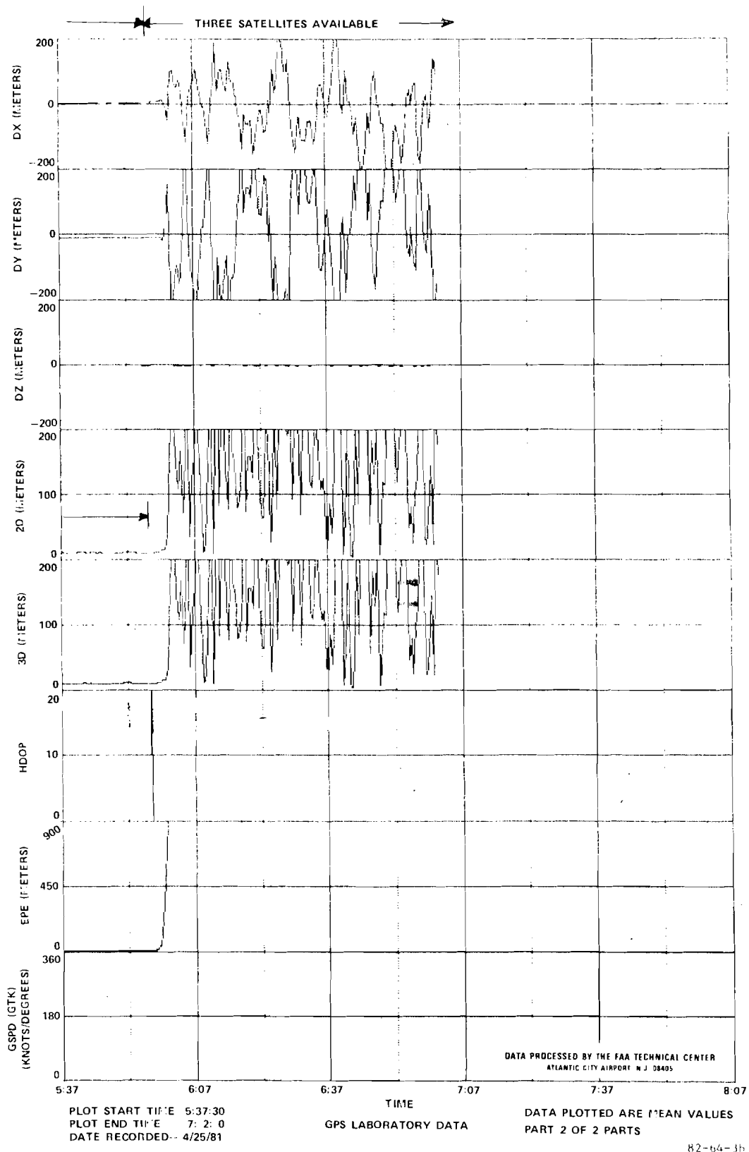
FIGURE 3. DELTA MEAN PLOT FOR CALIBRATION MODE ON APRIL 25, 1981 (SHEET 2 OF 2)
