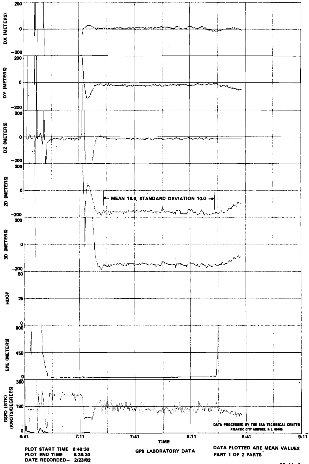
FIGURE 9. DELTA MEAN PLOT FOR NAVIGATION MODE WITH ALTIMETER ON FEBRUARY 23, 1982 (SHEET 1 OF 2)
