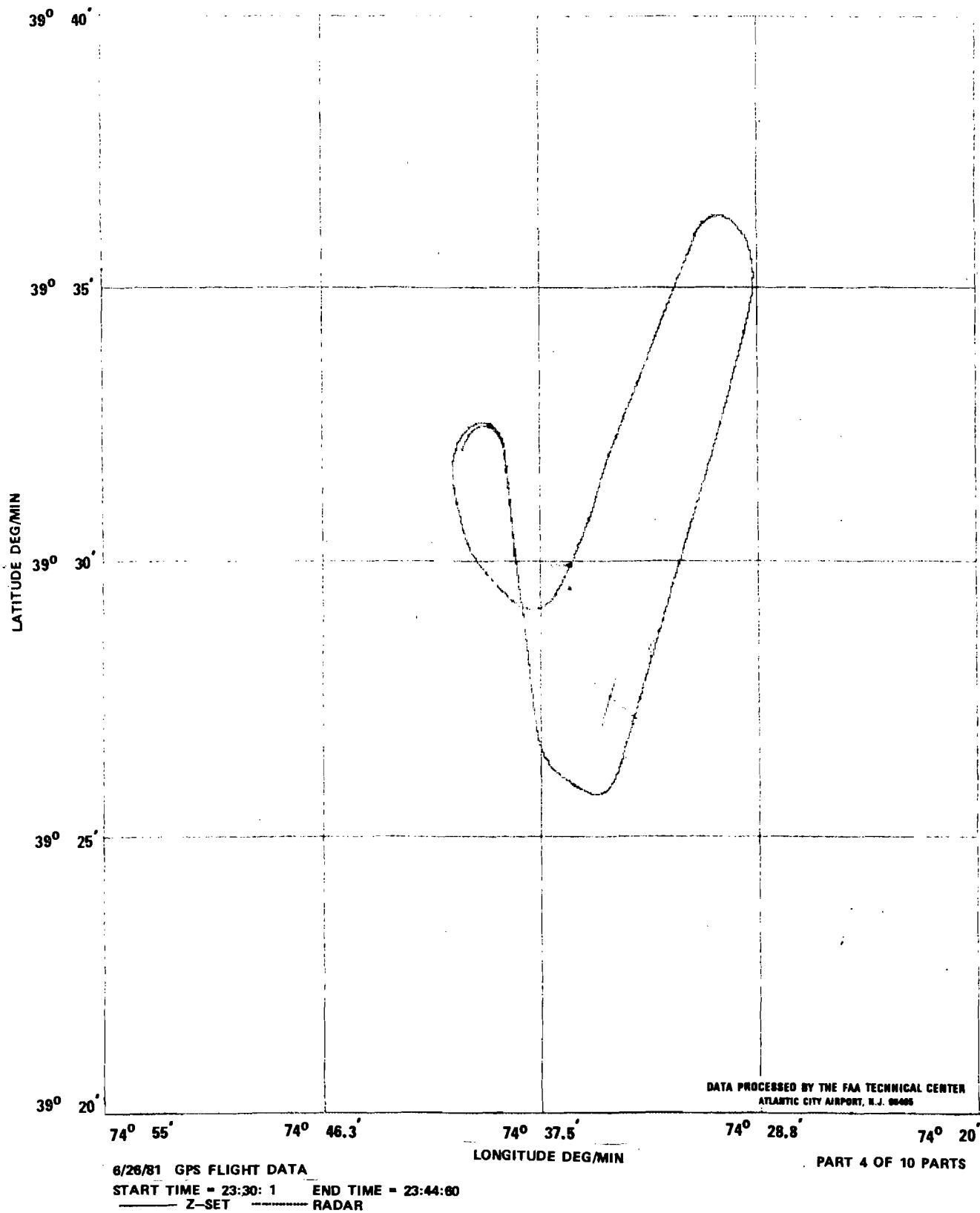
FIGURE 25. GPS AND RADAR DETERMINED NONPRECISION FLIGHTPATH ON JUNE 26, 1981 (SHEET 4 OF 10)
