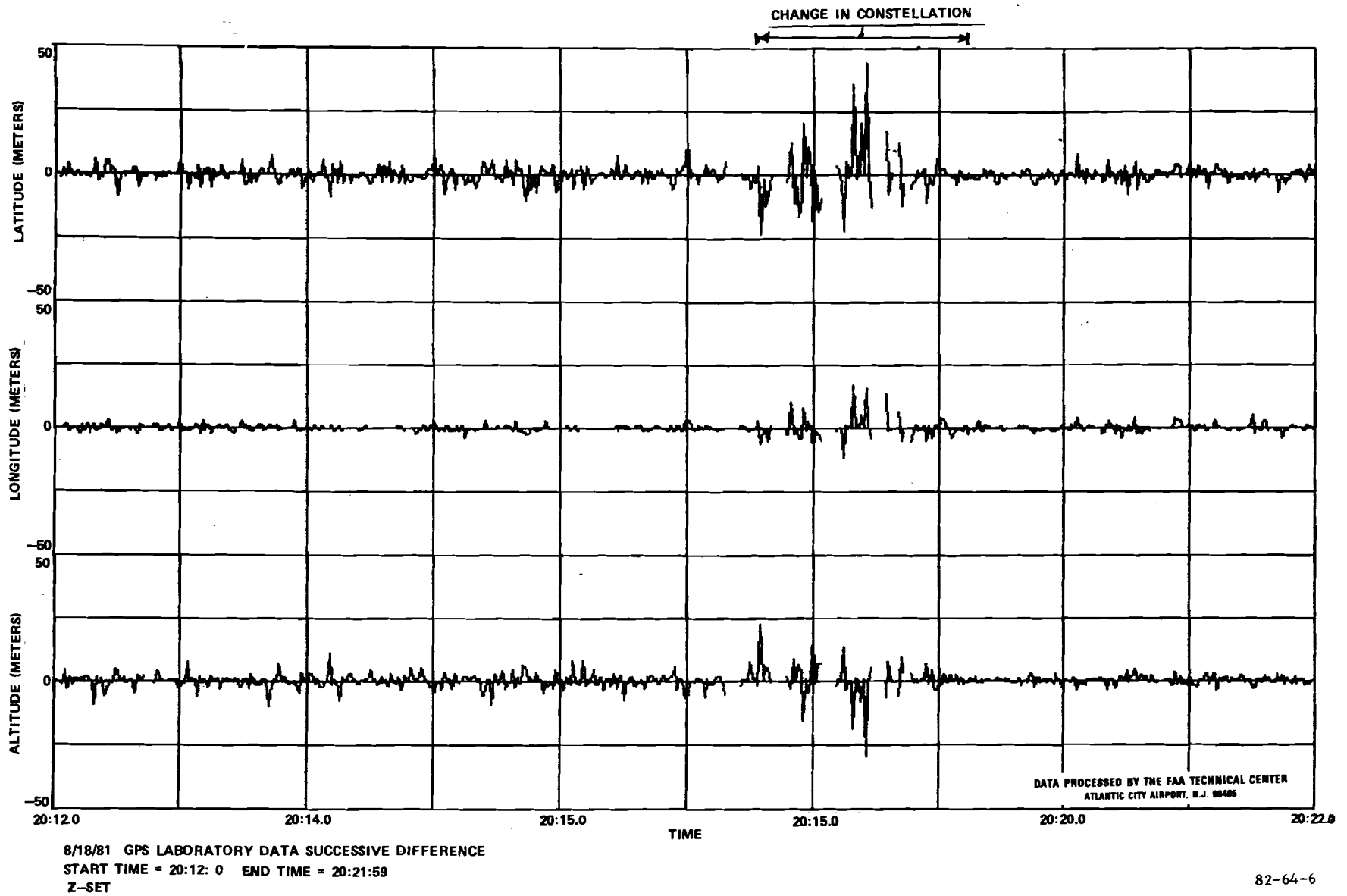
FIGURE 6. SUCCESSIVE DIFFERENCE PLOT SHOWING CHANGE IN SATELLITE CONSTELLATION ON AUGUST 18, 1981
