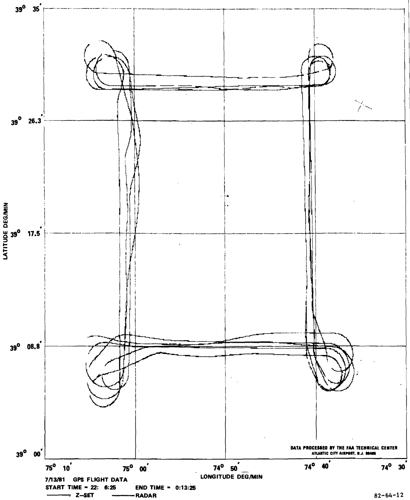
FIGURE 12. GPS AND RADAR DETERMINED FLIGHTPATH ON JULY 13, 1981
