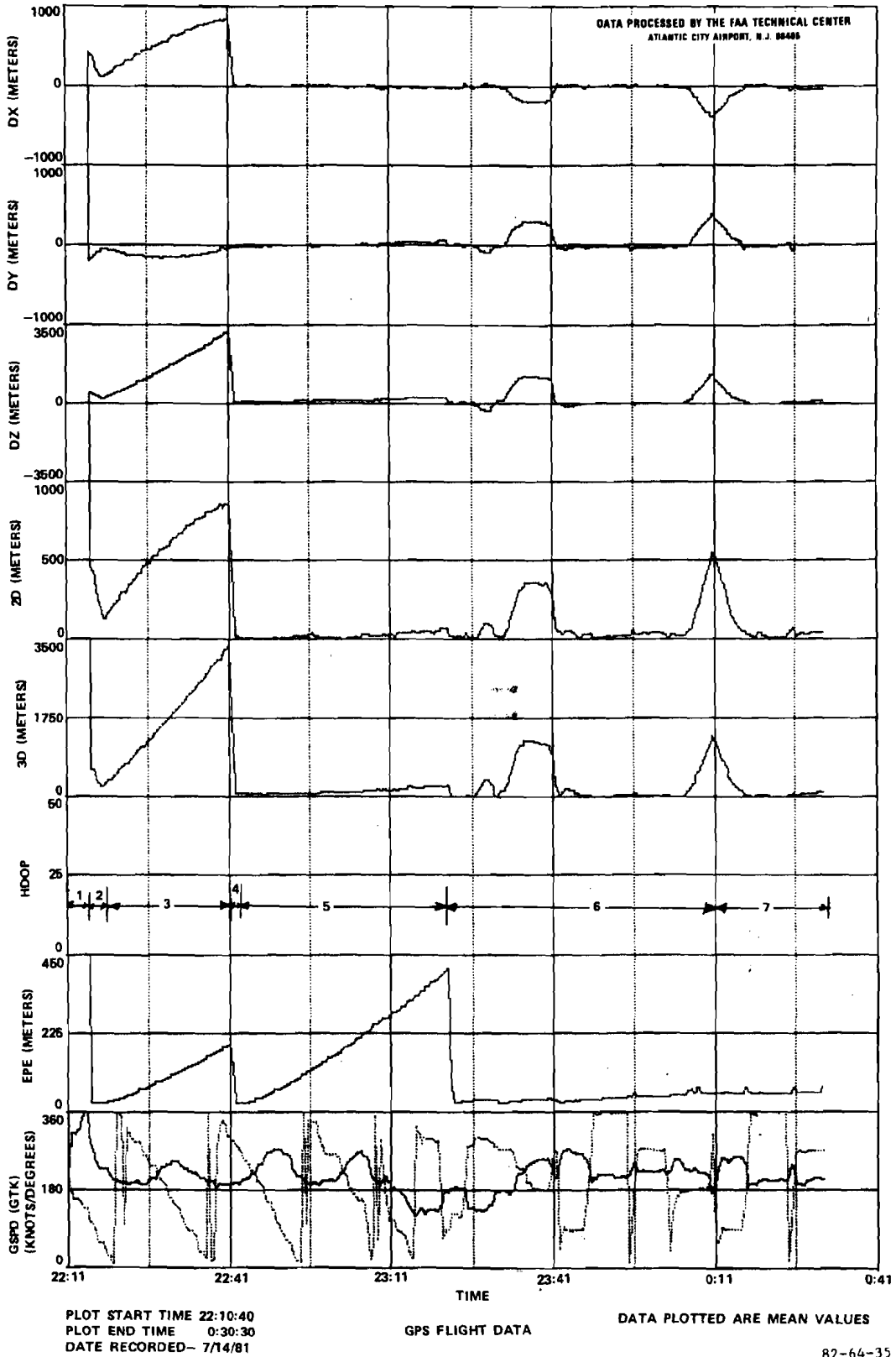
FIGURE 35. DELTA MEAN PLOT FOR JULY 14, 1981, FLIGHT TESTING DIGITAL ALTITUDE INPUT
