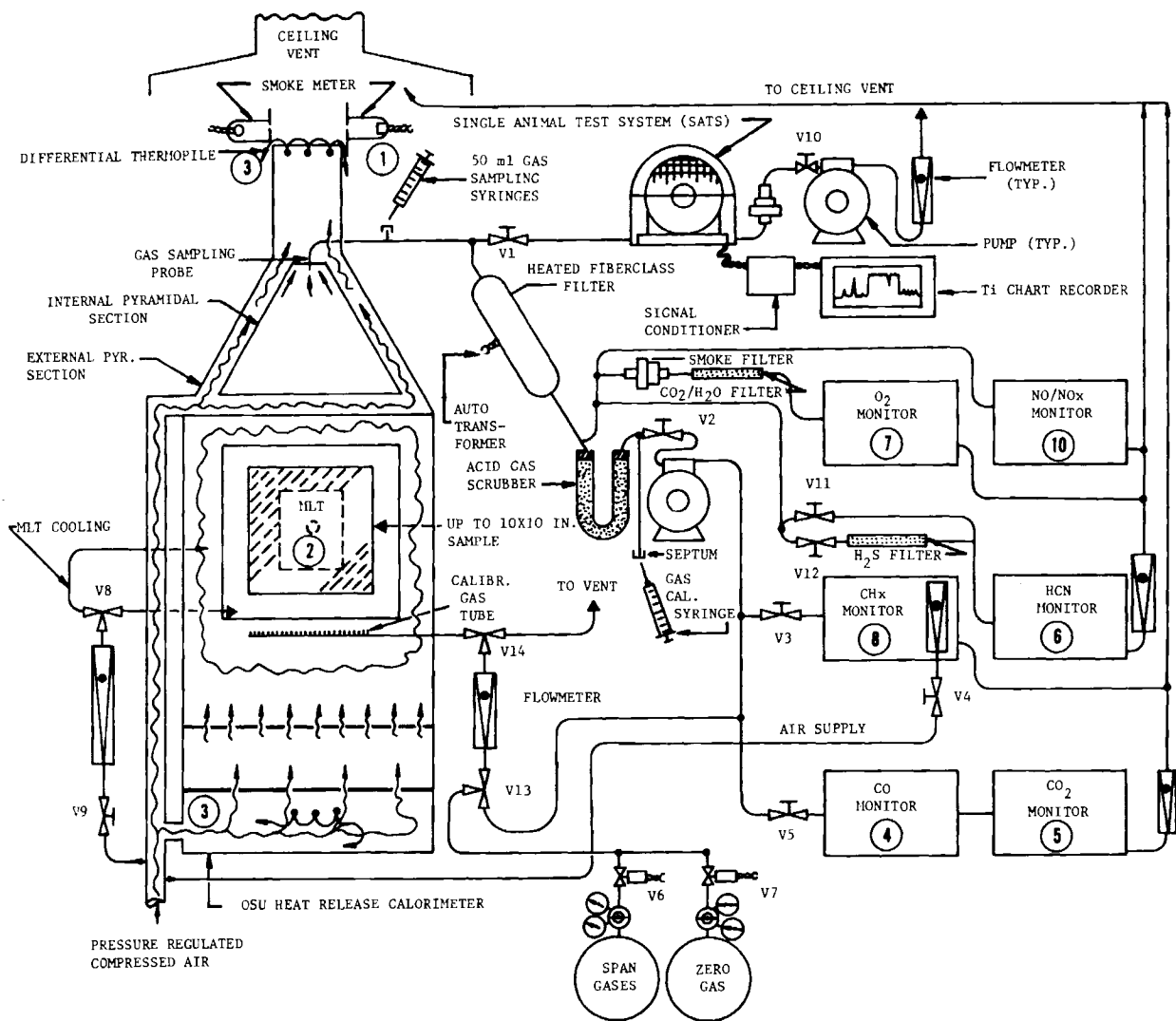
FIGURE 8. SCHEMATIC DIAGRAM OF THE CHAS/SATS
