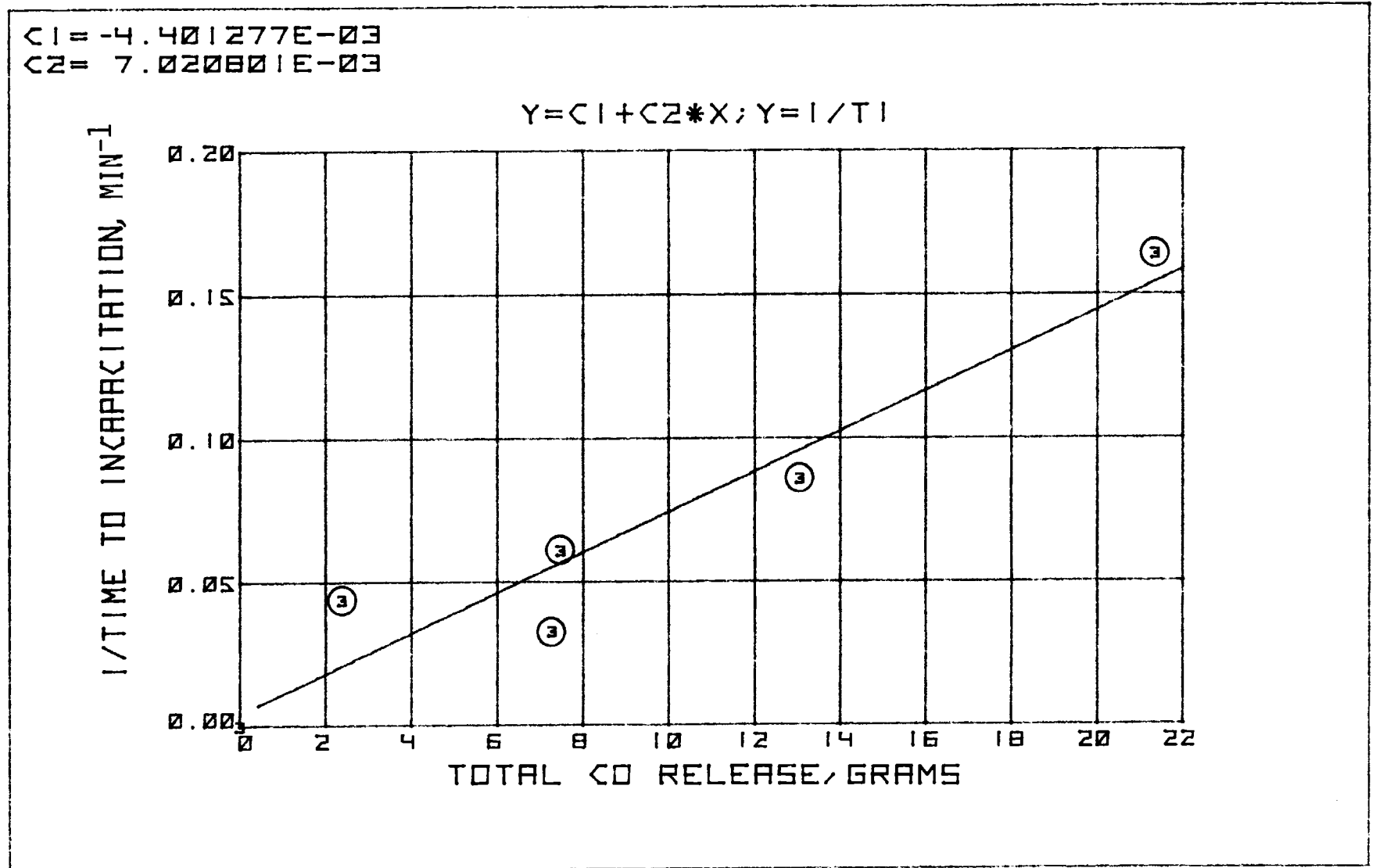
FIGURE 37. CORRELATION OF 1/T_i ( \text{MIN}^{-1} ) VALUES WITH PANEL 3 CHAS/SATS CO YIELDS
