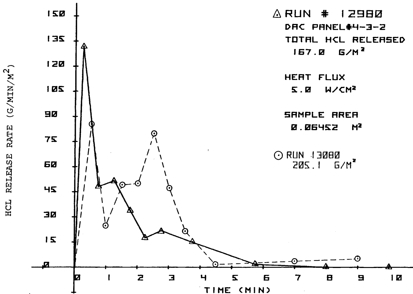
FIGURE 28. HYDROGEN CHLORIDE RELEASE RATES FOR TWO TESTS OF PANEL 4 AT 4.41 Btu/ft 2 SEC (AT DIFFERENT TIME INTERVALS)
