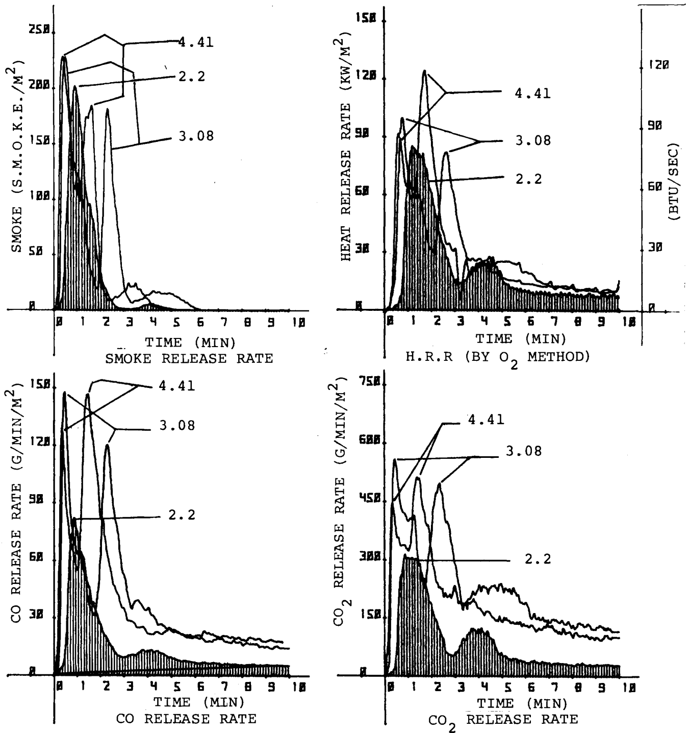
FIGURE 34. CHAS HAZARDS RELEASE RATES COMPARISON OF PARTITION PANEL NO. 4 TESTED AT 3 HEAT FLUXES 2.2, 3.08, AND 4.41 Btu/ft 2 SEC (Sheet 1 of 3)
