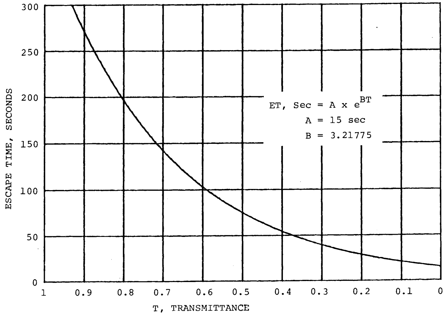
FIGURE 14. ESCAPE TIME VERSUS LIGHT TRANSMITTANCE THROUGH SMOKE
