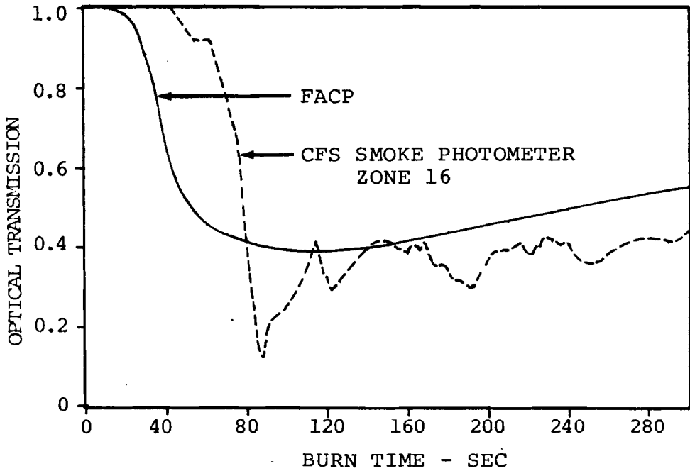
FIGURE 52. COMPARISON OF SMOKE EVOLUTION PROFILES - SINGLE ZONE FACP PREDICTION WITH CFS EXHAUST READINGS FOR PANEL 2 AT 2.2 Btu/ft 2 SEC
