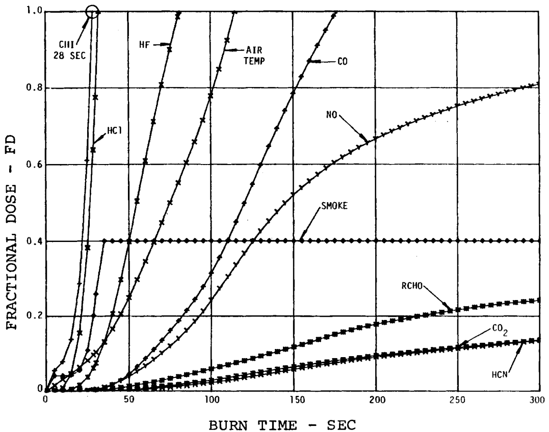
FIGURE 75. TWENTY ZONE FACP CHI AND FRACTIONAL DOSE PLOTS PANEL 4 AT 4.41 Btu/ft 2 SEC
