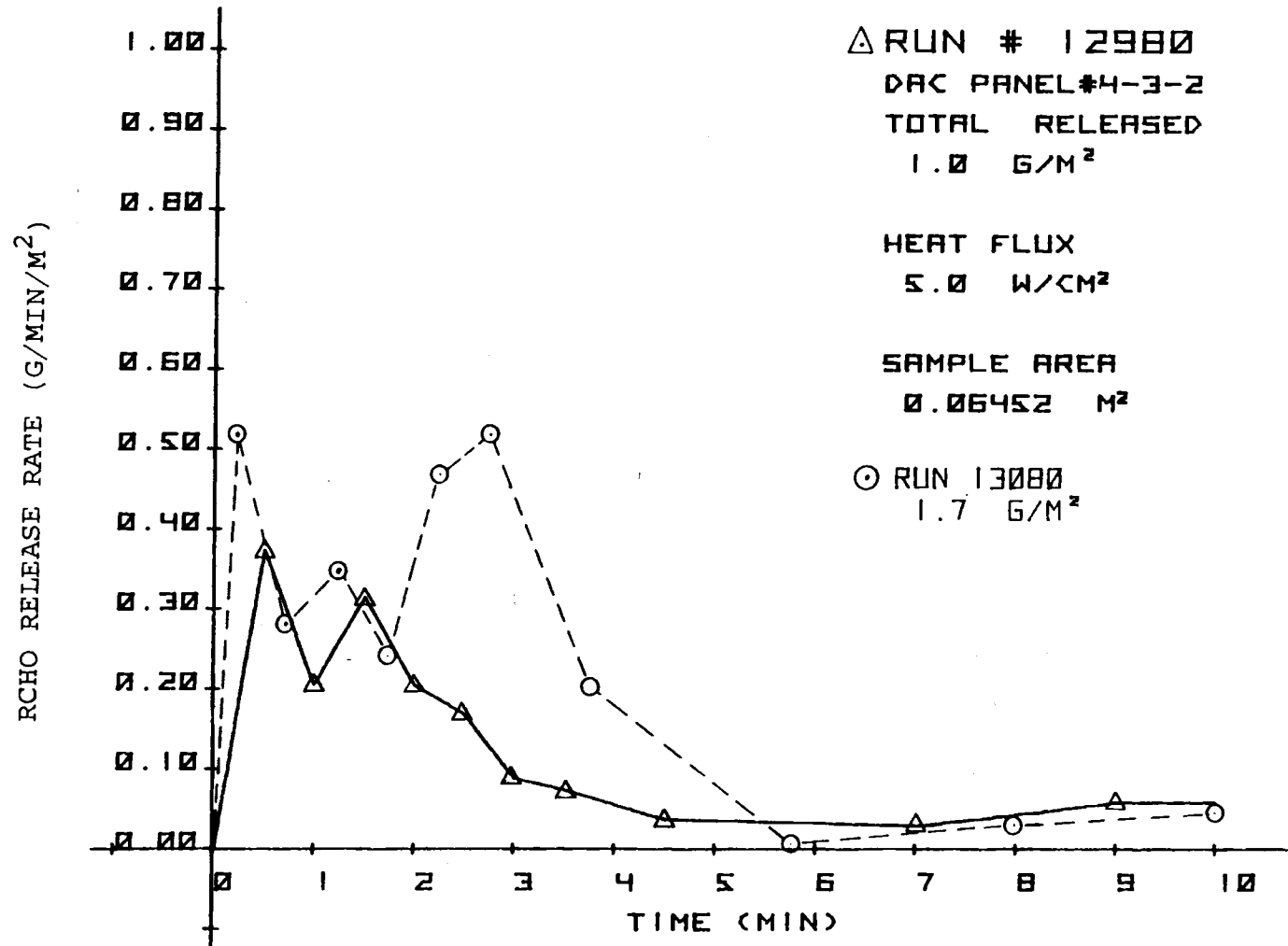
FIGURE 26 ALIPHATIC ALDEHYDE RELEASE RATES FOR TWO TESTS OF PANEL 4 AT 4.41 Btu/ft 2 sec (AT DIFFERENT TIME INTERVALS)
