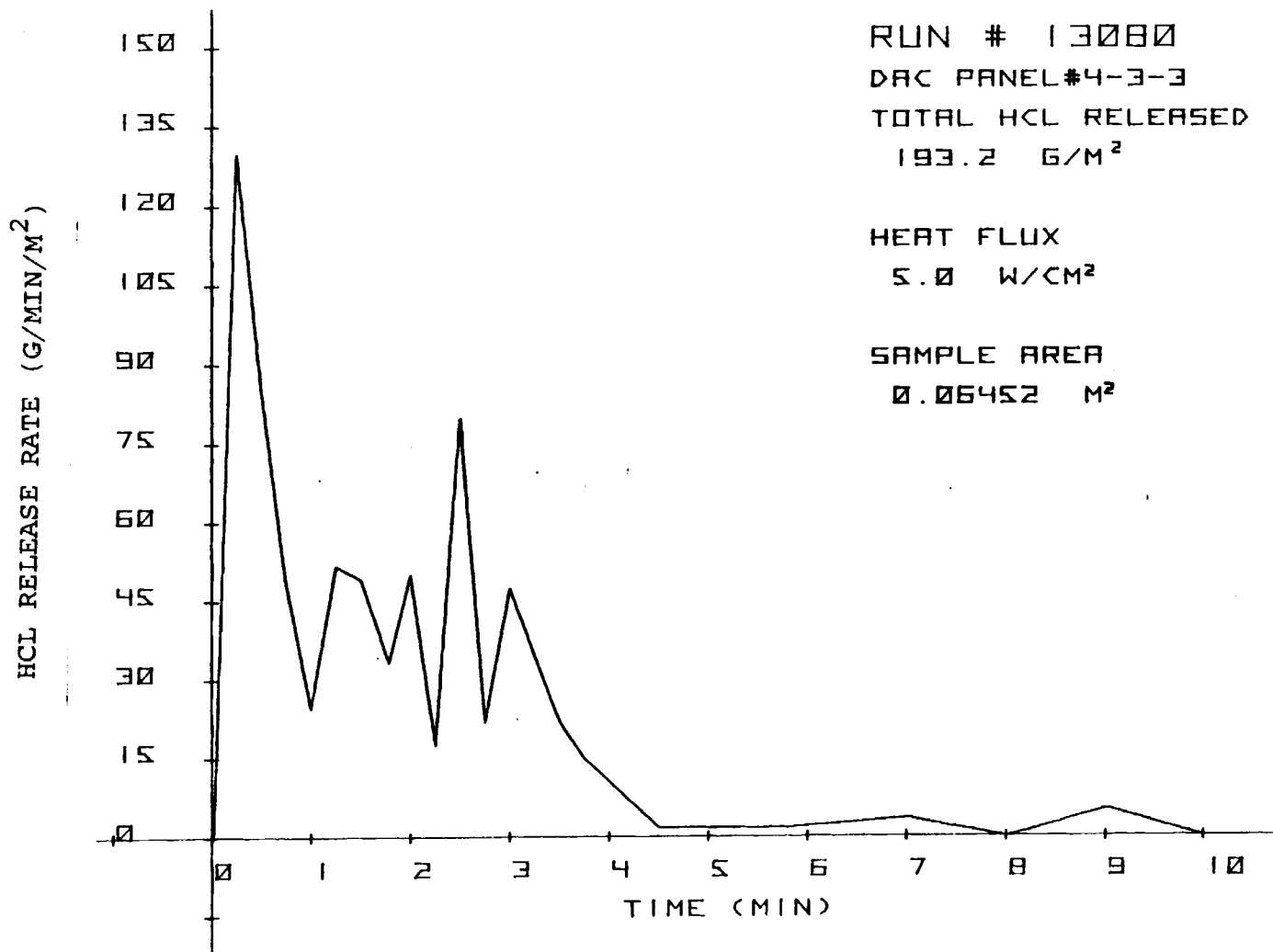
FIGURE 29. HYDROGEN CHLORIDE RELEASE RATE COMPOSITED FROM PANEL 4 TESTS (FIGURE 28)
