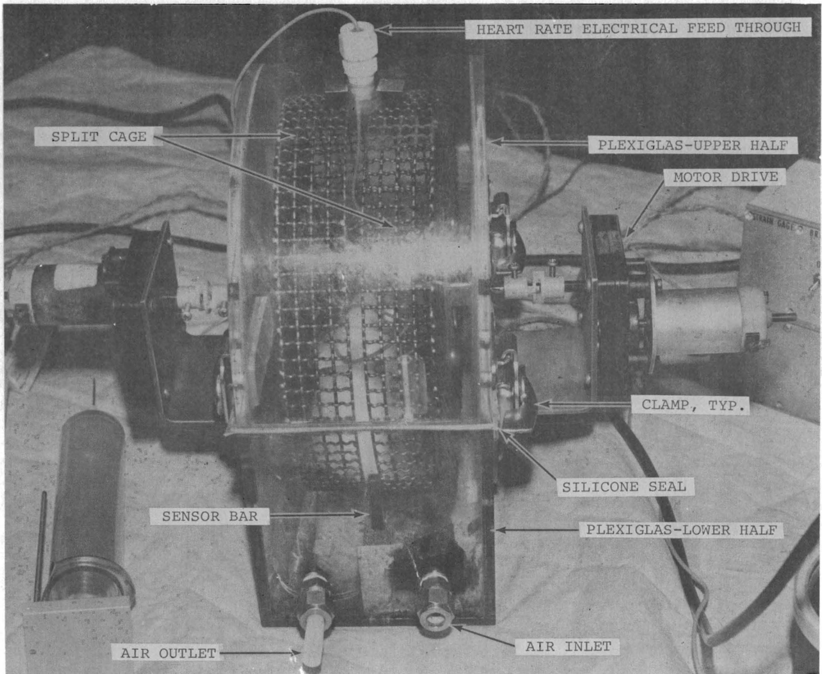
FIGURE 6. SINGLE ANIMAL TEST SYSTEM (SATS)
