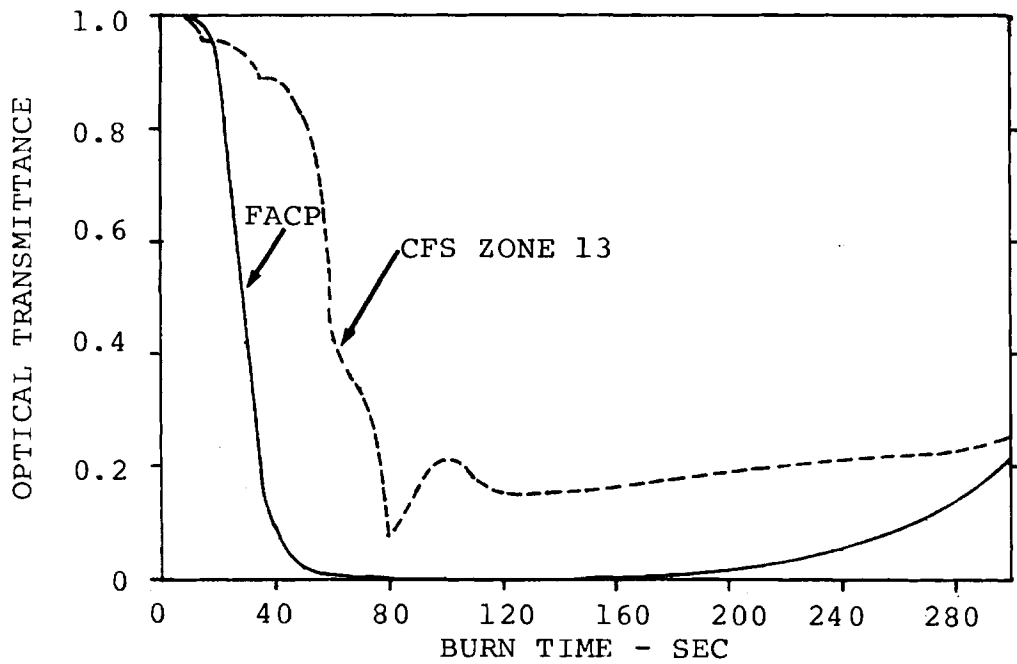
FIGURE 65. COMPARISON OF SMOKE OPTICAL TRANSMITTANCE OF CFS (ZONE 13) WITH 20 ZONE FACP PREDICTION PANEL 4 AT 4.41 Btu/ft 2 SEC
