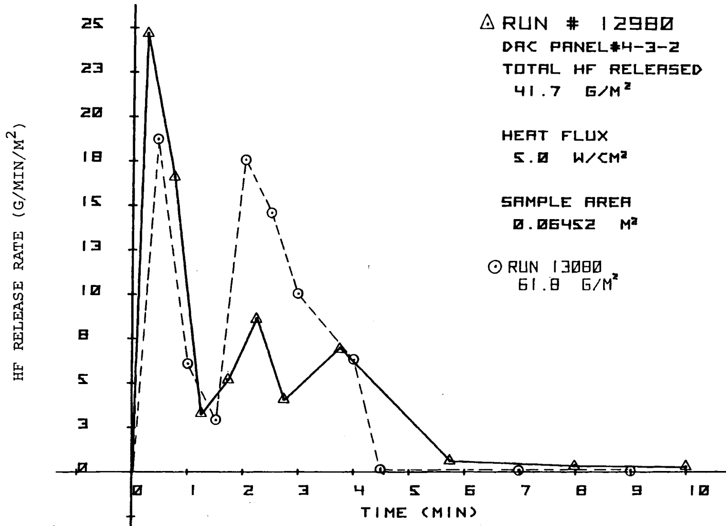
FIGURE 30. HYDROGEN FLUORIDE RELEASE RATES FOR TWO TESTS OF PANEL 4 AT 4.41 Btu/Ft 2 SEC (AT DIFFERENT TIME INTERVALS)
