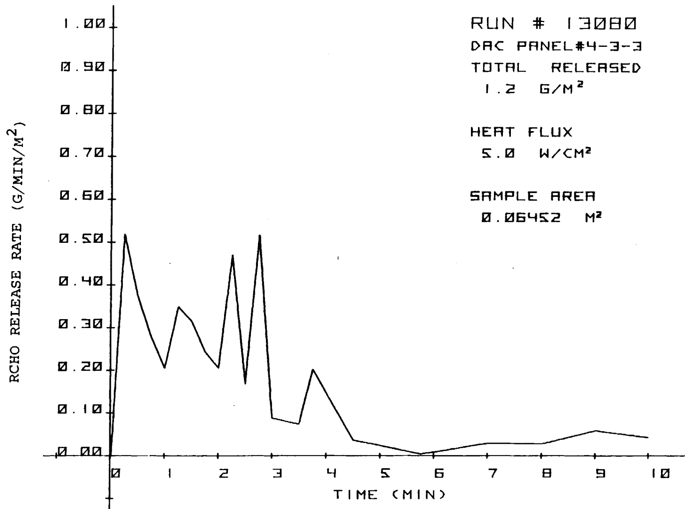
FIGURE 27 ALIPHATIC ALDEHYDE RELEASE RATE COMPOSITED FROM PANEL 4 TESTS (FIGURE 26)
