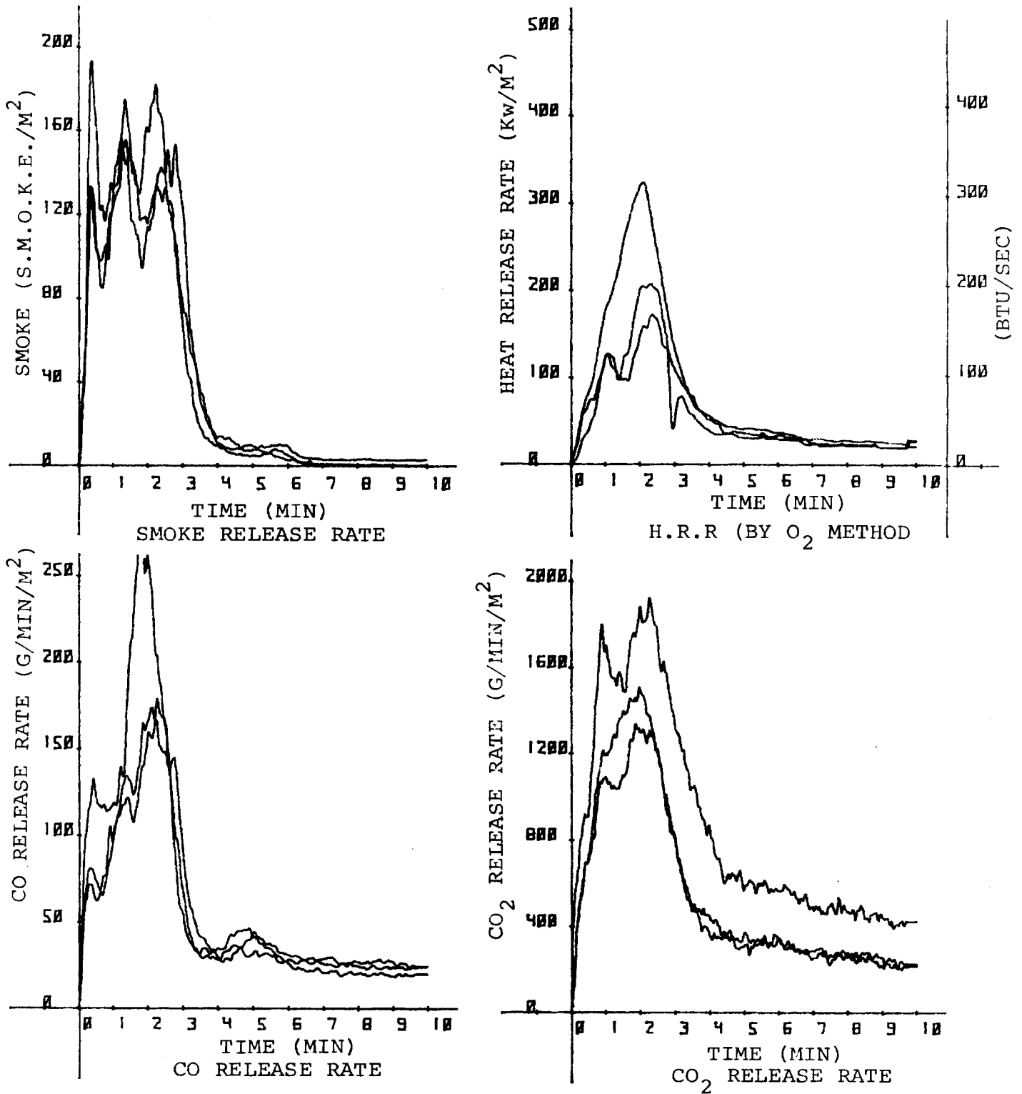
FIGURE 23. CHAS REPRODUCIBILITY OF HAZARDS RELEASE RATES-- POPLAR WOOD FACED PANEL NO. 3, 3 TESTS AT 4.41 Btu/ft 2 SEC (5 W/cm 2 ) (Sheet 2 of 2)
