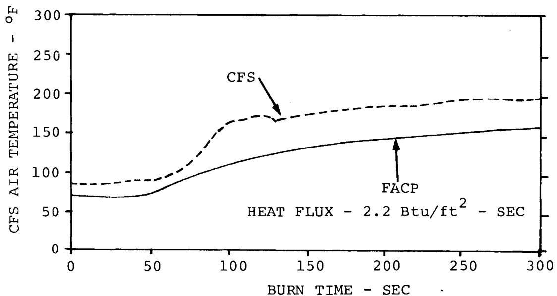
FIGURE 45. COMPARISON OF CFS EXHAUST TEMPERATURES PREDICTED BY THE SINGLE ZONE FACP WITH DIRECT TC MEASUREMENTS PANEL 4 TESTED AT 3 HEAT FLUXES
