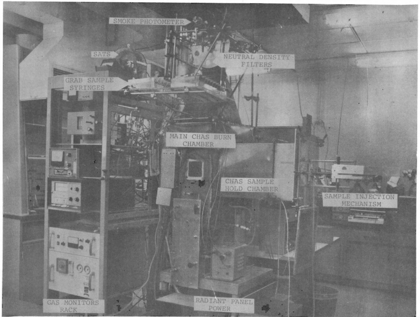
FIGURE 3. THE COMBINED HAZARDS ANALYSIS/SINGLE ANIMAL TEST SYSTEMS-CHAS/SATS
