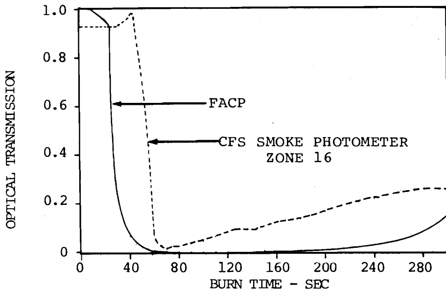
FIGURE 50. COMPARISON OF SMOKE EVOLUTION PROFILES - SINGLE ZONE FACP PREDICTION WITH CFS EXHAUST READINGS FOR PANEL 4 AT 4.41 Btu/ft 2 SEC
