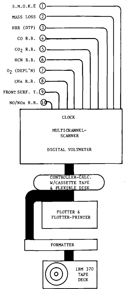
SCHEMATIC DIAGRAM OF THE CHAS/SATS
