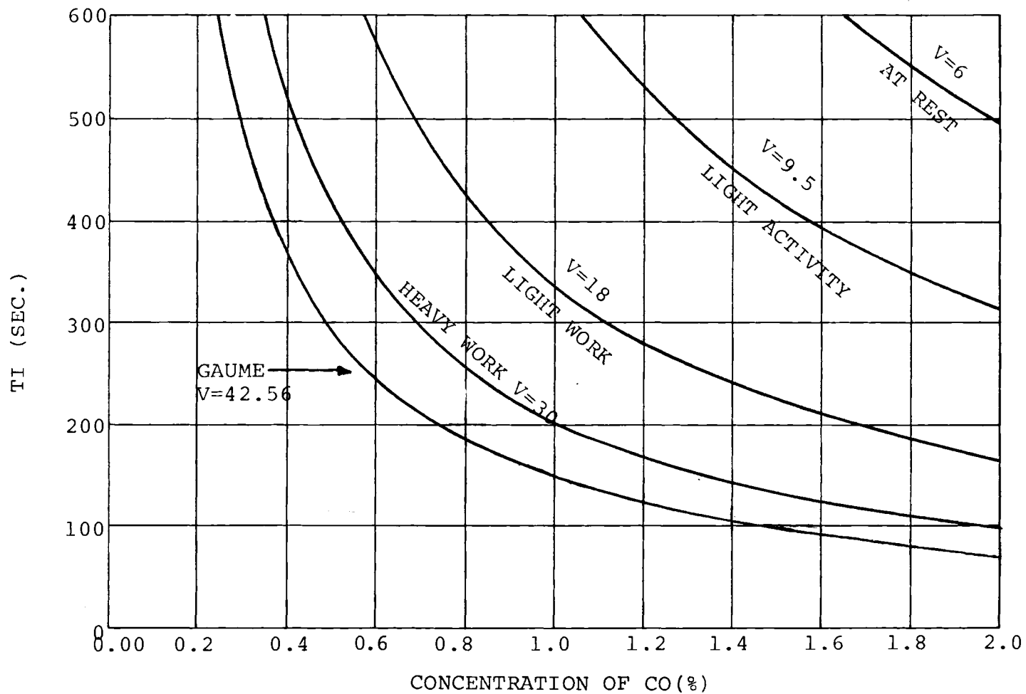
FIGURE 13. COMPARISON OF CHI HAZARD LIMIT CURVE WITH LITERATURE DATA
