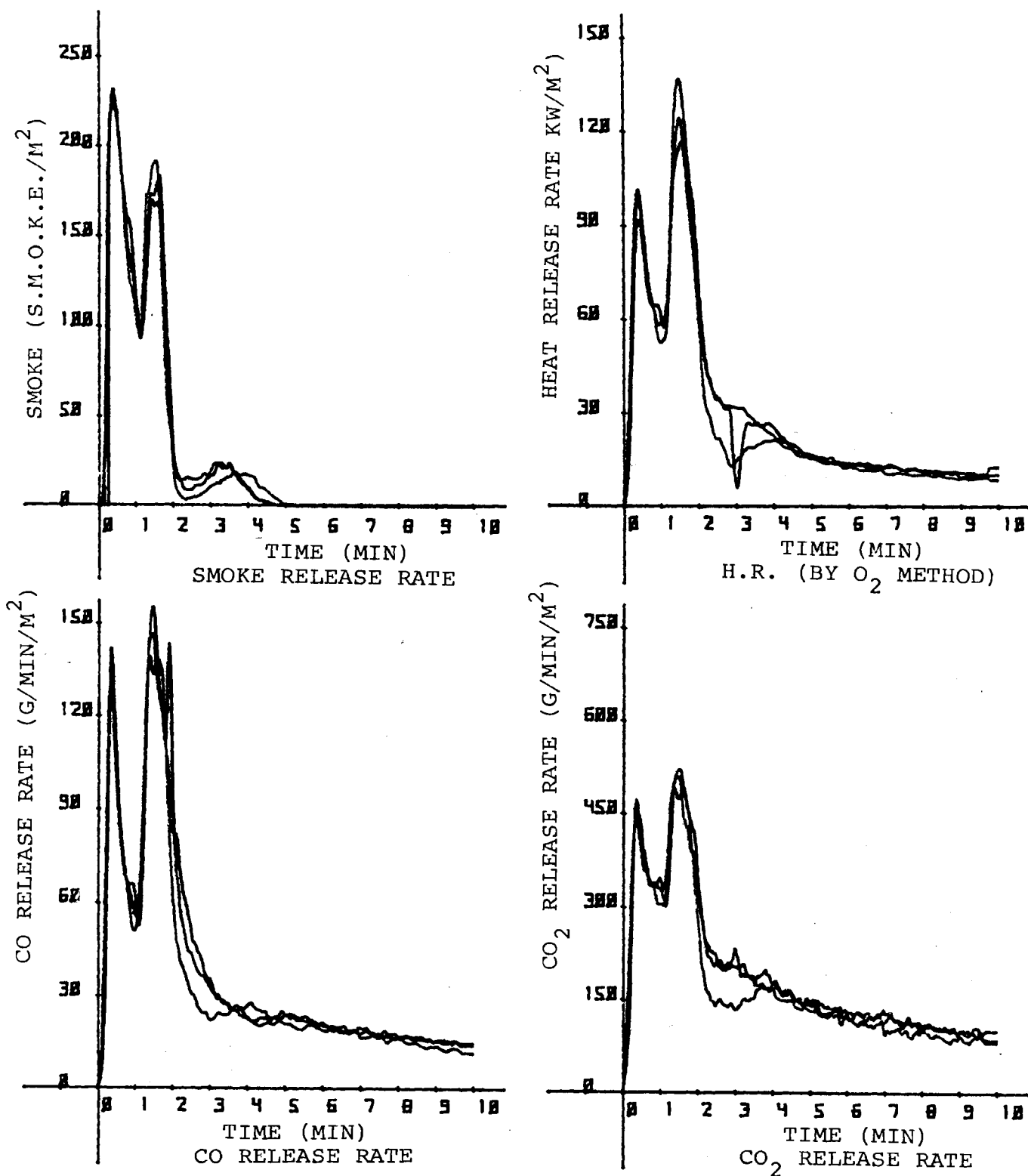
FIGURE 24. CHAS REPRODUCIBILITY OF HAZARDS RELEASE RATE-- PARTITION PANEL NO. 4, 3 TESTS AT 4.41 Btu/ft 2 SEC (5 W/cm 2 ) (Sheet 1 of 2)
