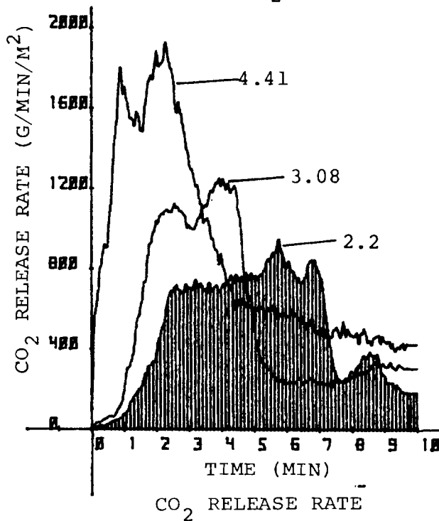
FIGURE 33. CHAS HAZARDS RELEASE RATES COMPARISON OF POPLAR WOOD FACED PANEL NO. 3 TESTED AT 3 HEAT FLUXES-- 2.2, 3.08, & 4.41 BTU/FT 2 SEC (2.5, 3.5, 5 W/CM 2 (Sheet 1 of 3)
