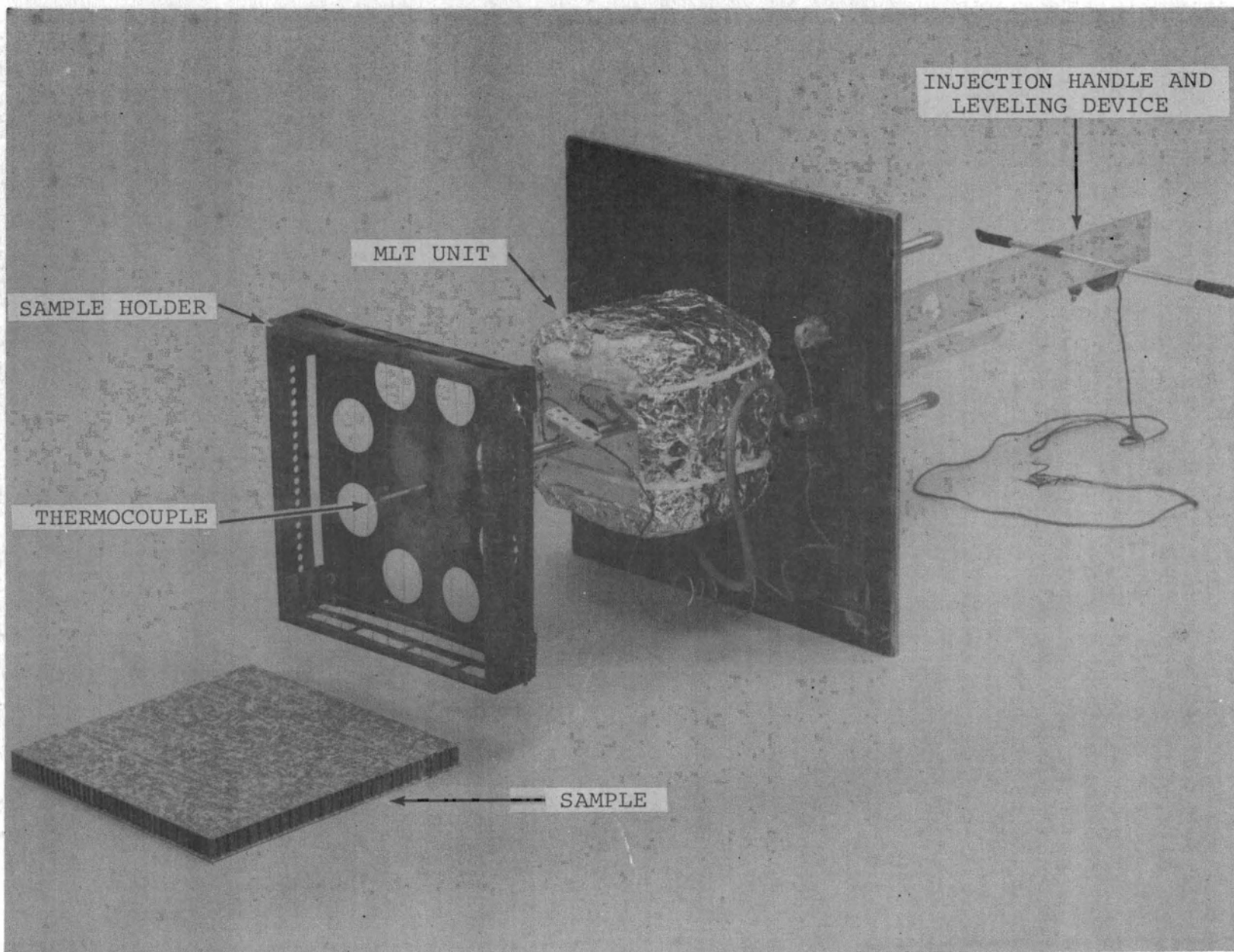
FIGURE 5. SAMPLE HOLDERS AND INJECTION MECHANISM (WITH MLT UNIT)
