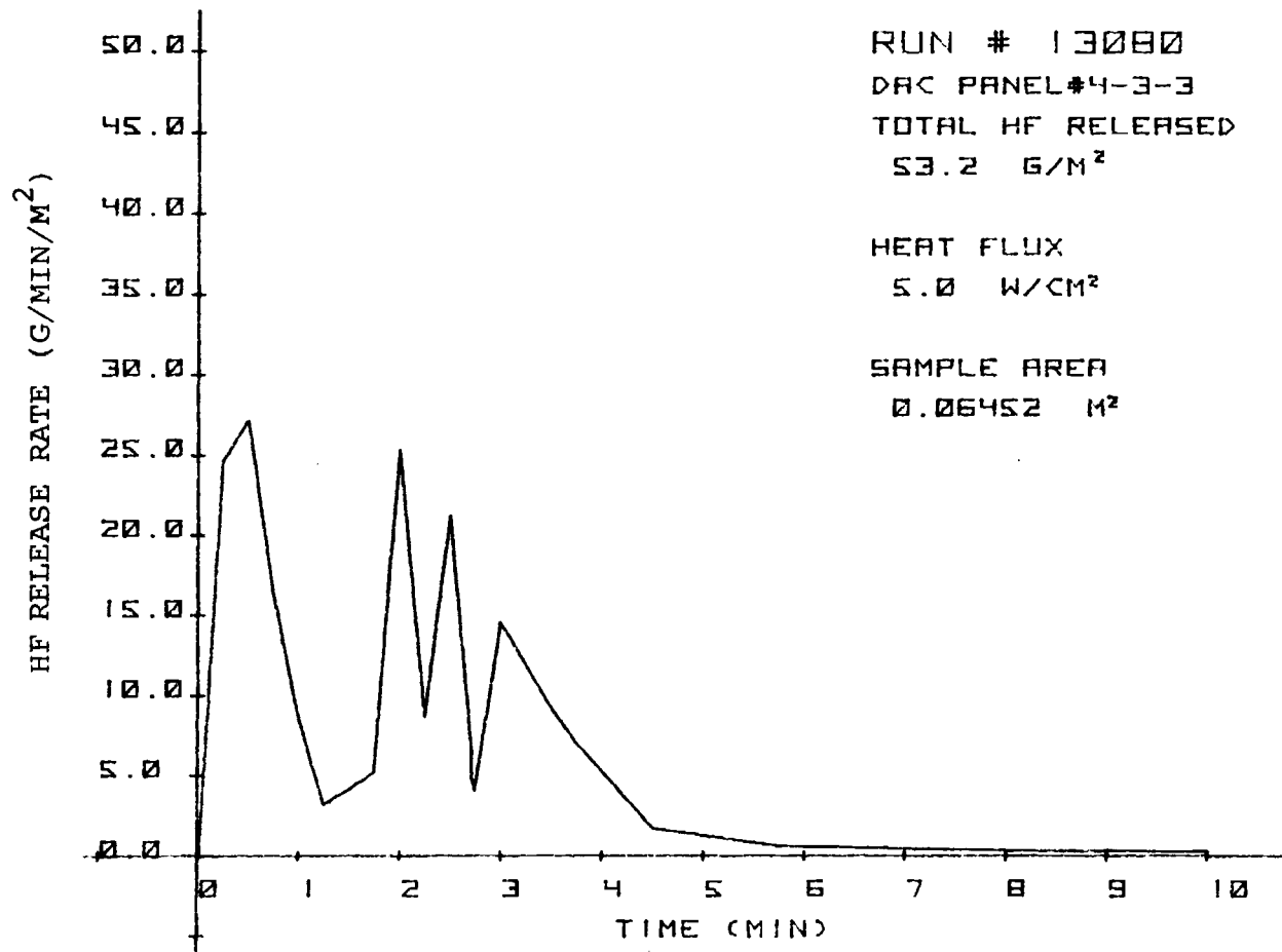
FIGURE 31. HYDROGEN FLUORIDE RELEASE RATE COMPOSITED FROM PANEL 4 TESTS (FIGURE 30)
