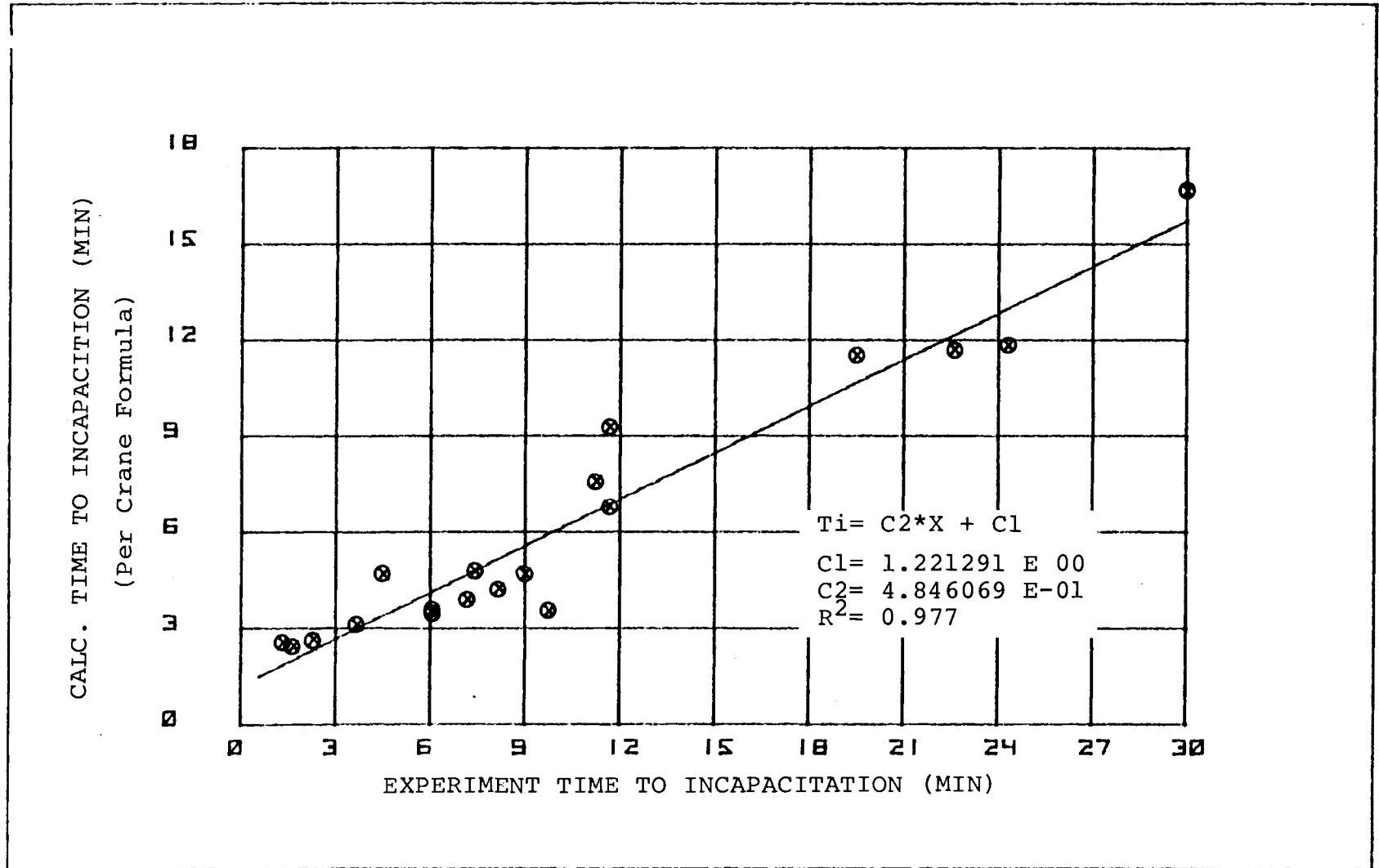
FIGURE 39. GROUPED DATA FOR PANELS 2,3 and 4--COMPARISON OF CALCULATED AND OBSERVED T_i VALUES
