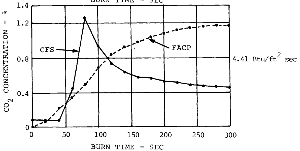
FIGURE 46. COMPARISON PLOTS OF CFS EXHAUST CO 2 CONCENTRATIONS WITH FACP RESULTS - PANEL 4 AT 3 HEAT FLUX TEST LEVELS
