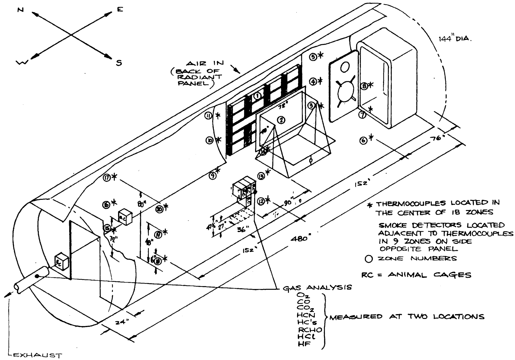
FIGURE 1. CHI TEST SETUP IN CFS
