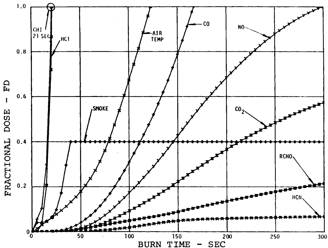
FIGURE 72. TWENTY ZONE FACP CHI AND FRACTIONAL DOSE PLOTS PANEL 3 AT 4.41 Btu/ft 2 SEC
