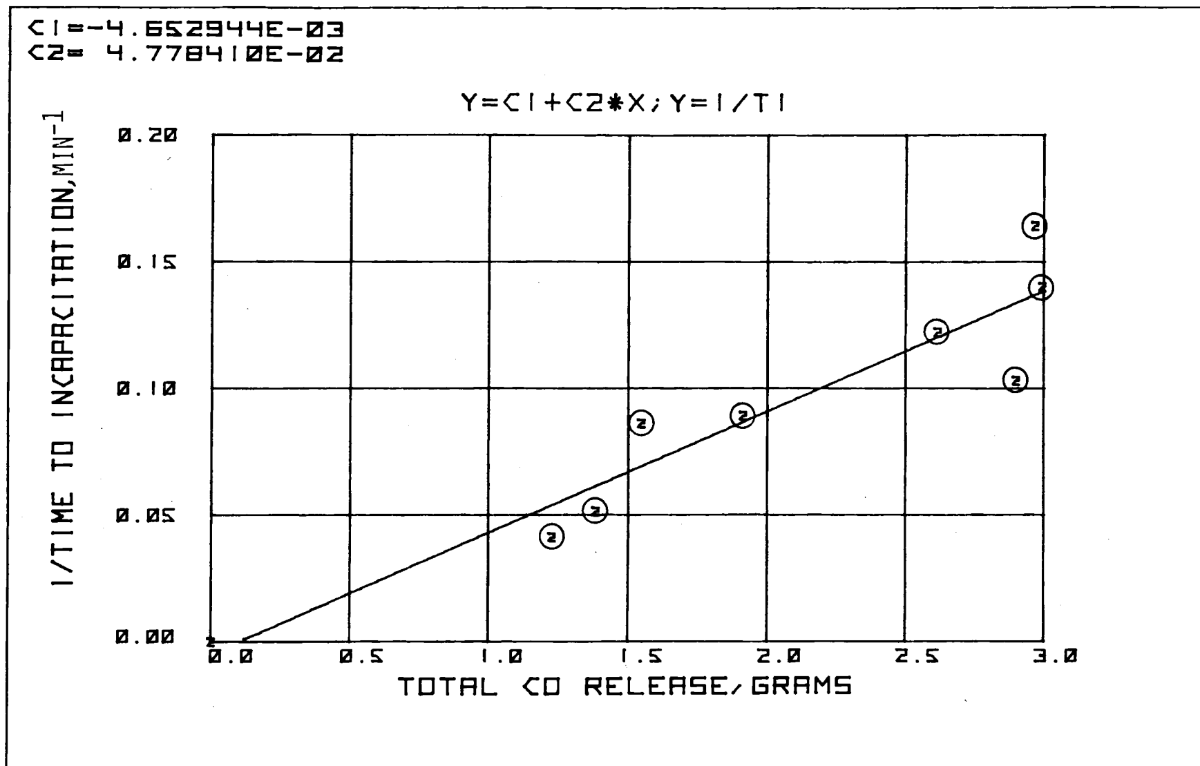
FIGURE 36. CORRELATION OF 1/T_i ( \text{MIN}^{-1} ) VALUES WITH PANEL 2 CHAS/SATS CO YIELDS
