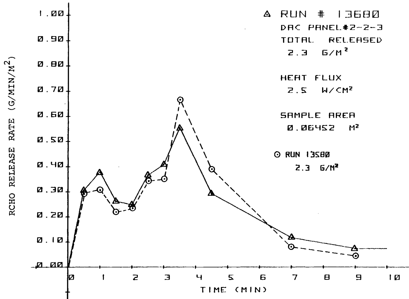
FIGURE 25. COMPARISON OF ALIPHATIC ALDEHYDE RELEASE RATES FOR TWO TESTS OF PANEL 2 AT 2.2 Btu/ft 2 SEC (SAMPLED AT SAME TIME INTERVALS)
