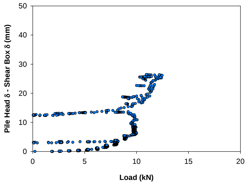
Figure 58. Relative displacement for glacial till (Pile 5)
