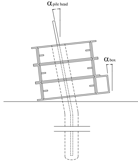
(b) elevation view (tilt)
