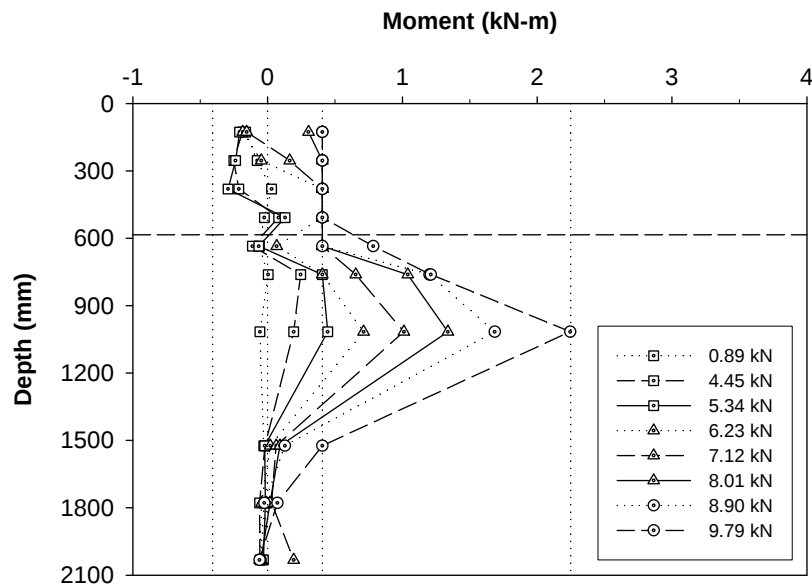
Figure 92. Bending moment profiles for reinforced glacial till (Pile 5)
