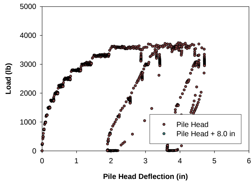
Figure C 29. Pile head deflection for glacial till (Pile 14 B)
