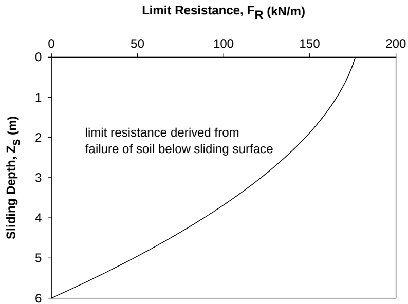
(b) Limit anchorage resistance curve
