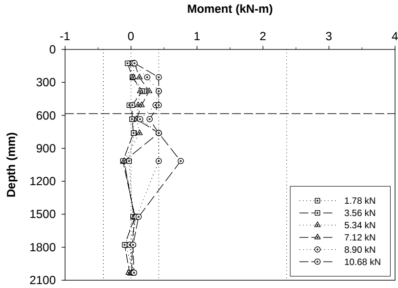
Figure 99. Bending moment profiles for reinforced glacial till (Pile 13 A)
