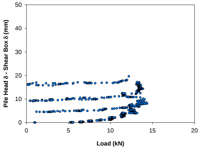
Figure 64. Relative displacement for glacial till (Pile 9)
