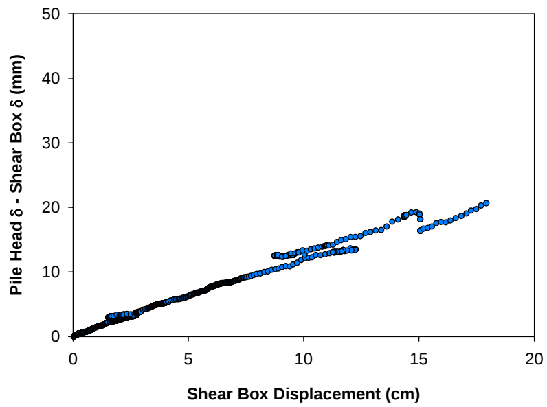
Figure 59. Relative displacement for glacial till (Pile 5)
