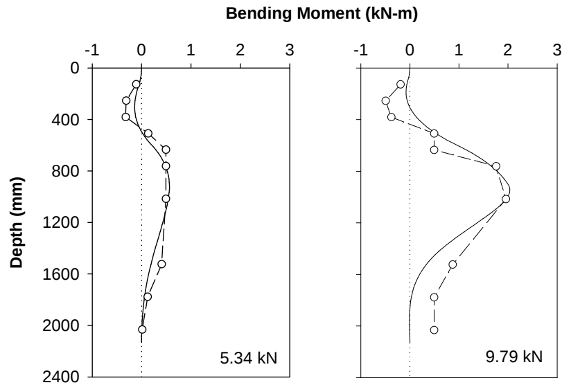
Figure 130. Sample bending moment correlation for isolated pile in weathered shale (Pile 6)
