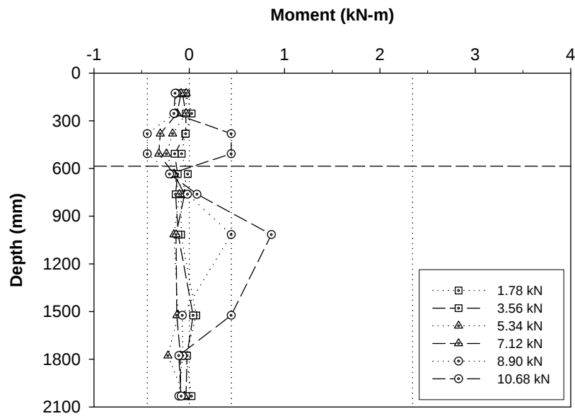
Figure 100. Bending moment profiles for reinforced glacial till (Pile 13 B)
