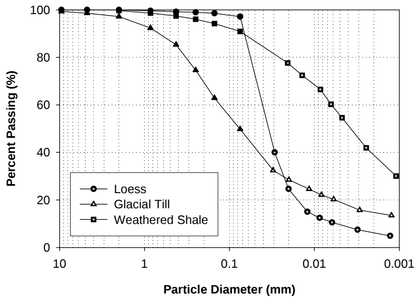
Figure 16. Grain size distribution curve
