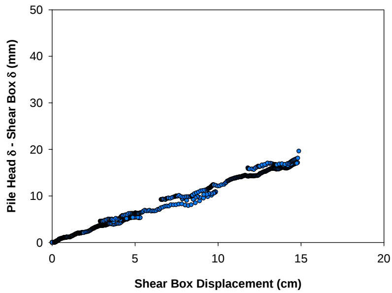
Figure 65. Relative displacement for glacial till (Pile 9)
