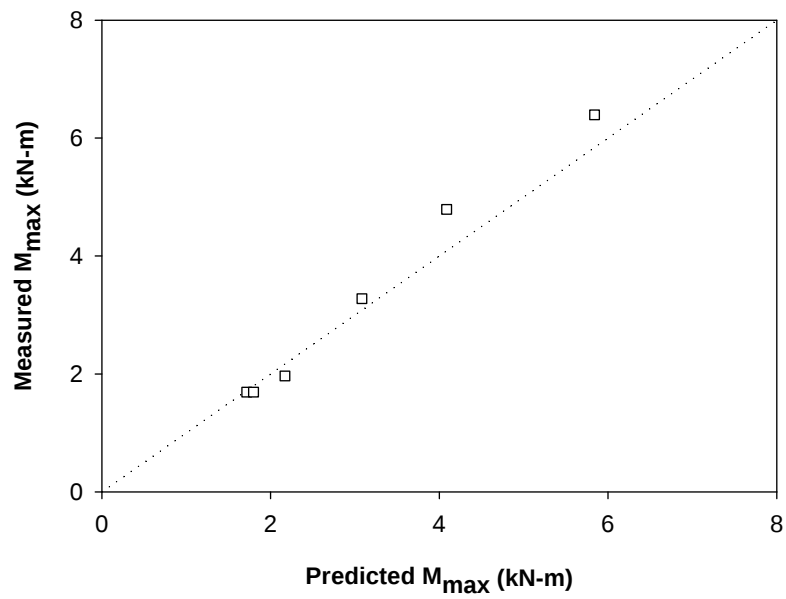
Figure H 11. Maximum moment correlation in glacial till (Pile 12)
