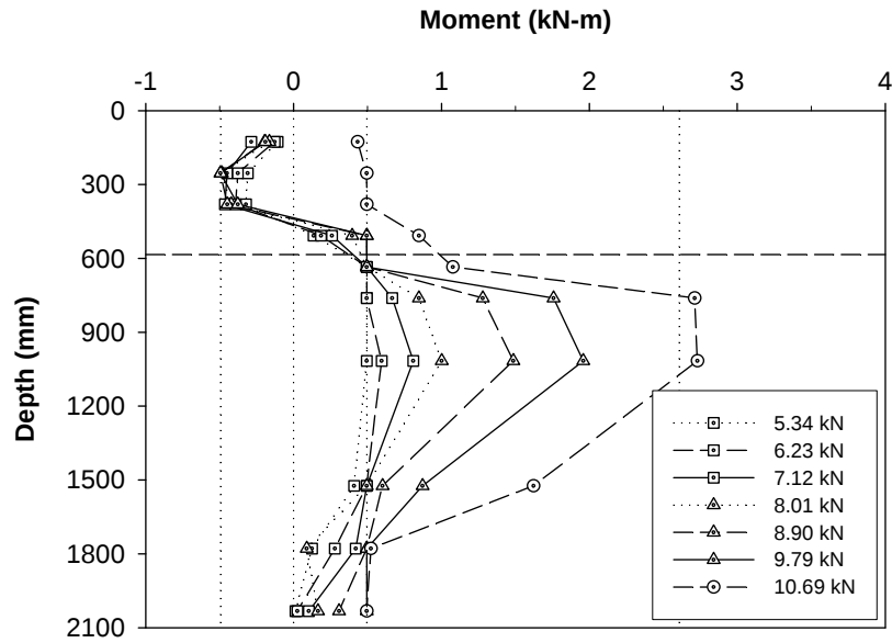
Figure 93. Bending moment profiles for reinforced weathered shale (Pile 6)
