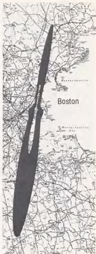
The noise "footprint" of a DC-8 over Boston. The area exposed to 90EPNdB (effective perceived noise decibels) with its earlier engine (black outline) is contrasted with the area affected by the plane with a new, quieter engine installed in response to the FAR (white outline).
