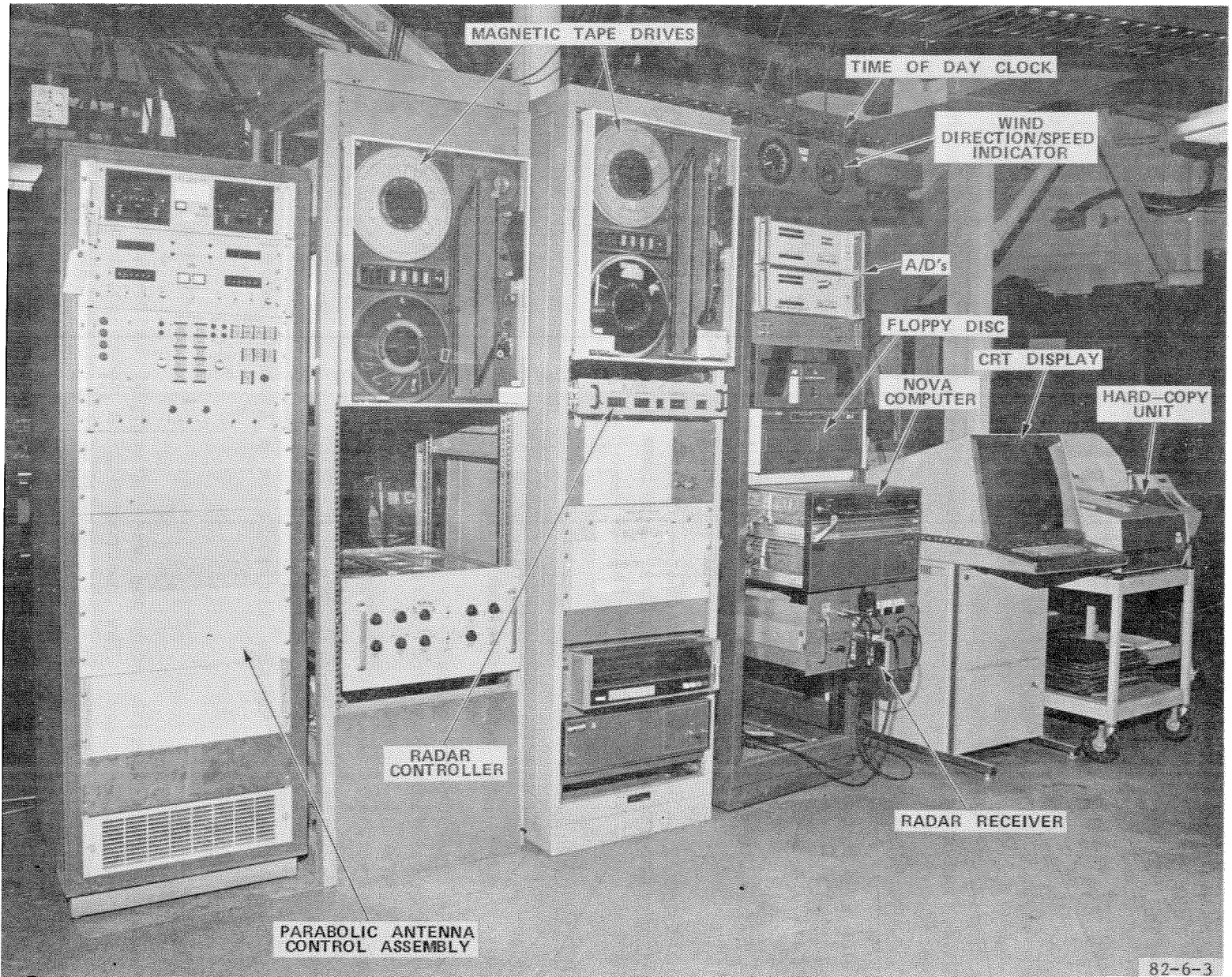
FIGURE 3. TURBULENCE TEST BED RECORDING AND CONTROL EQUIPMENT
