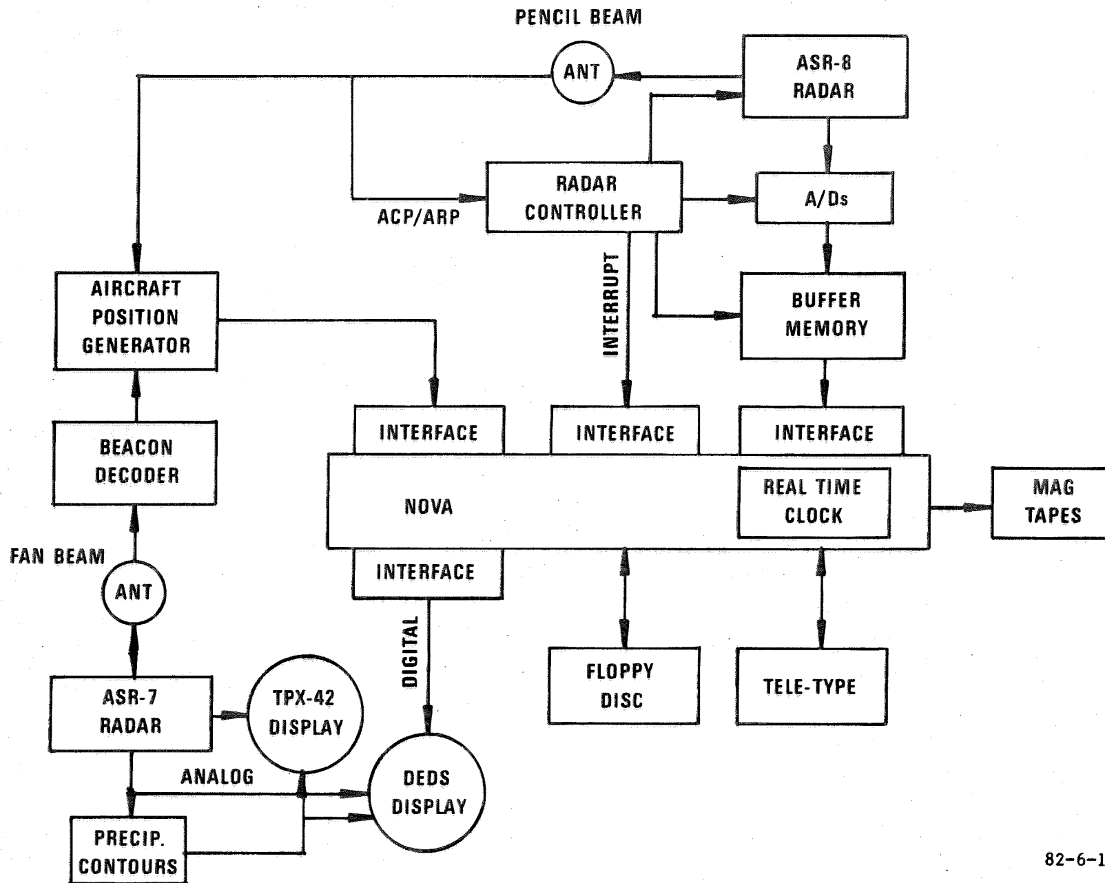
FIGURE 1. TURBULENCE MEASUREMENT SYSTEM
