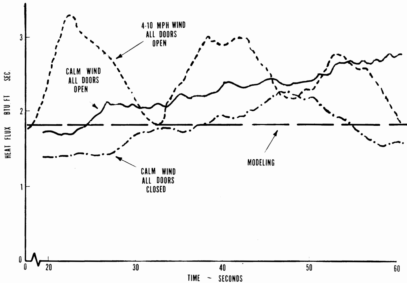
FIGURE 5. DC7 SYMMETRY PLANE HEAT FLUX
