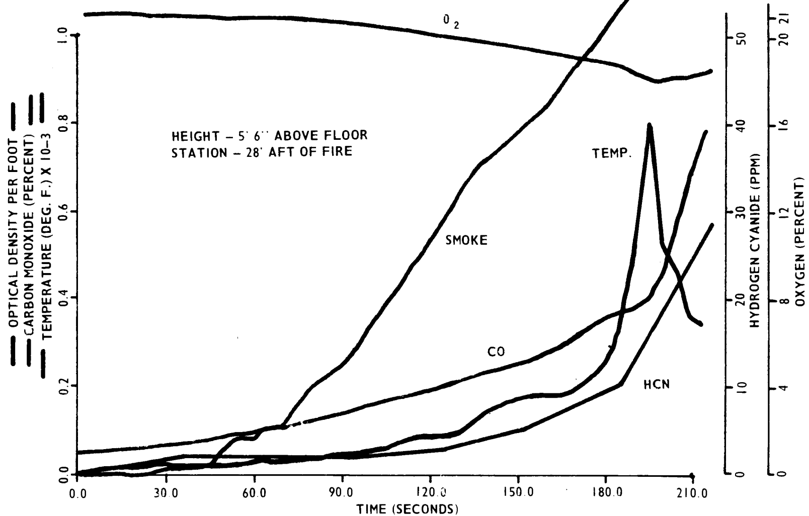
FIGURE 7. C-133 HAZARD LEVELS WITH CABIN MATERIALS TEST 12/12/79
