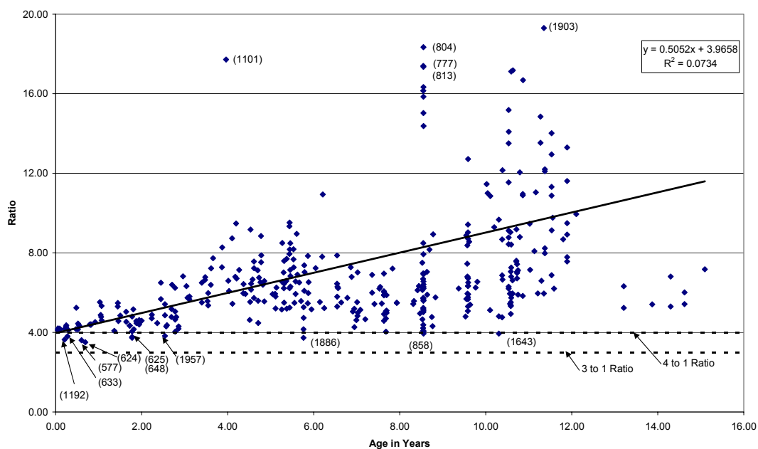
Figure 4-26: Red/White ASTM Type III Ratio versus Age for Unwiped Signs Excluding the Crawfordsville Bonepile (cropped) (n = 422)
