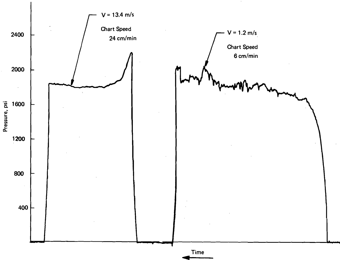
FIGURE 8. PRESSURE-TIME TRACE FOR FLOW OF AMK THROUGH 10- \mu m SCREEN ( A = 0.184 \text{ cm}^2 )
