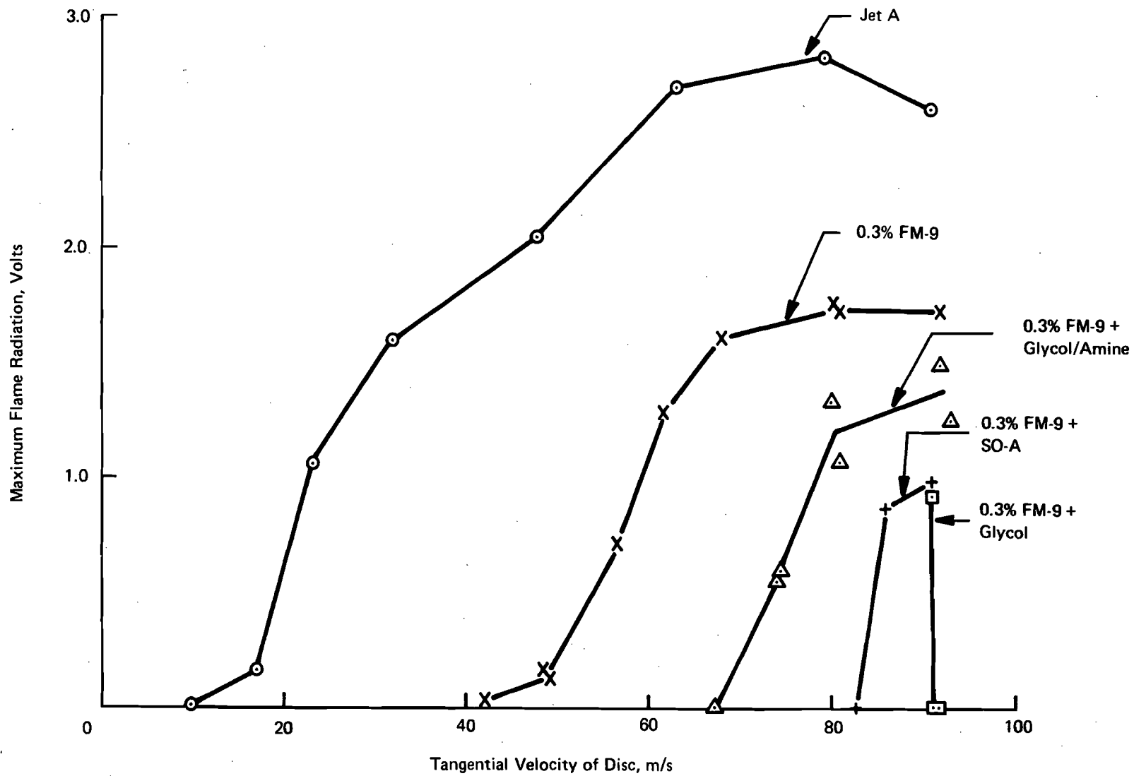
FIGURE 3. EFFECT OF CARRIER FLUID COMPONENTS AND SO-A ON MIST FLAMMABILITY OF FM-9 IN JET A - FUEL FLOW = 2.8 l/min.
