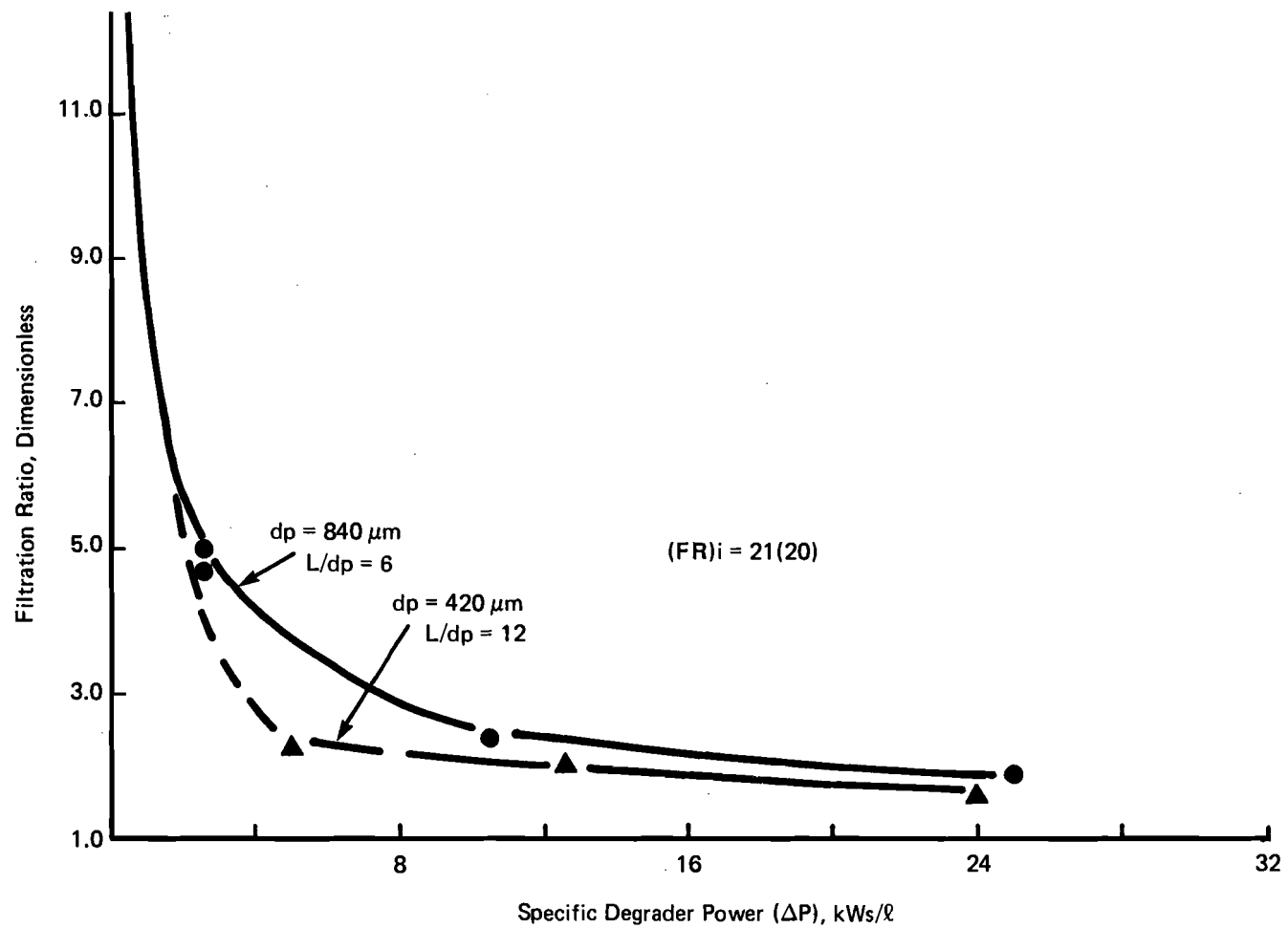
FIGURE 22. EFFECT OF SPECIFIC DEGRADER POWER ON THE FILTRATION RATIO OF AMK WITHOUT AMINE
