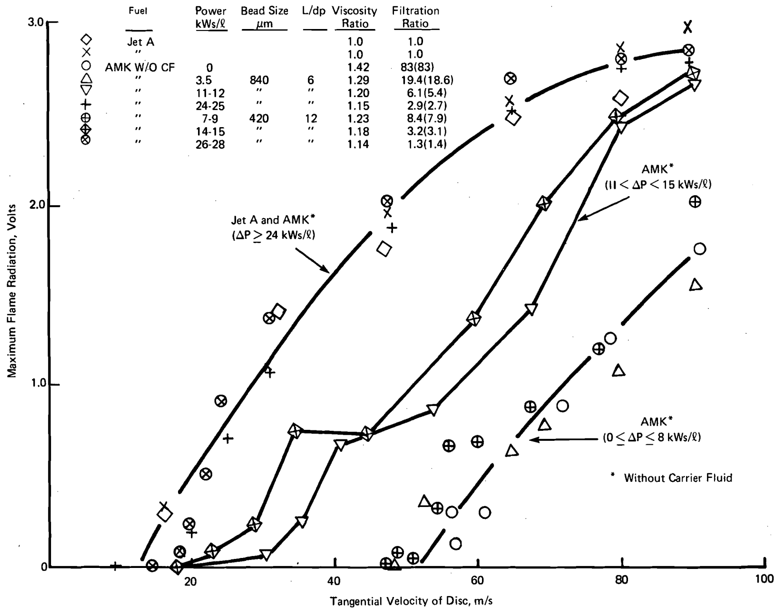
FIGURE 21. EFFECT OF SPECIFIC DEGRADER POWER AND BEAD SIZE ON MIST FLAMMABILITY OF AMK WITHOUT CARRIER FLUID
