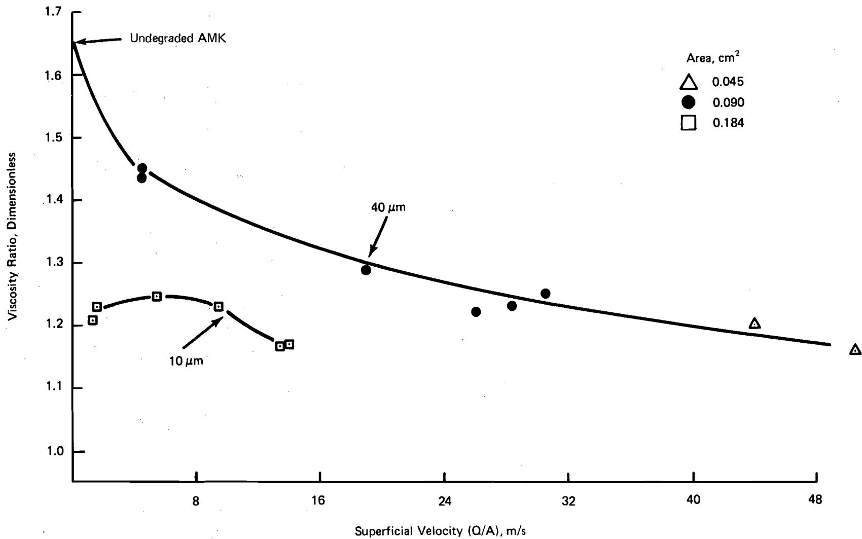
FIGURE 9. EFFECT OF SUPERFICIAL VELOCITY THROUGH METAL SCREENS ON THE VISCOSITY RATIO
