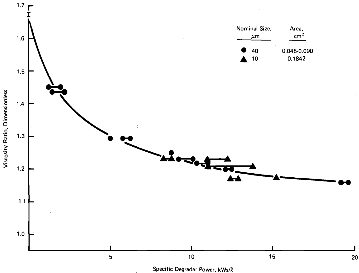
FIGURE 10. EFFECT OF SPECIFIC DEGRADER POWER THROUGH METAL SCREENS ON THE VISCOSITY RATIO
