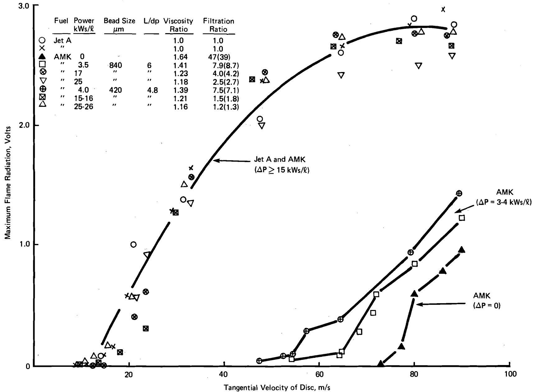
FIGURE 19. EFFECT OF SPECIFIC DEGRADER POWER AND BEAD SIZE ON MIST FLAMMABILITY OF AMK BLENDED BY ICI AMERICAS, INC.
