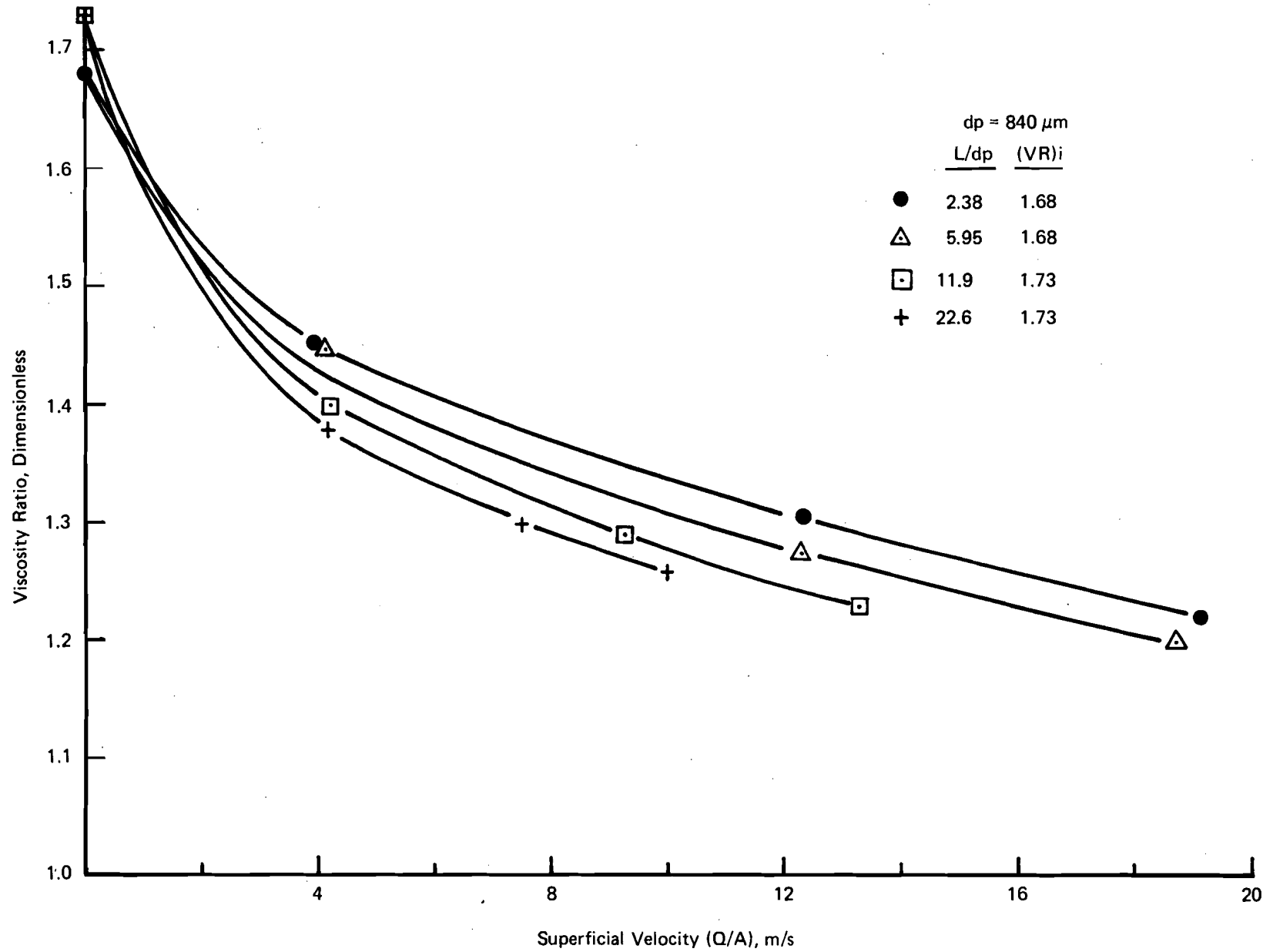
FIGURE 13. EFFECT OF TUBE LENGTH AND SUPERFICIAL VELOCITY ON THE VISCOSITY RATIO
