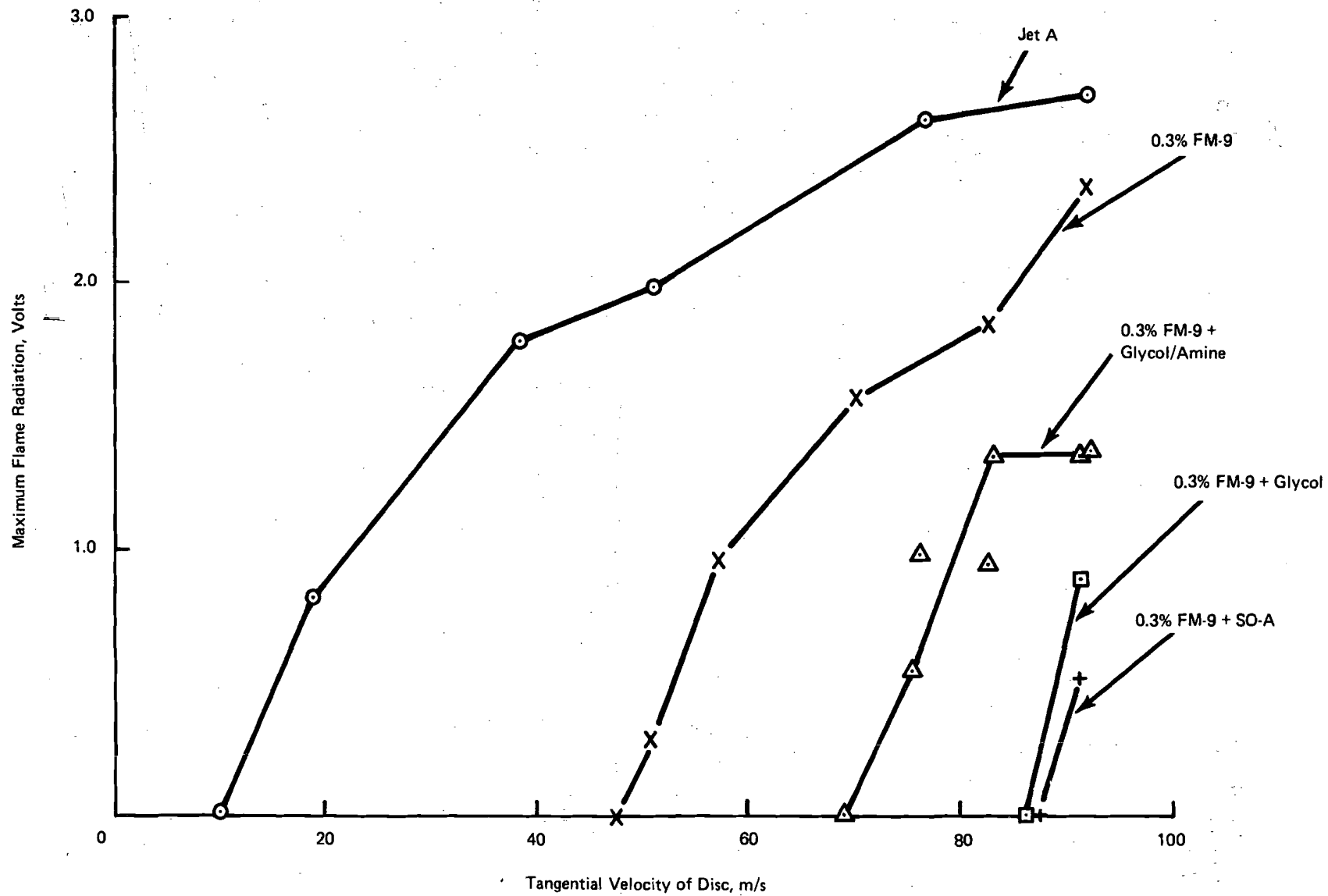
FIGURE 2. EFFECT OF CARRIER FLUID COMPONENTS AND SO-A ON MIST FLAMMABILITY OF FM-9 IN JET A - FUEL FLOW = 2.0 l/min.
