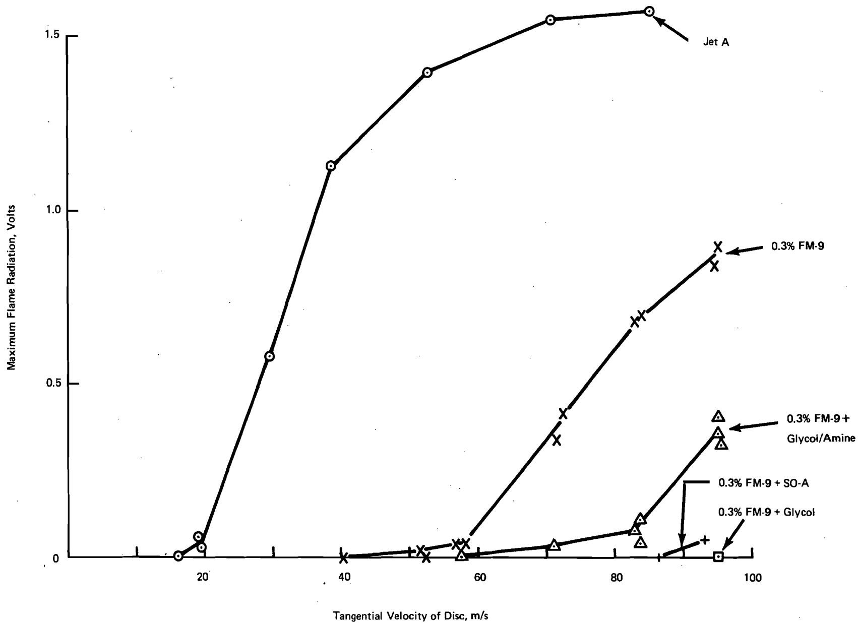
FIGURE 1. EFFECT OF CARRIER FLUID COMPONENTS AND SO-A ON MIST FLAMMABILITY OF FM-9 IN JET A - FUEL FLOW = 1.0 l/min.
