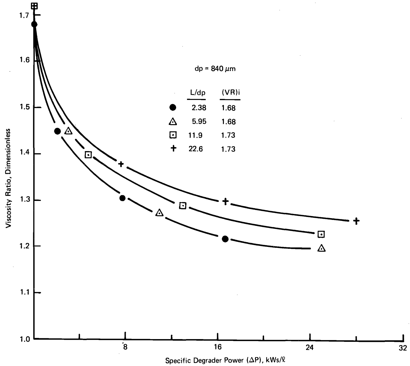
FIGURE 14. EFFECT OF TUBE LENGTH AND SPECIFIC DEGRADER POWER ON THE VISCOSITY RATIO
