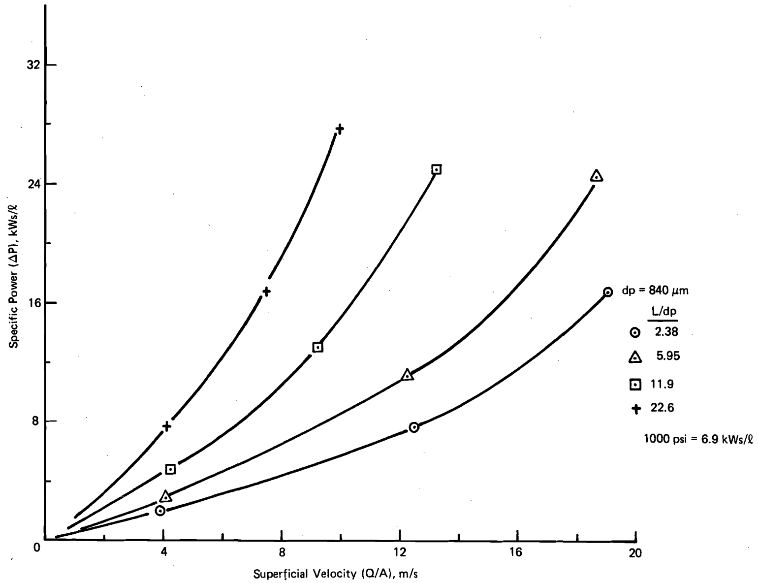
FIGURE 12. FLOW OF AMK THROUGH DIFFERENT LENGTH PACKED TUBES
