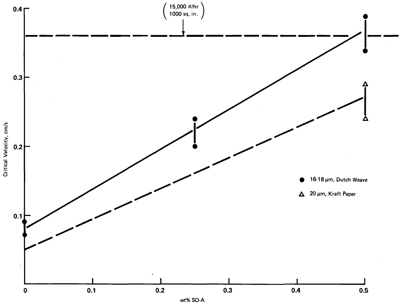
FIGURE 29. EFFECT OF SURFACTANT ON THE CRITICAL FILTRATION VELOCITY OF UNDEGRADED AMK
