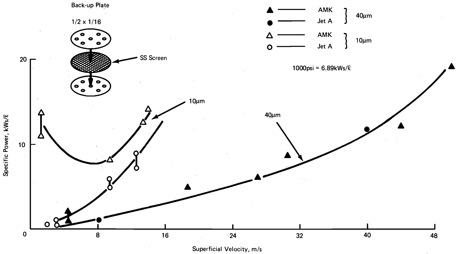
FIGURE 6. FLOW OF AMK THROUGH METAL SCREENS
