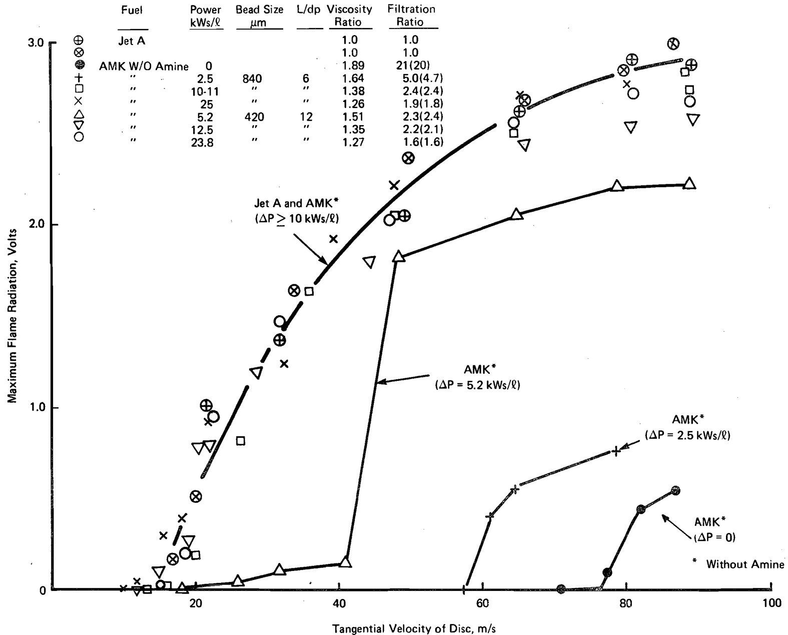
FIGURE 23. EFFECT OF SPECIFIC DEGRADER POWER AND BEAD SIZE ON MIST FLAMMABILITY OF AMK WITHOUT AMINE
