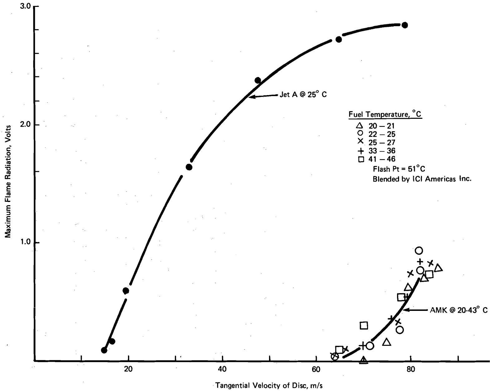
FIGURE 5. EFFECT OF TEMPERATURE ON MIST FLAMMABILITY OF AMK
