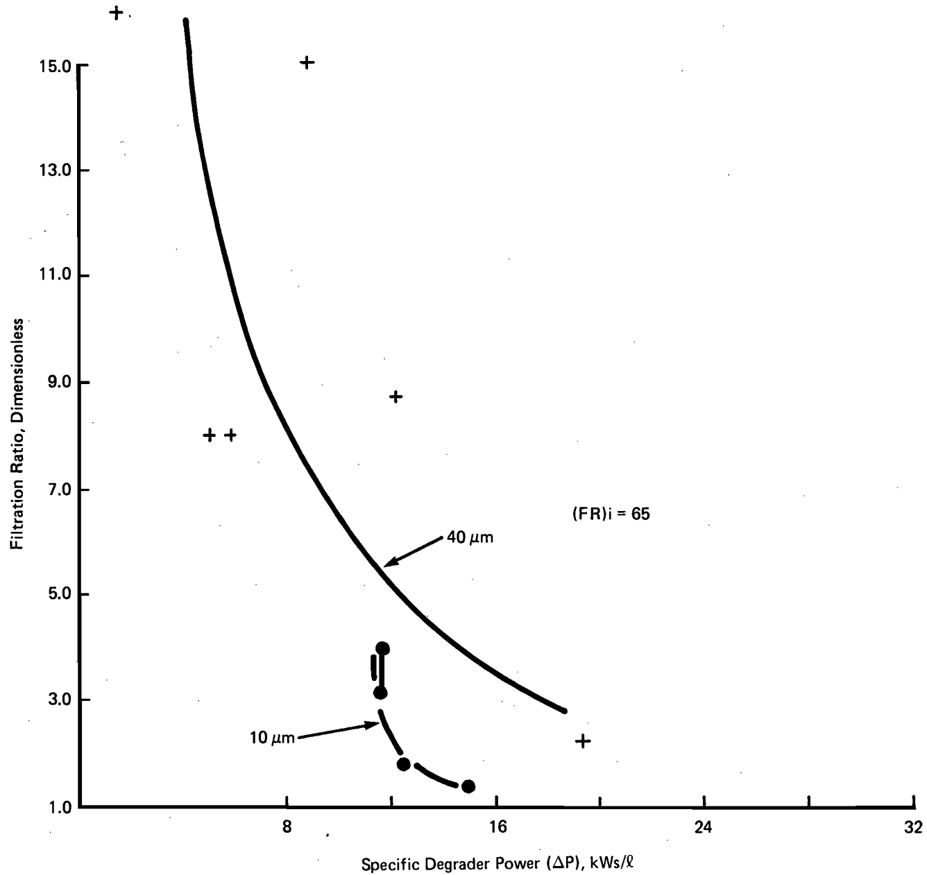
FIGURE 11. EFFECT OF SPECIFIC DEGRADER POWER THROUGH METAL SCREENS ON THE FILTRATION RATIO
