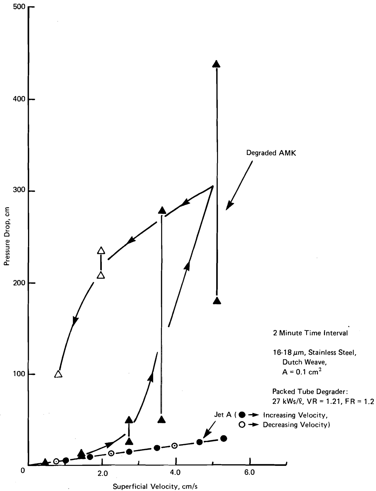
FIGURE 27. EFFECT OF SUPERFICIAL VELOCITY ON PRESSURE DROP ACROSS FILTER WITH JET A AND DEGRADED AMK
