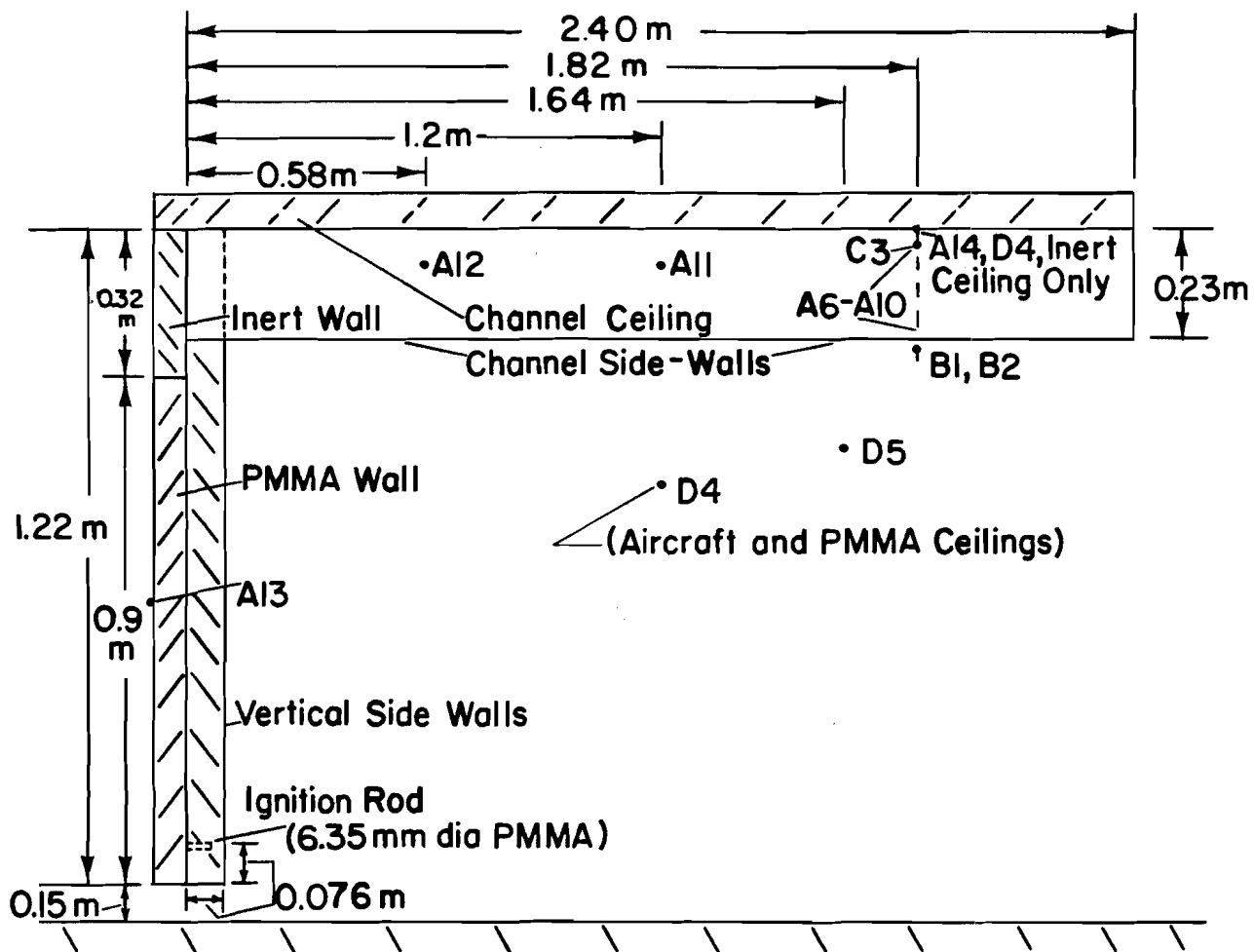
FIGURE 1 SIDE VIEW OF CHANNEL
