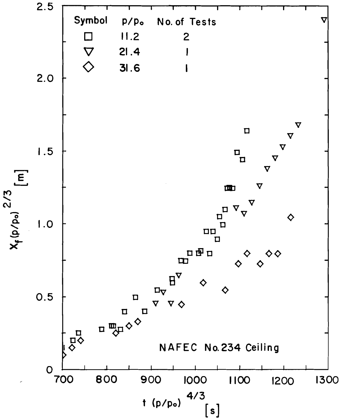
FIGURE 5 CORRELATION OF FLAME LENGTH UNDER NO. 234 MODEL CEILING
