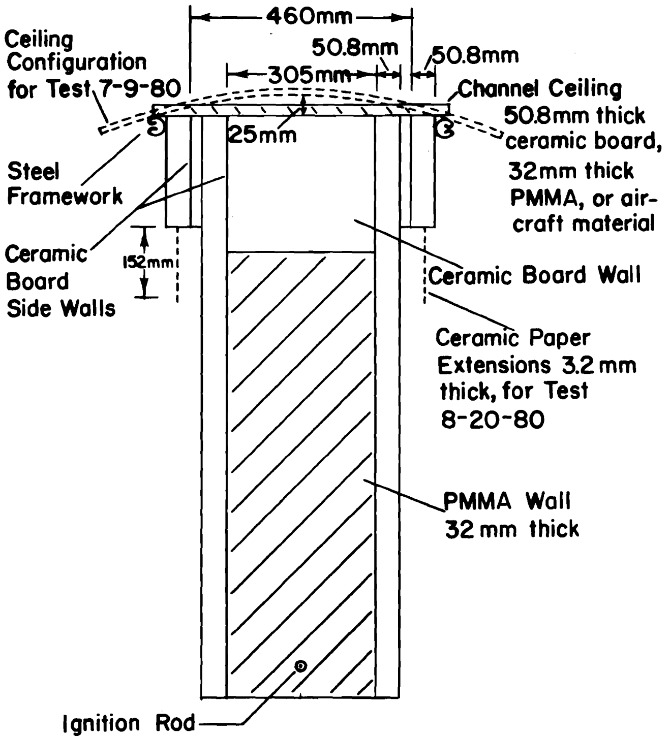
FIGURE 2 END VIEW OF CHANNEL
