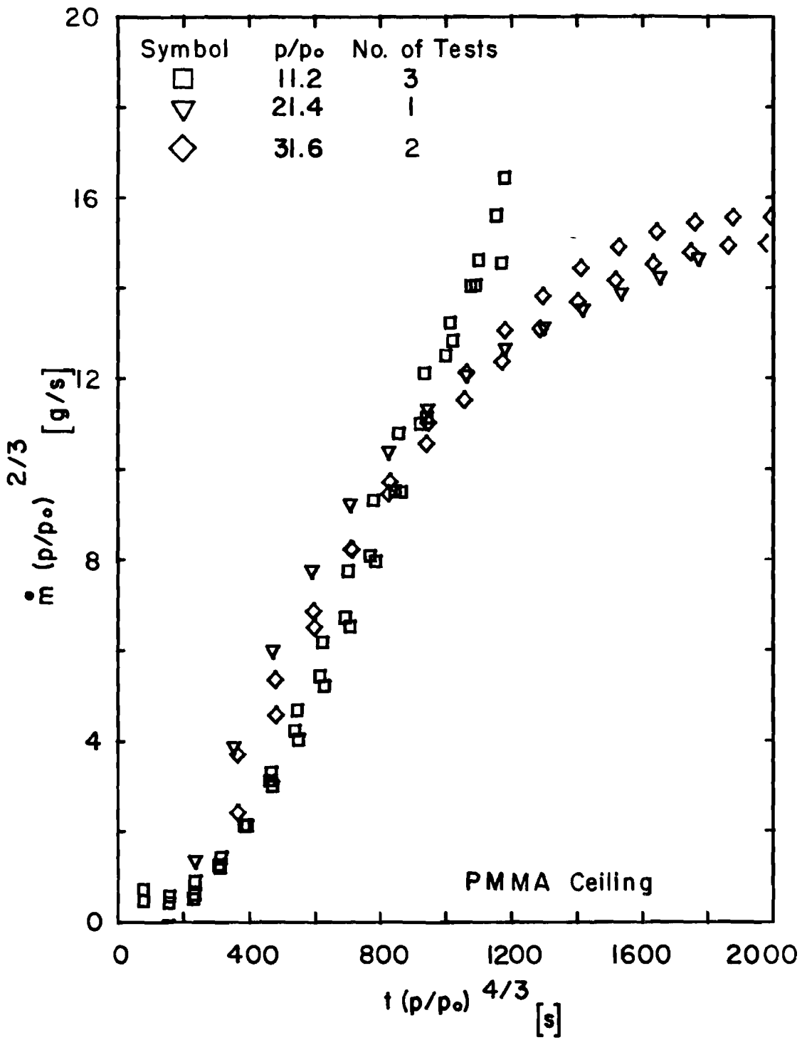
FIGURE 18 CORRELATION OF MASS LOSS RATE FOR PMMA MODEL CEILING
