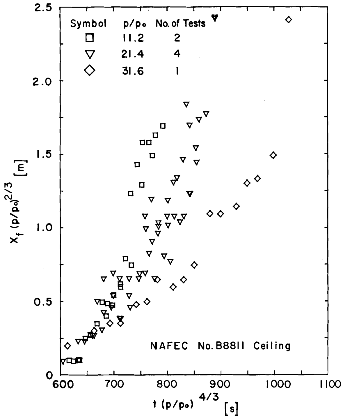
FIGURE 6 CORRELATION OF FLAME LENGTH UNDER NO. B8811 MODEL CELLINGS
