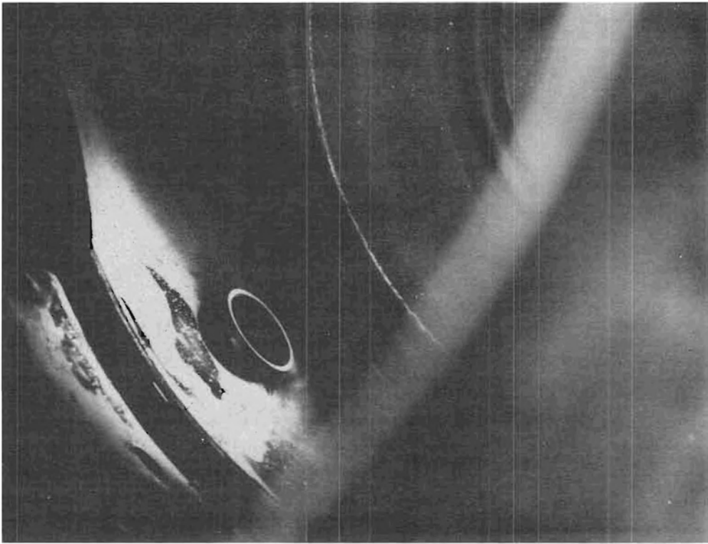
Figure 61 Post Test Photograph of B/M Combustor Can
