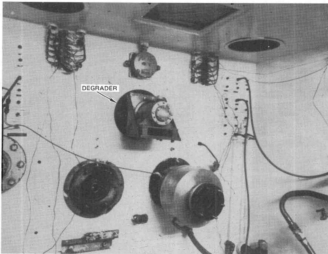
Figure 12 RAE Degradation Mounted On Test Stand
