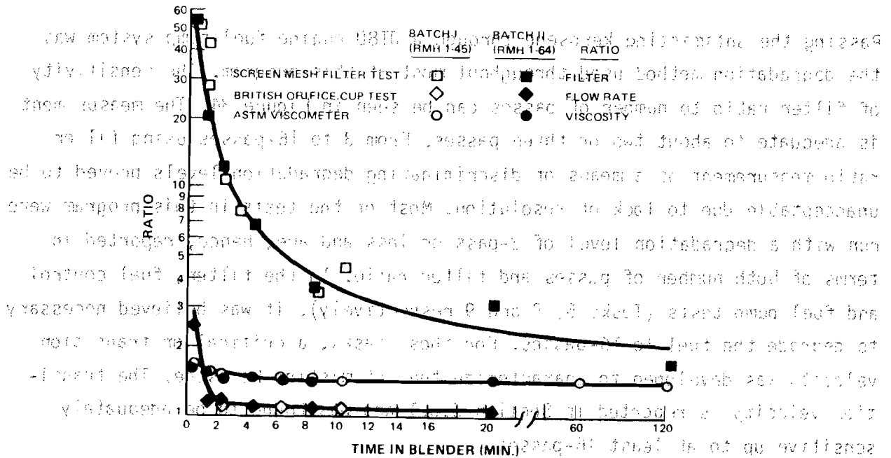
Figure 33 Correlation of Three Viscosity Measuring Device
