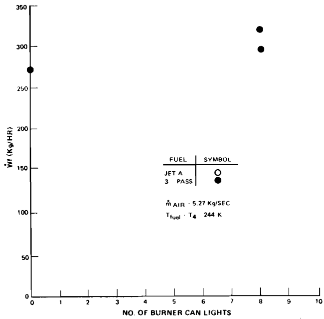
Figure 71 Sea Level Ignition - Low Emissions Combustor
