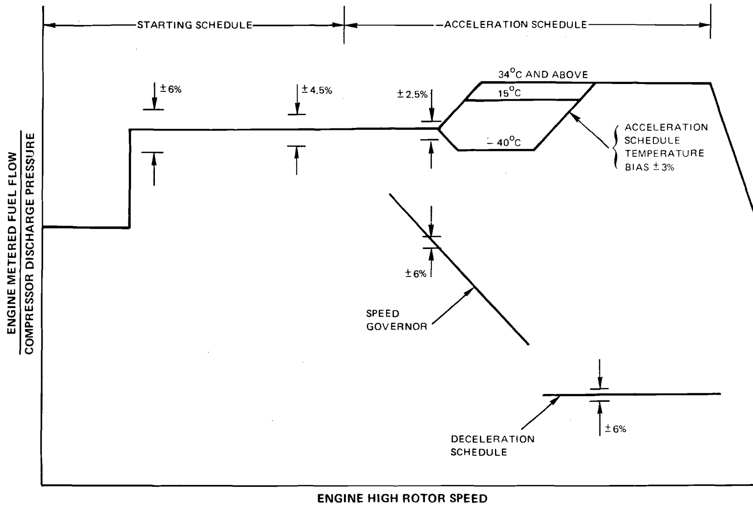
Figure 4 Fuel Control Scheduling Accuracy Requirements
