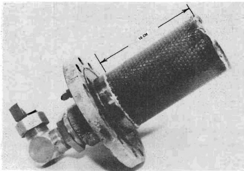
Figure 52 Degrader System Inlet Screen
