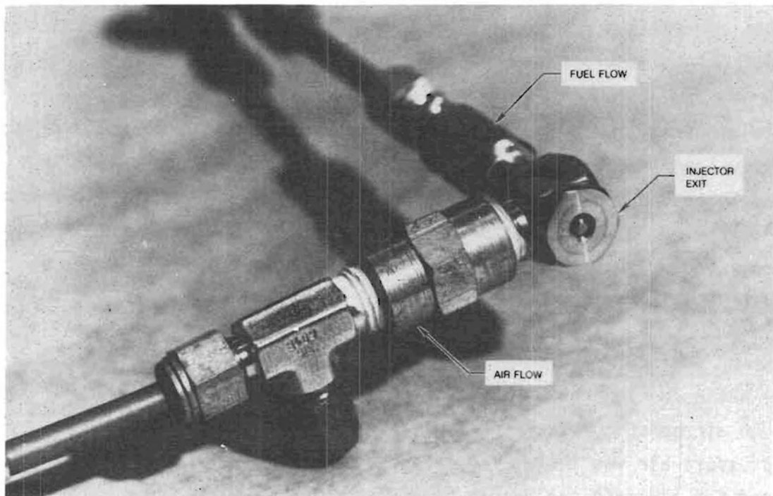
Figure 25 Delavan Air Boost Injector
