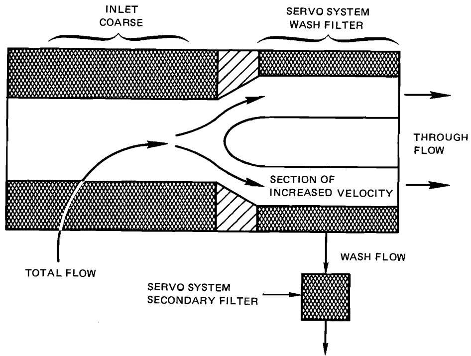
Figure 18 JT8D Fuel Control Filter Assembly
