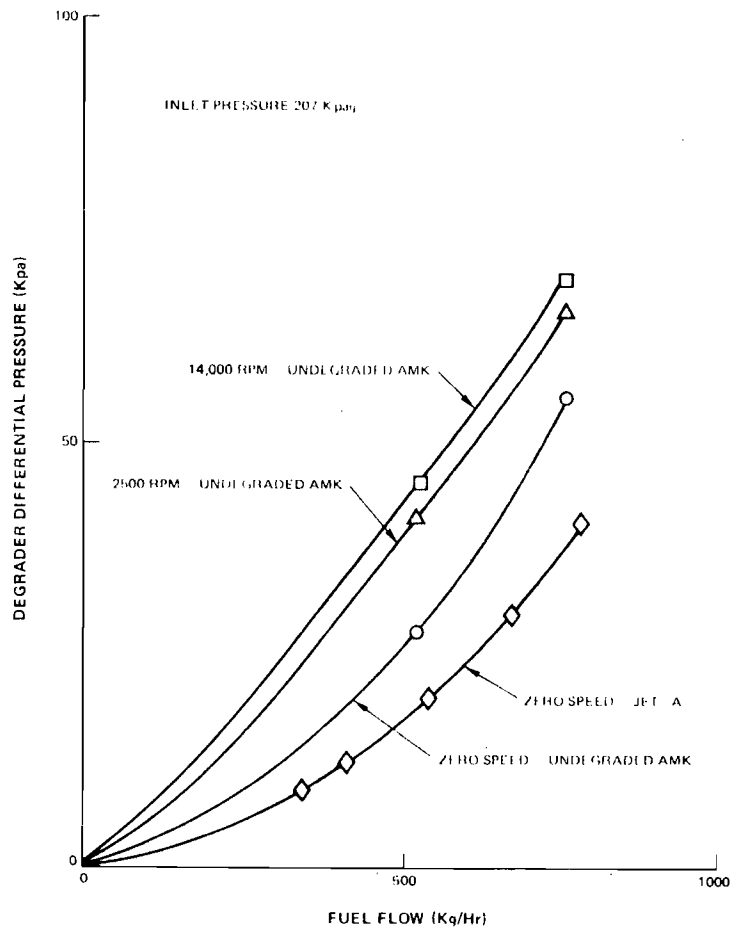
Figure 37 RAE Degradation Flow Characteristics
