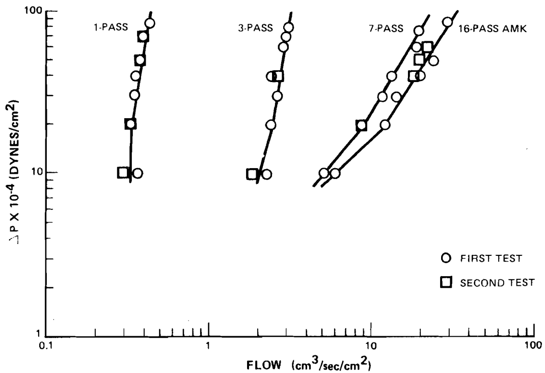
Figure 46 AMK Flow Through 10 μm Metal Screen
