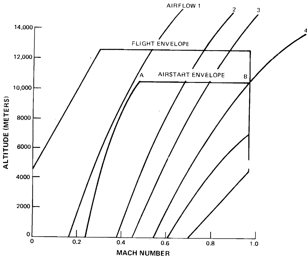
Figure 8 JT8D-17 Airstart Envelope
