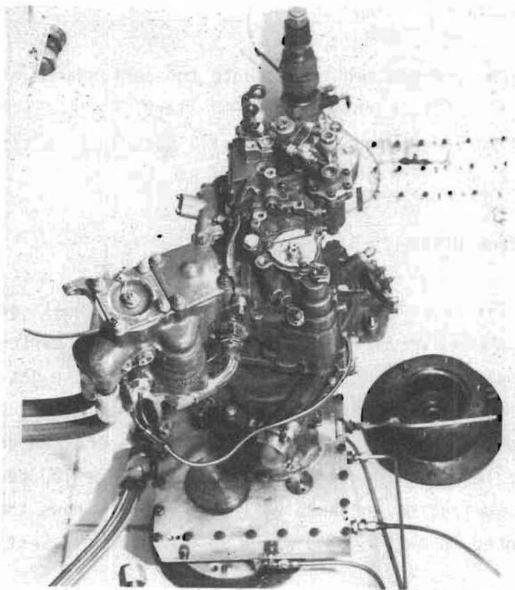
Figure 31 JT8D Engine Fuel Control and Fuel Pump
