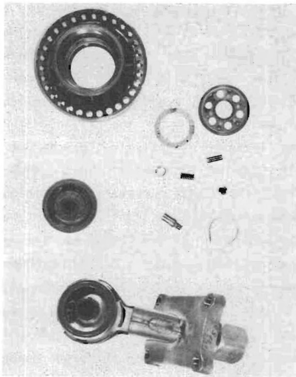
Figure 63 Post Test Disassembly of L/E Nozzle
