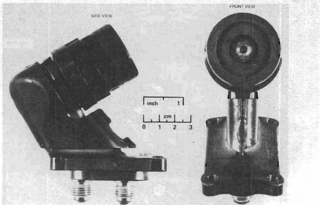
Figure 23 JT8D Bill-of-Material Injector
