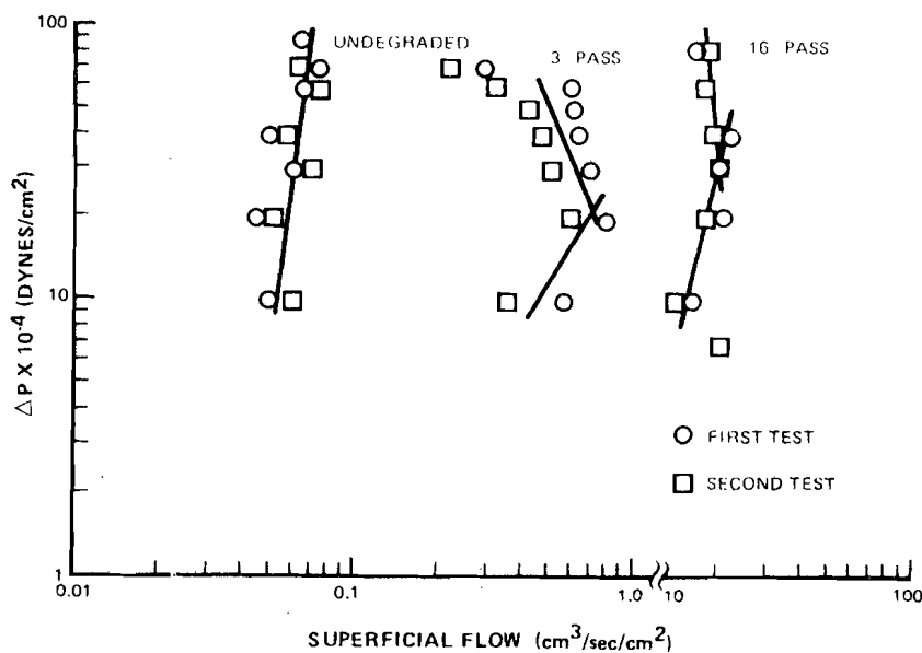
Figure 45 AMK Flow Through 40 \mu\text{m} Paper Filter
