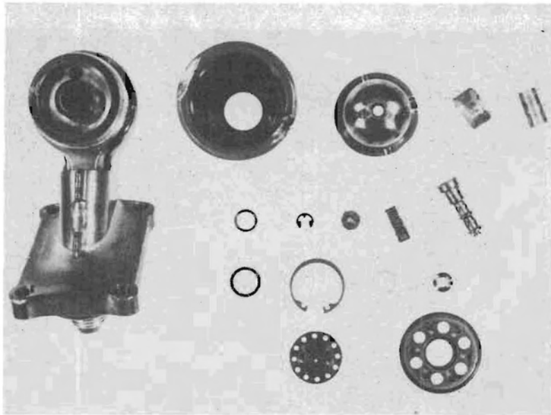
Figure 59 Post Test Disassembly of B/M Nozzle
