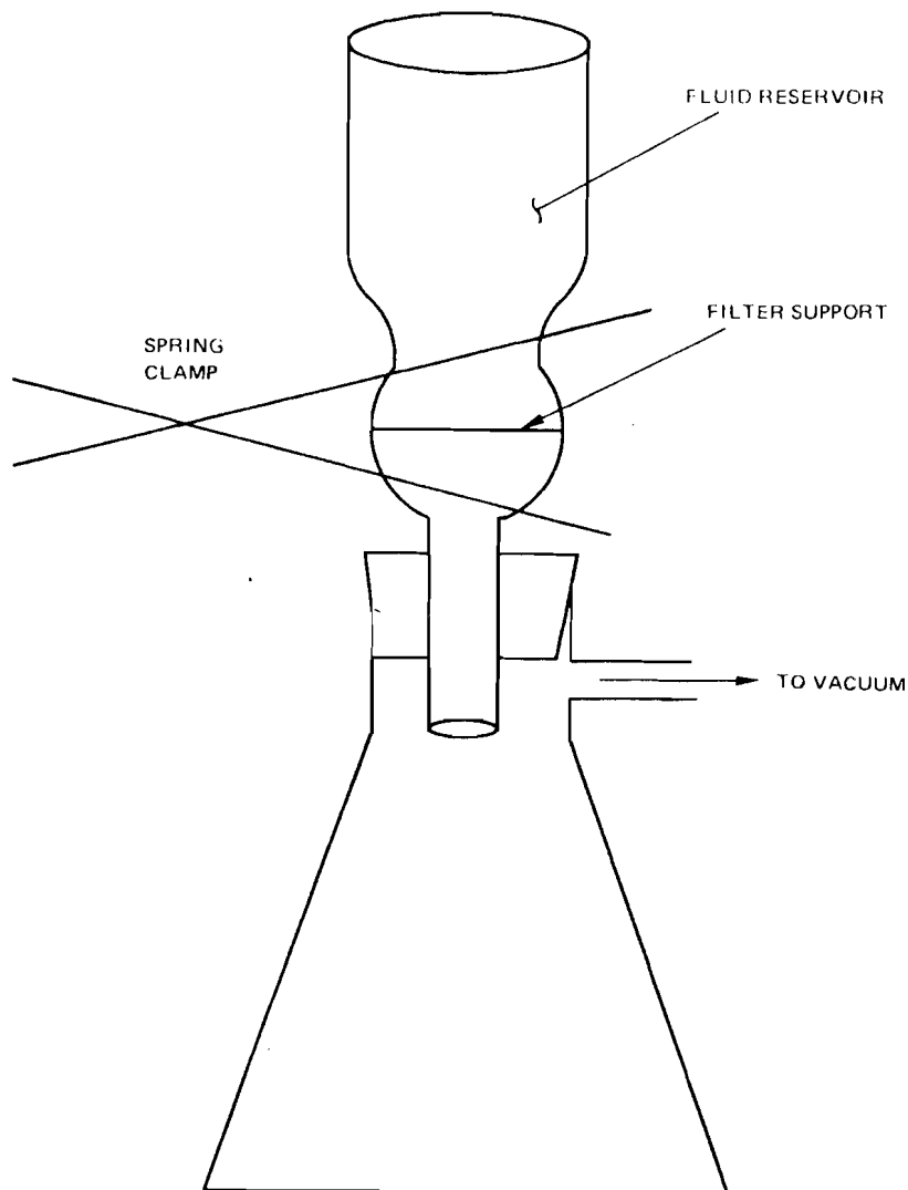
Figure 10 Millipore Apparatus
