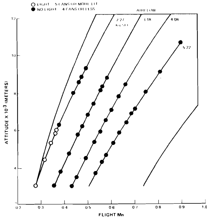
Figure 65 JT8D-17 Airstart Envelope - Bill-of-Material Combustor, 3-Pass AMK
