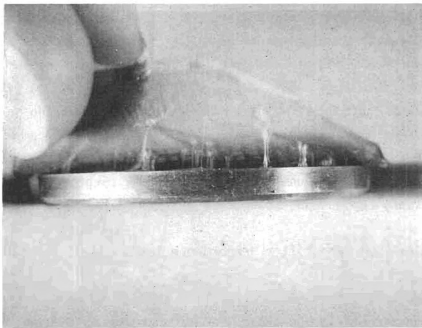
Figure 49 Gel Formed On Downstream Side of 10\mu\text{m} Metal Filter After Flow at -26^\circ\text{C}
