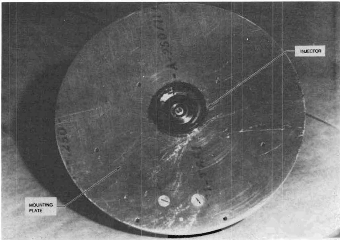
Figure 24 Low Emissions JT8D Injector
