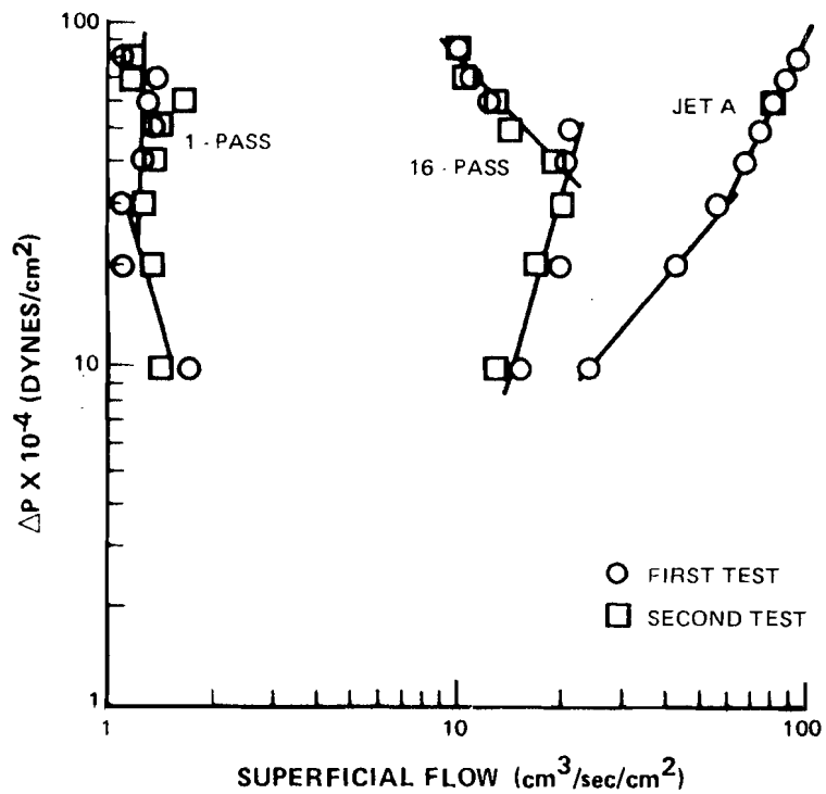
Figure 47 AMK Flow Through 17 μm Metal Screen
