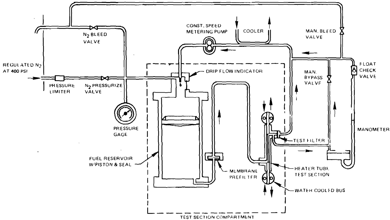
Figure 16 Thermal Stability Tester
