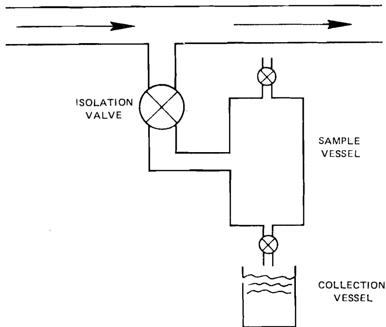
Figure 15 Sampling Apparatus
