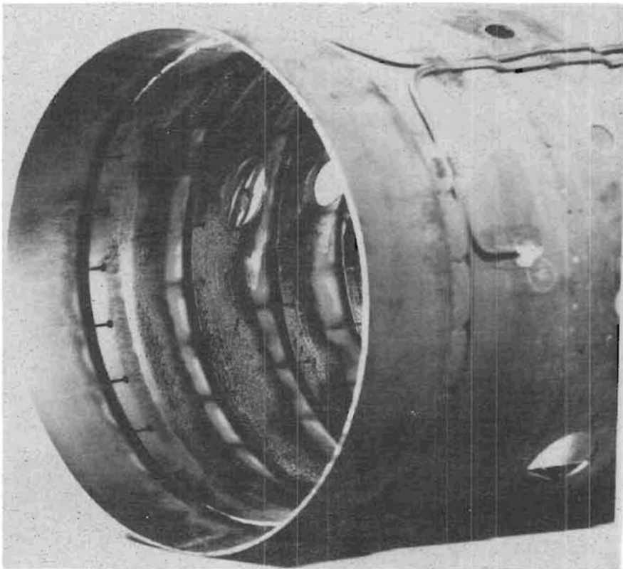
Figure 62 Post Test Photograph of L/E Combustor Can
