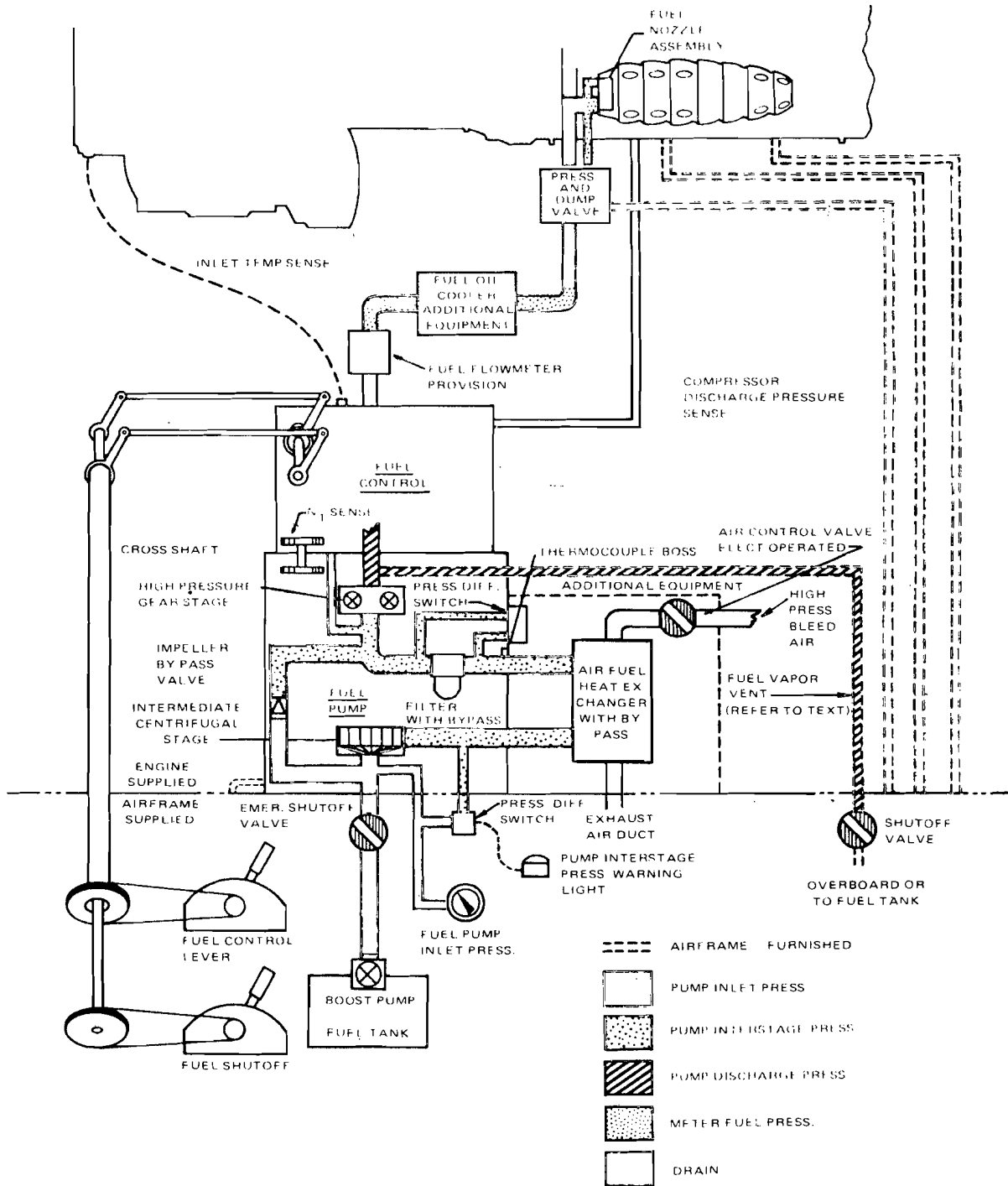
Figure 2 JT8D Turbofan Engine Fuel System Diagram
