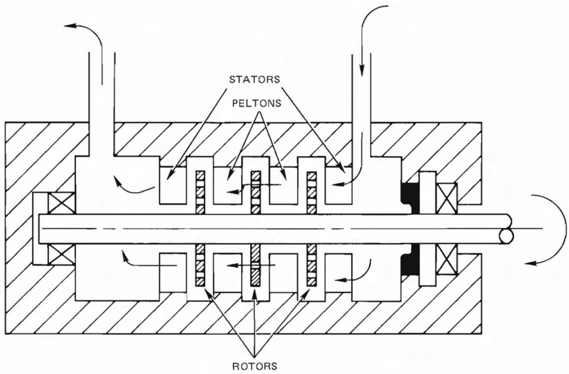
Figure 11 RAE Degradation Schematic
