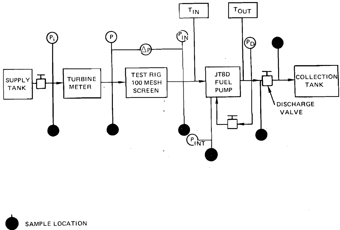
Figure 14 Instrumentation Fuel Sampling Locations
