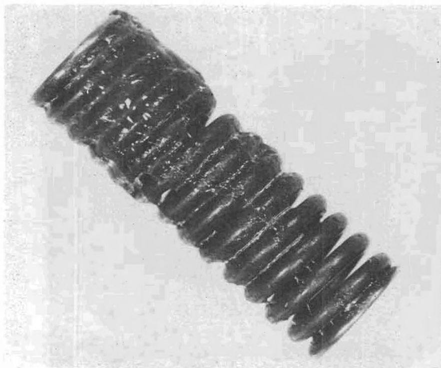
Figure 60 Gel On Spring From B/M Nozzle
