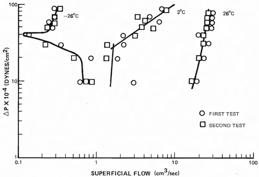
Figure 48 Effect of Reduced Temperature On Flow Properties of 3-Pass, ( F_R = 1.28 ) AMK Through 10\mu\text{m} Metal Screen
