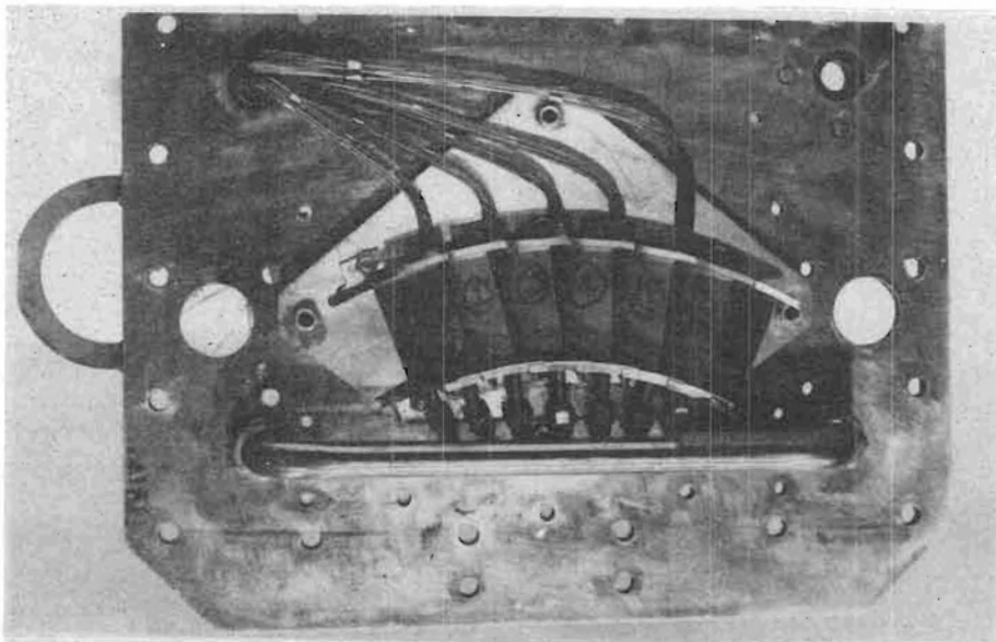
Figure 28 JT8D Combustor Exit Instrumentation Vane Pack
