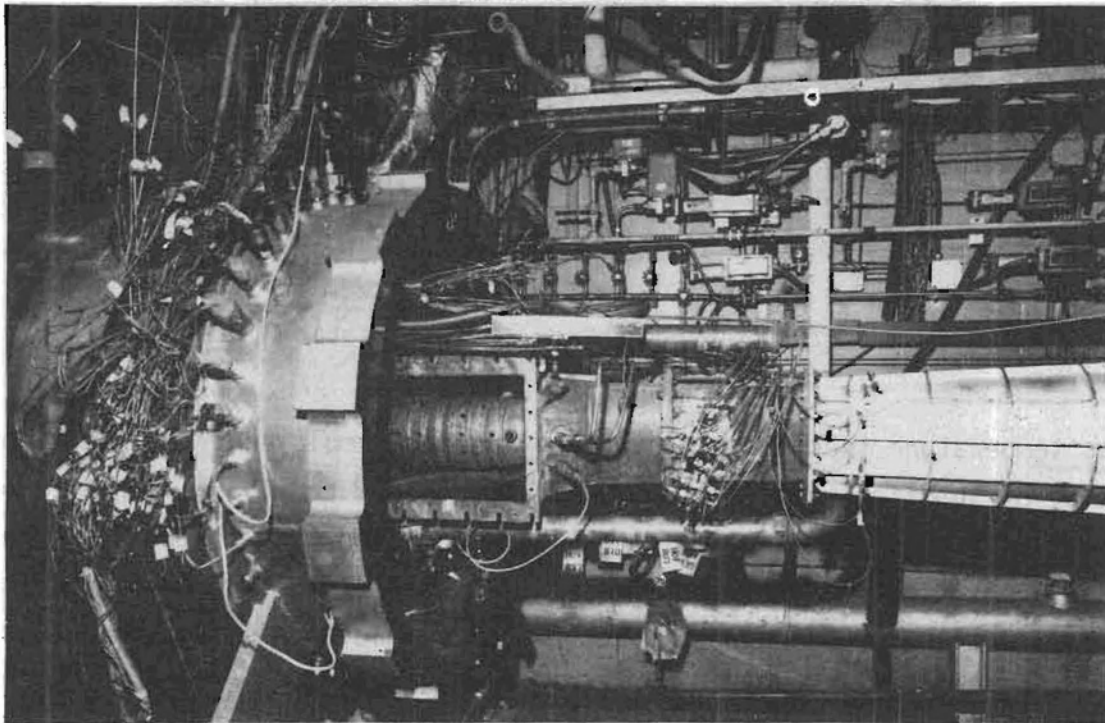
Figure 27 X-904, M.T.F., Open Rig, (Jan., 1977) R70293
