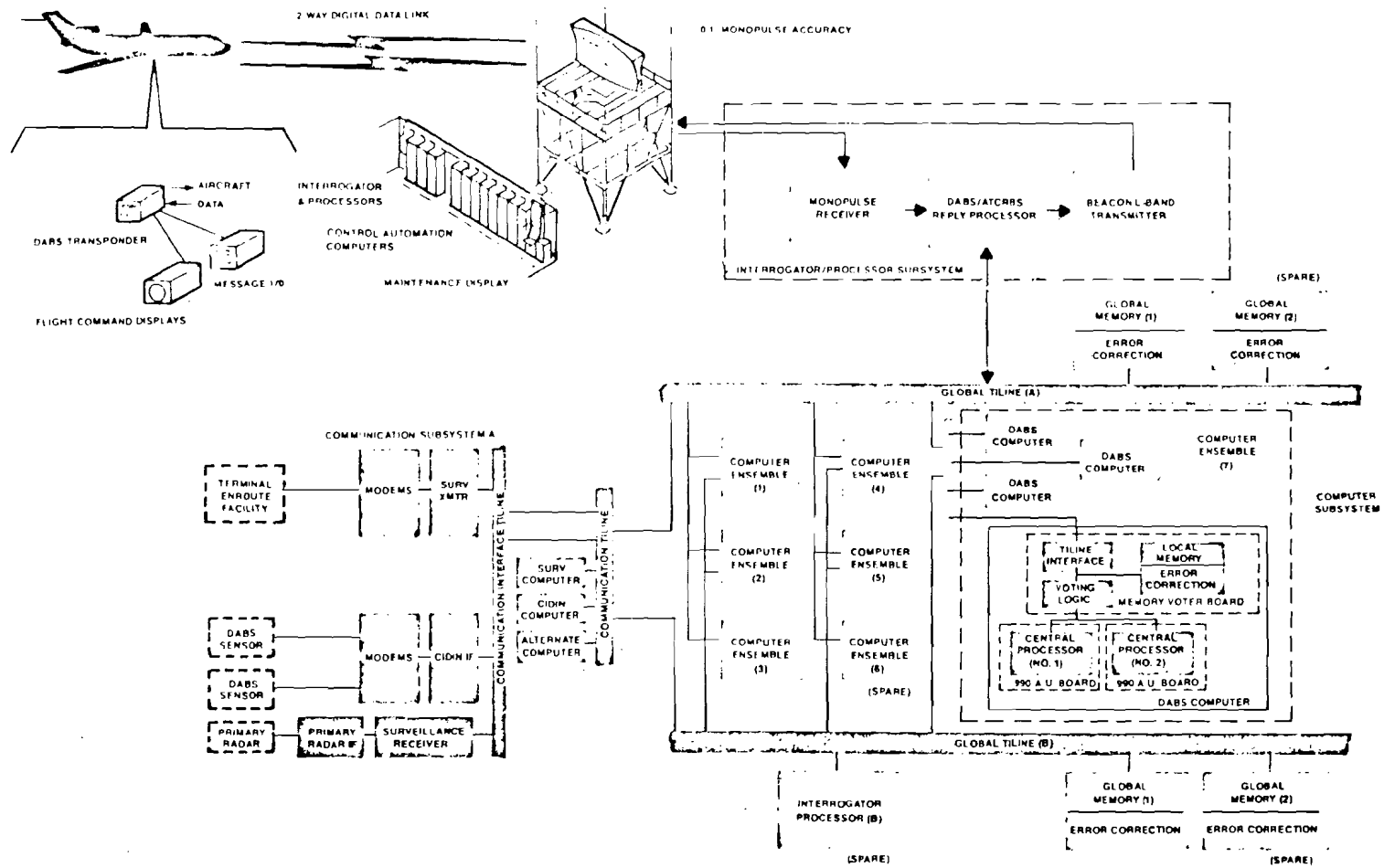
Figure 1. DABS Functional Block Diagram
