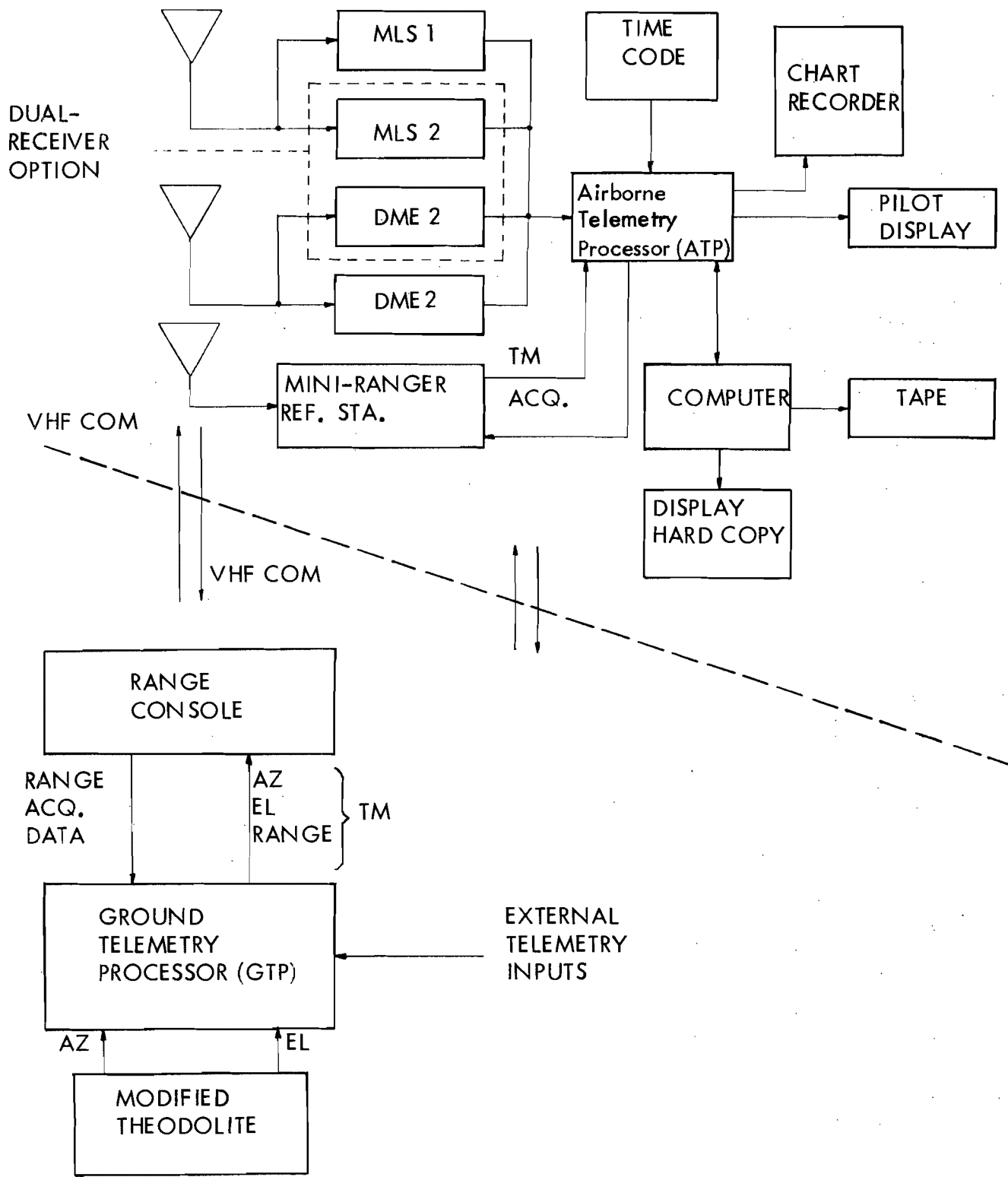
Figure 3-2. MLS Data-Collection System - Configuration 1.
