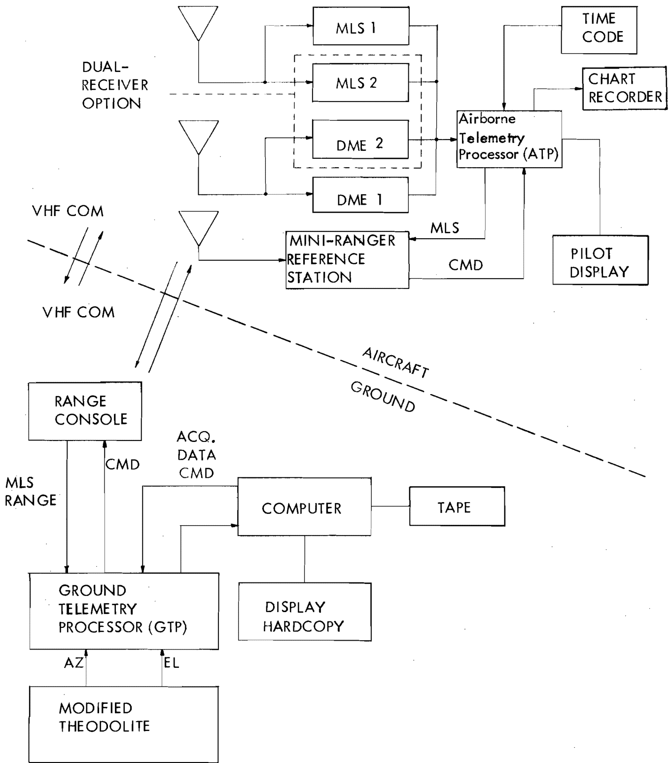
Figure 3-3. MLS Data-Collection System - Configuration 2.
