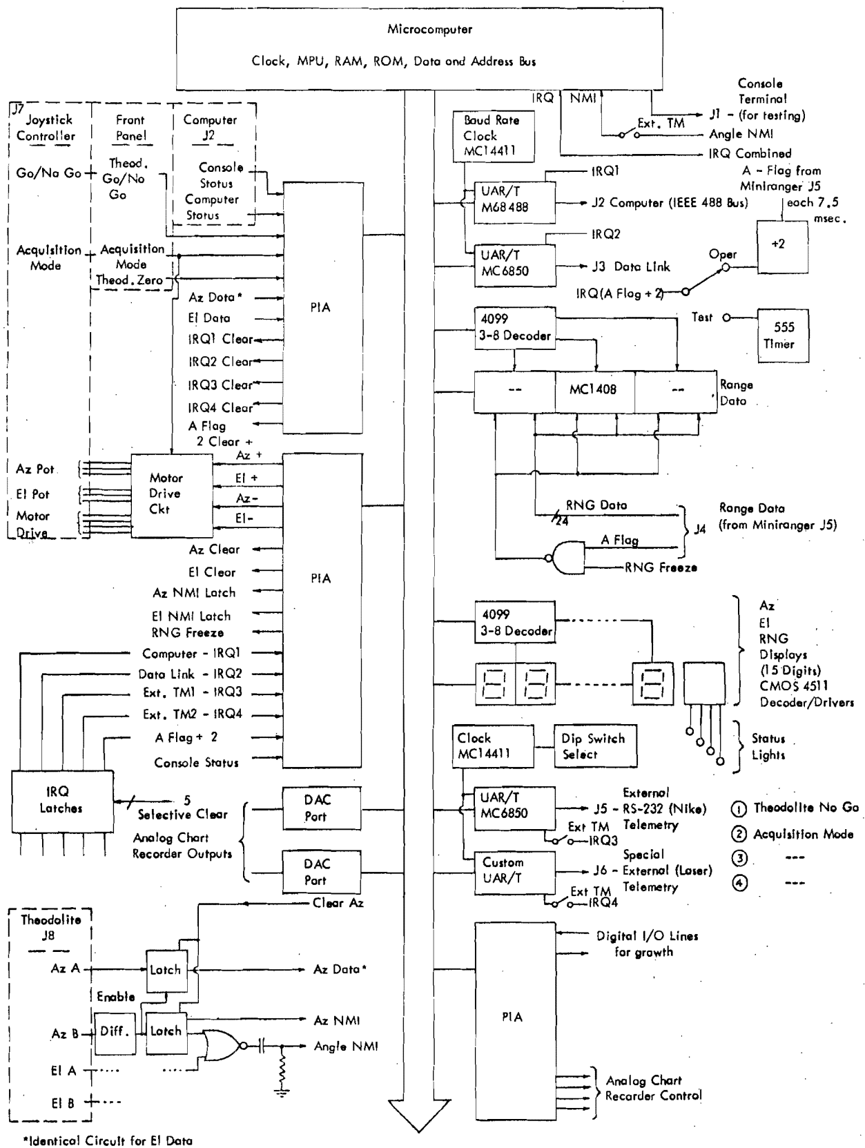
Figure 3-14. Ground Telemetry Processor - Block Diagram.
