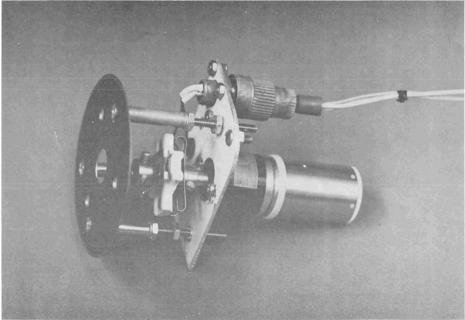
Figure 7-2. Theodolite Drive Motor Mount with Shaft Coupling for Encoder or Potentiometer. (Photograph by J. Nickum).
