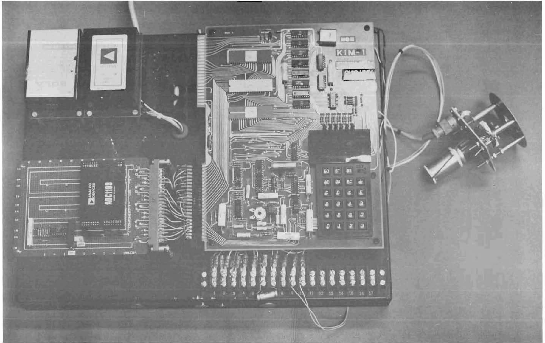
Figure 7-1. Theodolite Motor Drive Test Bed. (Photograph by J. Nickum).
