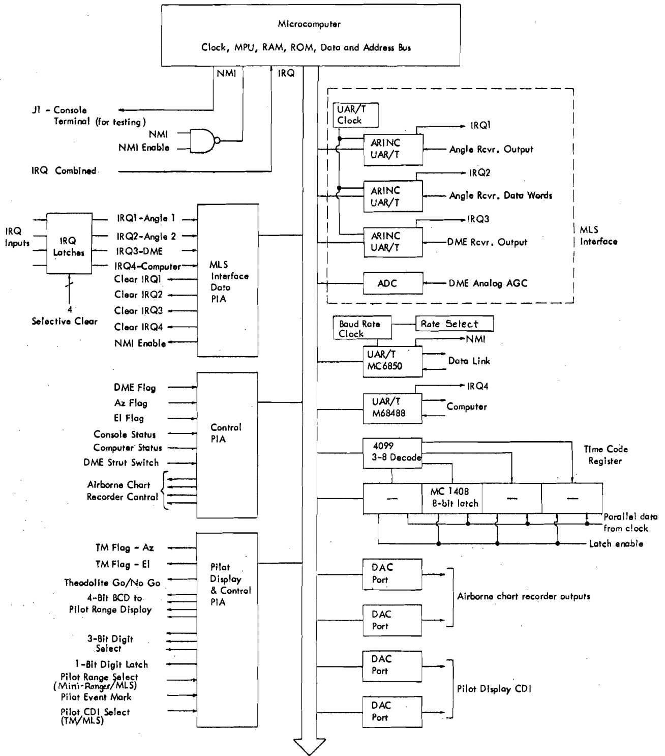
Figure 3-22. Airborne Telemetry Processor - Block Diagram.
