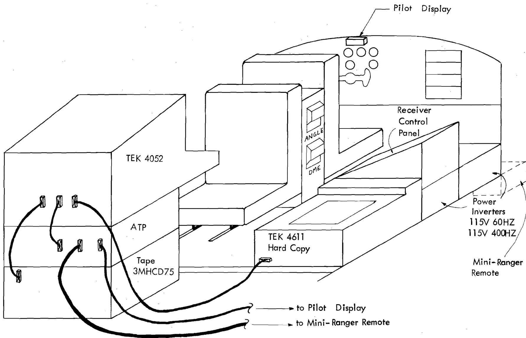
Figure 3-4. Physical Layout, Configuration 1.
