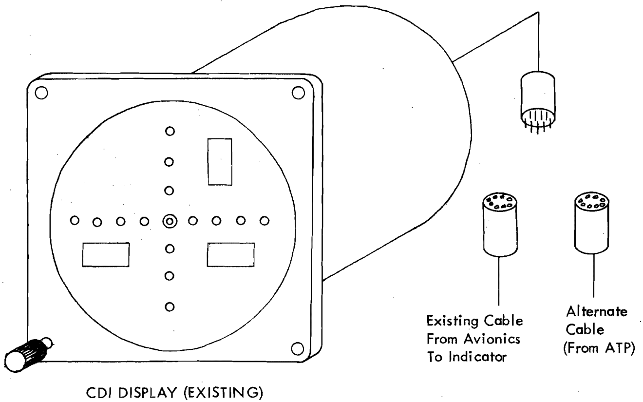
Figure 3-19. Pilot Display.
