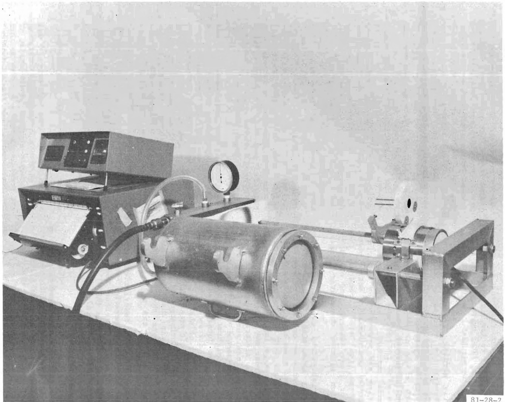
FIGURE 3. EVACUATION SLIDE MATERIAL LABORATORY TESTING APPARATUS
