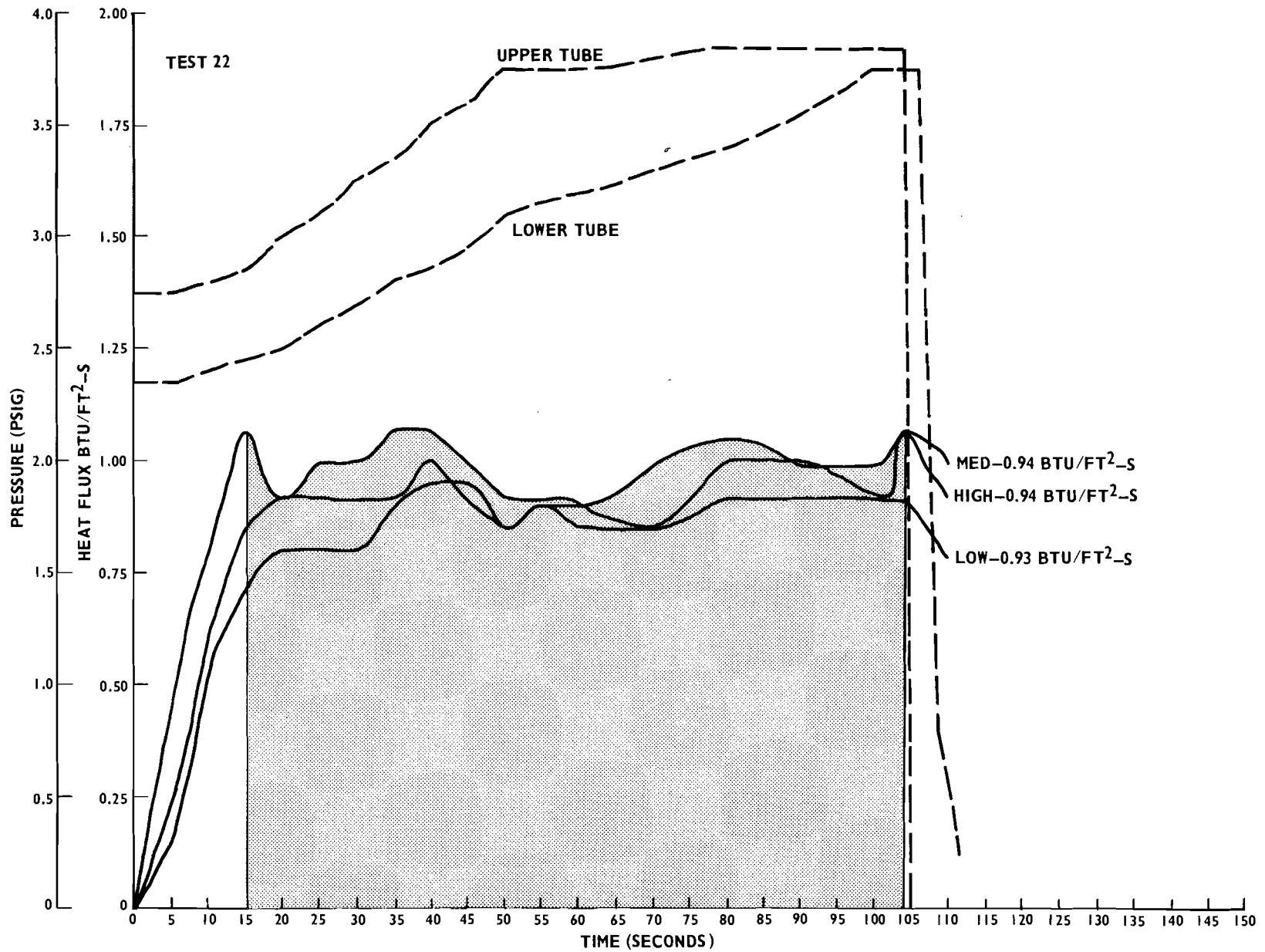
FIGURE B-17. HEAT FLUX AND PRESSURE PLOTS FOR FULL-SCALE TESTS (TEST 22)
