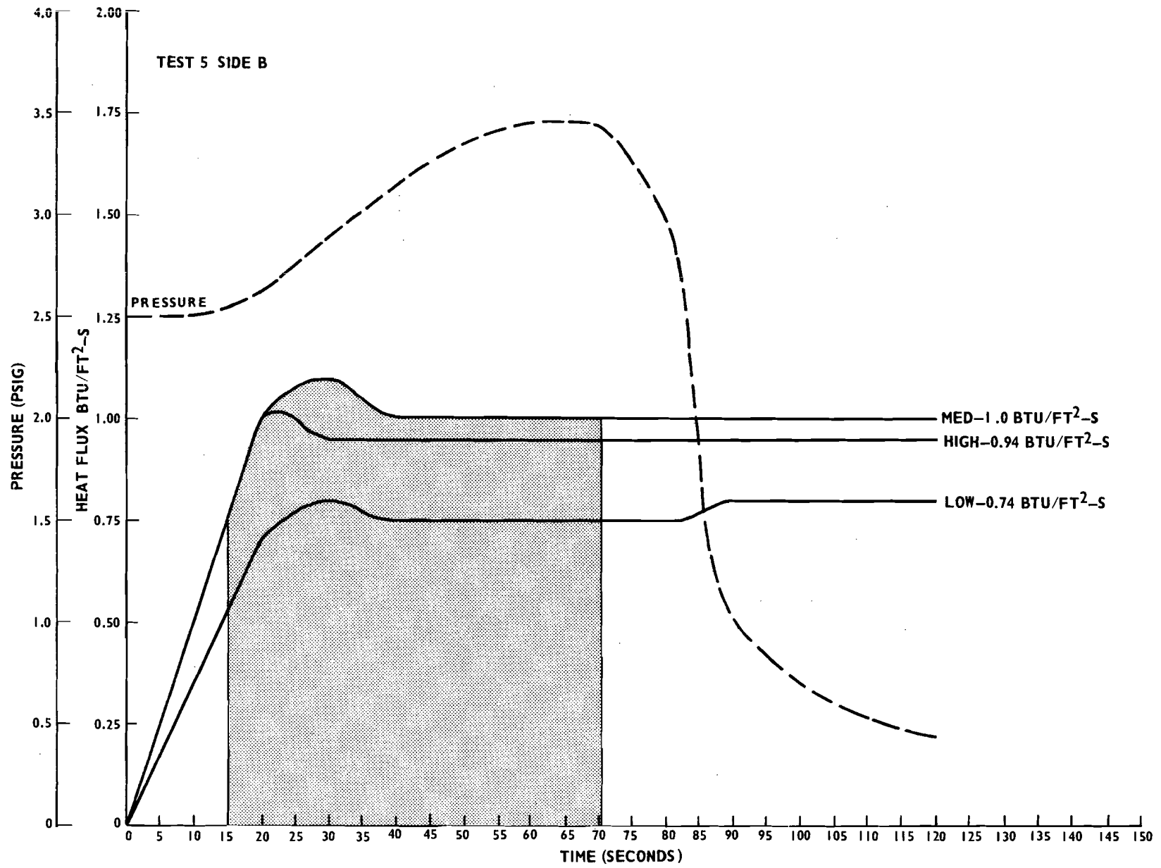
FIGURE B-4. HEAT FLUX AND PRESSURE PLOTS FOR FULL-SCALE TESTS (TEST 5, SIDE B)
