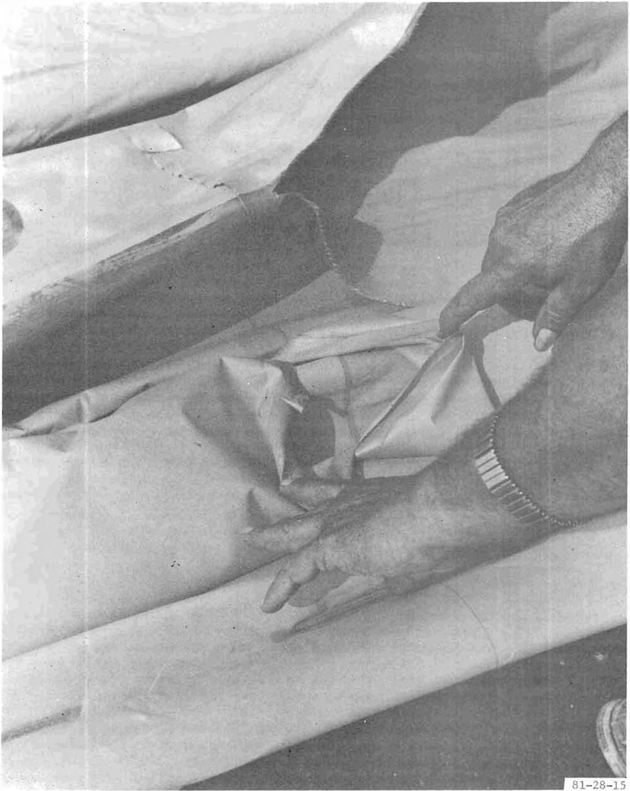
FIGURE 16. NEOPRENE NYLON SEAM FAILURE; TEST 22
