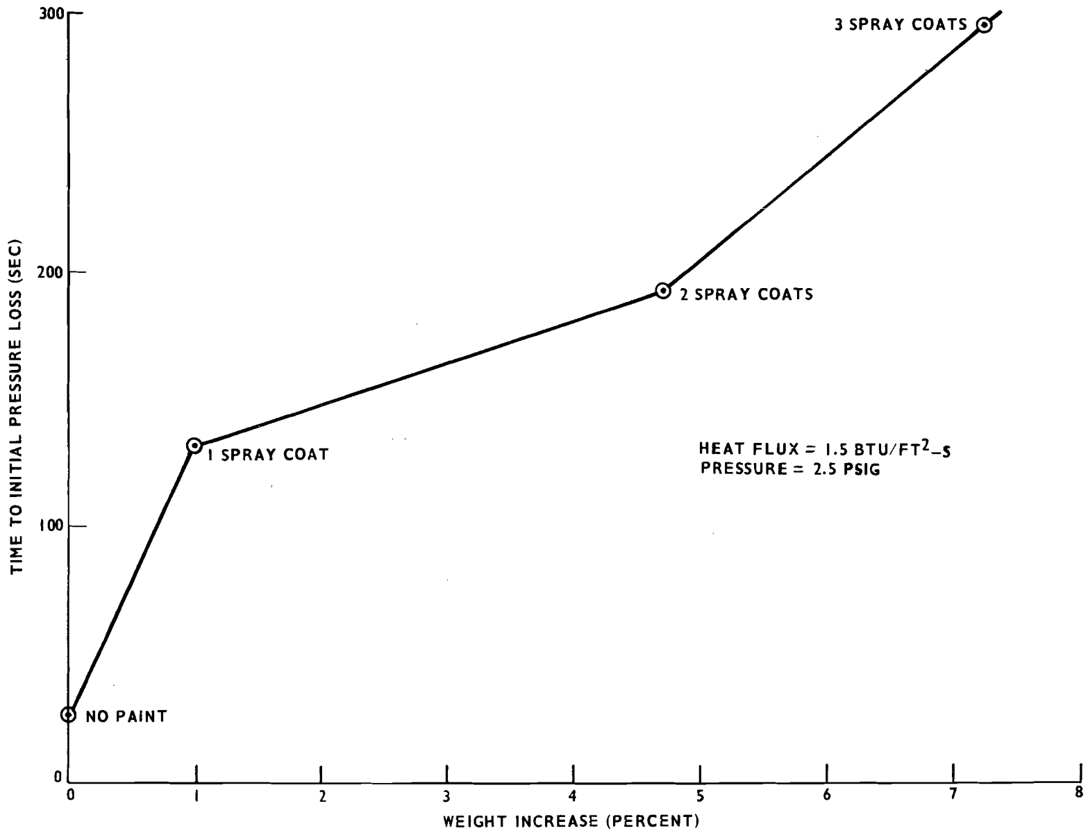
FIGURE 17. THE EFFECT OF REFLECTIVE COATING THICKNESSES
