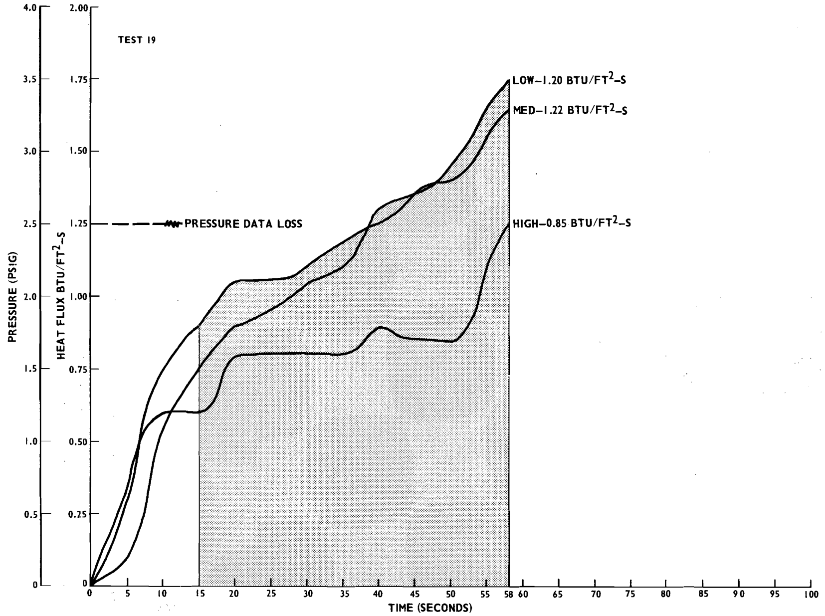
FIGURE B-15. HEAT FLUX AND PRESSURE PLOTS FOR FULL-SCALE TESTS (TEST 19)
