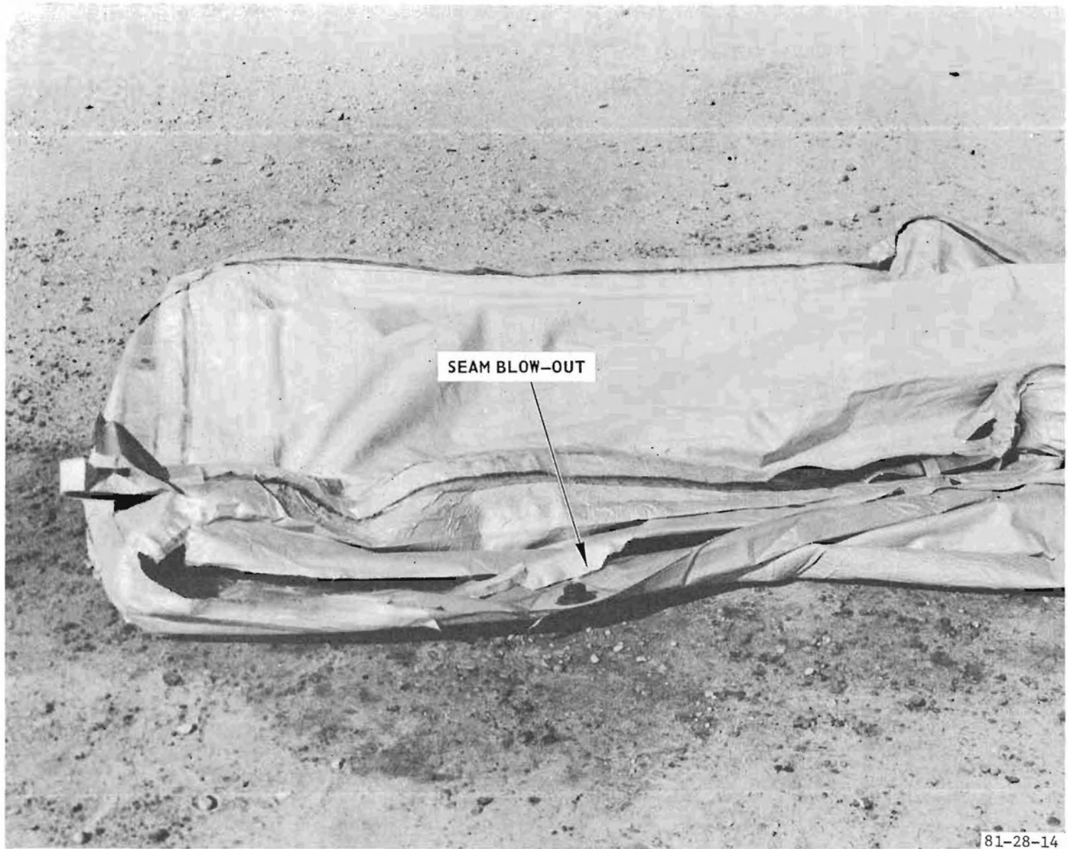
FIGURE 15. ALUMINIZED NEOPRENE NYLON SEAM FAILURE; TEST 20
