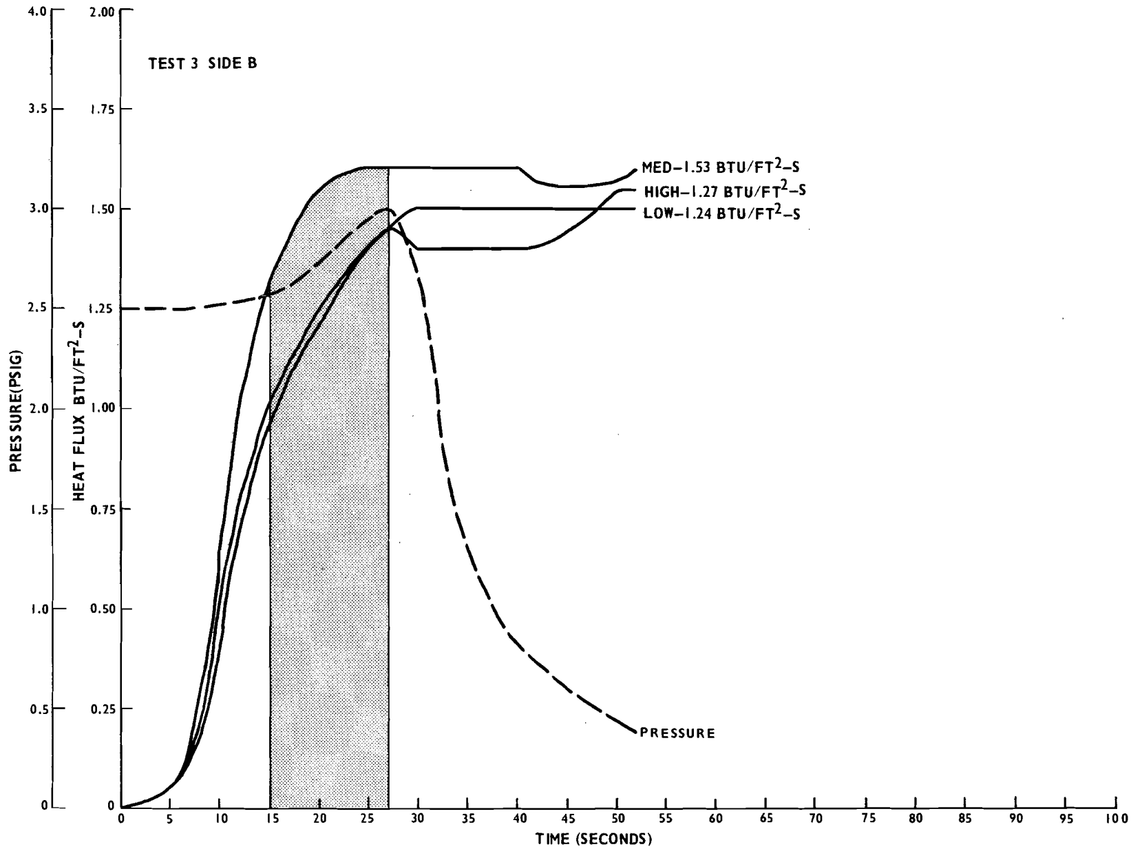
FIGURE B-2. HEAT FLUX AND PRESSURE PLOTS FOR FULL-SCALE TESTS (TEST 3, SIDE B)
