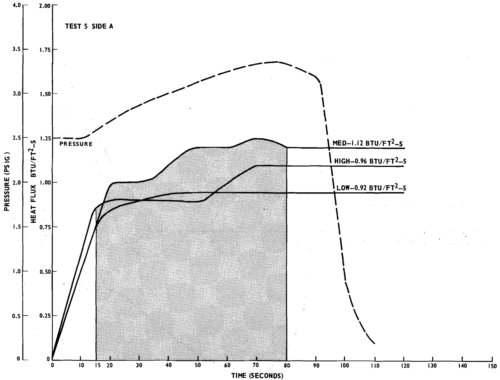
FIGURE B-3. HEAT FLUX AND PRESSURE PLOTS FOR FULL-SCALE TESTS (TEST 5, SIDE A)
