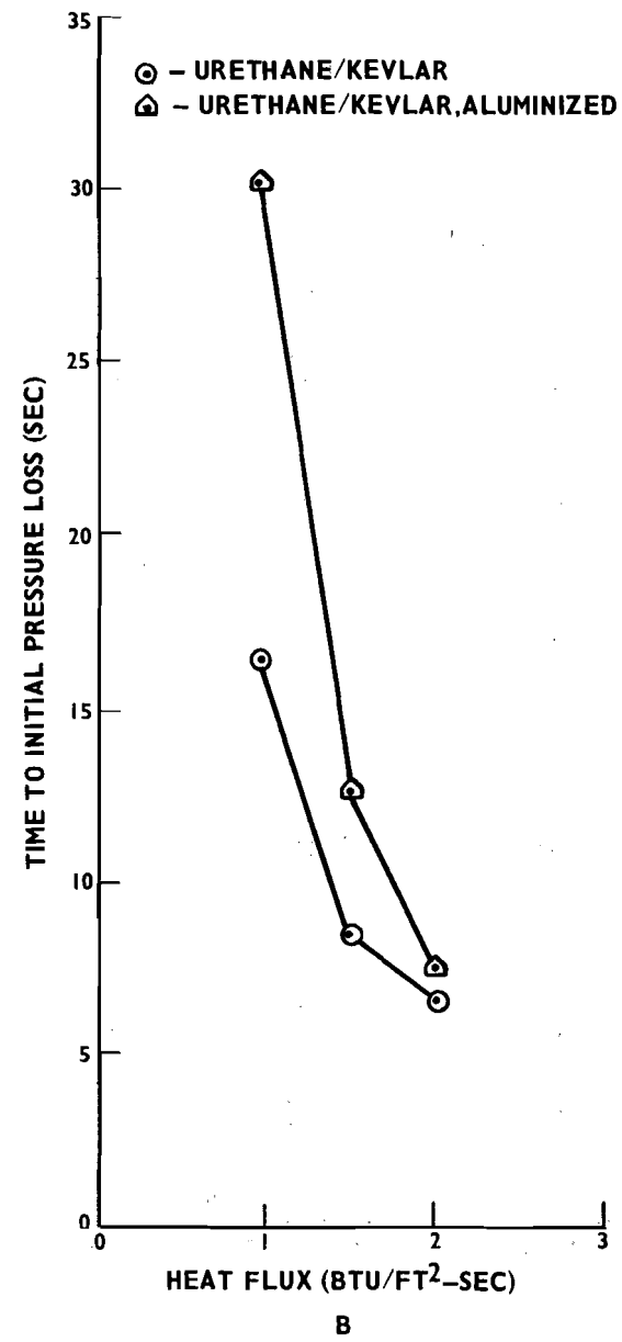
FIGURE 19. HEAT FLUX VERSUS TIME TO INITIAL PRESSURE LOSS
