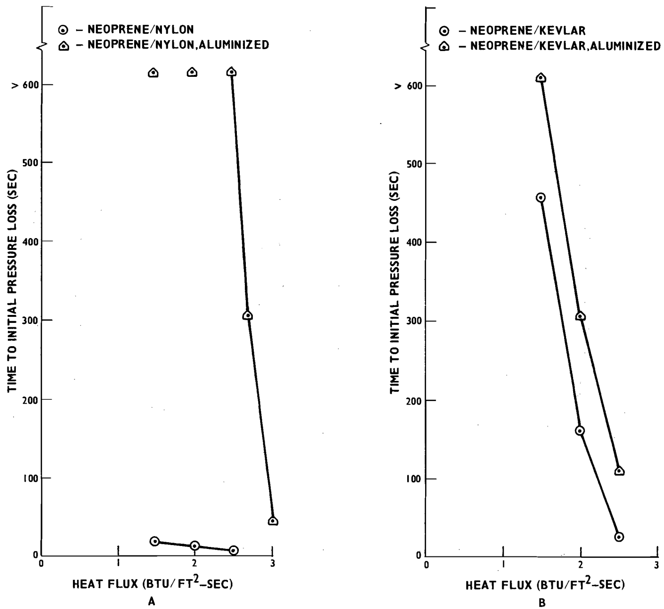
FIGURE 20. HEAT FLUX VERSUS TIME TO INITIAL PRESSURE LOSS
