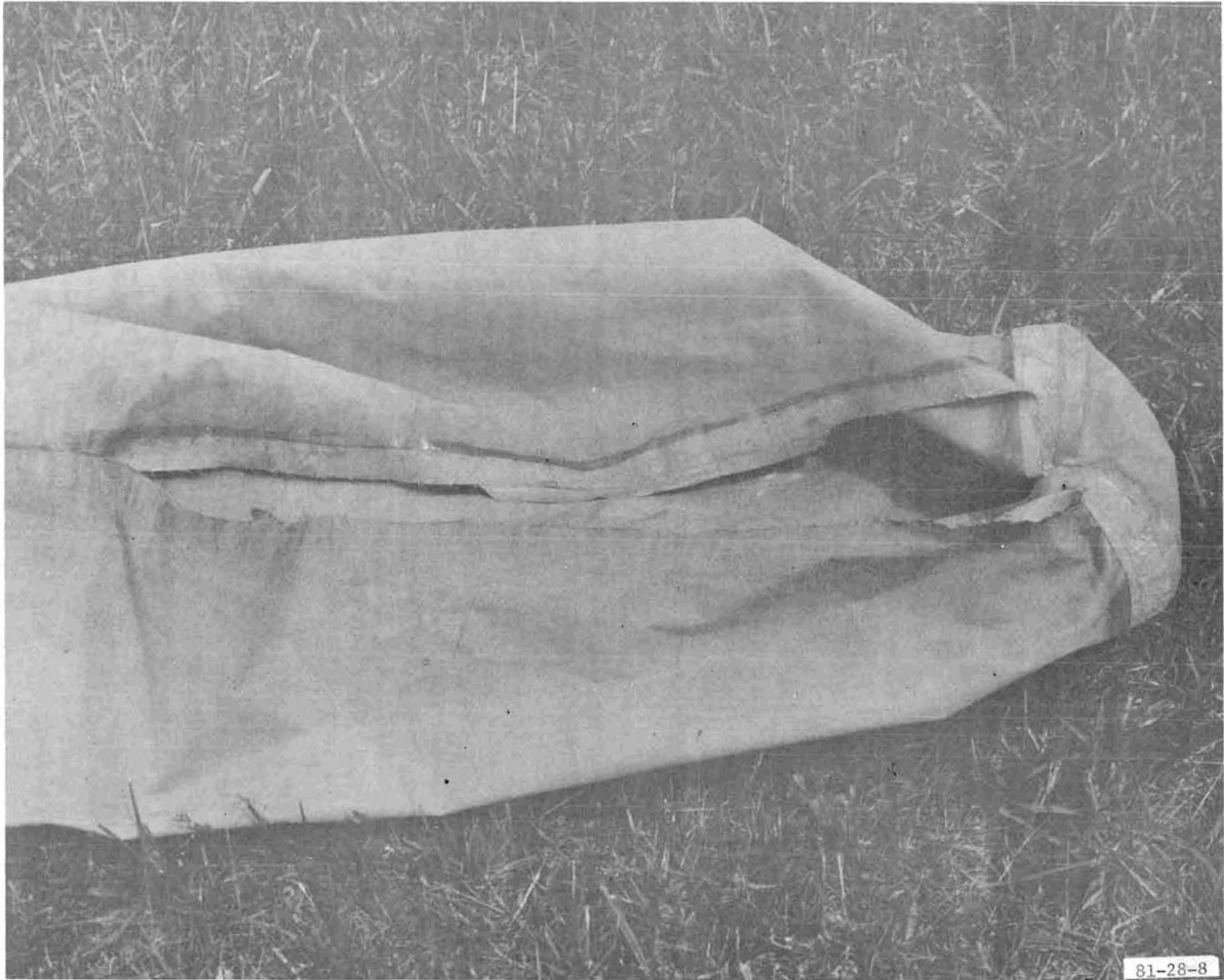
FIGURE 9. NEOPRENE KEVLAR SEAM FAILURE; TEST 14
