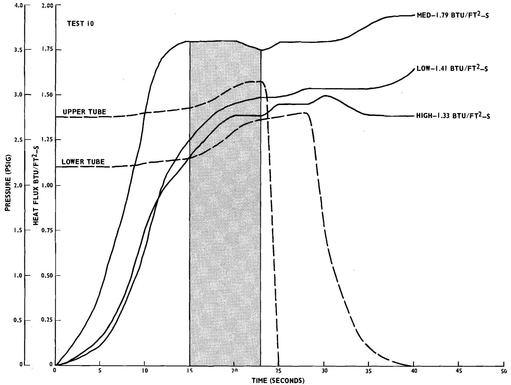
FIGURE B-8. HEAT FLUX AND PRESSURE PLOTS FOR FULL-SCALE TESTS (TEST 10)
