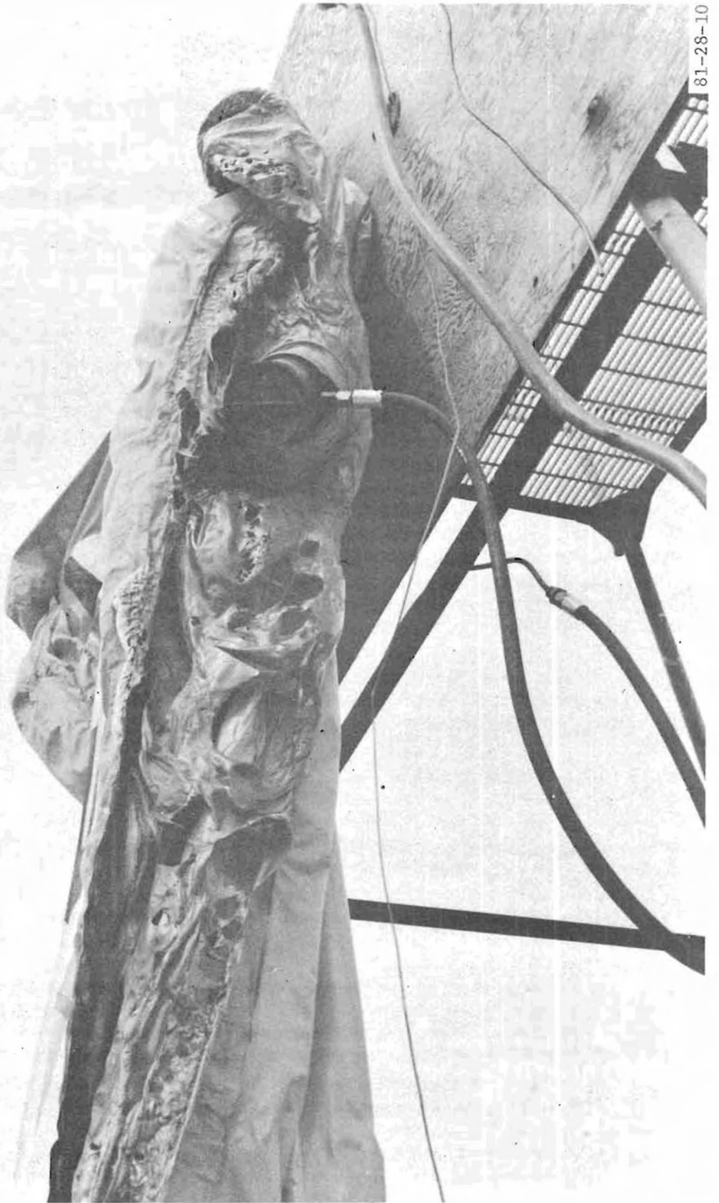
FIGURE 11. URETHANE NYLON NONSEAM FAILURE; TEST 16A
