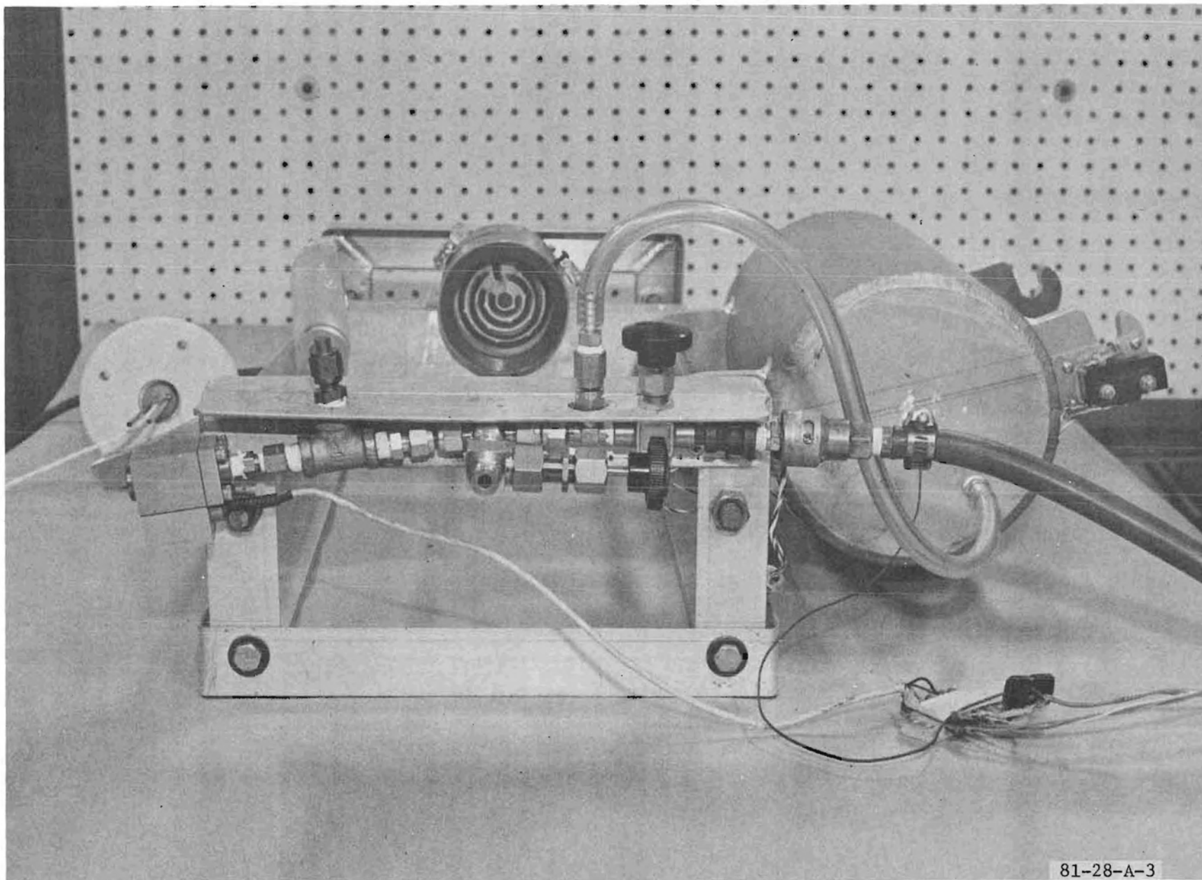
FIGURE A-3. SLIDE/SLIDE RAFT MATERIAL TEST FRONT VIEW
