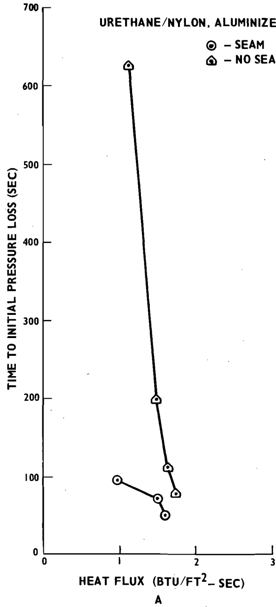
FIGURE 21. HEAT FLUX VERSUS TIME TO INITIAL PRESSURE LOSS
