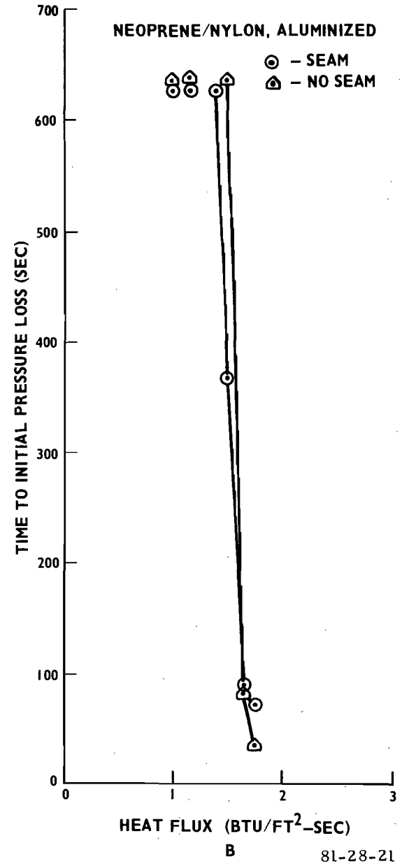
FIGURE 21. HEAT FLUX VERSUS TIME TO INITIAL PRESSURE LOSS
