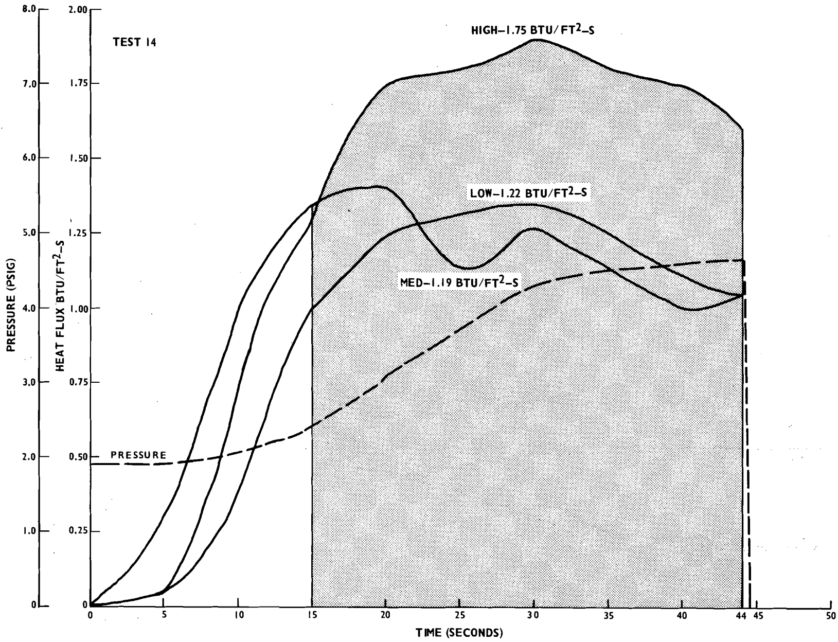
FIGURE B-11. HEAT FLUX AND PRESSURE PLOTS FOR FULL-SCALE TESTS (TEST 14)
