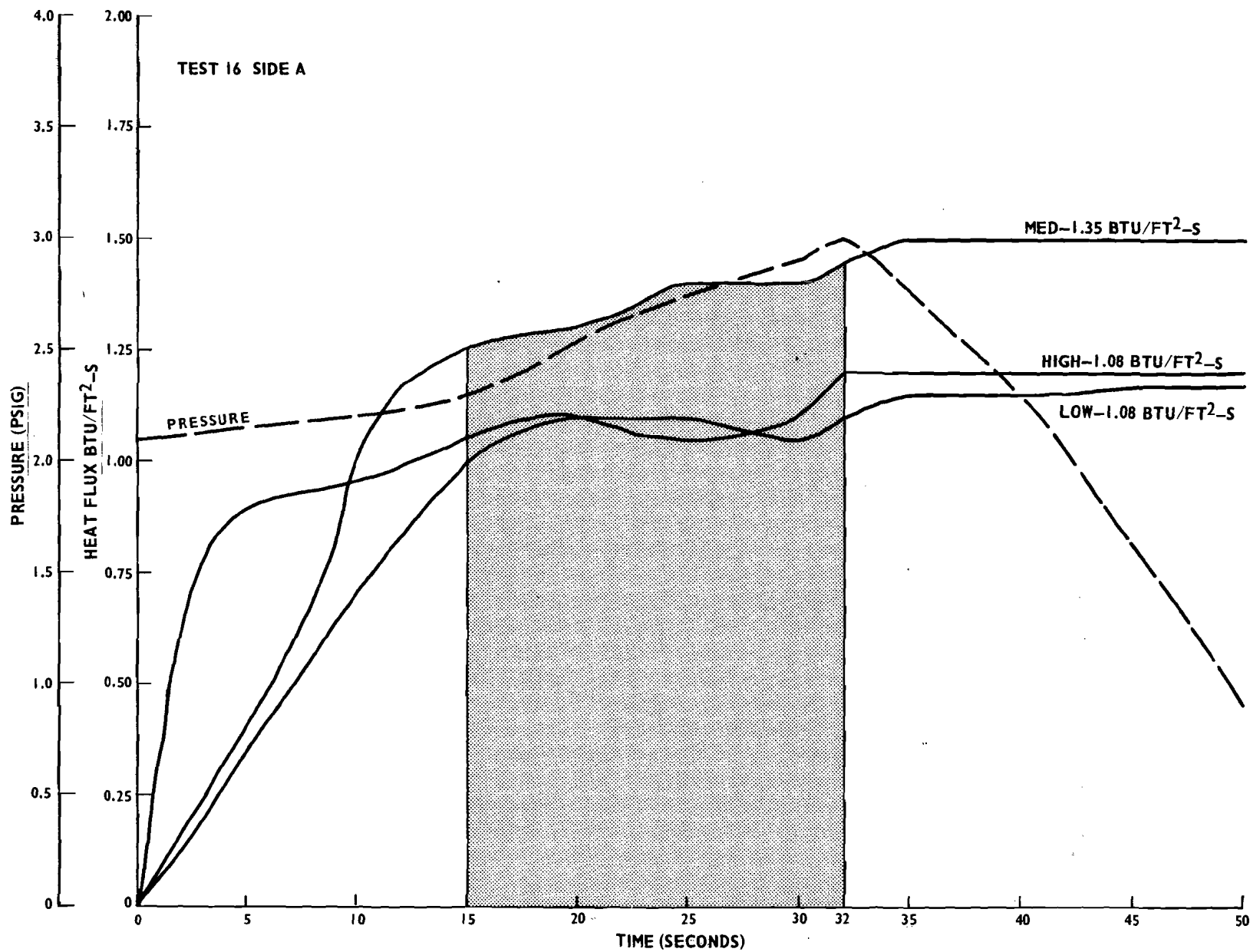
FIGURE B-12. HEAT FLUX AND PRESSURE PLOTS FOR FULL-SCALE TESTS (TEST 16, SIDE A)
