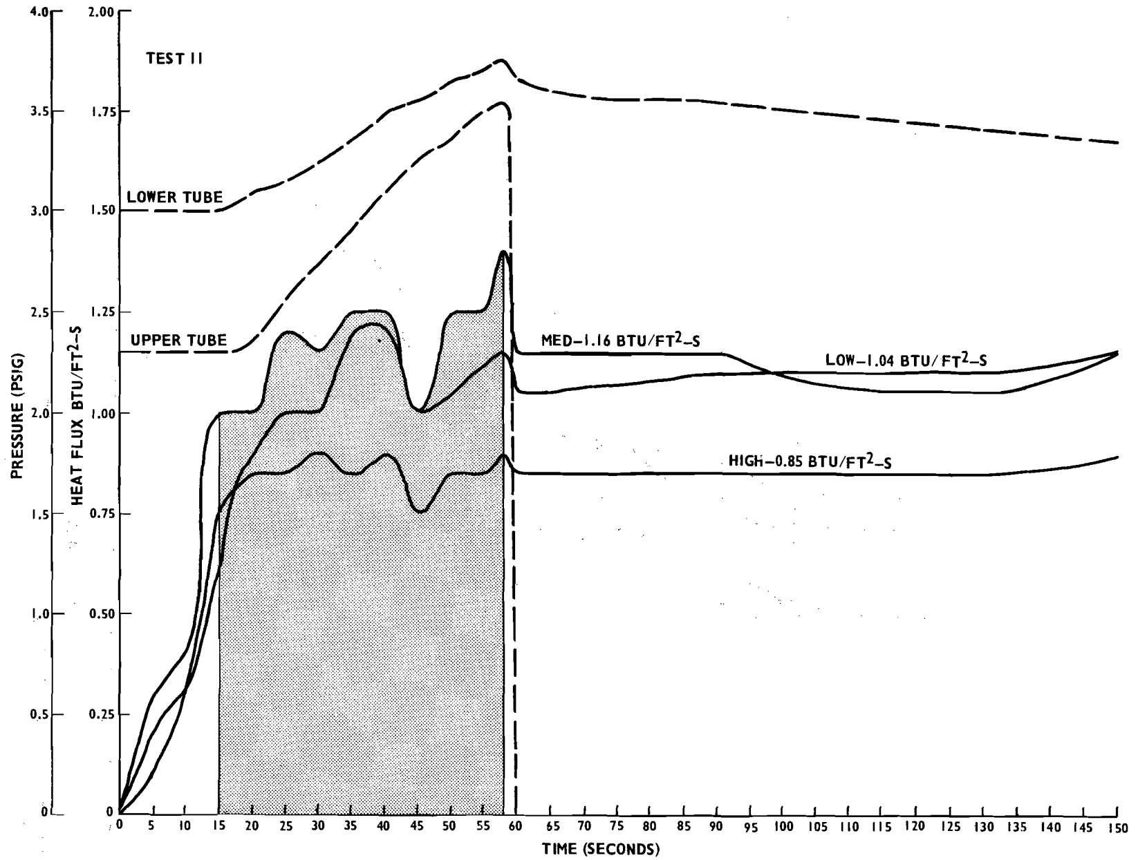
FIGURE B-9. HEAT FLUX AND PRESSURE PLOTS FOR FULL-SCALE TESTS (TEST 11)
