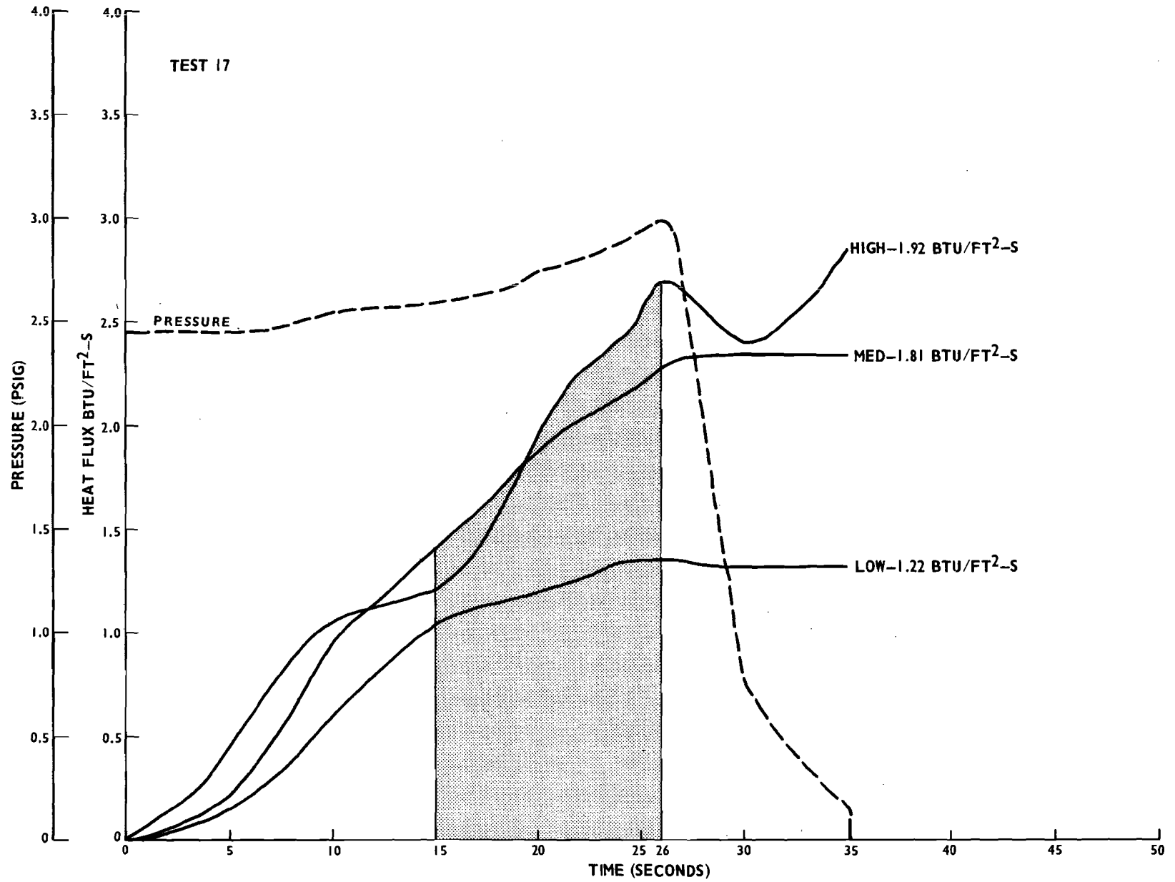
FIGURE B-14. HEAT FLUX AND PRESSURE PLOTS FOR FULL-SCALE TESTS (TEST 17)
