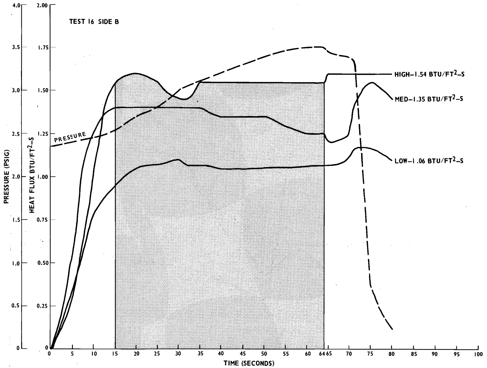
FIGURE B-13. HEAT FLUX AND PRESSURE PLOTS FOR FULL-SCALE TESTS (TEST 16, SIDE B)
