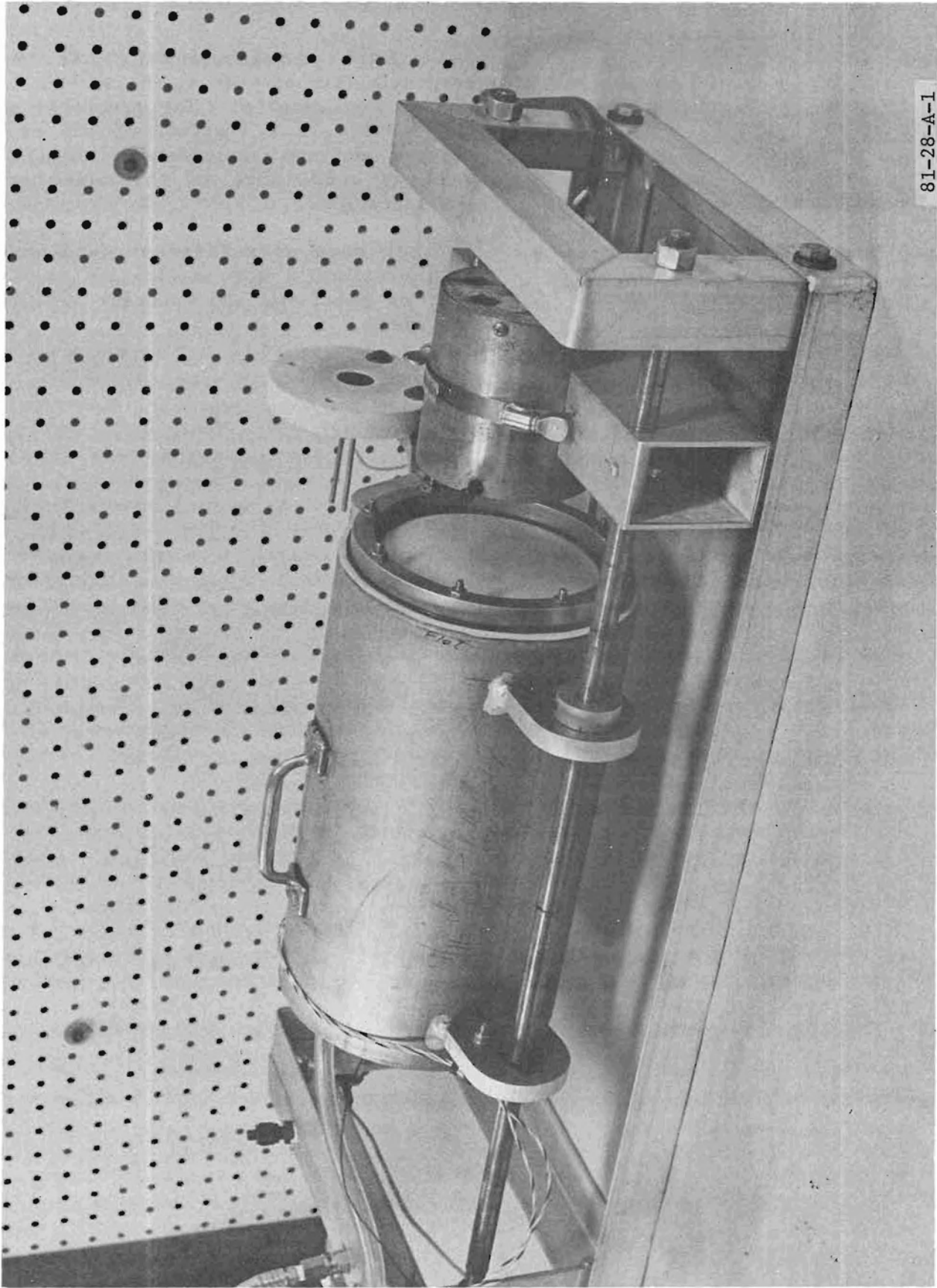
FIGURE A-1. SLIDE/SLIDE RAFT MATERIAL TEST APPARATUS
