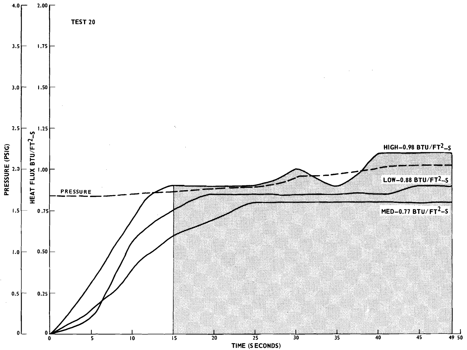
FIGURE B-16. HEAT FLUX AND PRESSURE PLOTS FOR FULL-SCALE TESTS (TEST 20)
