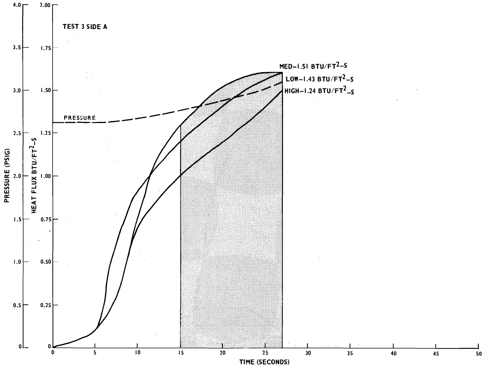
FIGURE B-1. HEAT FLUX AND PRESSURE PLOTS FOR FULL-SCALE TESTS (TEST 3, SIDE A)
