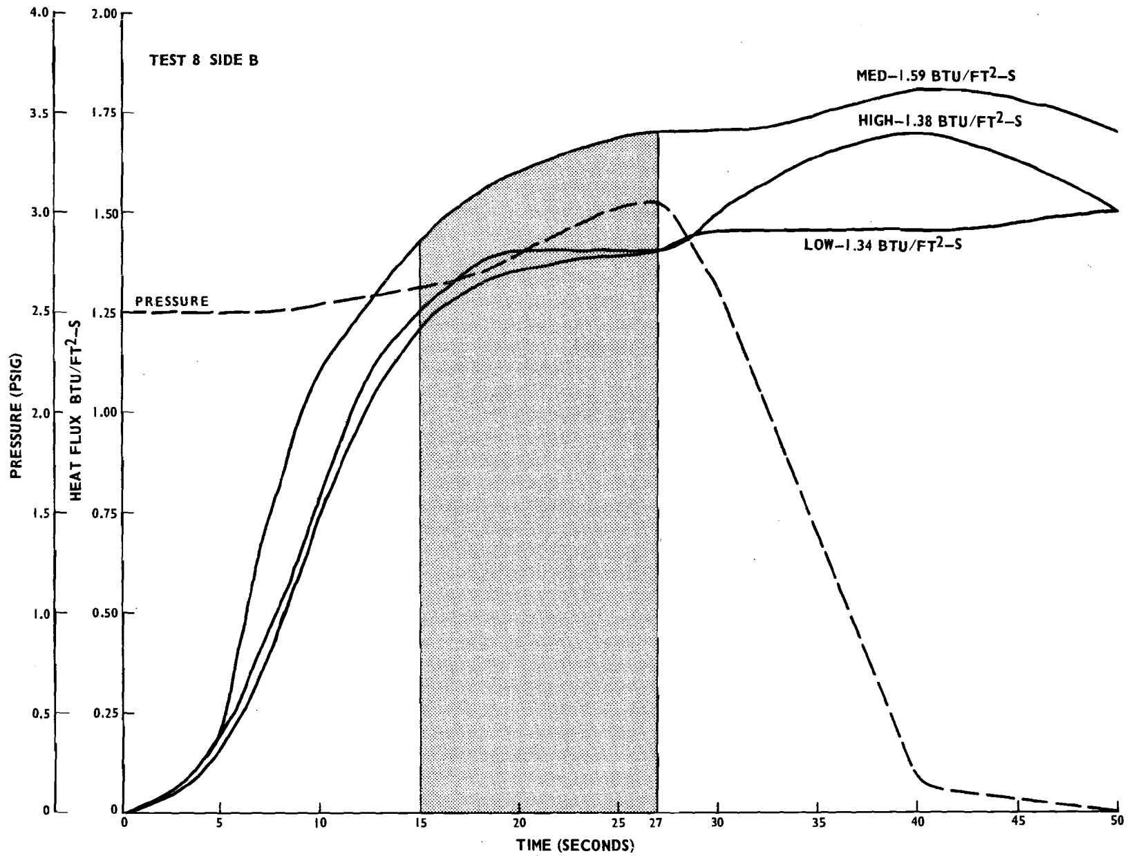
FIGURE B-6. HEAT FLUX AND PRESSURE PLOTS FOR FULL-SCALE TESTS (TEST 8, SIDE B)
