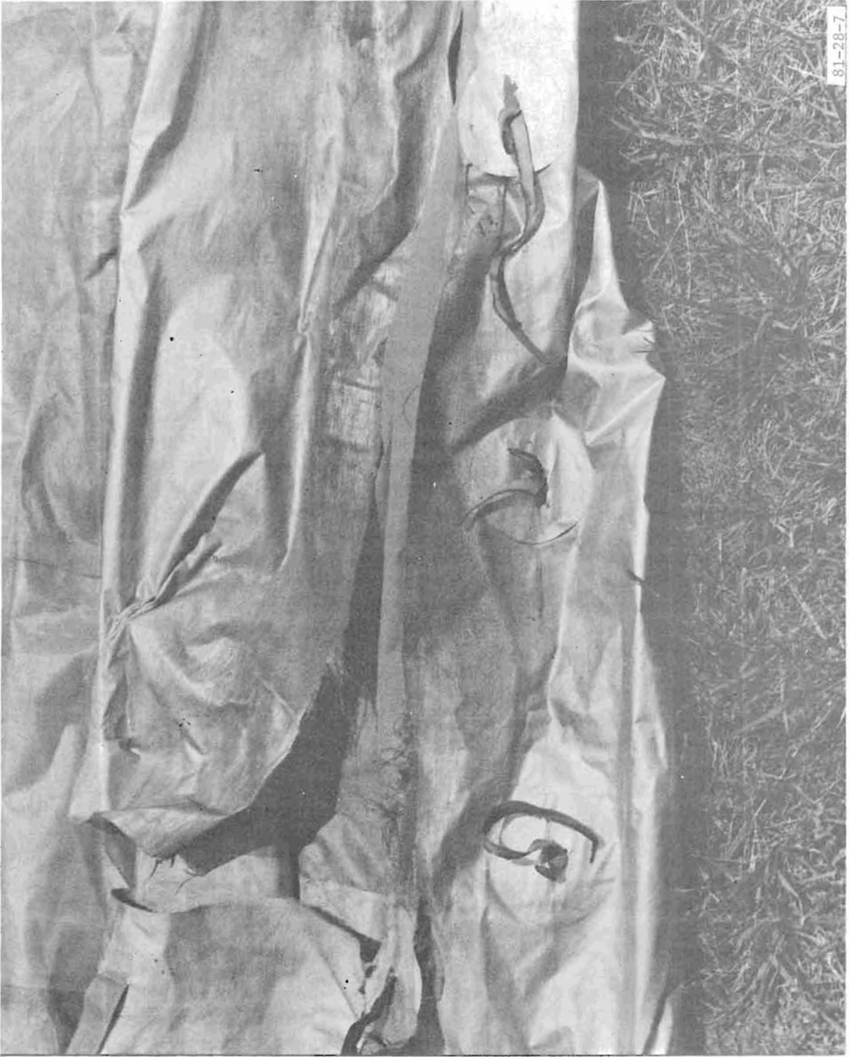
FIGURE 8. ALUMINIZED NEOPRENE KEVLAR SEAM FAILURE; TEST 12
