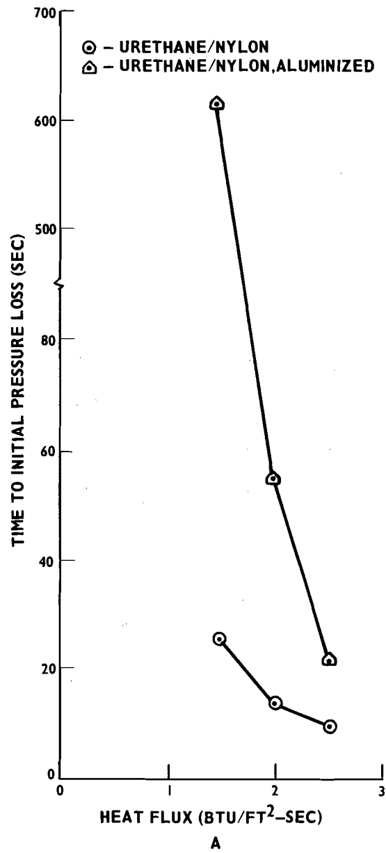
FIGURE 19. HEAT FLUX VERSUS TIME TO INITIAL PRESSURE LOSS
