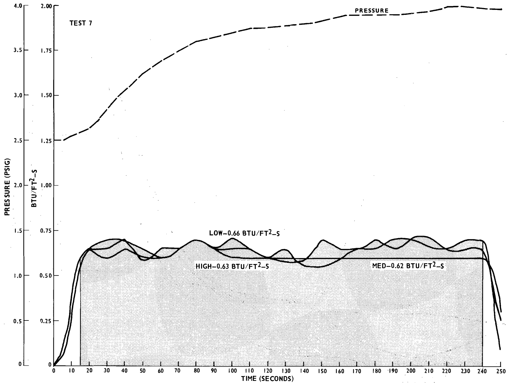
FIGURE B-5. HEAT FLUX AND PRESSURE PLOTS FOR FULL-SCALE TESTS (TEST 7)
