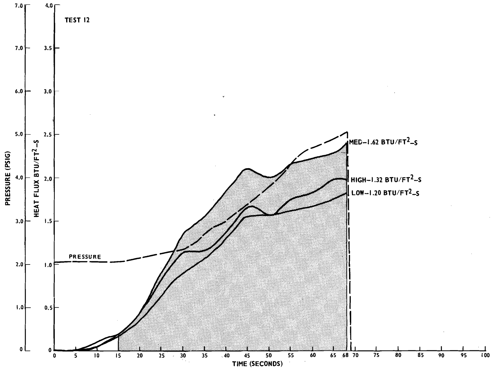
FIGURE B-10. HEAT FLUX AND PRESSURE PLOTS FOR FULL-SCALE TESTS (TEST 12)
