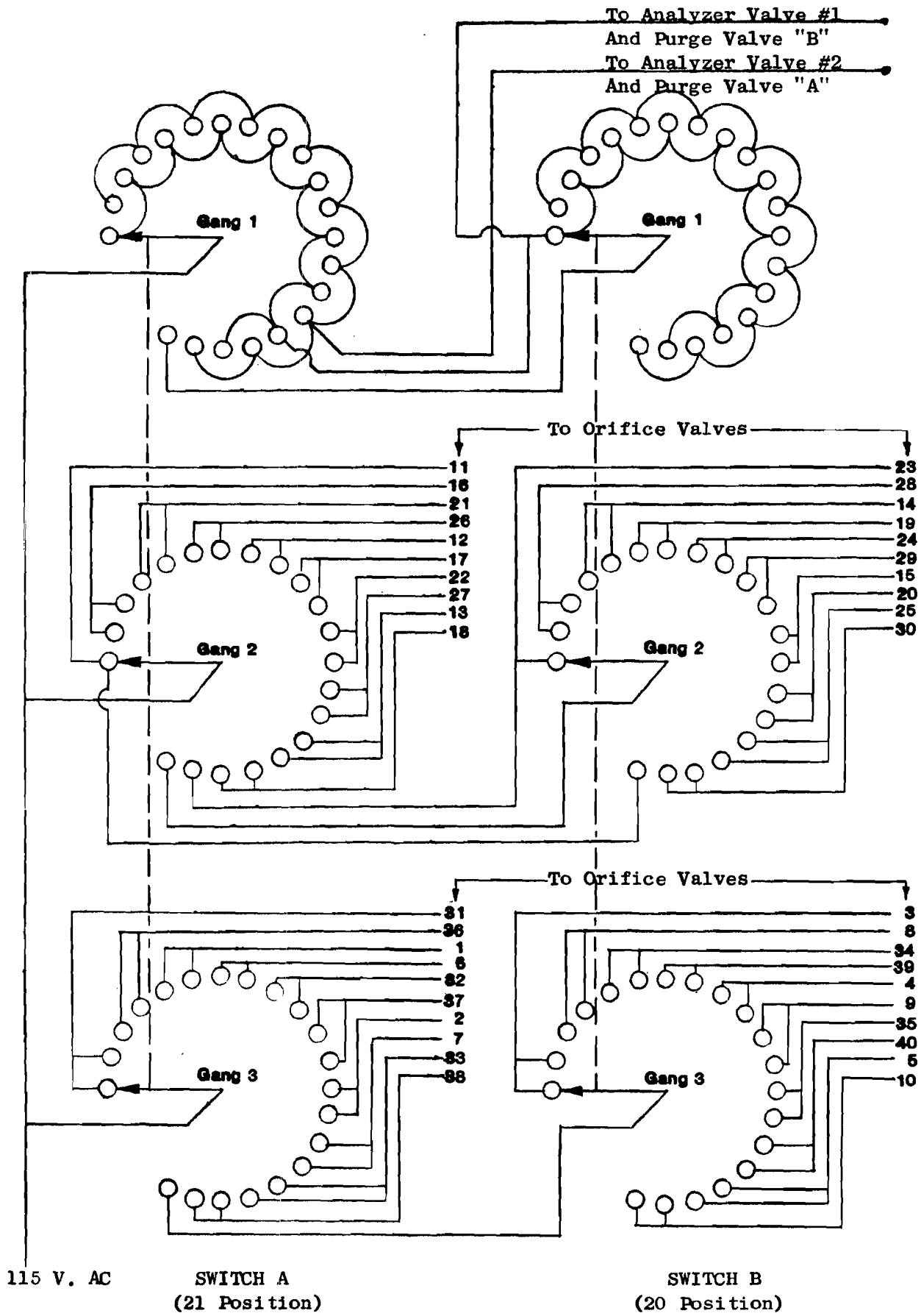
FIGURE 7. WIRING SCHEMATIC FOR SAMPLING SYSTEM SEQUENCING SWITCHES.
