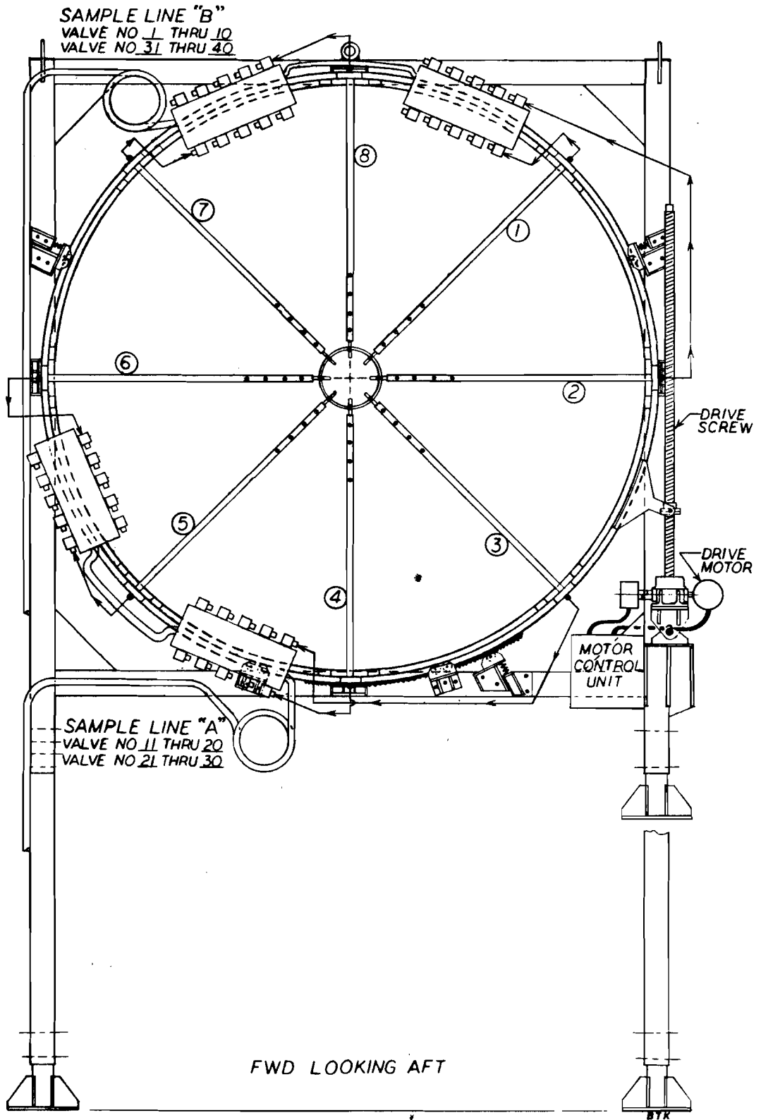
FIGURE 3. TRAVERSE PROBE SYSTEM.
