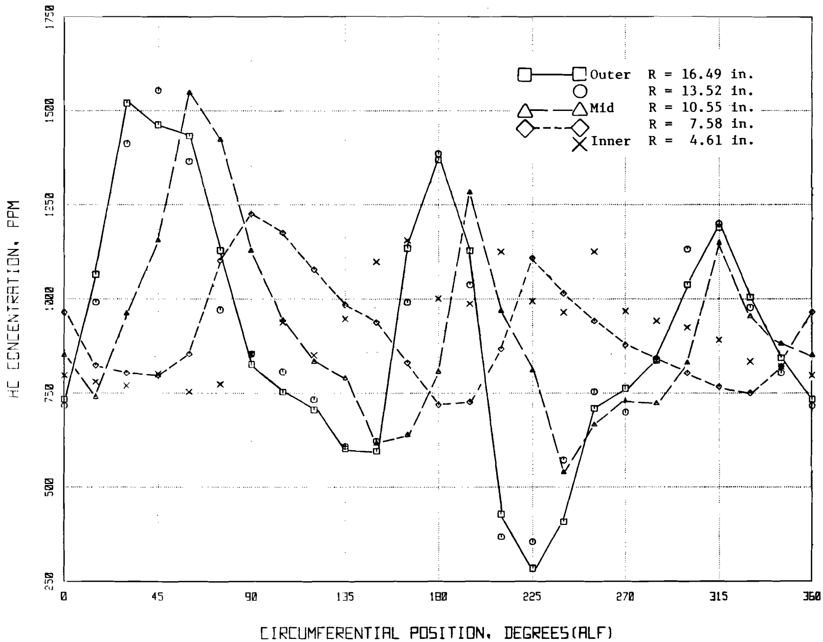
FIGURE 13. HC CONCENTRATION DISTRIBUTION AT IDLE POWER.
