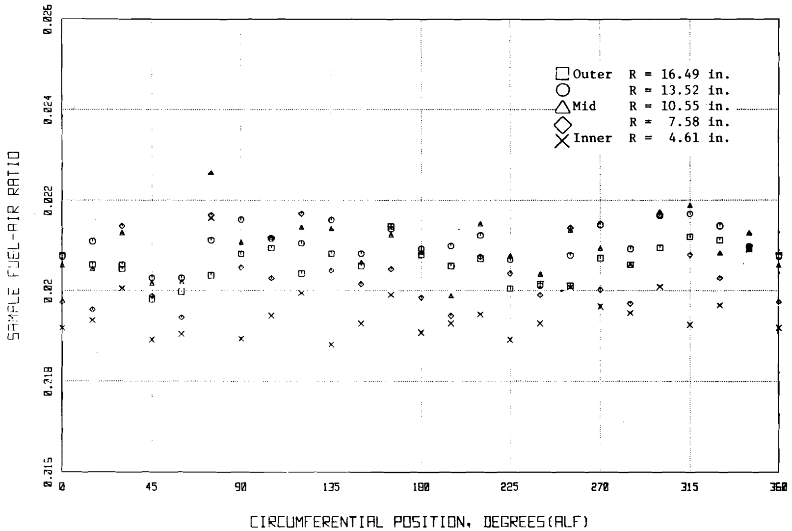
FIGURE 19. FUEL-AIR RATIO DISTRIBUTION AT 85 PERCENT POWER.
