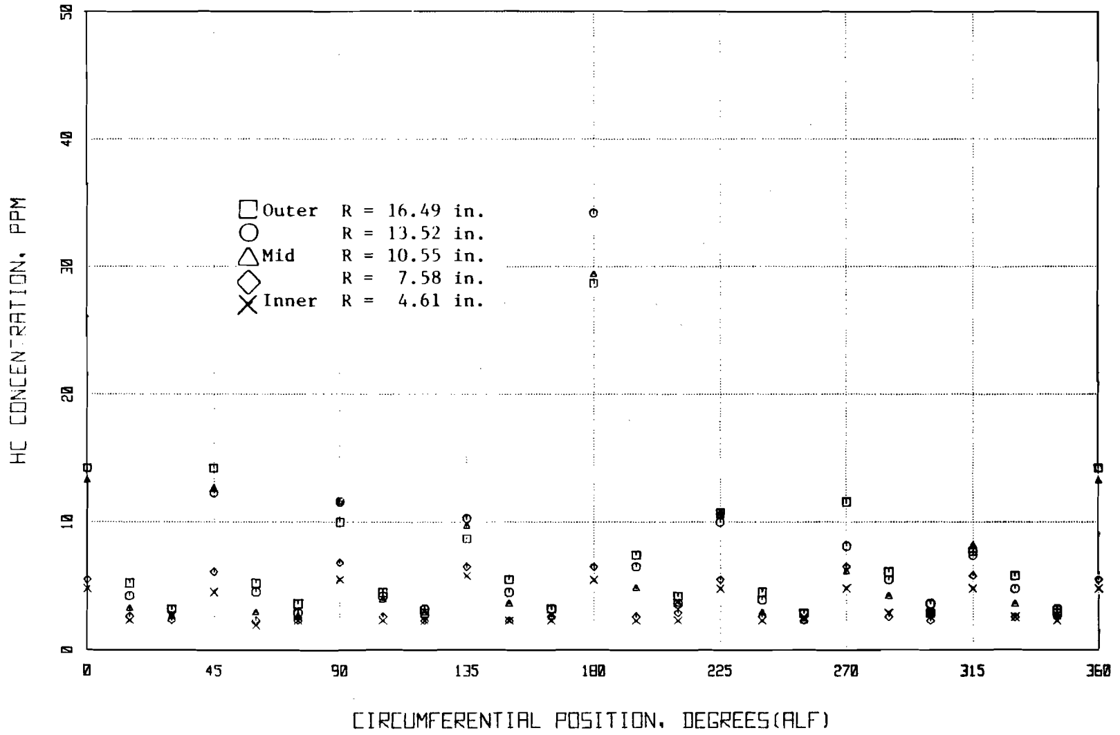
FIGURE 17. HC DISTRIBUTION AT 30 PERCENT POWER.
