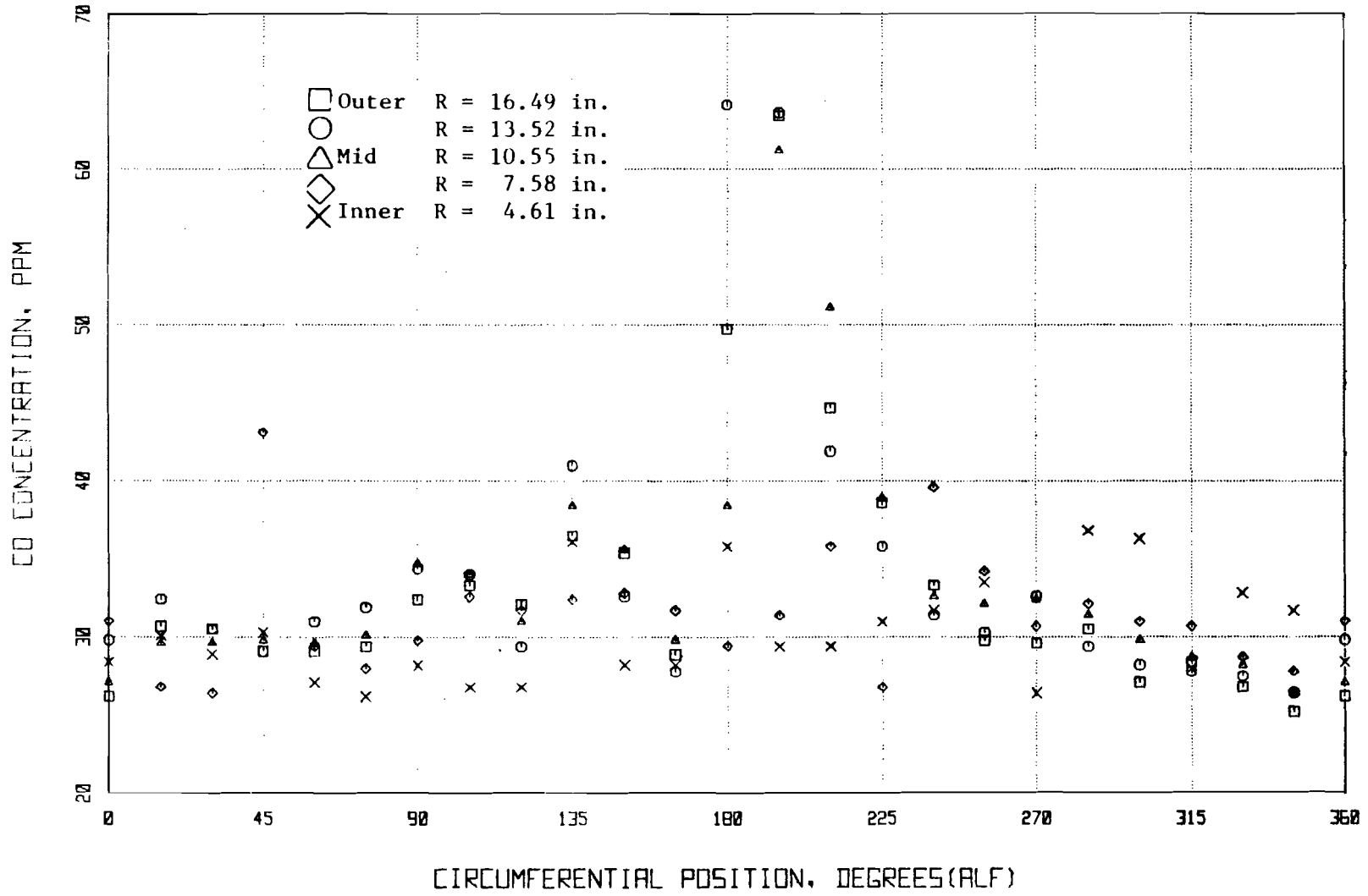
FIGURE 16. CO DISTRIBUTION AT 30 PERCENT POWER.
