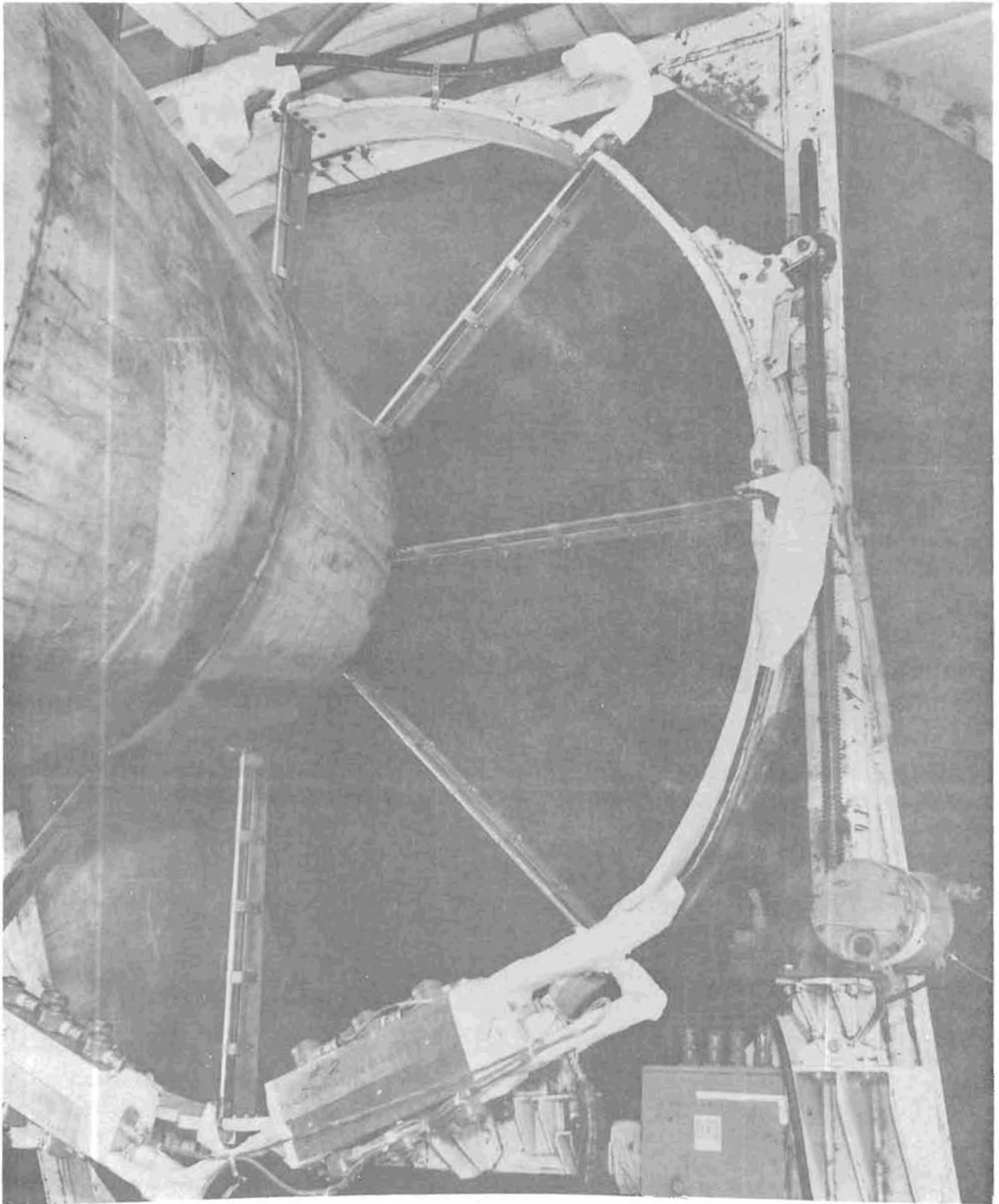
FIGURE 8. TRAVERSE PROBE SYSTEM MOUNTED BEHIND CF6-50 ENGINE IN TEST CELL.
