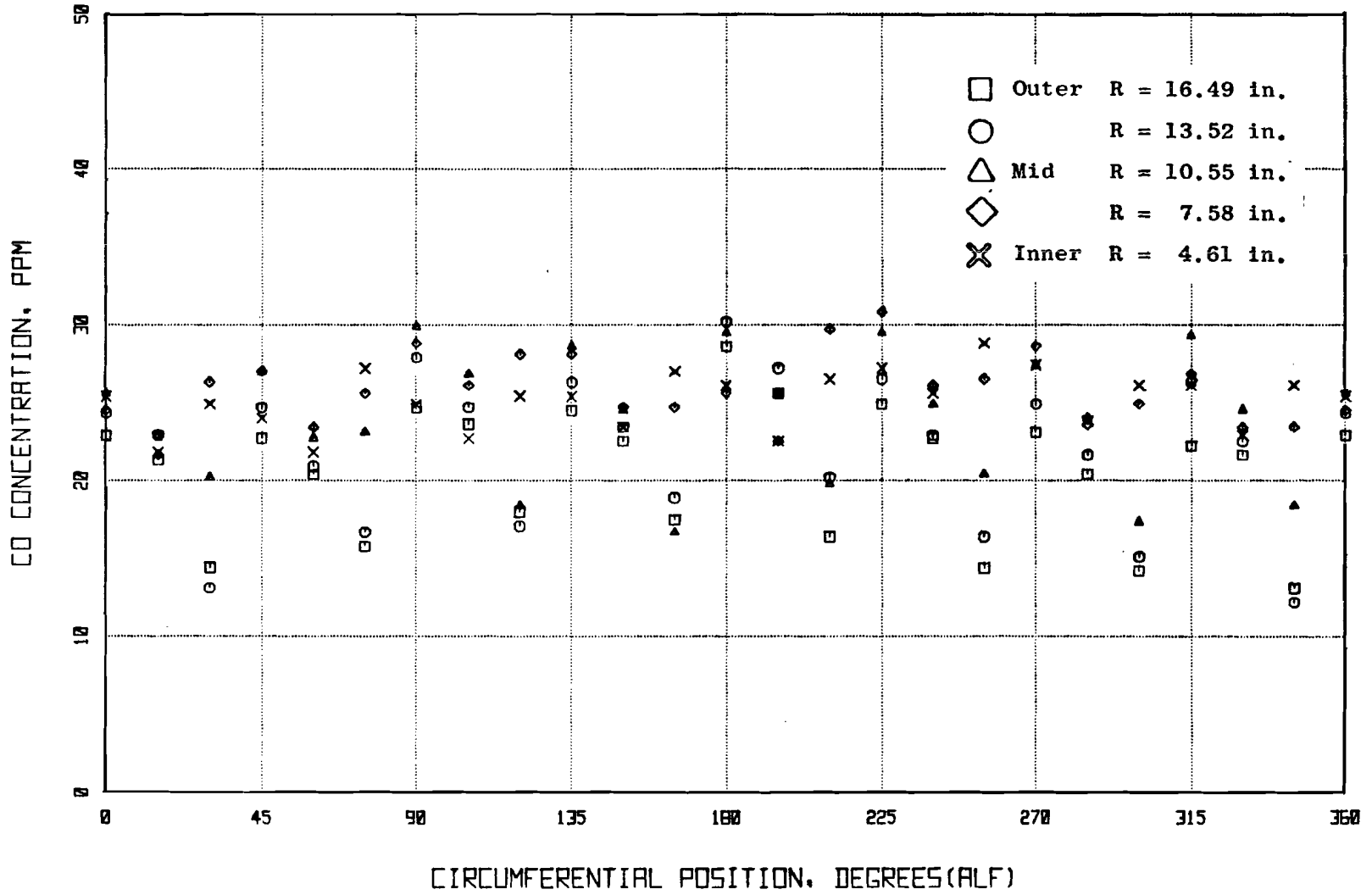
FIGURE 20. CO CONCENTRATION DISTRIBUTION AT 85 PERCENT POWER.
