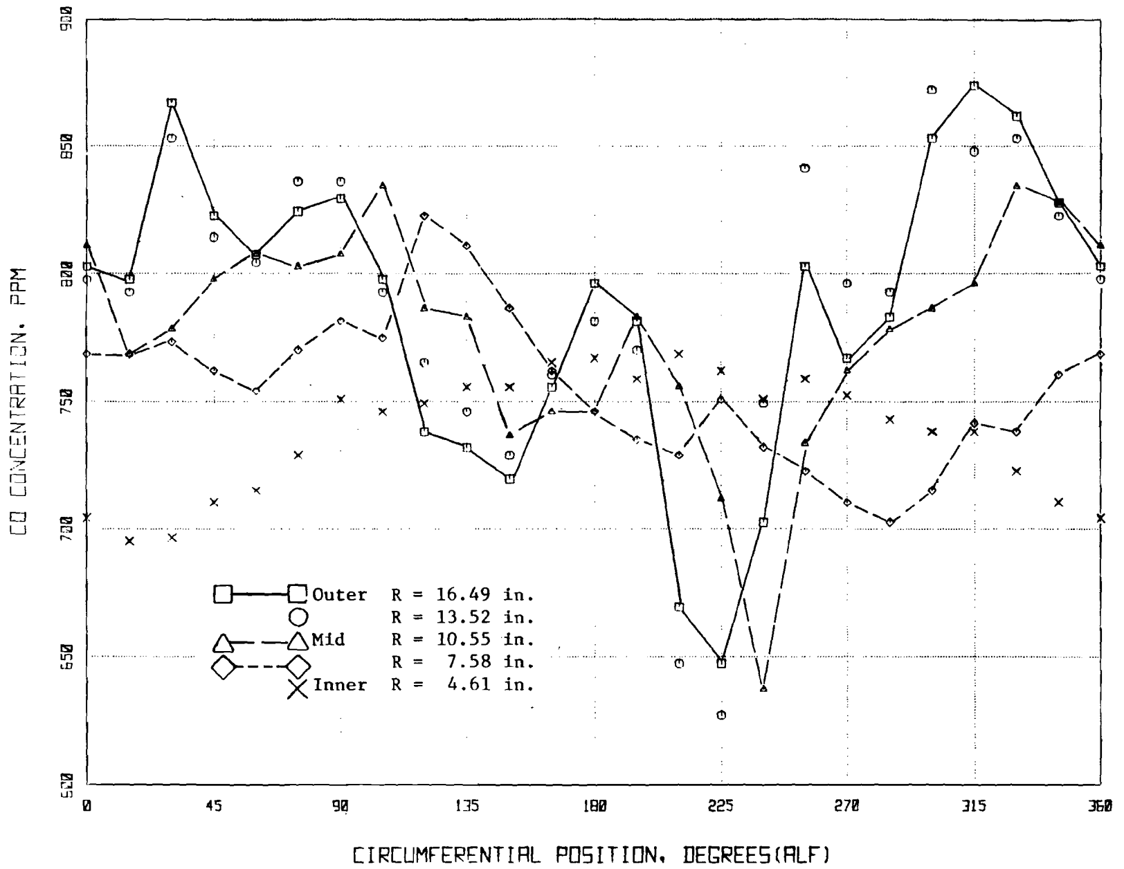
FIGURE 12. CO CONCENTRATION DISTRIBUTION AT IDLE POWER.
