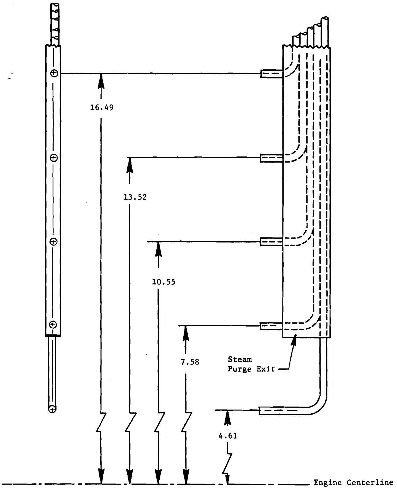
FIGURE 4. SAMPLE PORTS FOR TRAVERSE PROBE.
