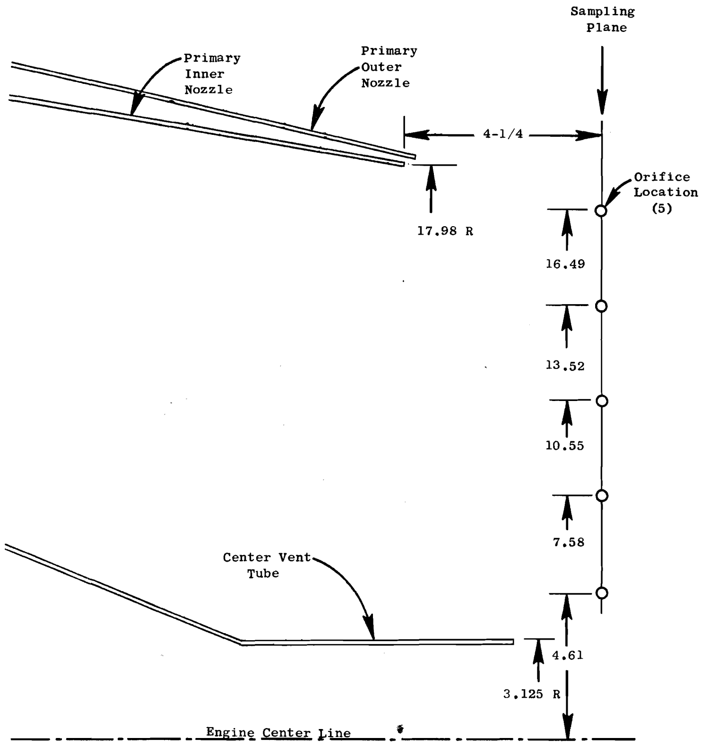
FIGURE 5. CF6-50 PRIMARY NOZZLE CONFIGURATION AND RADIAL SAMPLING LOCATIONS FOR TRAVERSE PROBE.
