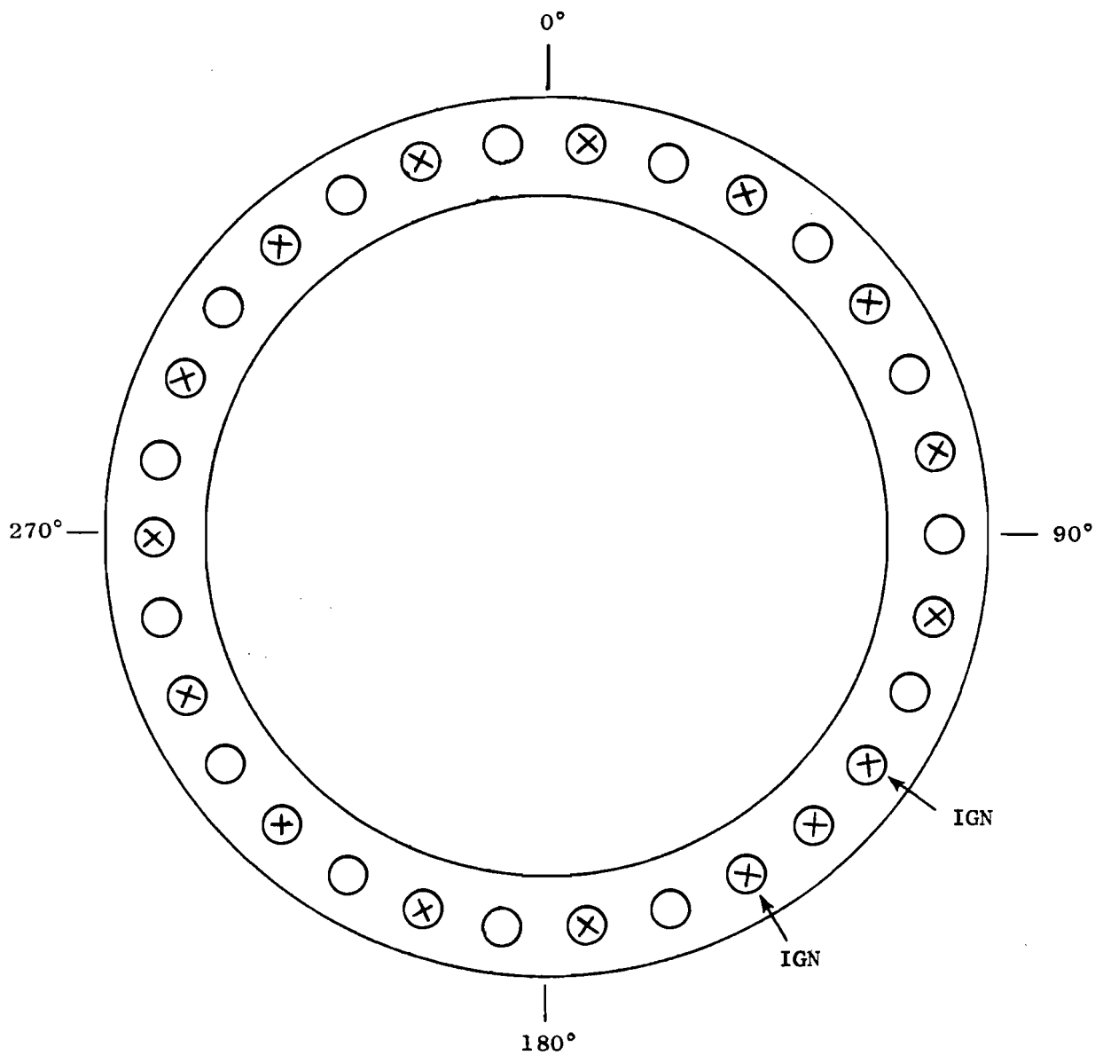
FIGURE 2. CF6-50 FUEL NOZZLE CONFIGURATION (AFT LOOKING FORWARD).
