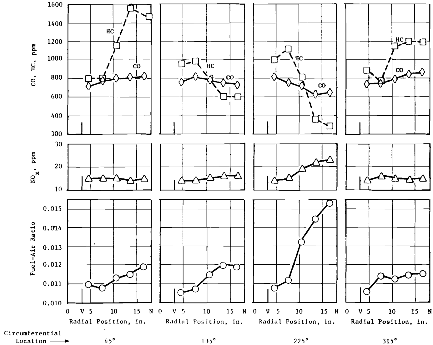
FIGURE 22. RADIAL PROFILES OF FUEL-AIR RATIO, CO, HC, AND NO x CONCENTRATIONS AT IDLE POWER AND FOR SELECTED CIRCUMFERENTIAL LOCATIONS. V AND N INDICATE VENT TUBE (R = 3.1 IN.) AND EXHAUST NOZZLE (R = 18.0 IN.) RADII.
