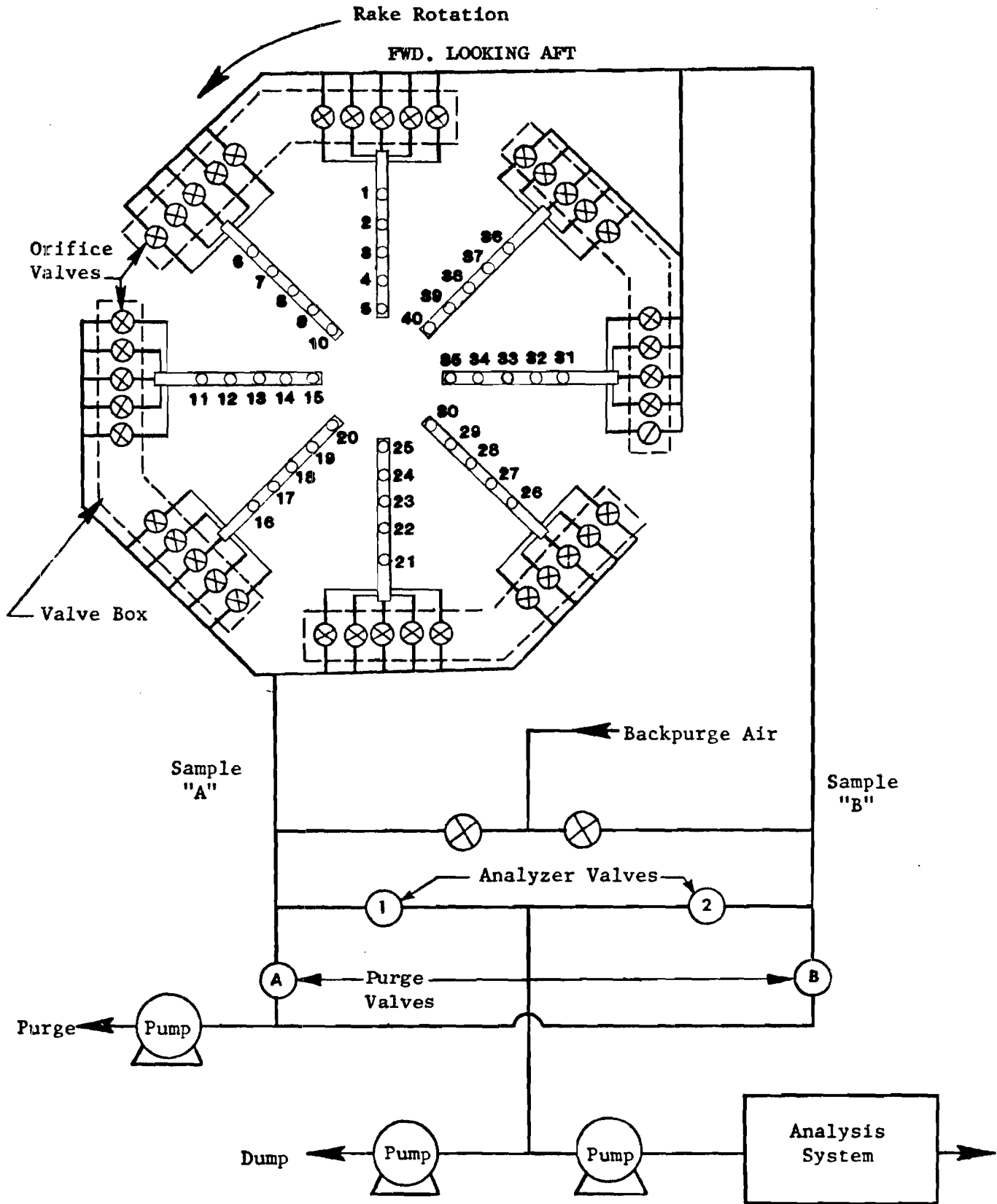
FIGURE 6. SAMPLING SYSTEM SCHEMATIC.
