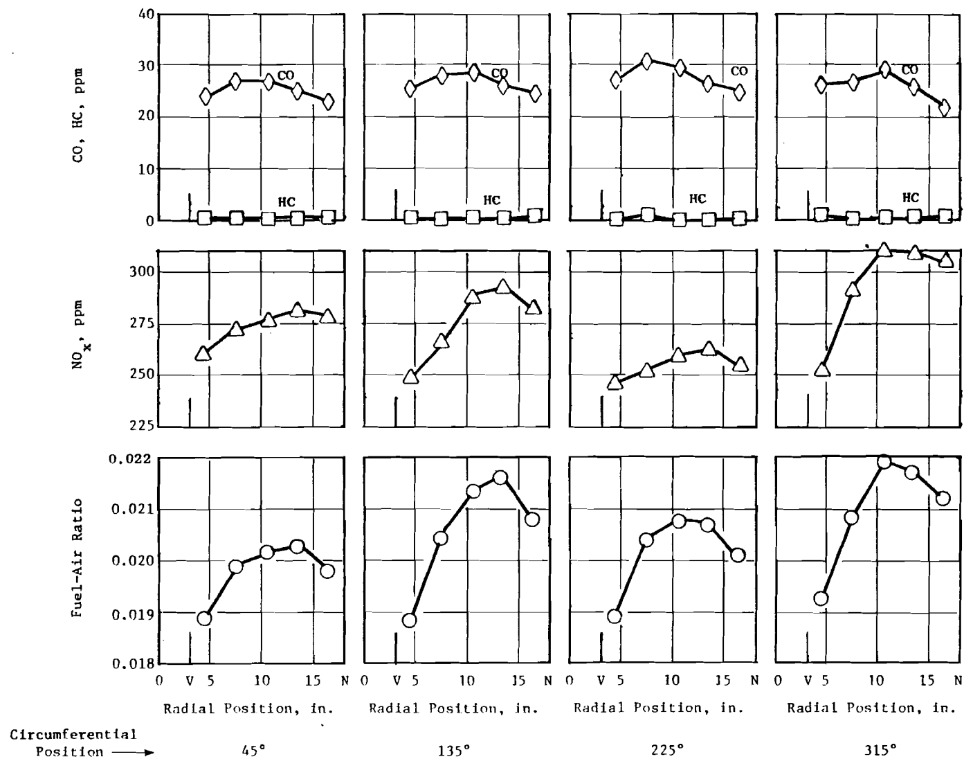
FIGURE 24. RADIAL PROFILES OF FUEL-AIR RATIO, CO, HC, AND NO x CONCENTRATIONS AT 85% POWER AND FOR SELECTED CIRCUMFERENTIAL LOCATIONS. V AND N INDICATE VENT TUBE (R = 3.1 IN.) AND EXHAUST NOZZLE (18.0 IN.) RADII.
