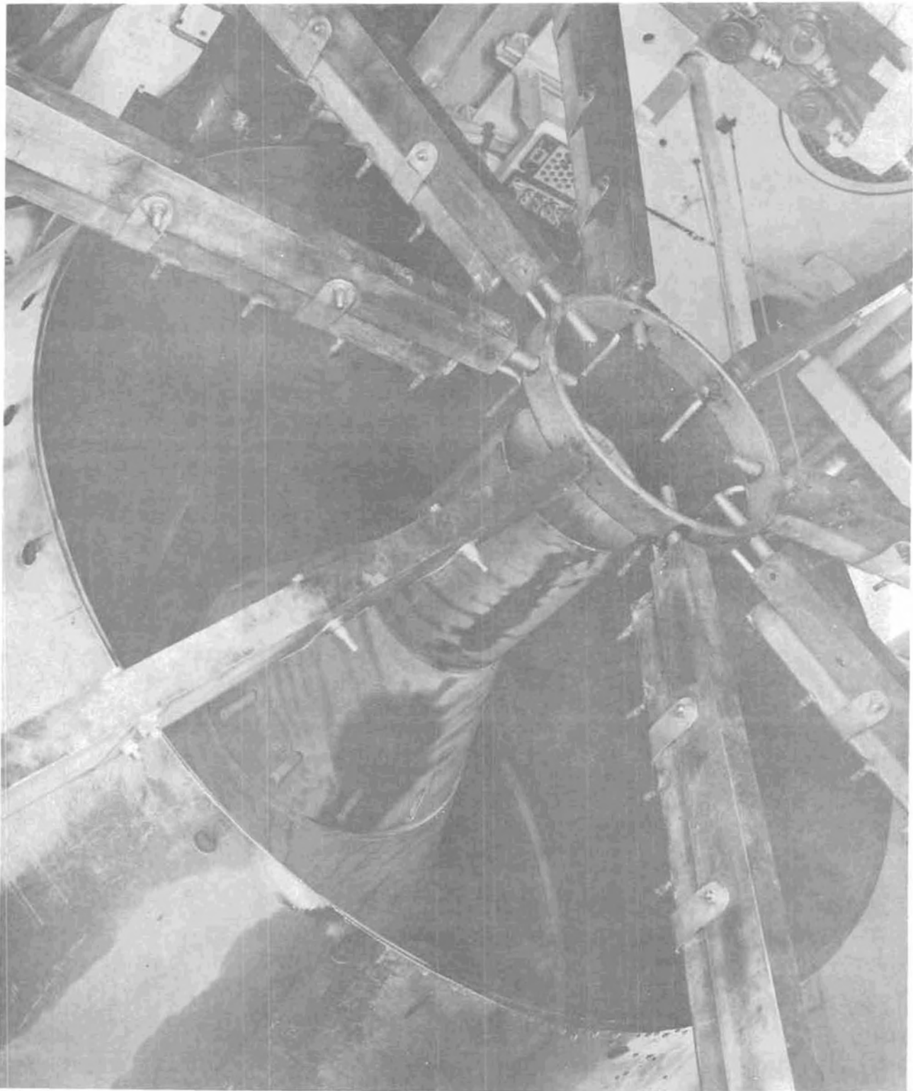
FIGURE 9. TRAVERSE PROBE SAMPLING ORIFICES IN POSITION TO SAMPLE CF6-50 EXHAUST.
