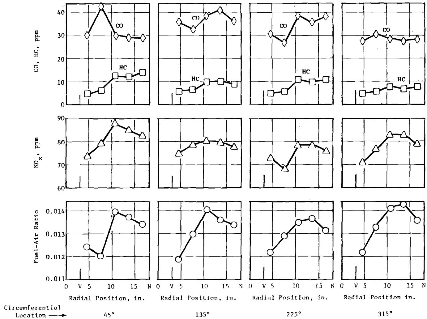
FIGURE 23. RADIAL PROFILES OF FUEL-AIR RATIO, CO, HC, AND NO x CONCENTRATIONS AT 30% POWER AND FOR SELECTED CIRCUMFERENTIAL LOCATIONS. V AND N INDICATE VENT TUBE (R = 3.1 IN.) AND EXHAUST NOZZLE (R = 18.0 IN.) RADII.
