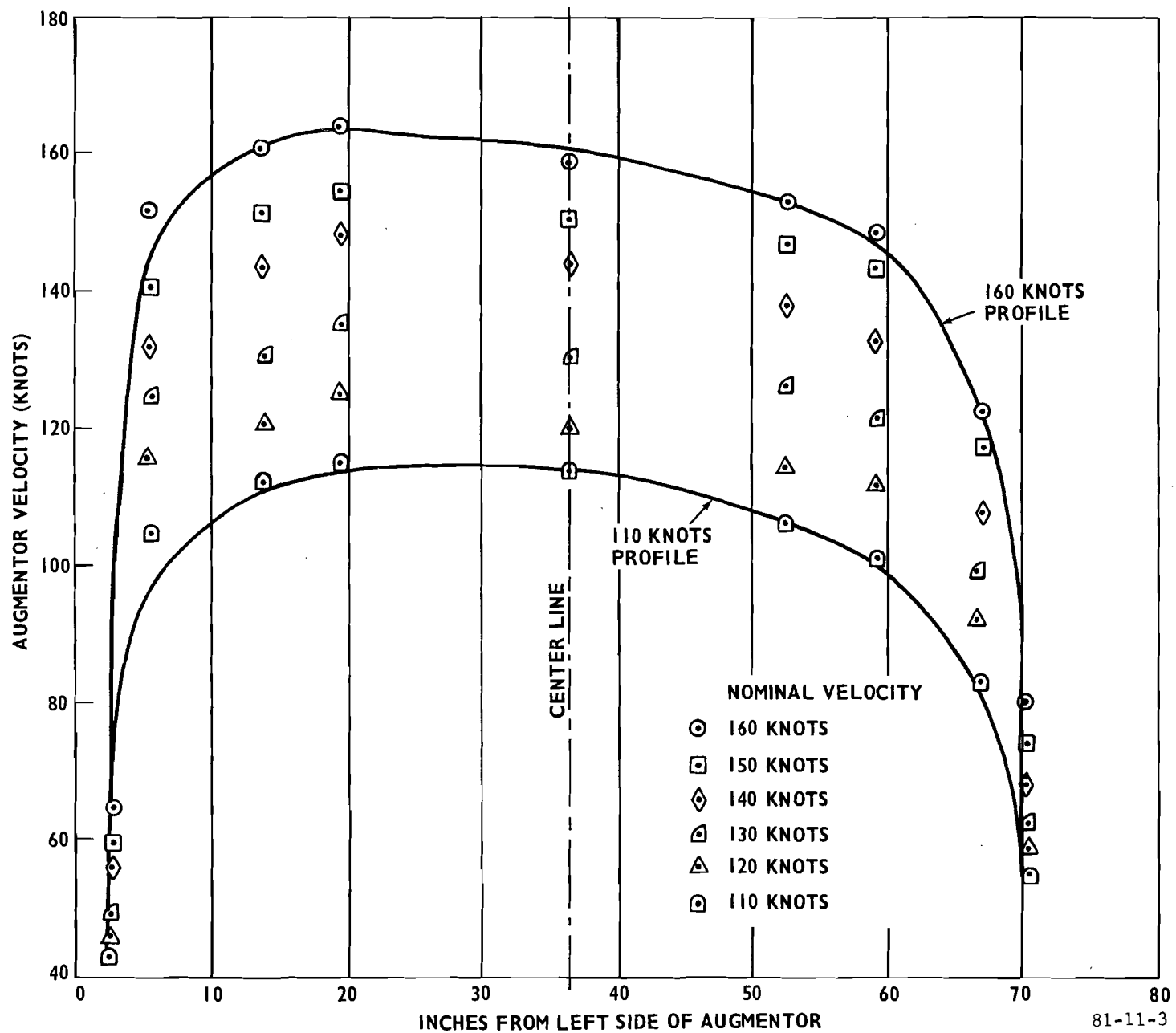
FIGURE 3. AUGMENTOR AIR VELOCITY AT HORIZONTAL CENTERLINE (21 FEET AFT)
