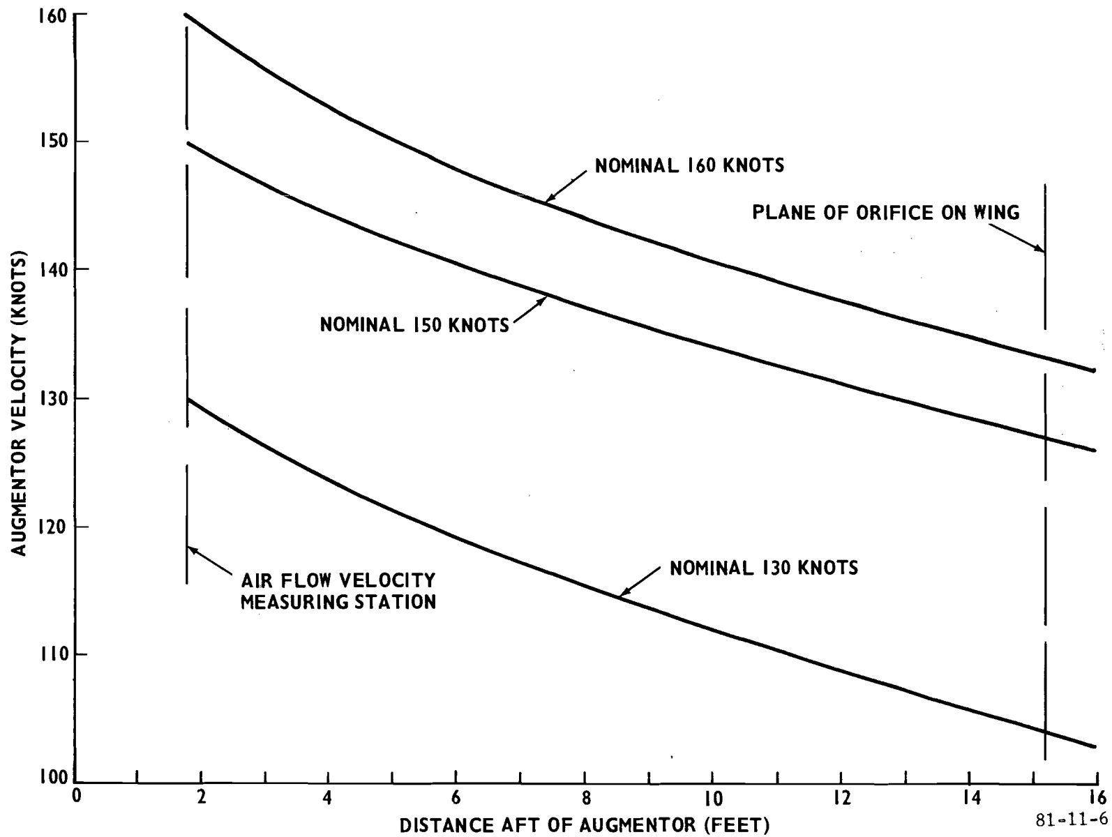
FIGURE 6. AUGMENTOR VELOCITY DECLINE VS. DISTANCE AFT OF EXIT
