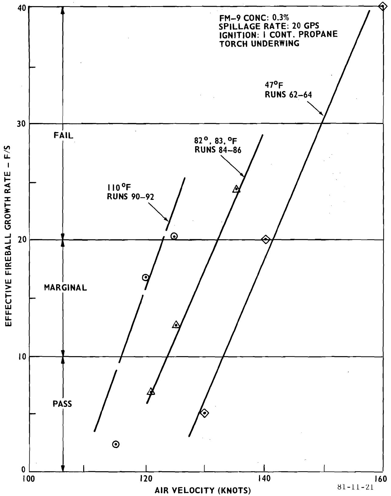
FIGURE 21. GROUP 4 RESULTS (FUEL TEMPERATURE)
