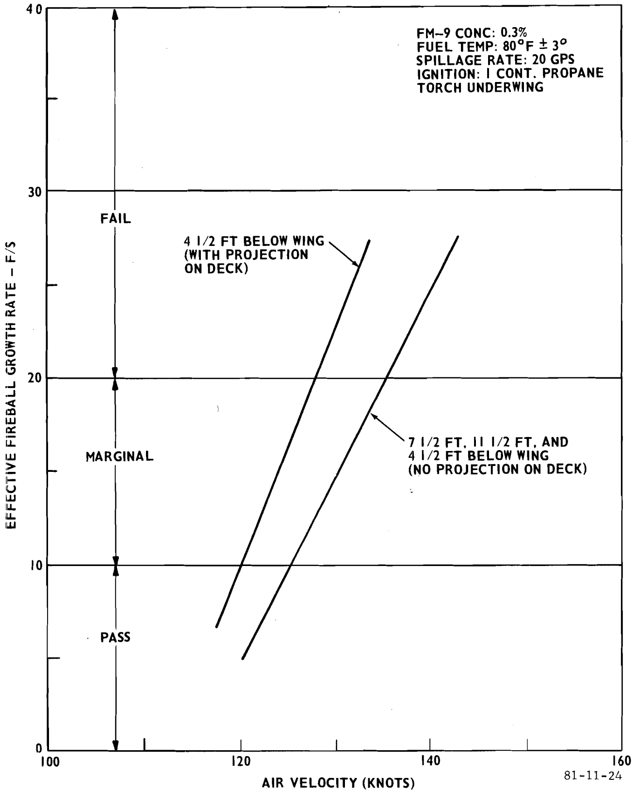
FIGURE 24. GROUP 7 RESULTS (GROUND LEVEL EFFECTS)
