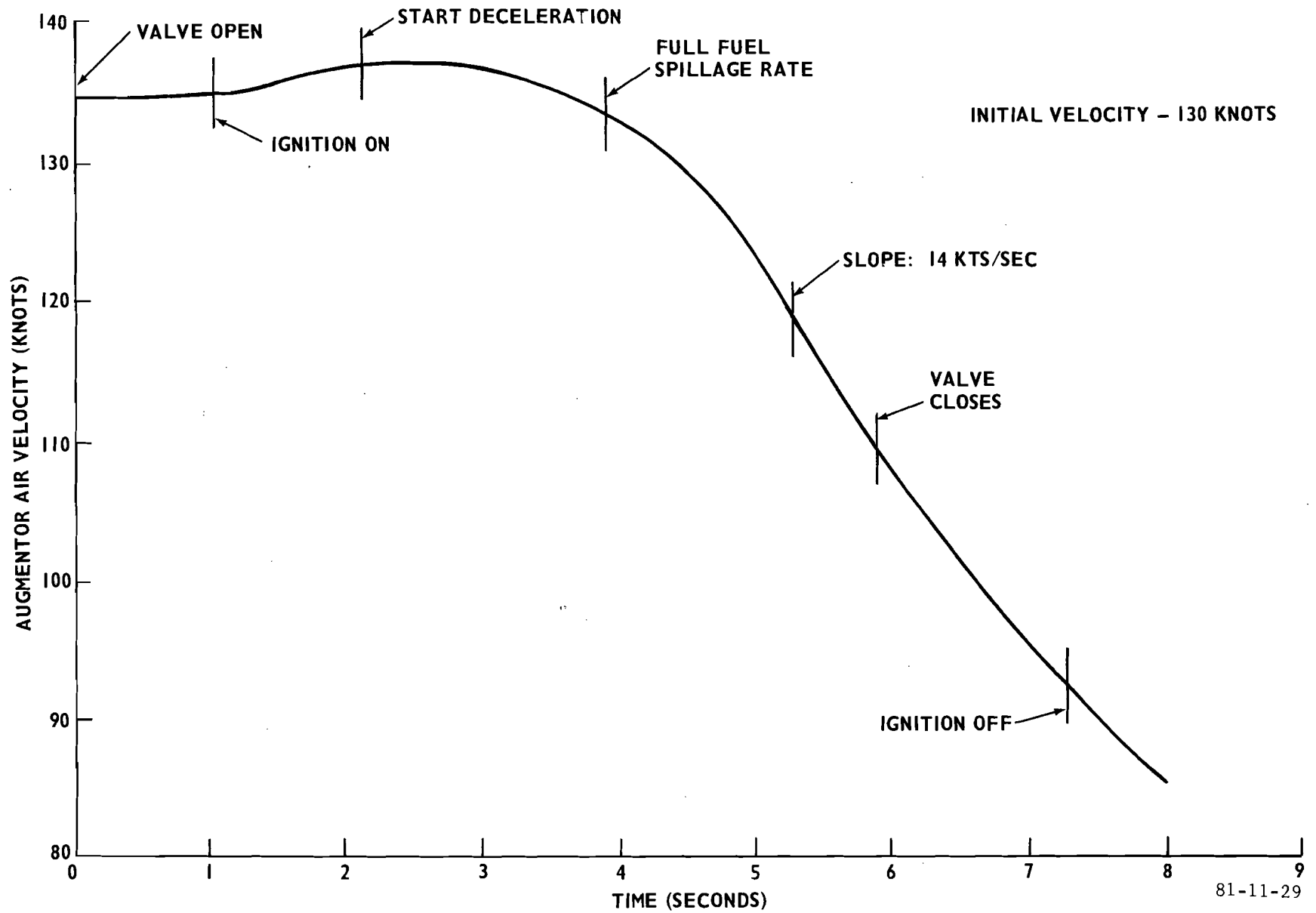
FIGURE 29. GROUP 10 DECELERATION CALIBRATION
