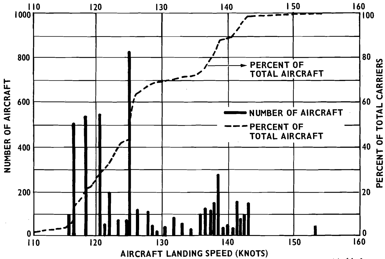
FIGURE 1. AIRCRAFT POPULATION VS. LANDING SPEED
