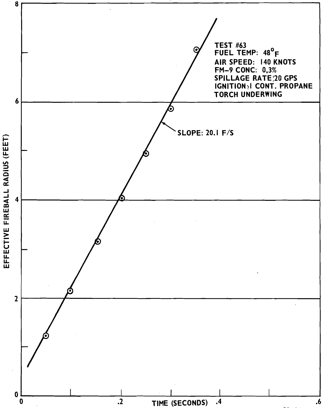
FIGURE 17. EFFECTIVE FIREBALL RADIUS VS. TIME (NO. 63)
