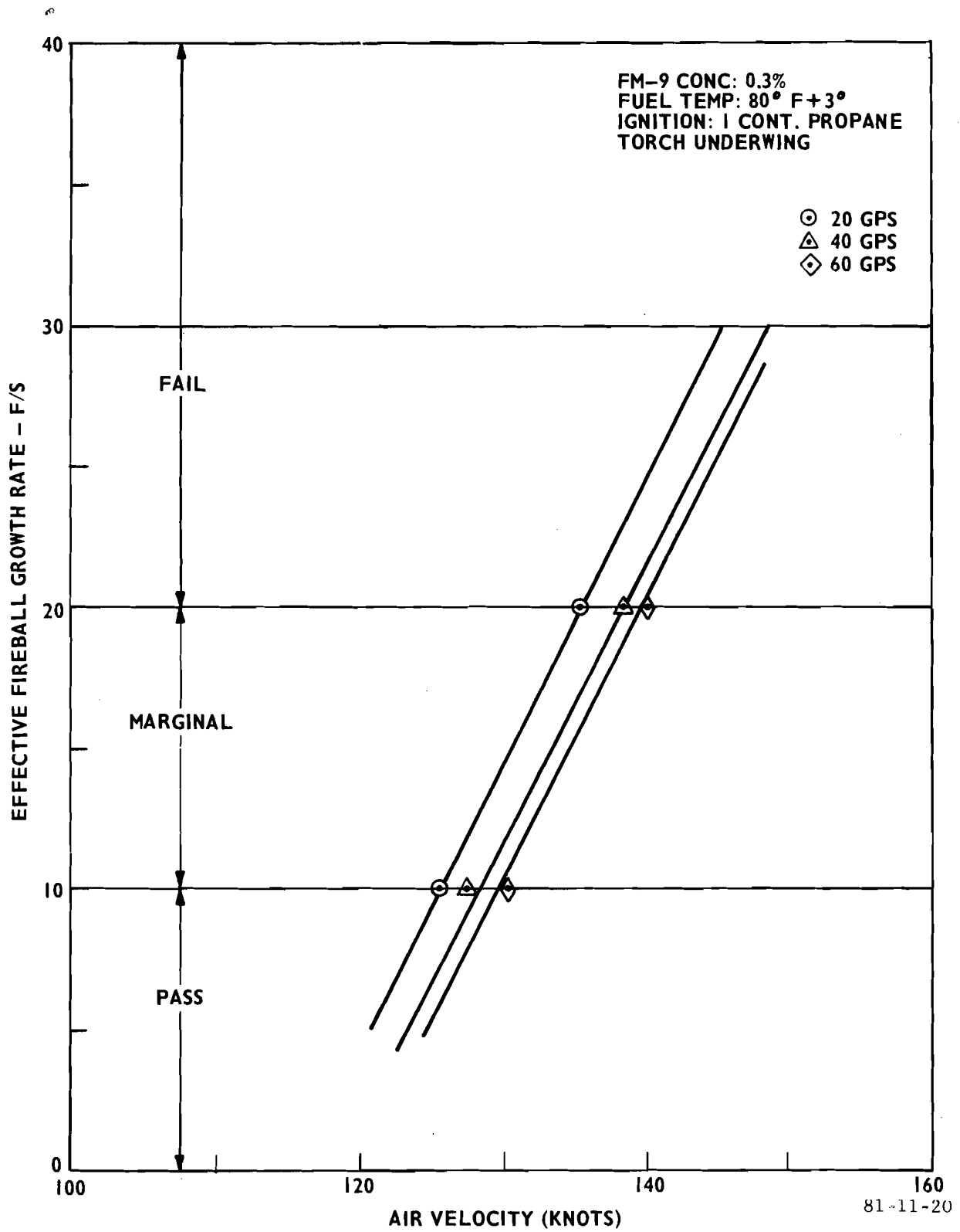
FIGURE 20. GROUP 3 RESULTS (SPILLAGE)
