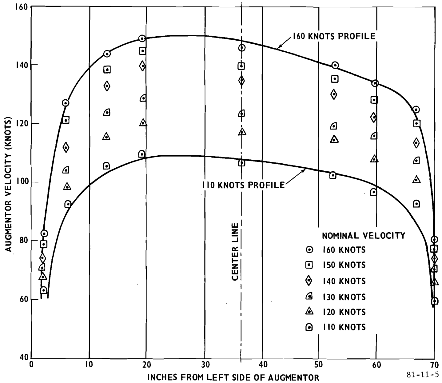
FIGURE 5. AUGMENTOR AIR VELOCITY AT HORIZONTAL CENTERLINE (93 FEET AFT)
