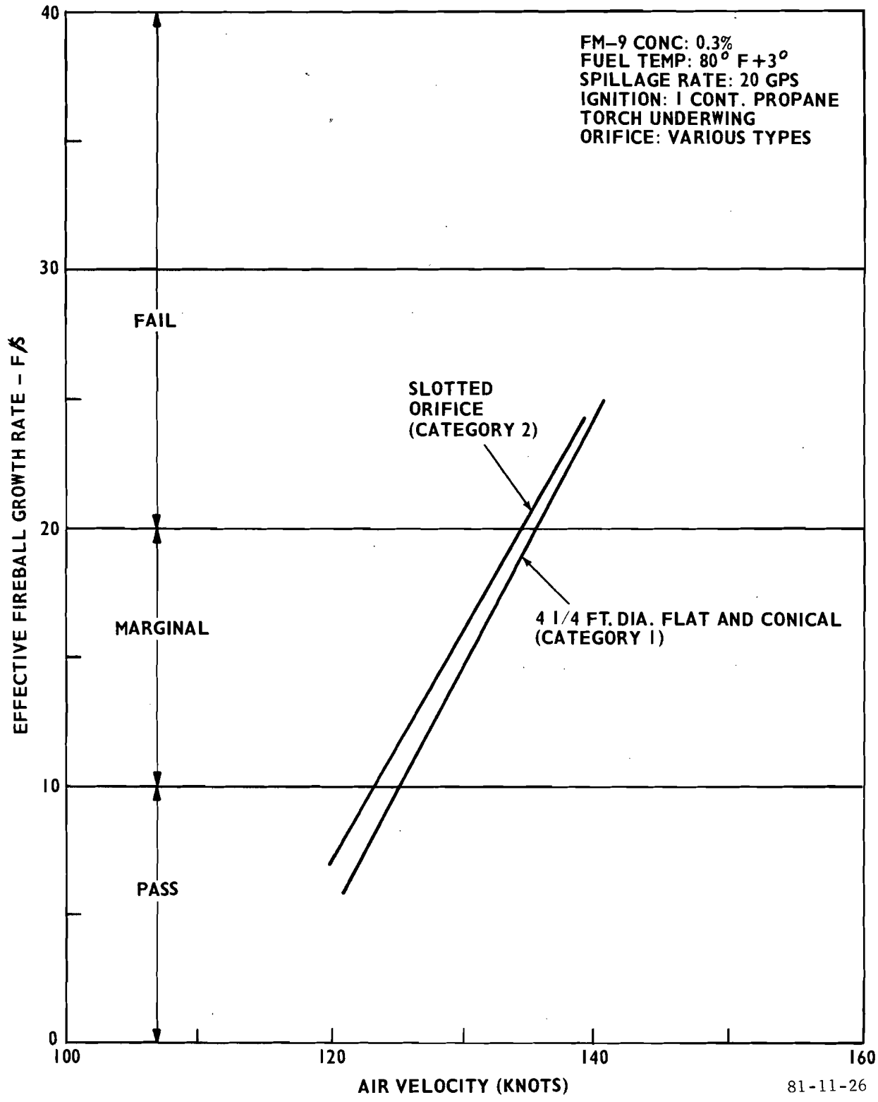
FIGURE 26. GROUP 8 RESULTS (ORIFICE CONFIGURATION)
