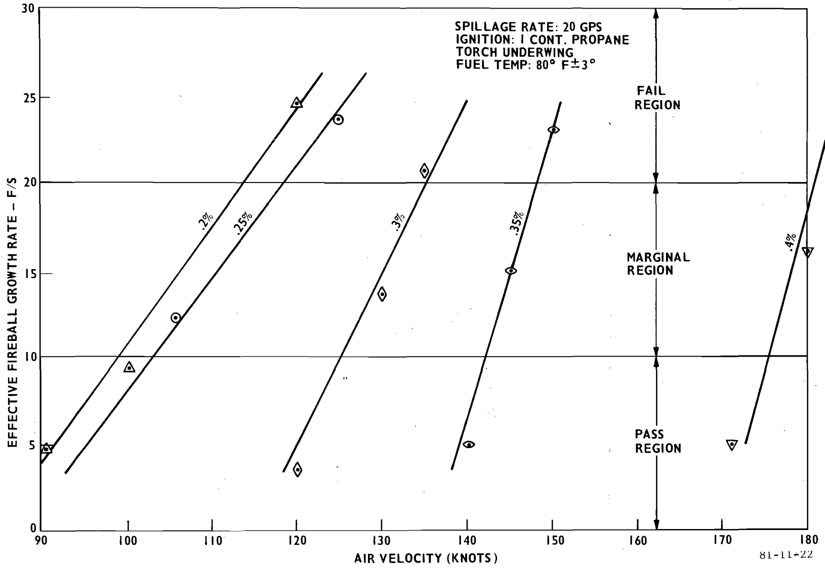
FIGURE 22. GROUP 5 RESULTS (FUEL ADDITIVE CONCENTRATION)
