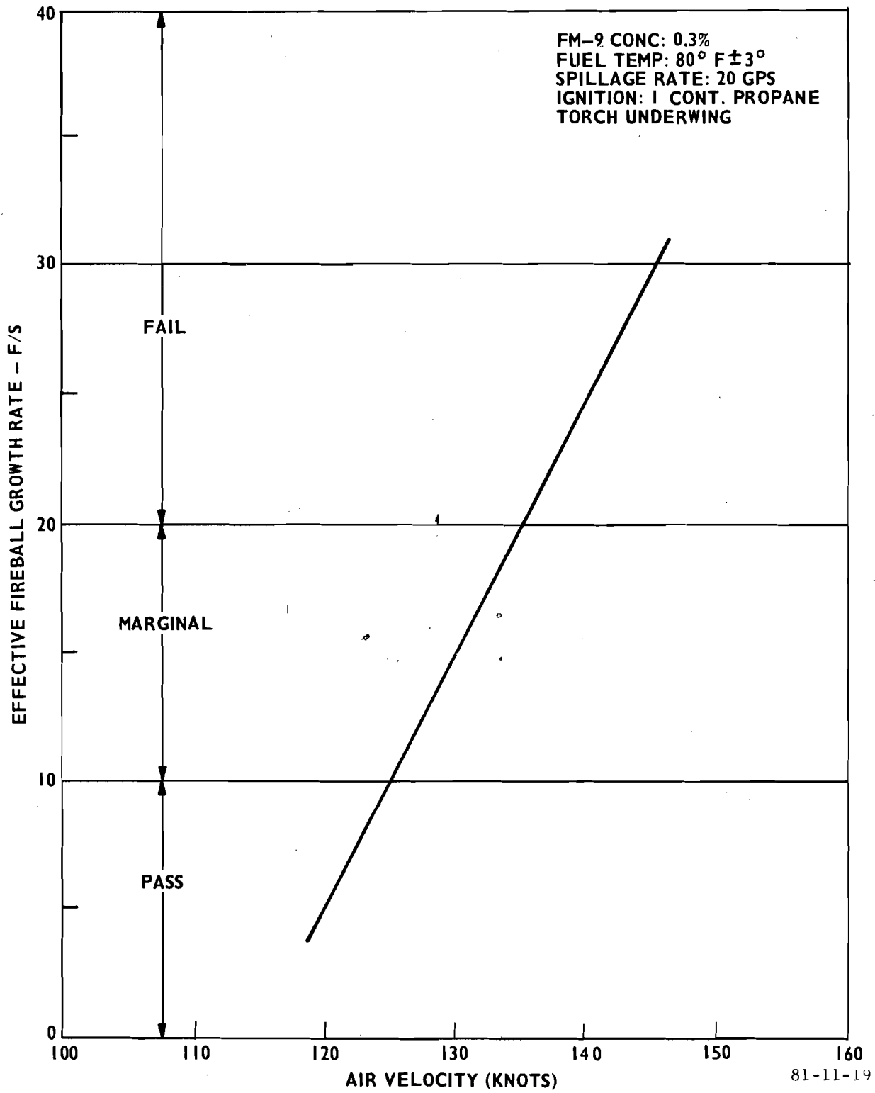
FIGURE 19. GROUP 2 RESULTS (VELOCITY)
