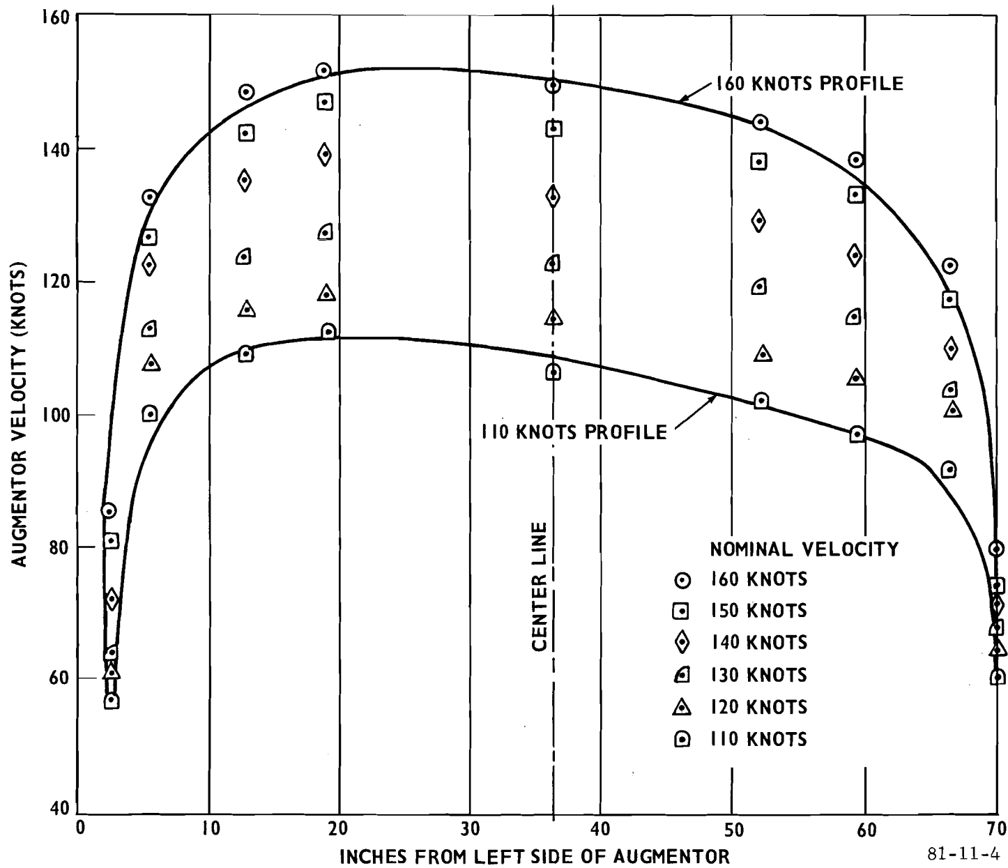
FIGURE 4. AUGMENTOR AIR VELOCITY AT HORIZONTAL CENTERLINE (57 FEET AFT)
