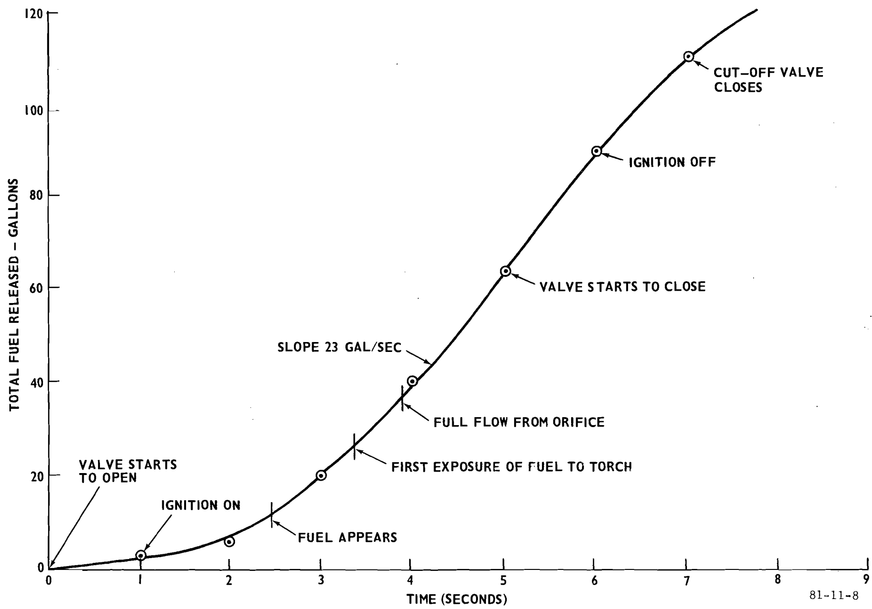
FIGURE 8. FUEL SPILLAGE VS. TIME (20 GALLONS PER SECOND)
