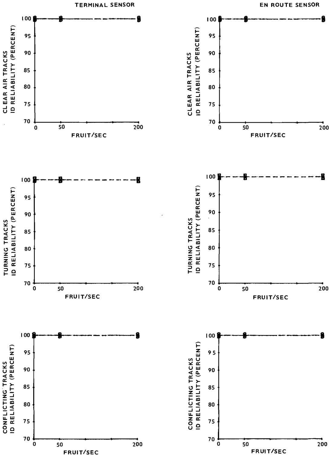
FIGURE 18. ID RELIABILITY (MODE S) TERMINAL VERSUS EN ROUTE SENSOR, EFFECTIVE BEAM WIDTH 3.4°
