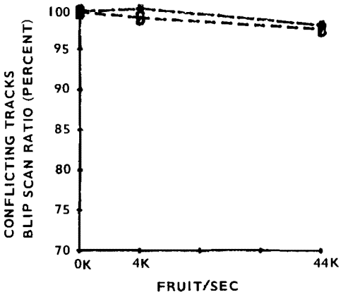
FIGURE 25. BLIP SCAN RATIO (ATCRBS) TERMINAL VERSUS EN ROUTE SENSOR, EFFECTIVE BEAM WIDTH 3.4°
