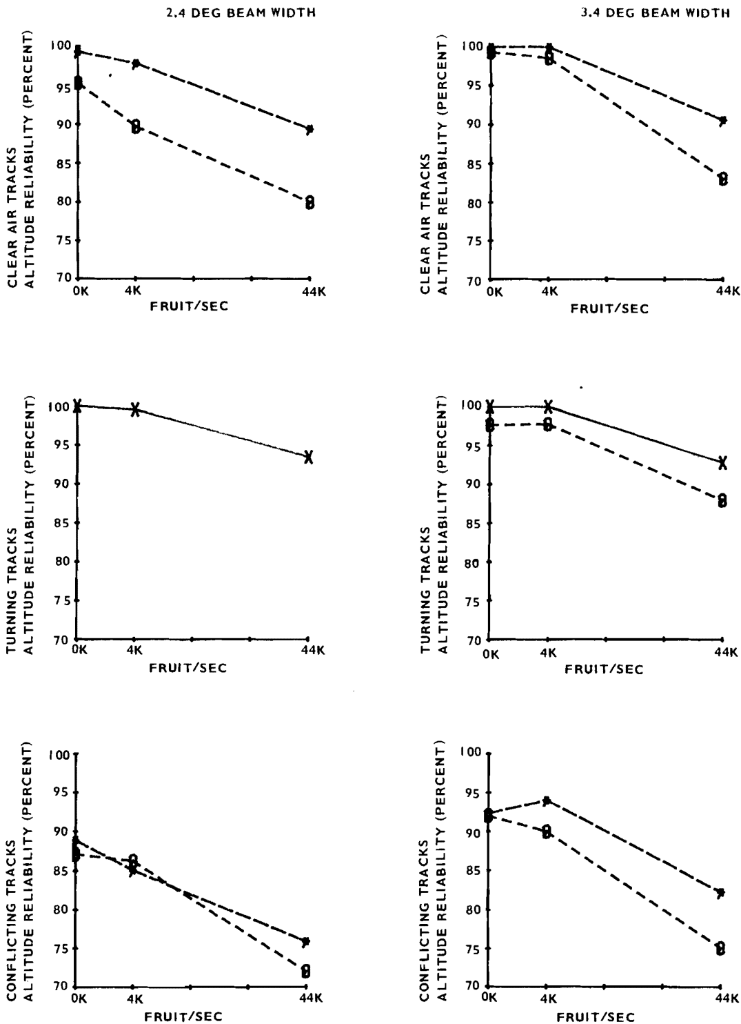
FIGURE 12. ALTITUDE RELIABILITY (ATCRBS) TERMINAL SENSOR, EFFECTIVE BEAM WIDTH 2.4° VERSUS 3.4°
