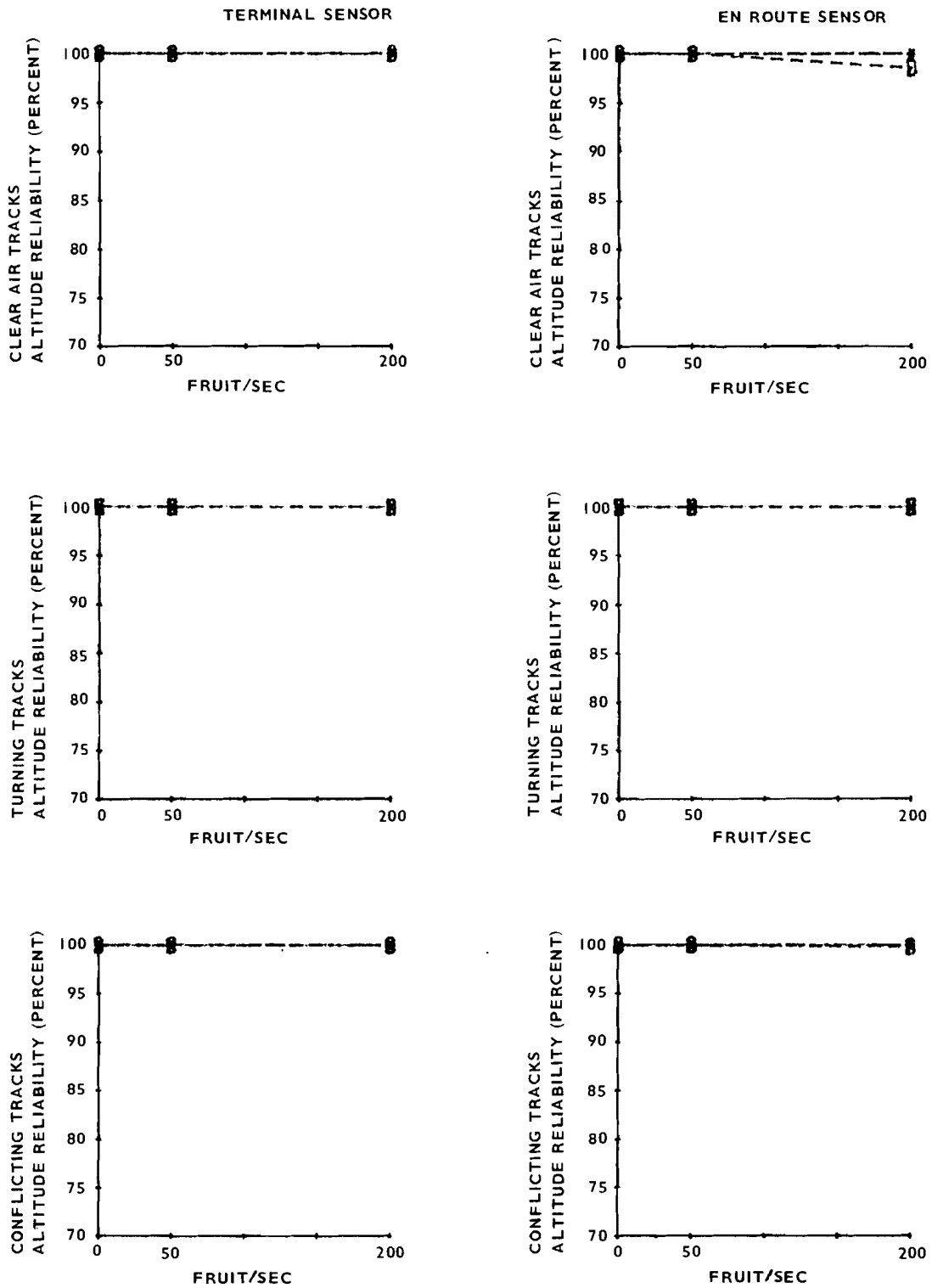
FIGURE 20. ALTITUDE RELIABILITY (MODE S) TERMINAL VERSUS EN ROUTE SENSOR, EFFECTIVE BEAM WIDTH 3.4°
