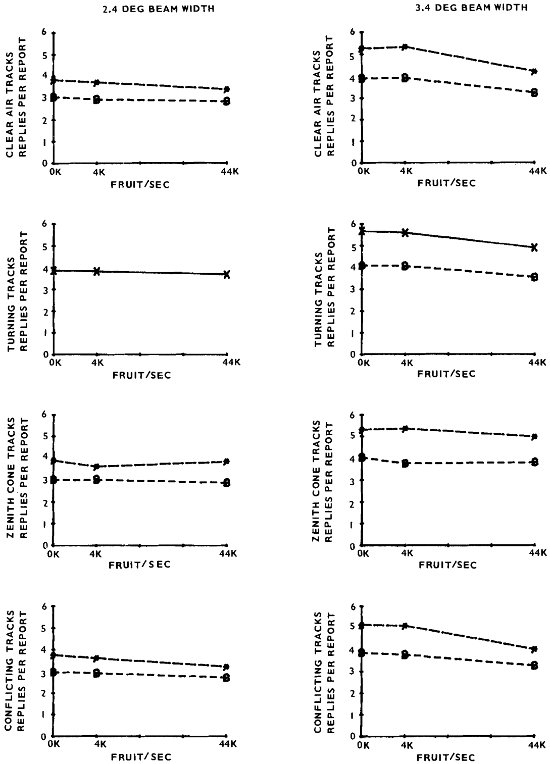
FIGURE 13. REPLIES PER REPORT (ATCRBS) TERMINAL SENSOR, EFFECTIVE BEAM WIDTH 2.4° VERSUS 3.4°
