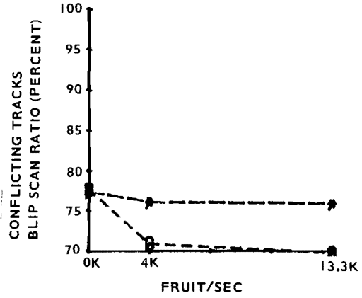
FIGURE 25. BLIP SCAN RATIO (ATCRBS) TERMINAL VERSUS EN ROUTE SENSOR, EFFECTIVE BEAM WIDTH 3.4°
