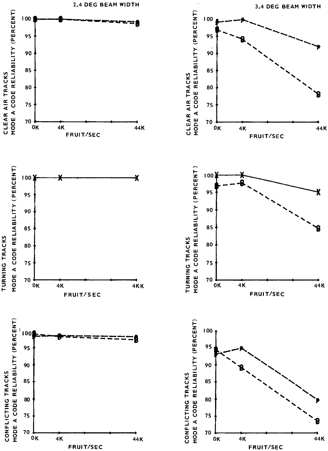
FIGURE 11. MODE 3/A CODE RELIABILITY (ATCRBS) TERMINAL SENSOR, EFFECTIVE BEAM WIDTH 2.4° VERSUS 3.4°
