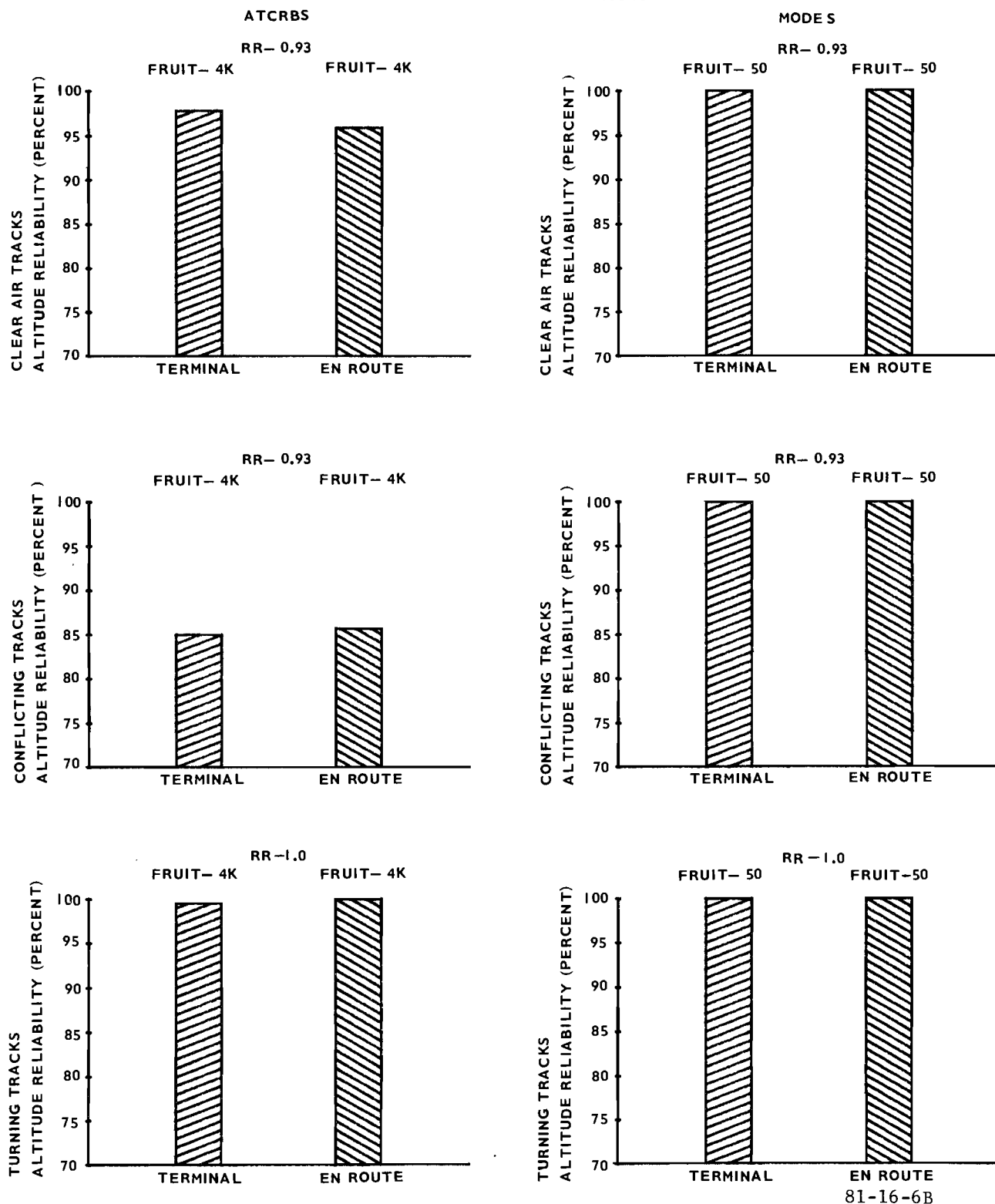
FIGURE 6. ALTITUDE RELIABILITY — TERMINAL VERSUS EN ROUTE SENSOR, EFFECTIVE RECEIVE BEAM WIDTH 2.4^\circ (Sheet 2 of 3)
