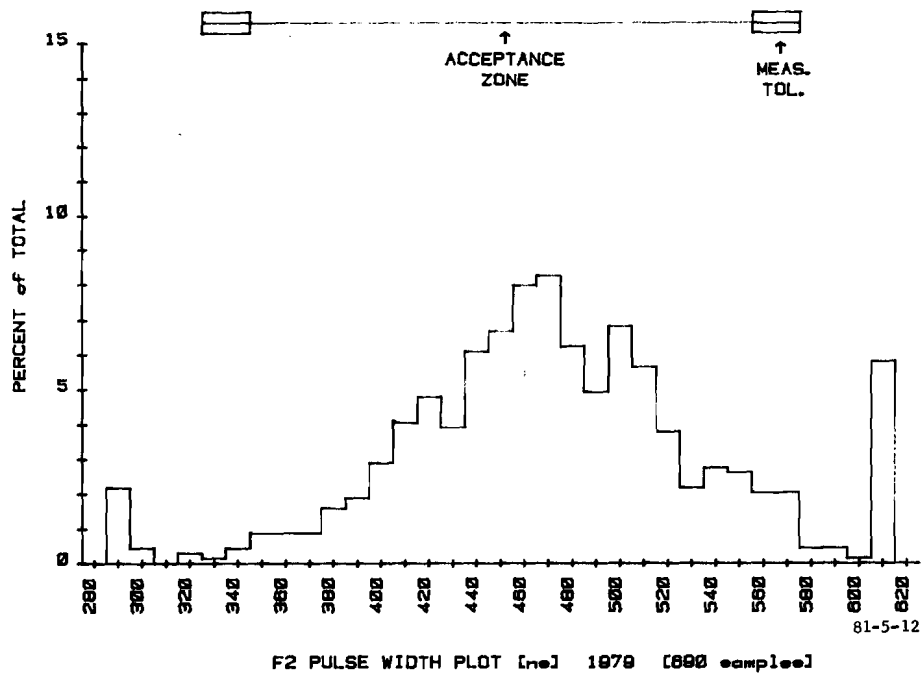
FIGURE 12. F 1 PULSE Width (ns) (690 SAMPLES, 1979)
