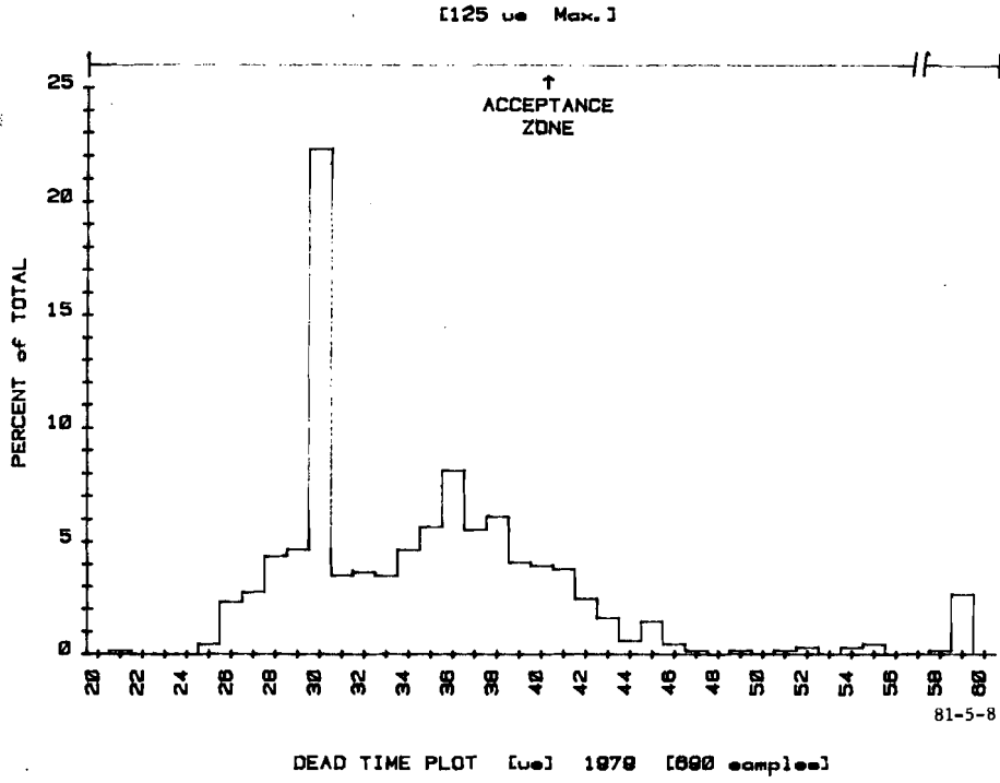
FIGURE 8. DEAD TIME ( \mu\text{s} ) (690 SAMPLES, 1979)
