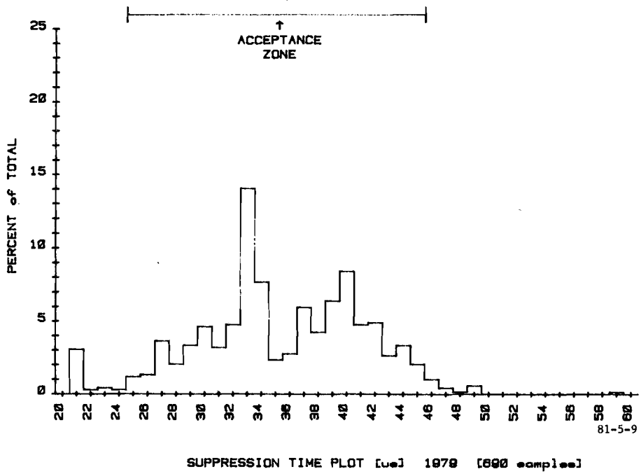
FIGURE 9. SUPPRESSION TIME ( \mu\text{s} ) (690 SAMPLES, 1979)
