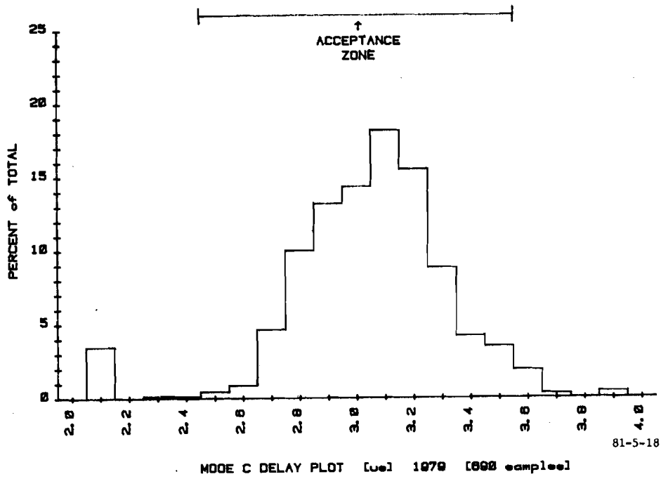
FIGURE 18. MODE C TIME DELAY ( \mu s ) (690 SAMPLES, 1979)
