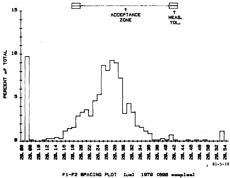
FIGURE 19. F_1 - F_2 SPACING ( \mu s ) (690 SAMPLES, 1979)
