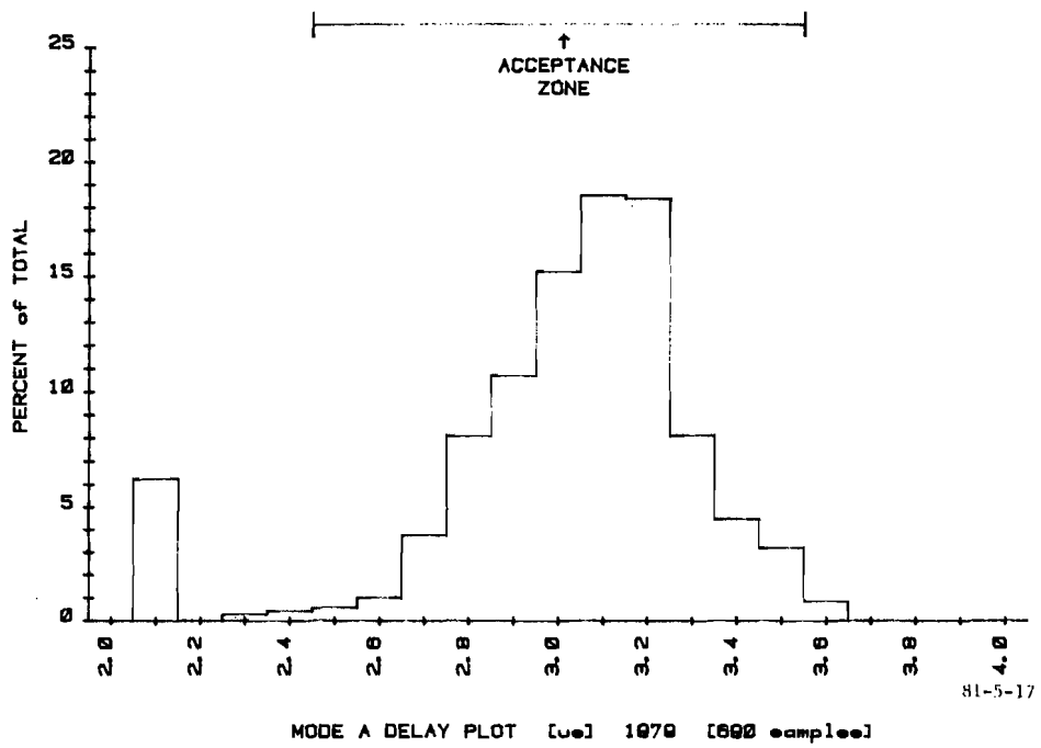
FIGURE 17. MODE A TIME DELAY ( \mu s ) (690 SAMPLES, 1979)
