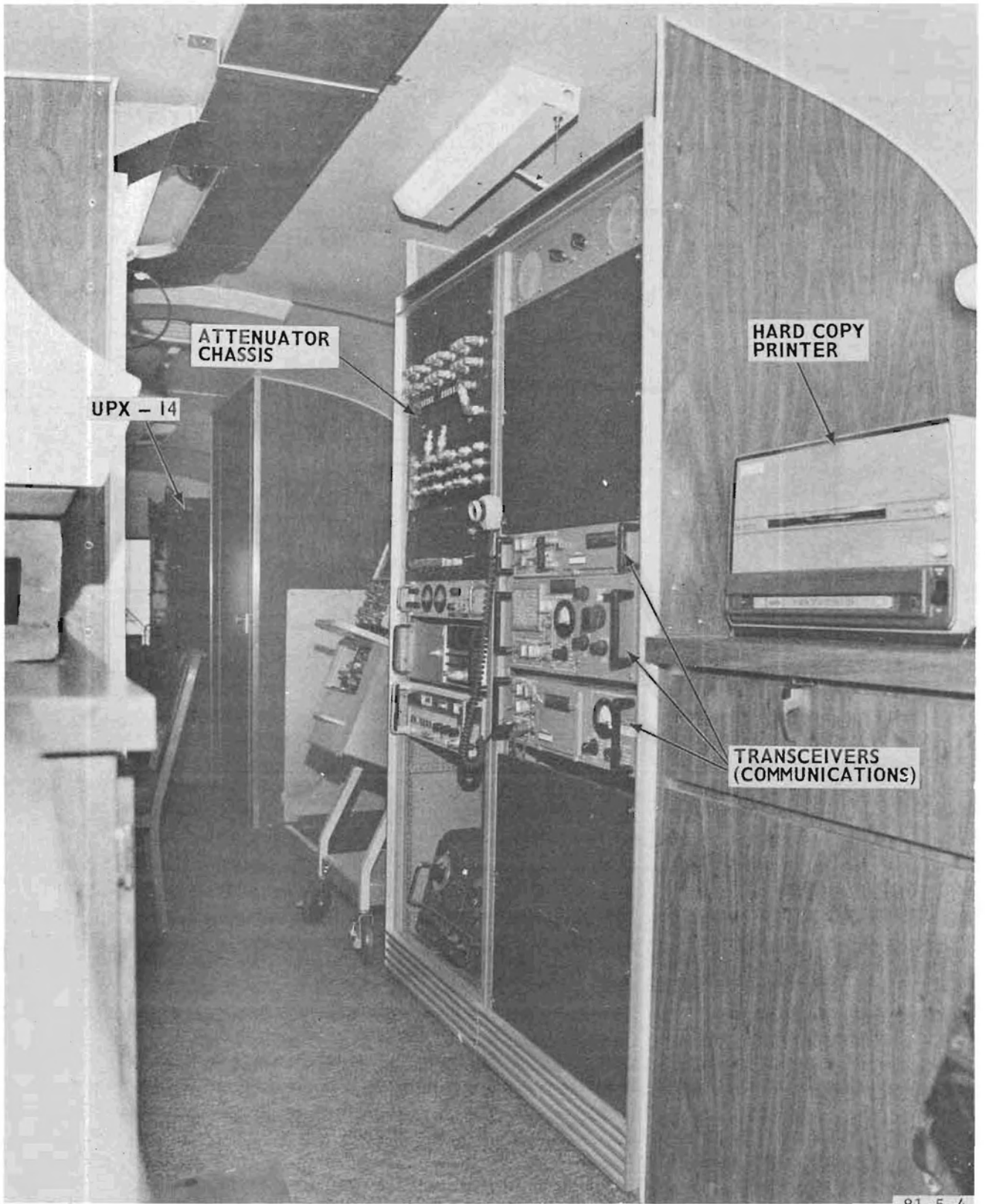
FIGURE 4. INTERIOR OF TPA BUS (RIGHT CENTER)
