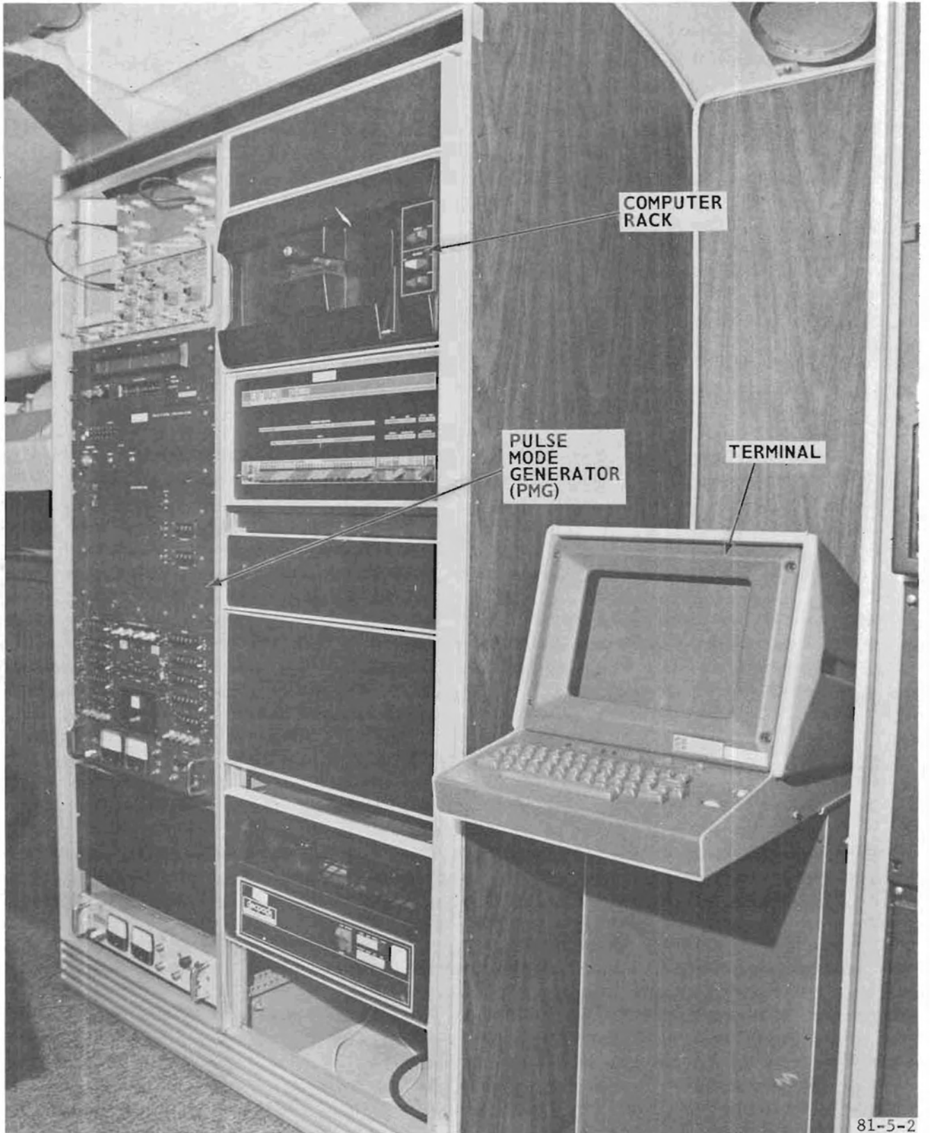
FIGURE 2. INTERIOR OF TPA BUS (LEFT CENTER)
