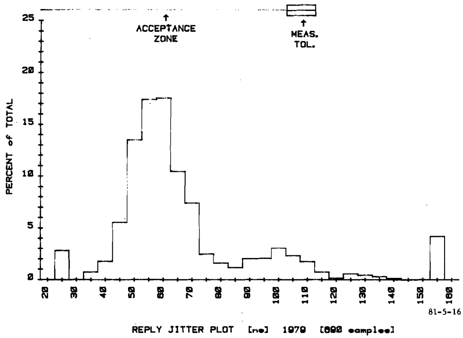
FIGURE 16. REPLY JITTER (ns) (690 SAMPLES, 1979)
