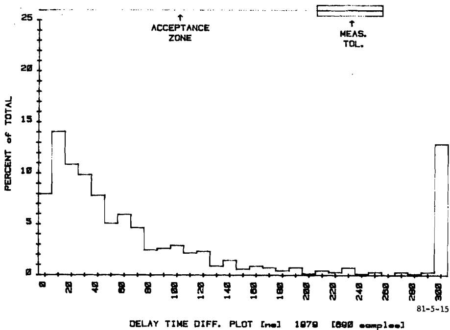
FIGURE 15. DELAY TIME DIFFERENCE (ns) (690 SAMPLES, 1979)
