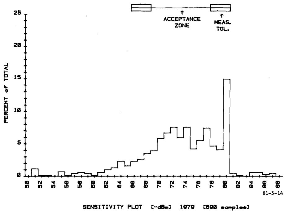
FIGURE 14. SENSITIVITY (-dBm) (690 SAMPLES, 1979)
