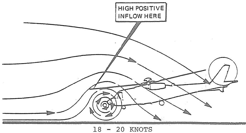
FIGURE 2-3. GROUND VORTEX
