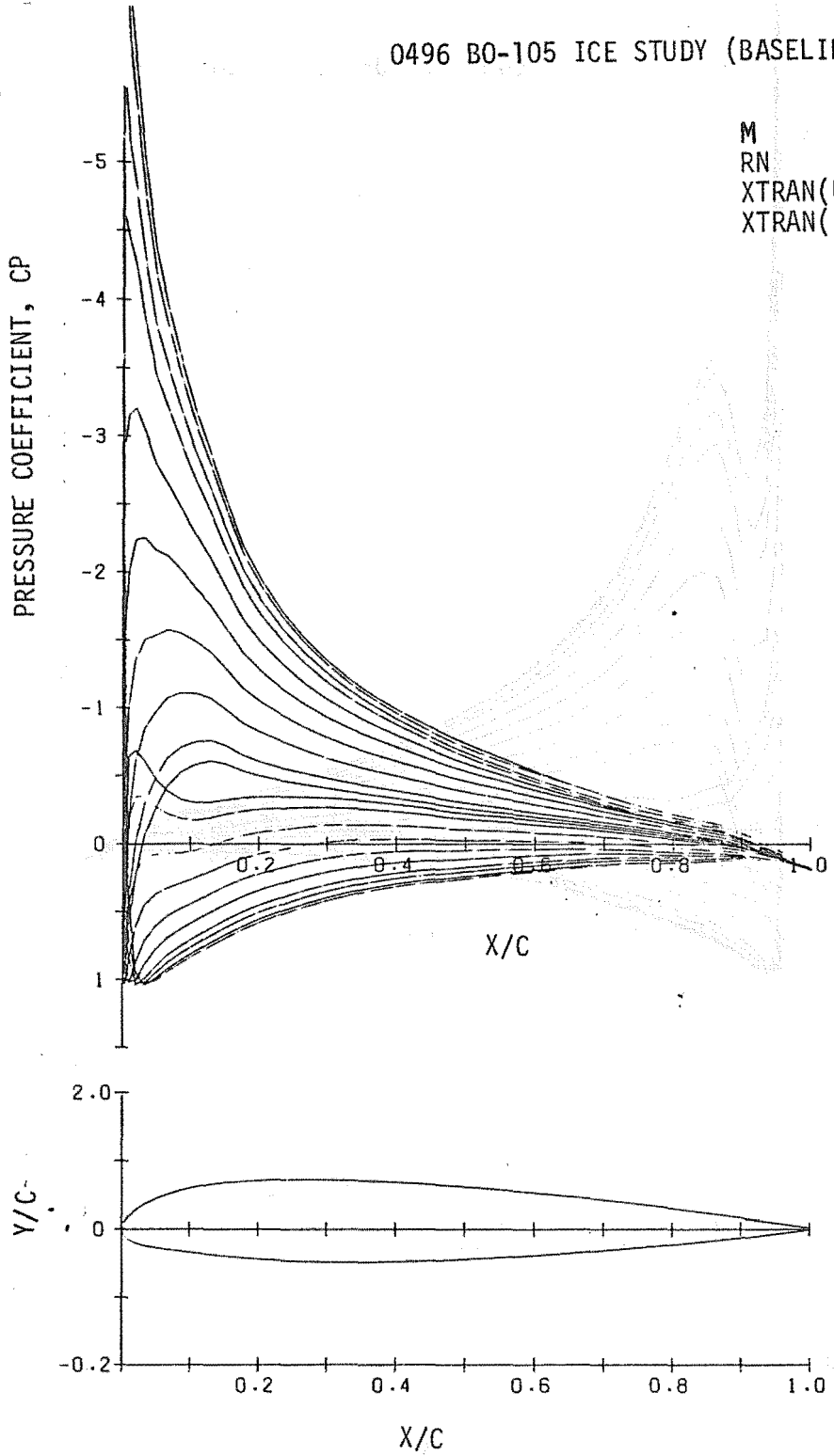
FIGURE C-9. BO-105 ROTOR ICE STUDY (BASELINE) - PRESSURE DISTRIBUTION
