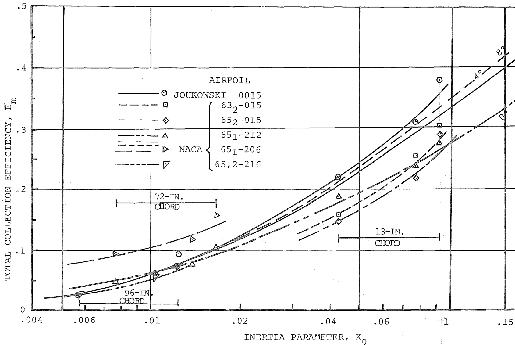
FIGURE B-6. AIRFOIL MATCHING USING KNOWN AIRFOIL COLLECTION DATA
