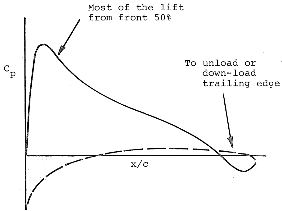
FIGURE C-3. Pitching Moment Requirements
