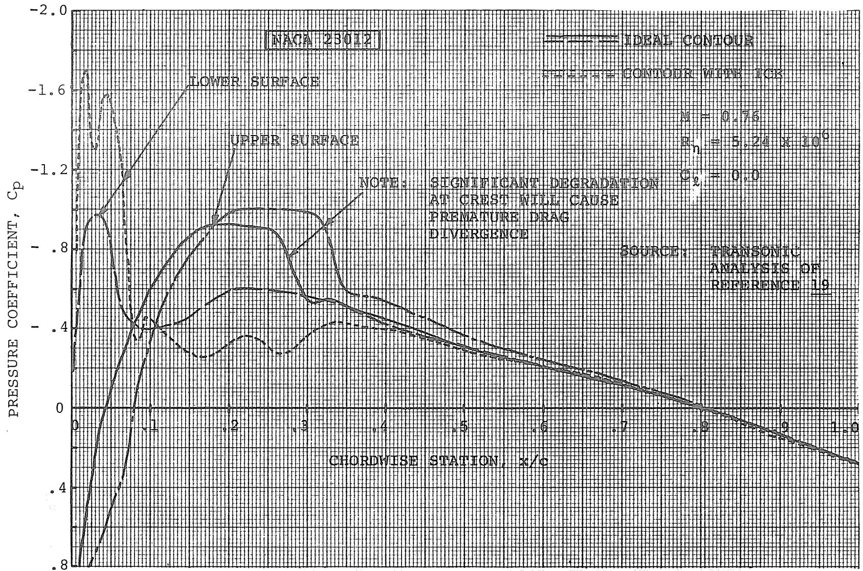
FIGURE C-22. EFFECT OF L.E. ICE ACCUMULATION ON A PRESSURE DISTRIBUTION OVER THE NACA 23012 AIRFOIL NEAR DRAG DIVERGENCE
