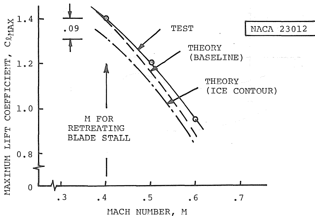
FIGURE C-15. MAXIMUM LIFT BOUNDARIES OF THE VR-7 AND NACA 23012 AIRFOILS
