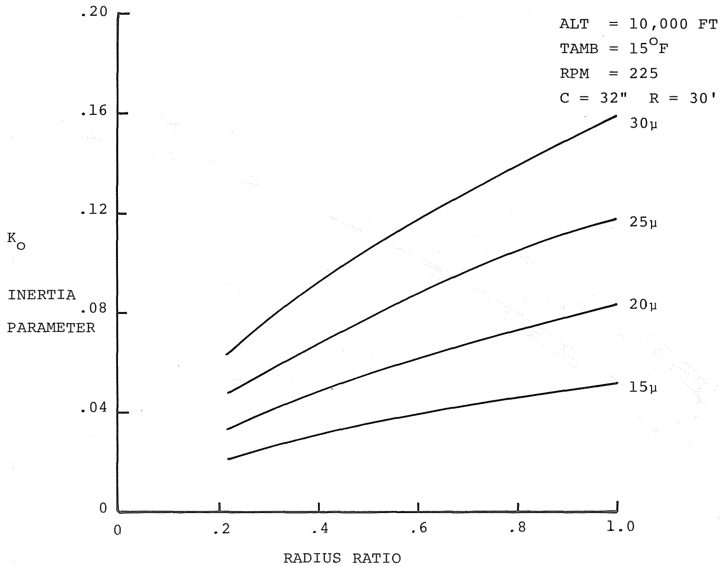
FIGURE B-5. MODIFIED INERTIA PARAMETER ACROSS ROTOR SPAN
