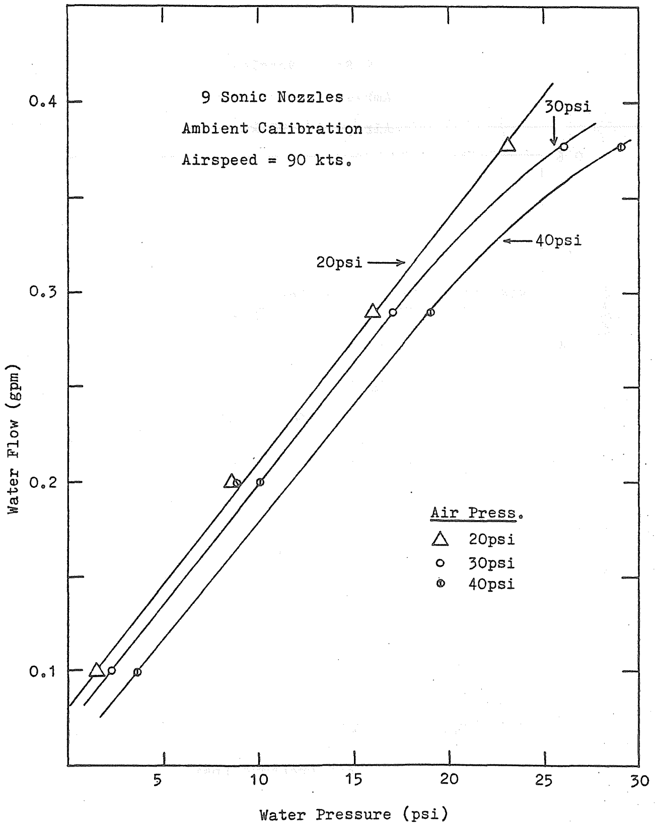
FIGURE A-9. NASA ICING TUNNEL RESULTS
