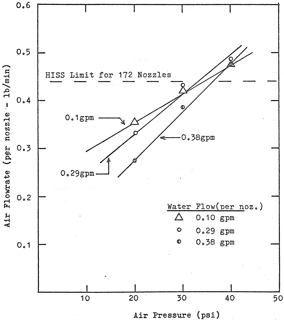
FIGURE A-8. NASA ICING TUNNEL RESULTS
