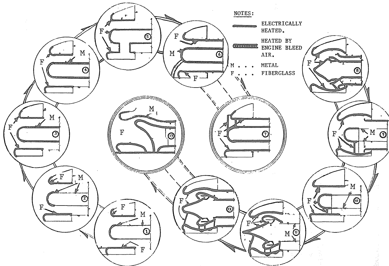
FIGURE 2-38. EVOLUTION OF TWO ENGINE INLET SYSTEMS
