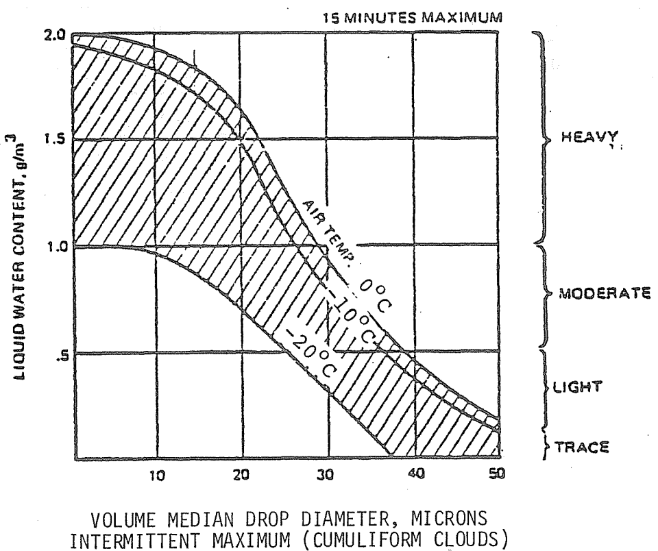
FIGURE B-3. ICING LEVEL DEFINITIONS PER TR-75-34A.
