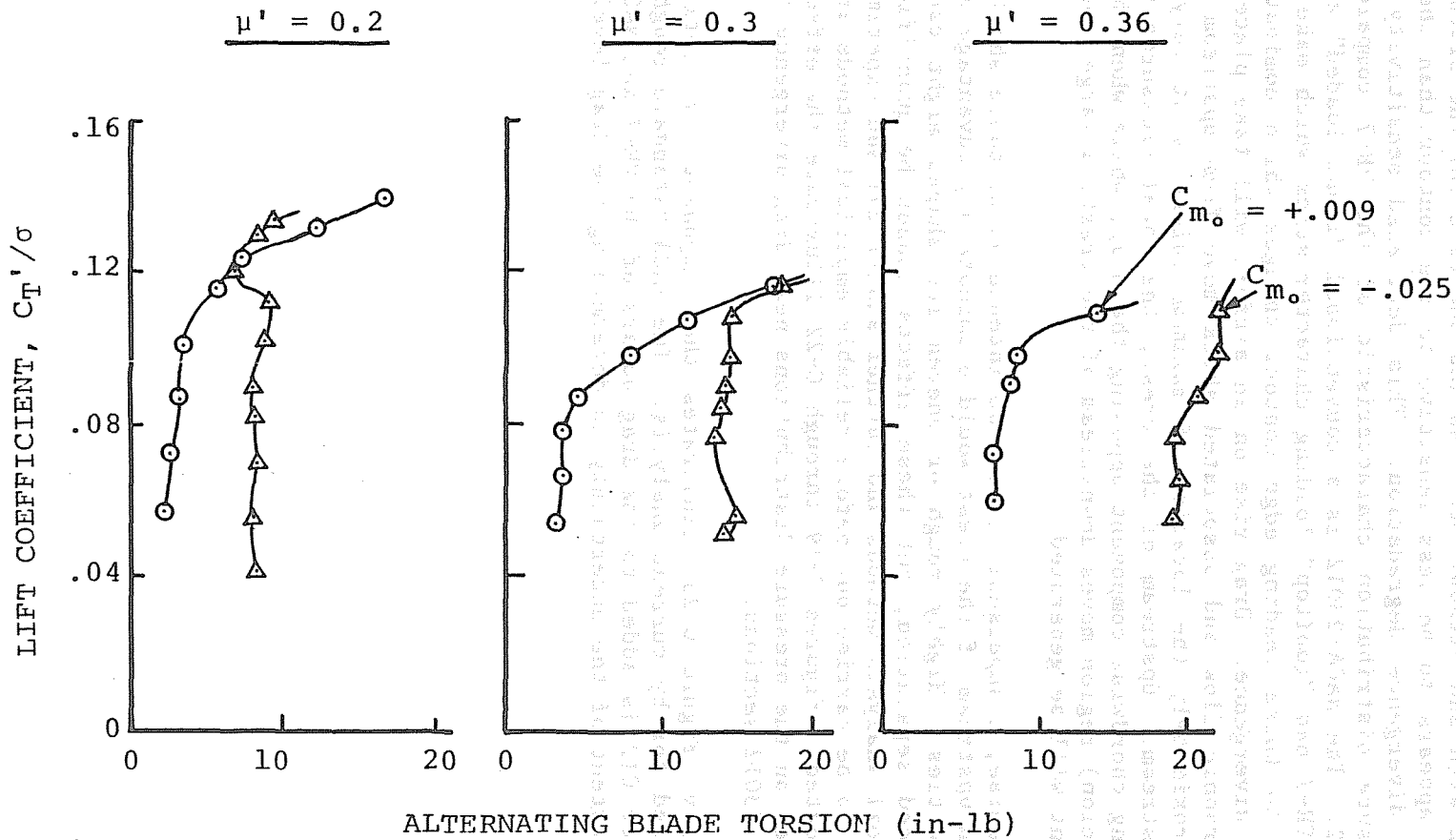
FIGURE C-17. EFFECT OF PITCHING MOMENT ON ROTOR LOADS
