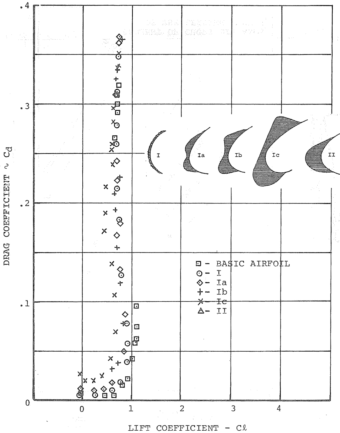
FIGURE 2-37. AIRFOIL DRAG DUE TO ICE
