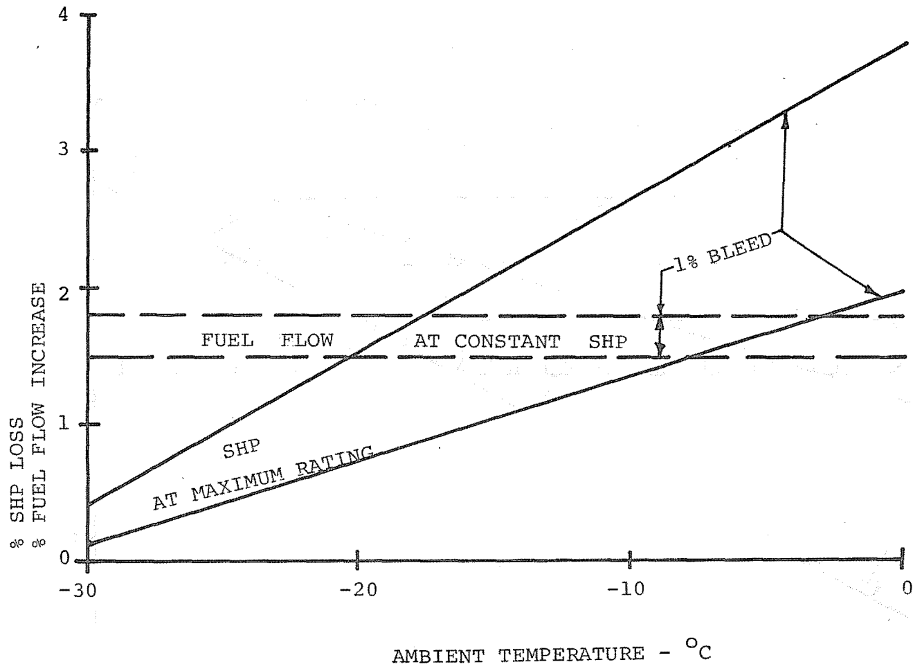
FIGURE 2-28. ENGINE COMPRESSOR BLEED EXTRACTION PENALTIES
