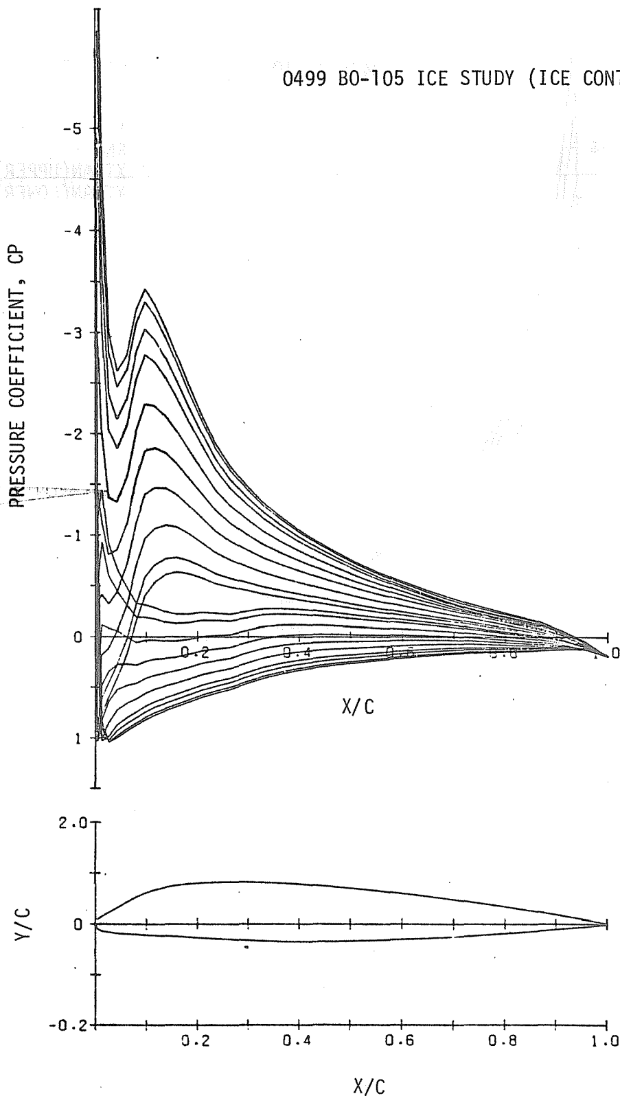
FIGURE C-10. BO-105 ROTOR ICE STUDY (ICE CONTOUR) - PRESSURE DISTRIBUTION
