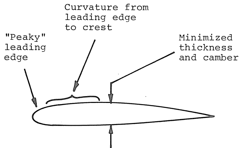
FIGURE C-4. Airfoil Geometric Characteristics
