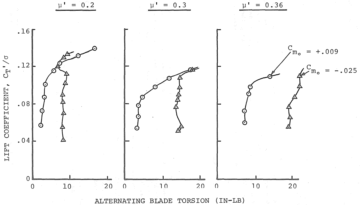
FIGURE 2-35. EFFECT OF PITCHING MOMENT ON ROTOR LOADS
