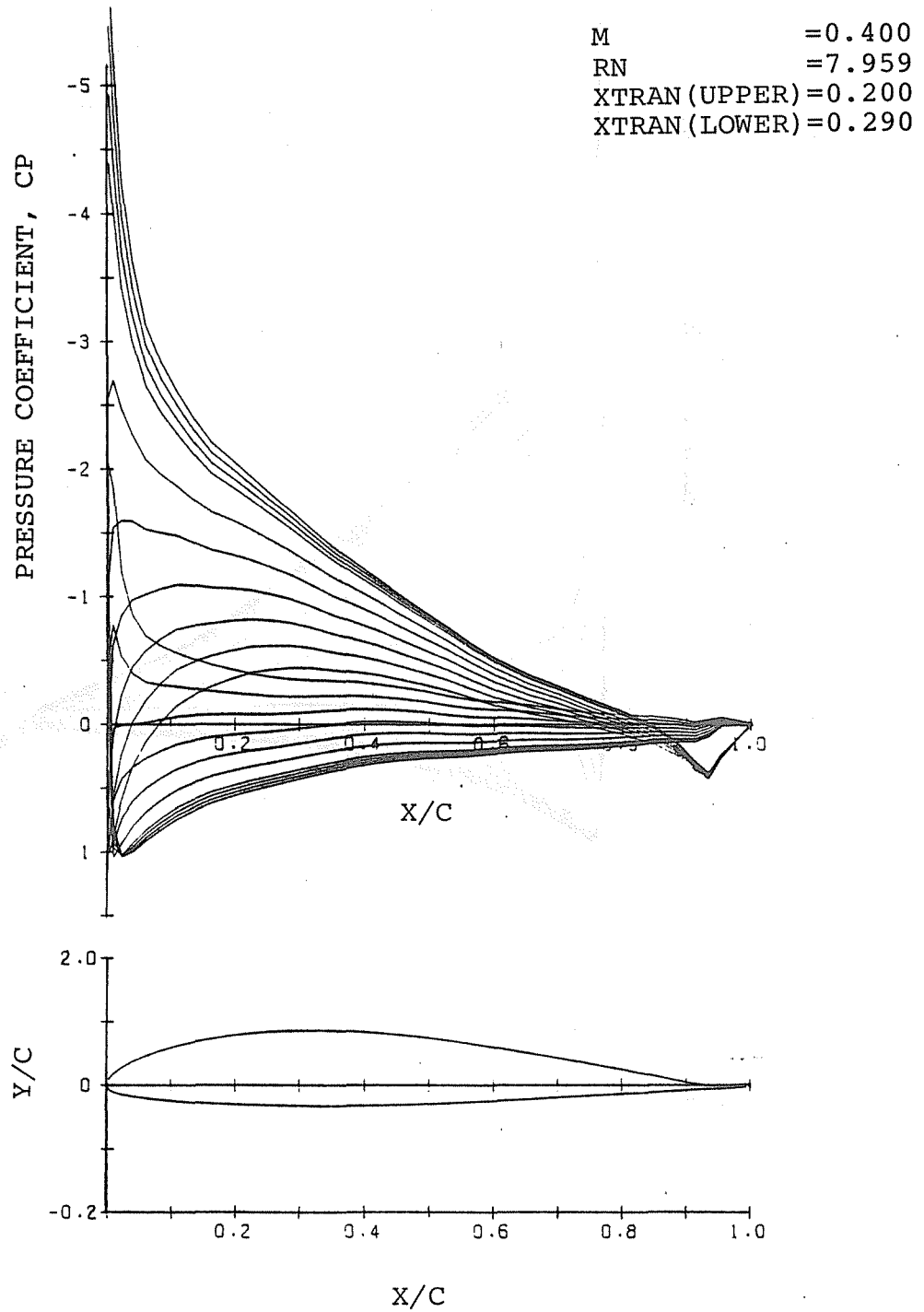
FIGURE C-13 VR-7 ROTOR ICE STUDY (BASELINE) - PRESSURE DISTRIBUTION
