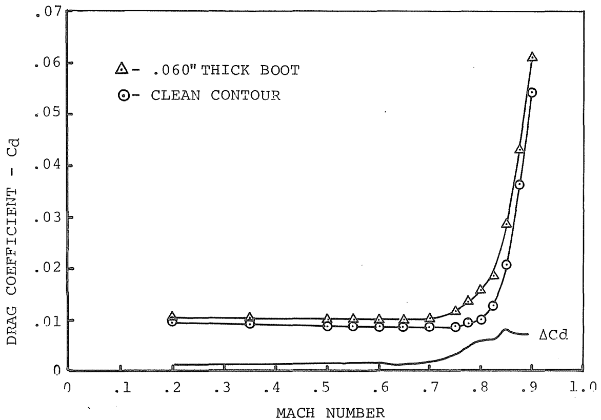
FIGURE 2-34. DRAG RISE DUE TO LEADING EDGE DISTURBANCE
