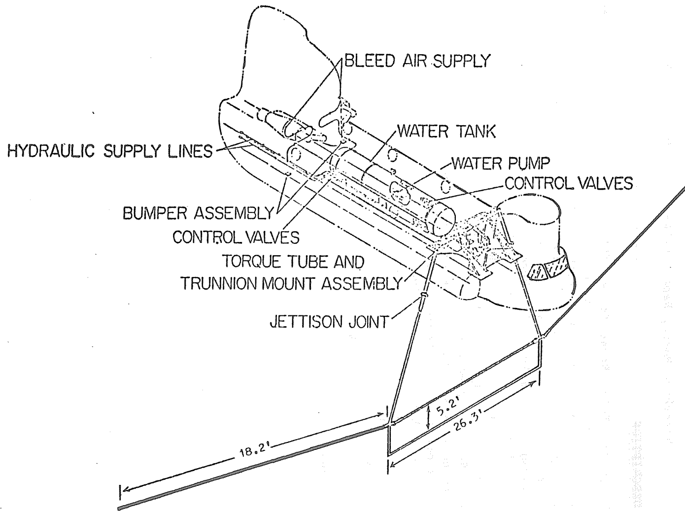
FIGURE A-1. HELICOPTER ICING SPRAY SYSTEM (HISS)
