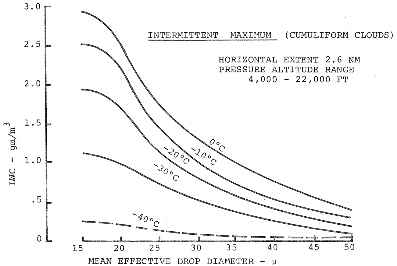
FIGURE 2-11. FAR PART 25 ICING LEVEL DEFINITIONS
