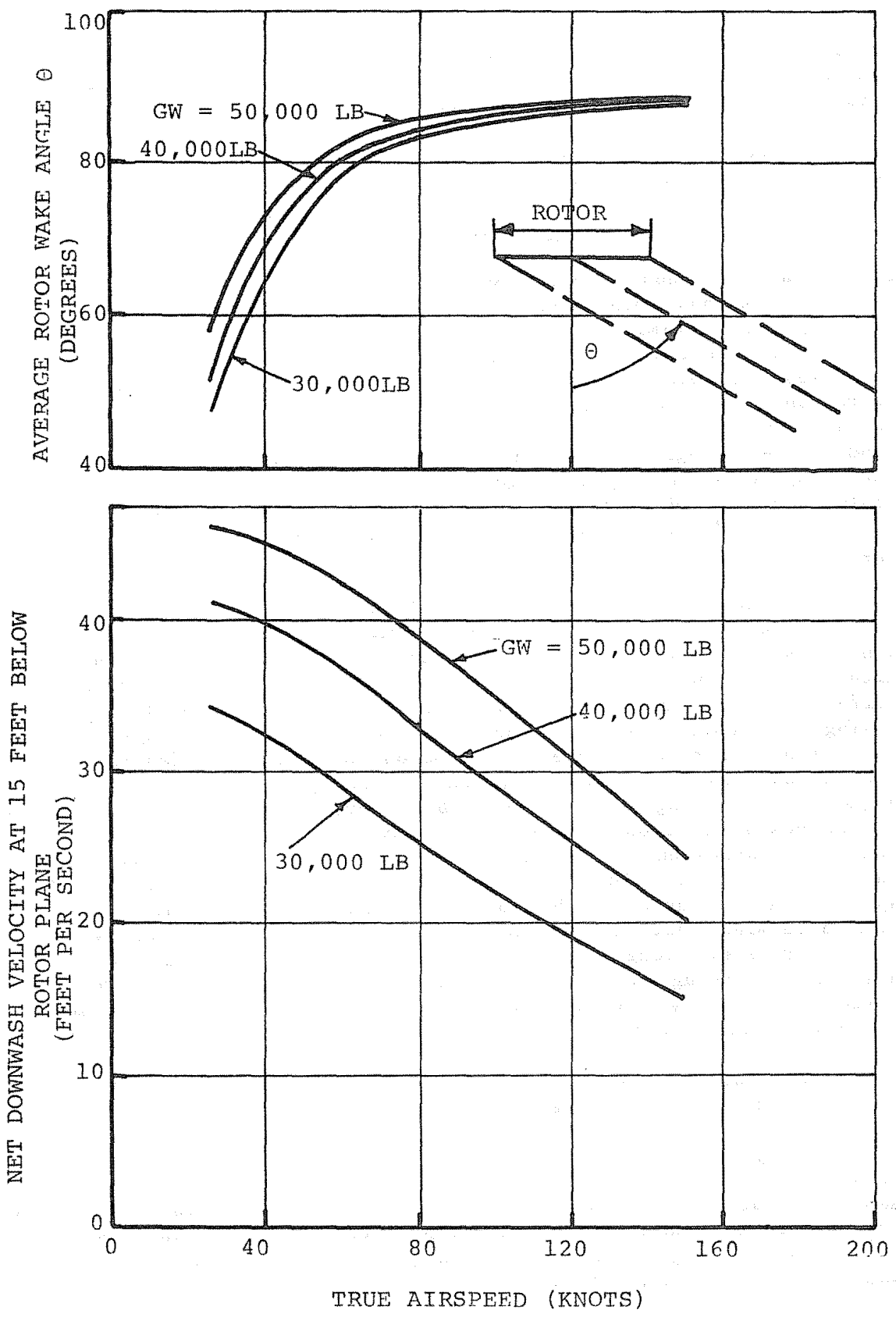
FIGURE 2-4. ROTOR DOWNWASH CHARACTERISTICS
