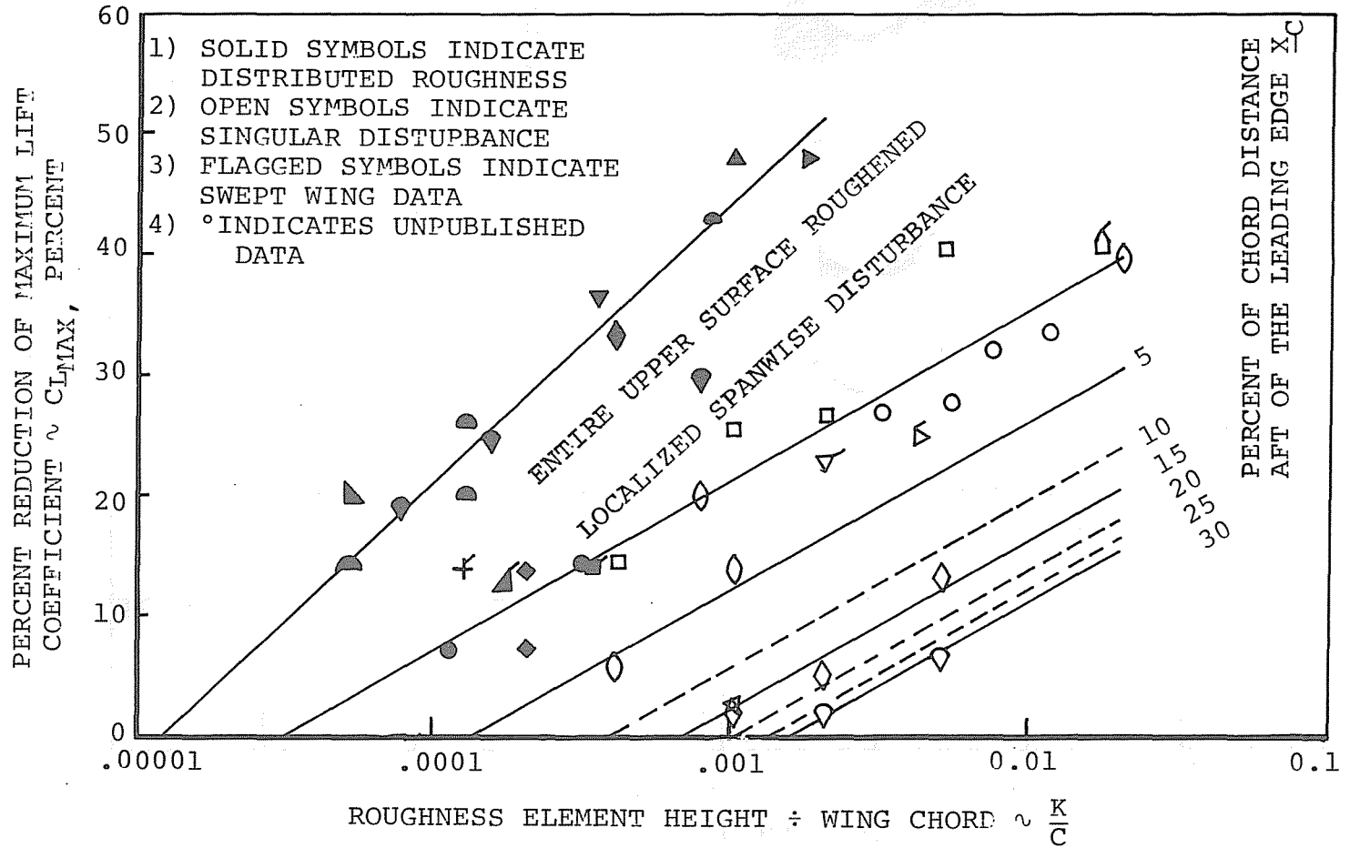
FIGURE 2-36. EFFECT OF SURFACE ROUGHNESS ON LOSS IN MAXIMUM LIFT CAPABILITY
