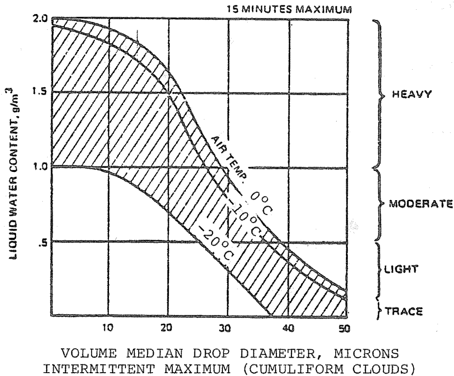
FIGURE 2-17. ICING LEVEL DEFINITIONS PER TR-75-34A.
