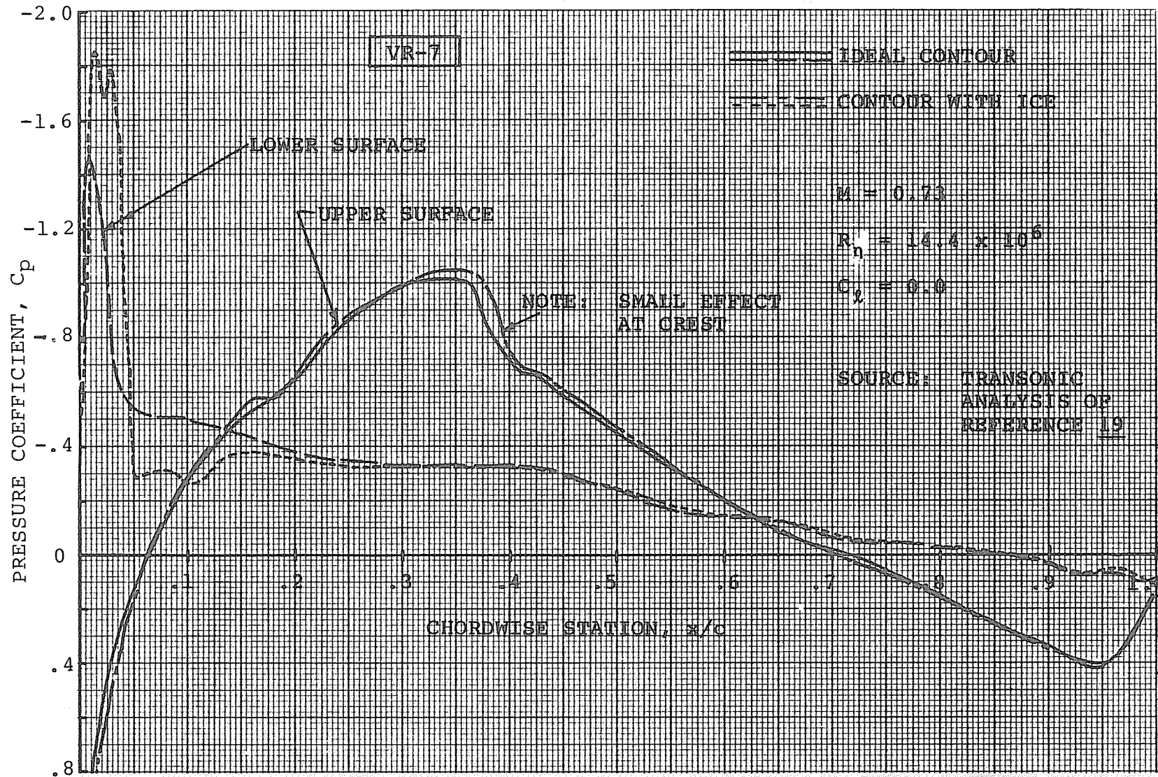
FIGURE C-20. EFFECT OF L.E. ICE ACCUMULATION ON A PRESSURE DISTRIBUTION OVER THE VR-7 AIRFOIL NEAR DRAG DIVERGENCE.
