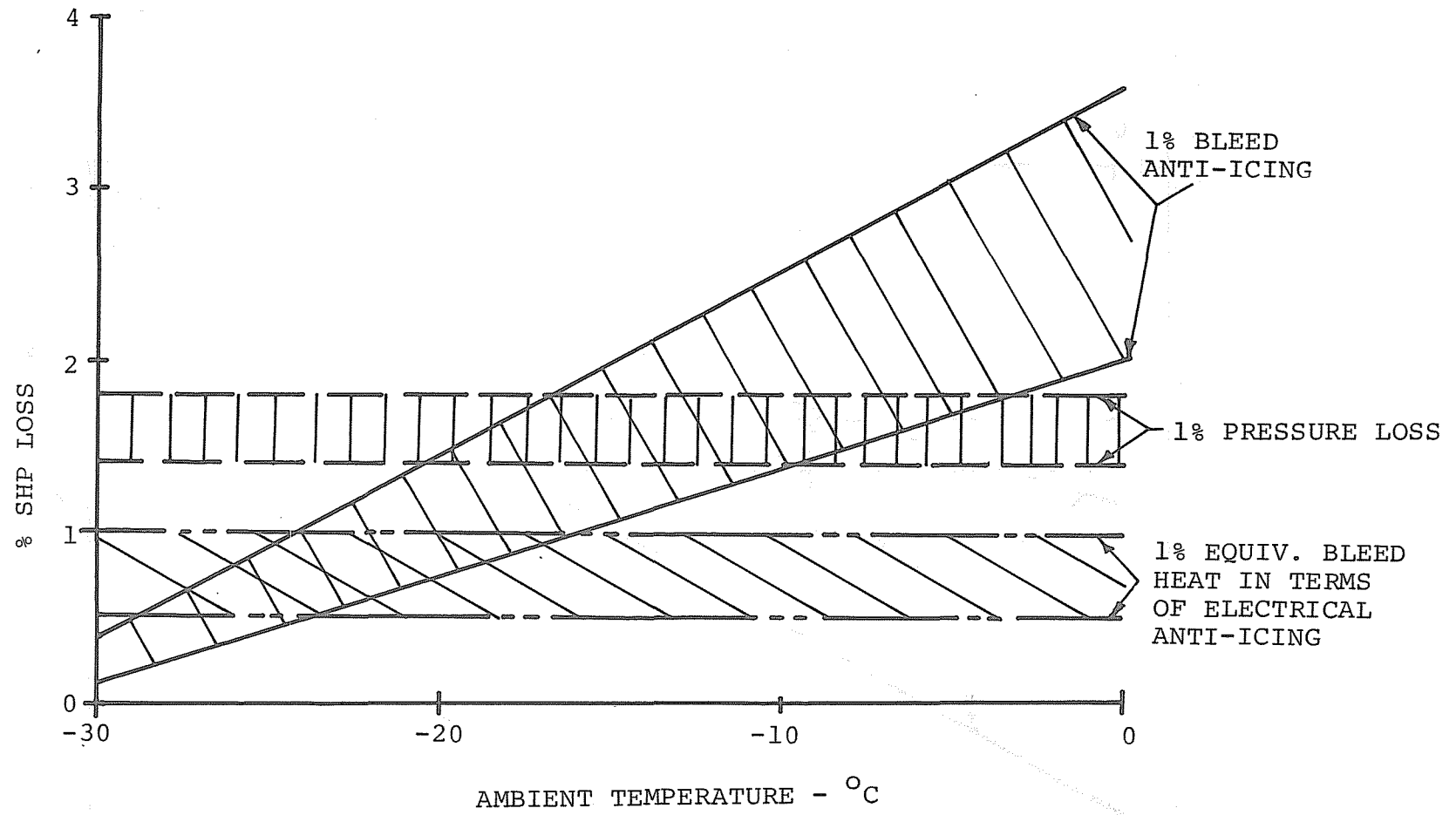
FIGURE 2-29. INDUCTION SYSTEM LOSSES UNDER ICING CONDITIONS
