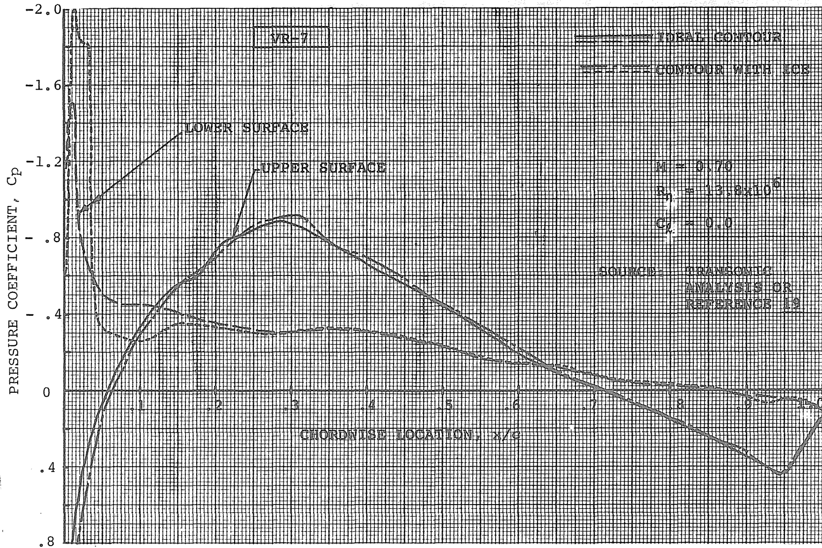
FIGURE C-19. EFFECT OF L.E. ICE ACCUMULATION ON A PRESSURE DISTRIBUTION OVER THE VR-7 AIRFOIL BELOW DRAG DIVERGENCE
