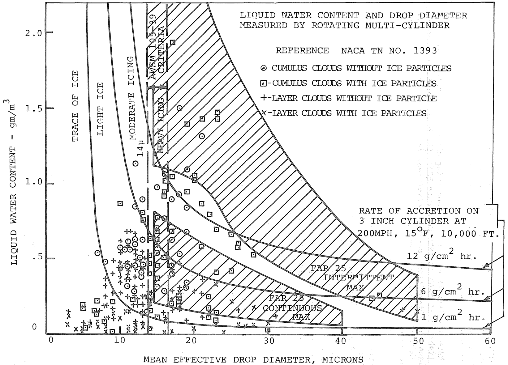
FIGURE 2-12. ICING INTENSITIES AND RATES OF ACCRETION DEVELOPED FROM MEASURED ICING DATA.
