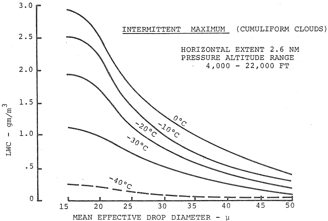
FIGURE B-2. FAR PART 25 ICING LEVEL DEFINITIONS
