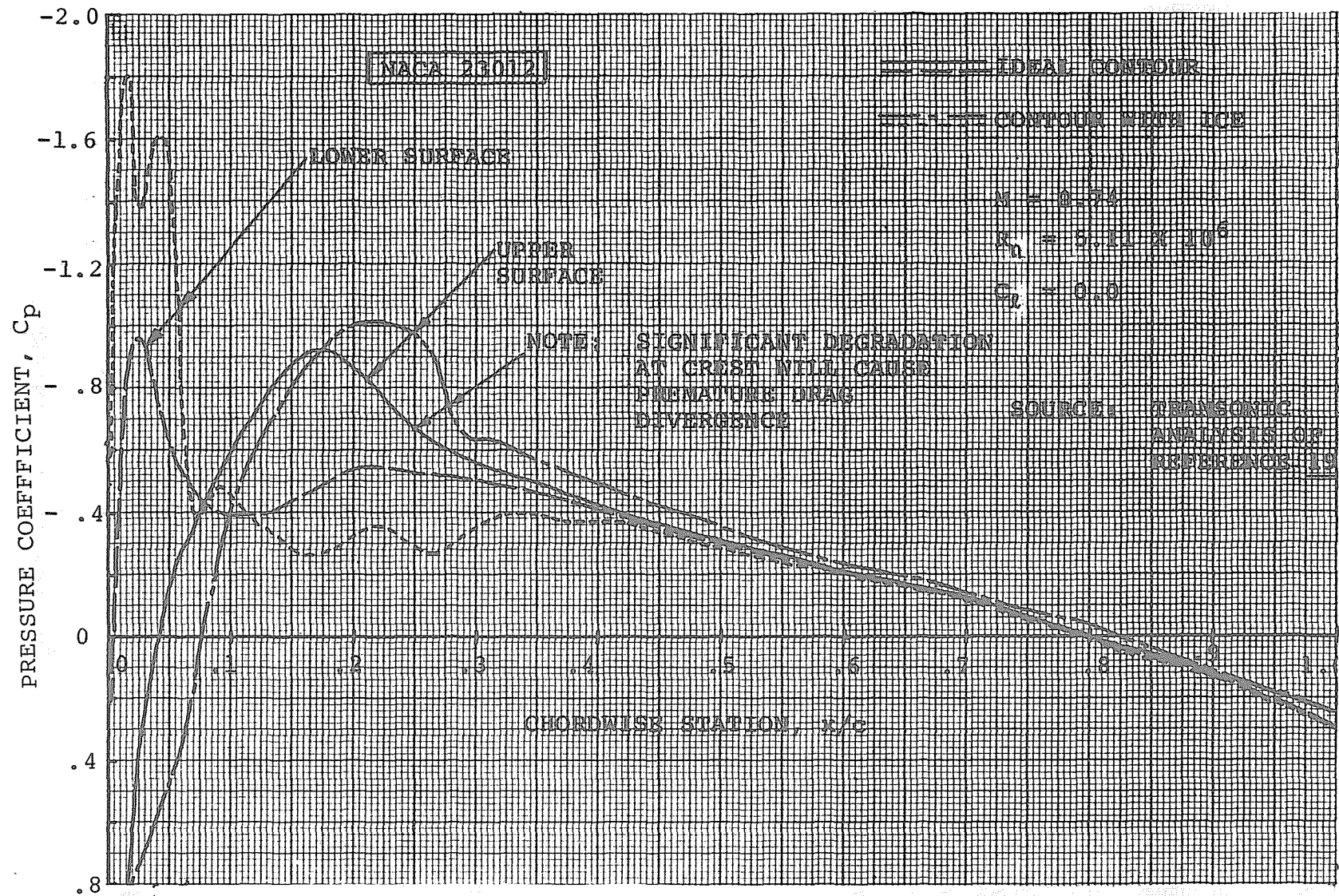
FIGURE C-21. EFFECT OF L.E. ICE ACCUMULATION ON A PRESSURE DISTRIBUTION OVER THE NACA 23012 AIRFOIL BELOW DRAG DIVERGENCE
