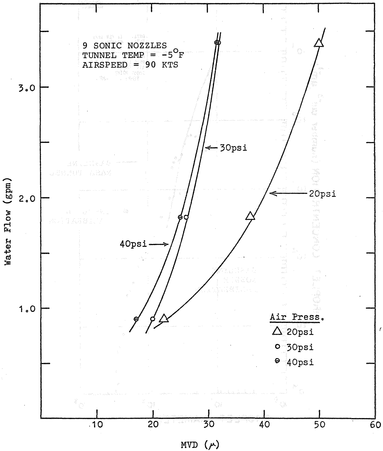
FIGURE A-10. NASA ICING TUNNEL RESULTS
