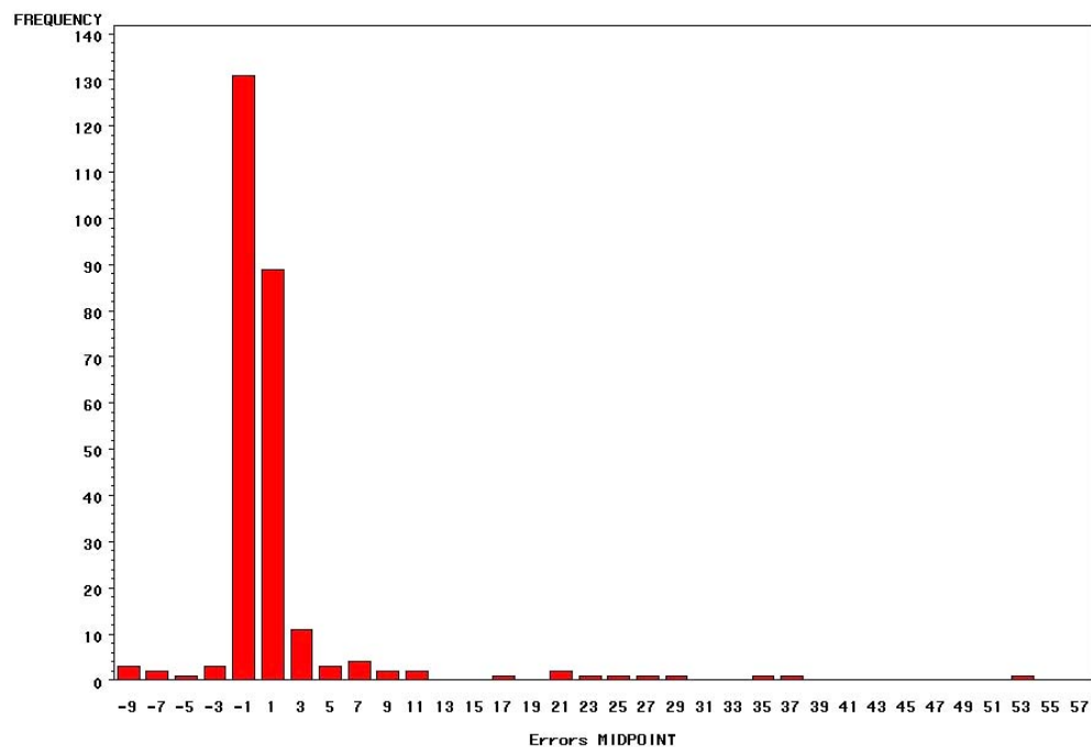
Figure 4-23: Histogram of Measurement Errors Using All Observations
