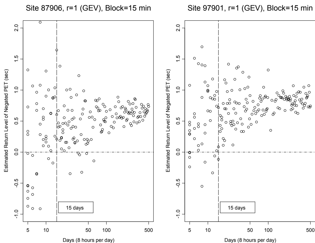
Figure 8-20: Comparison of Return Level Estimates
