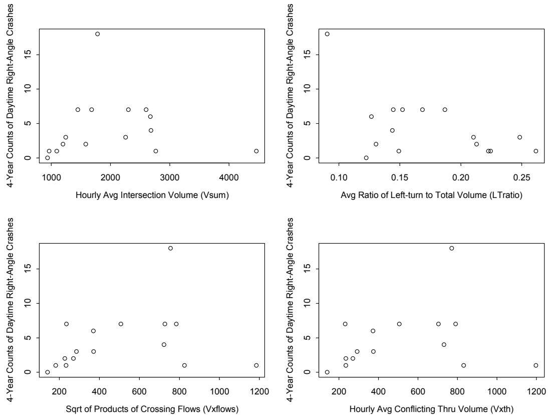
Figure 5-4: Scatter Plots of Volume Information versus Actual Counts of Crashes
