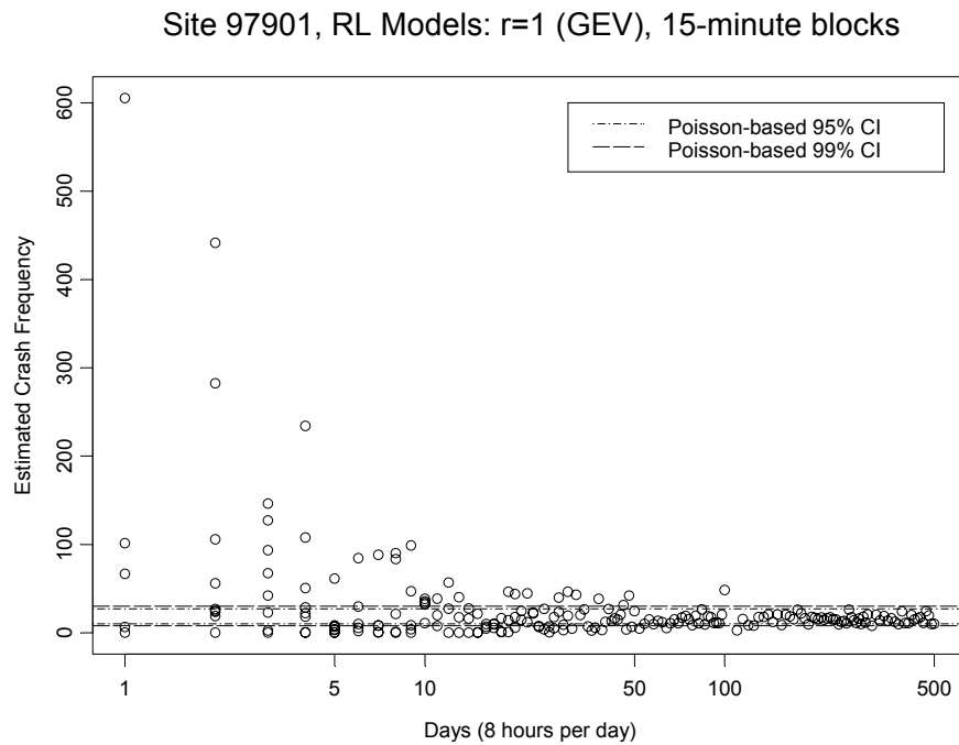
Figure G-7: Estimated Crash Frequency at Site 97901 using r = 1 and 15-minute Blocks
