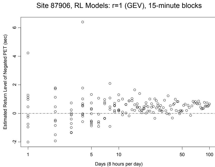
Figure G-2: Estimated Return Level at Site 87906 using r = 1 and 15-minute Blocks
