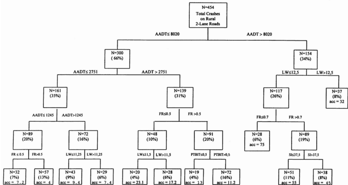
Figure 2-4: Example of Regression Tree Using HTBR (Karlaftis and Golias, 2002)
