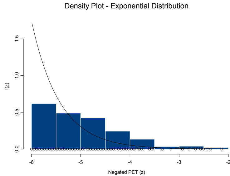
Figure 8-8: Fitted Constraint Exponential Density – Site 97901
