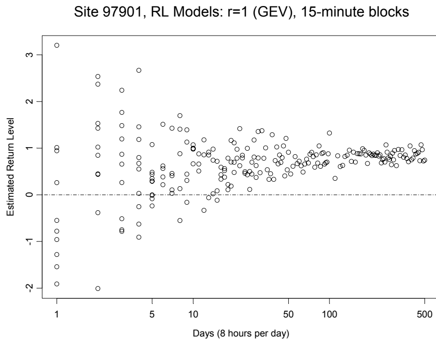
Figure G-8: Estimated Return Level at Site 97901 using r = 1 and 15-minute Blocks
