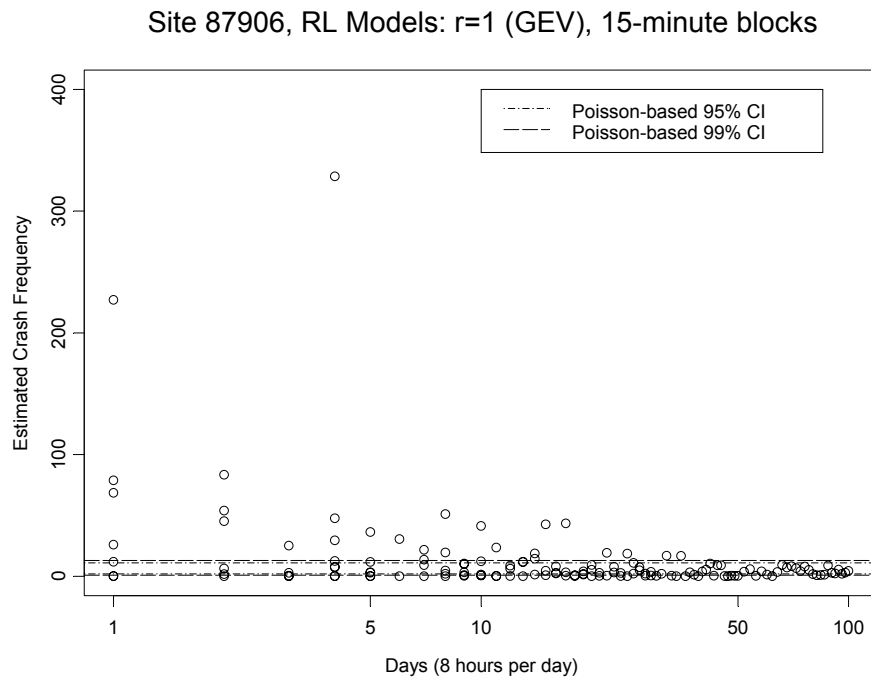
Figure G-1: Estimated Crash Frequency at Site 87906 using r = 1 and 15-minute Blocks
