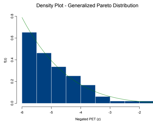
Figure 8-10: Fitted Constraint Generalized Pareto Distribution – Site 87906
