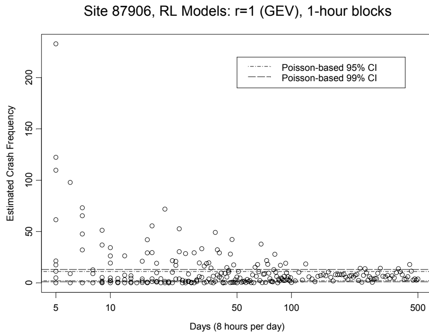
Figure G-3: Estimated Crash Frequency at Site 87906 using r = 1 and 1-hour Blocks
