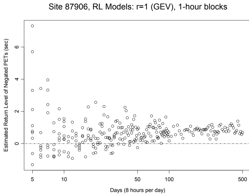
Figure G-4: Estimated Return Level at Site 87906 using r = 1 and 1-hour Blocks
