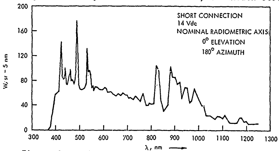
Figure 5-3. Spectral Peak Intensity of Grimes G-260 Strobe
