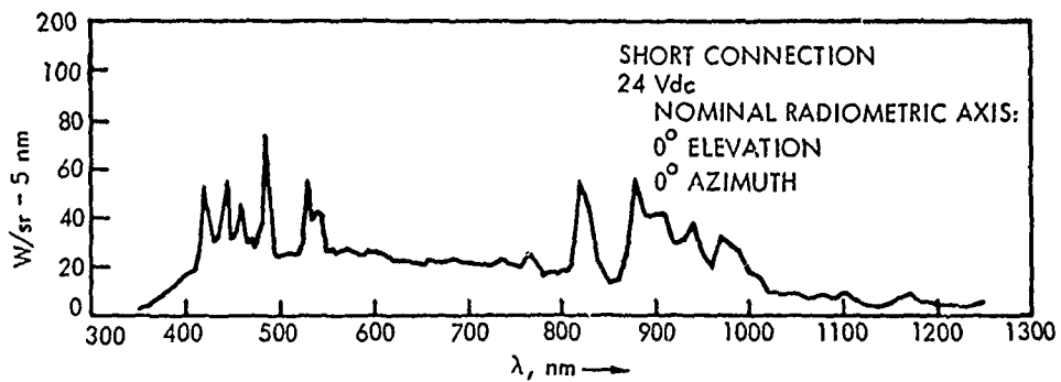
Figure 5-2. Spectral Peak Intensity of Whelen Strobe 7L
