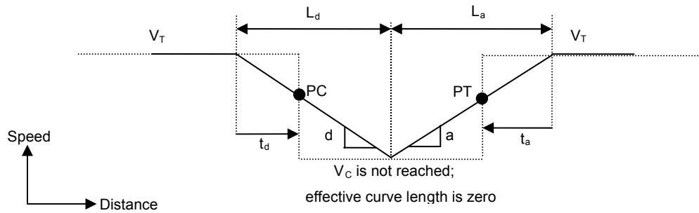
Figure 3-4 Modeling of transition sections for short curves
