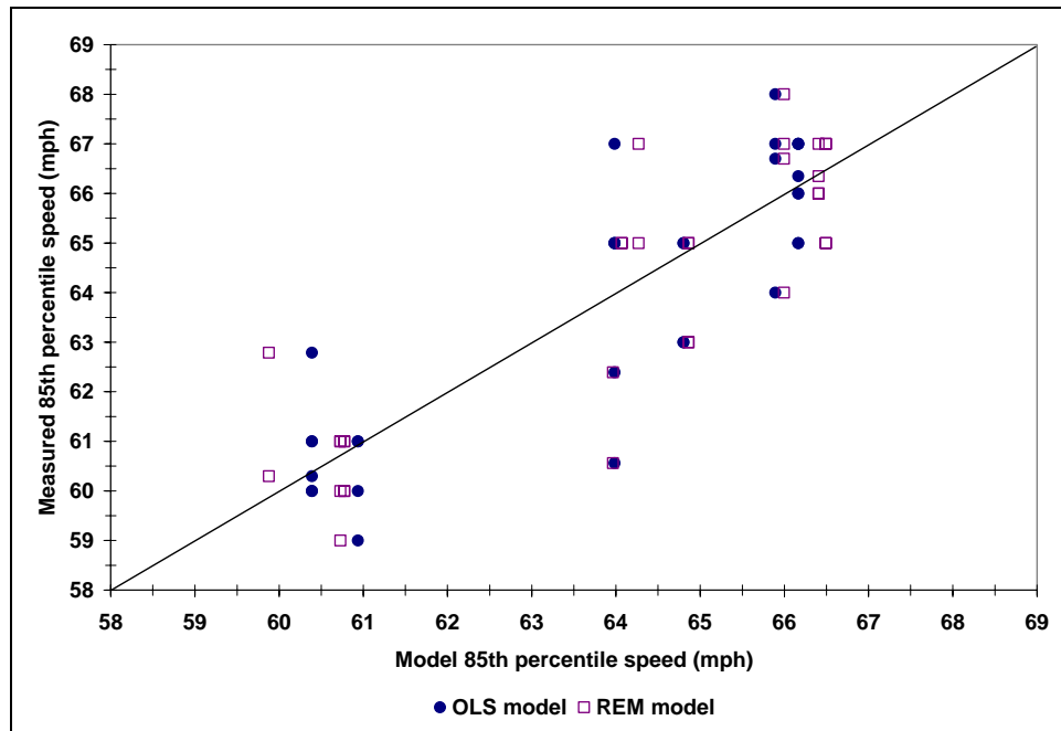
Figure 6-7 Performance of the traditional OLS and RE models in estimating 85 th percentile speed
