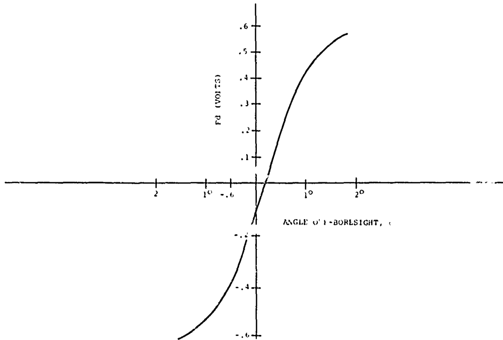
Figure 8. Difference Pattern Voltage Vs Angle Off Boresight, FA 7202 Antenna with Modified Feed Network
