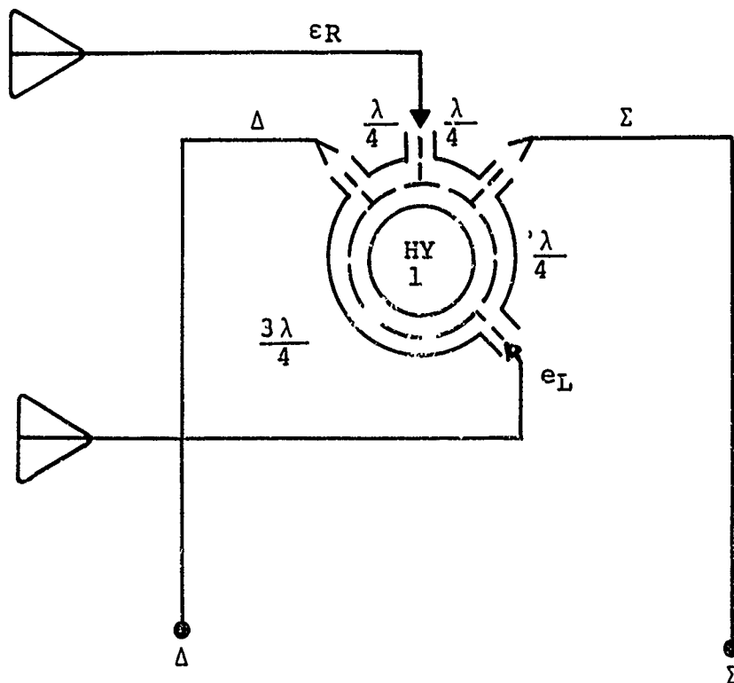
Figure E1. Hybrid Bridge Circuit for Tracking Feed
