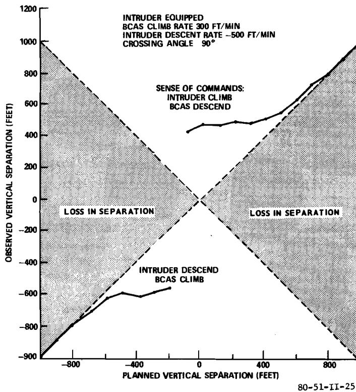
FIGURE 26. RESULTS FOR EQUIPPED INTRUDER VERTICALLY MANEUVERING EVALUATION
