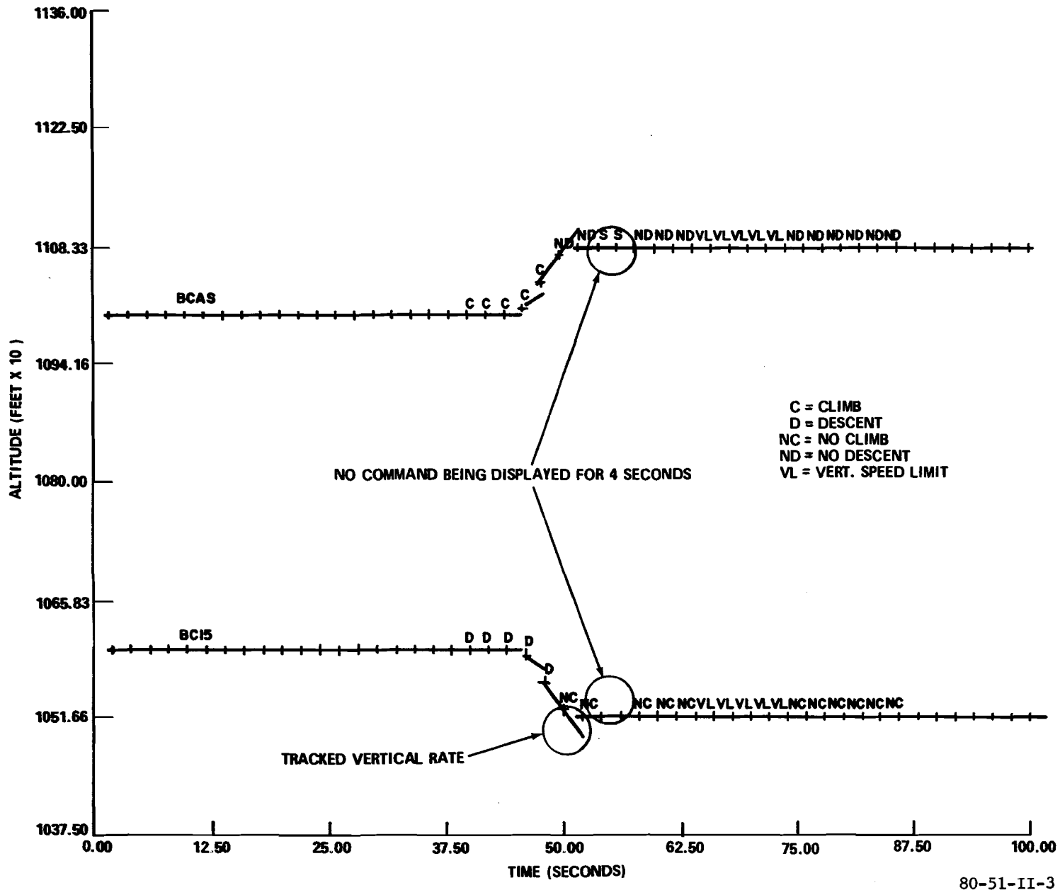
FIGURE 4. VERTICAL PROFILE OF GEOMETRY WHICH RESULTS IN EARLY COMMAND REMOVAL
