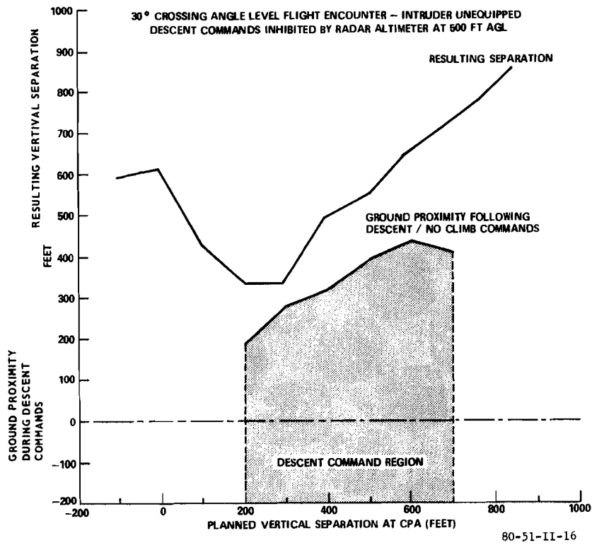
FIGURE 17. DESCENT COMMANDS INHIBITED BY RADAR ALTIMETER (INTRUDER UNEQUIPPED — 30° CROSSING ANGLE)
