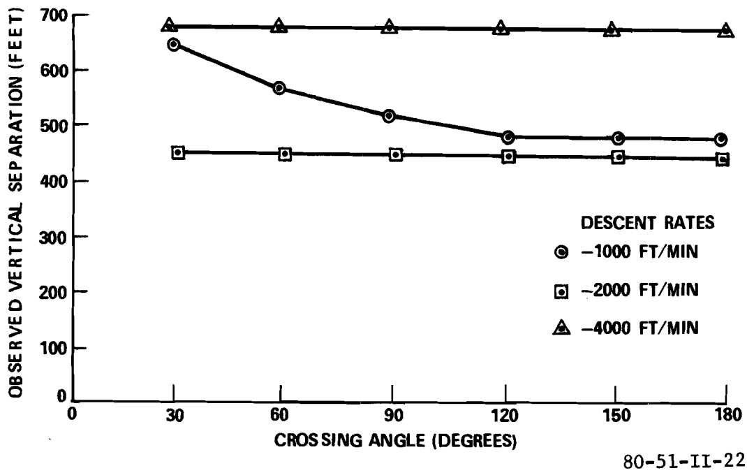
FIGURE 23. CROSSING ANGLE EFFECT ON EQUIPPED DESCENDING INTRUDER PERFORMANCE
