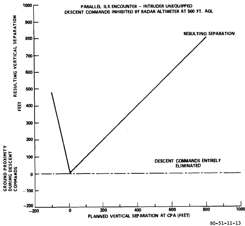
FIGURE 14. DESCENT COMMANDS INHIBITED BY RADAR ALTIMETER (INTRUDER UNEQUIPPED — PARALLEL ILS)
