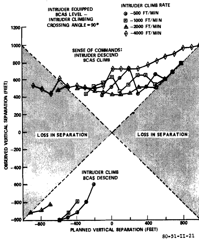
FIGURE 22. PERFORMANCE FOR EQUIPPED CLIMBING INTRUDERS
