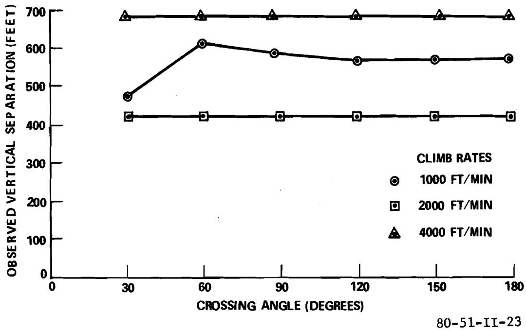
FIGURE 24. CROSSING ANGLE EFFECT ON EQUIPPED CLIMBING INTRUDER PERFORMANCE
