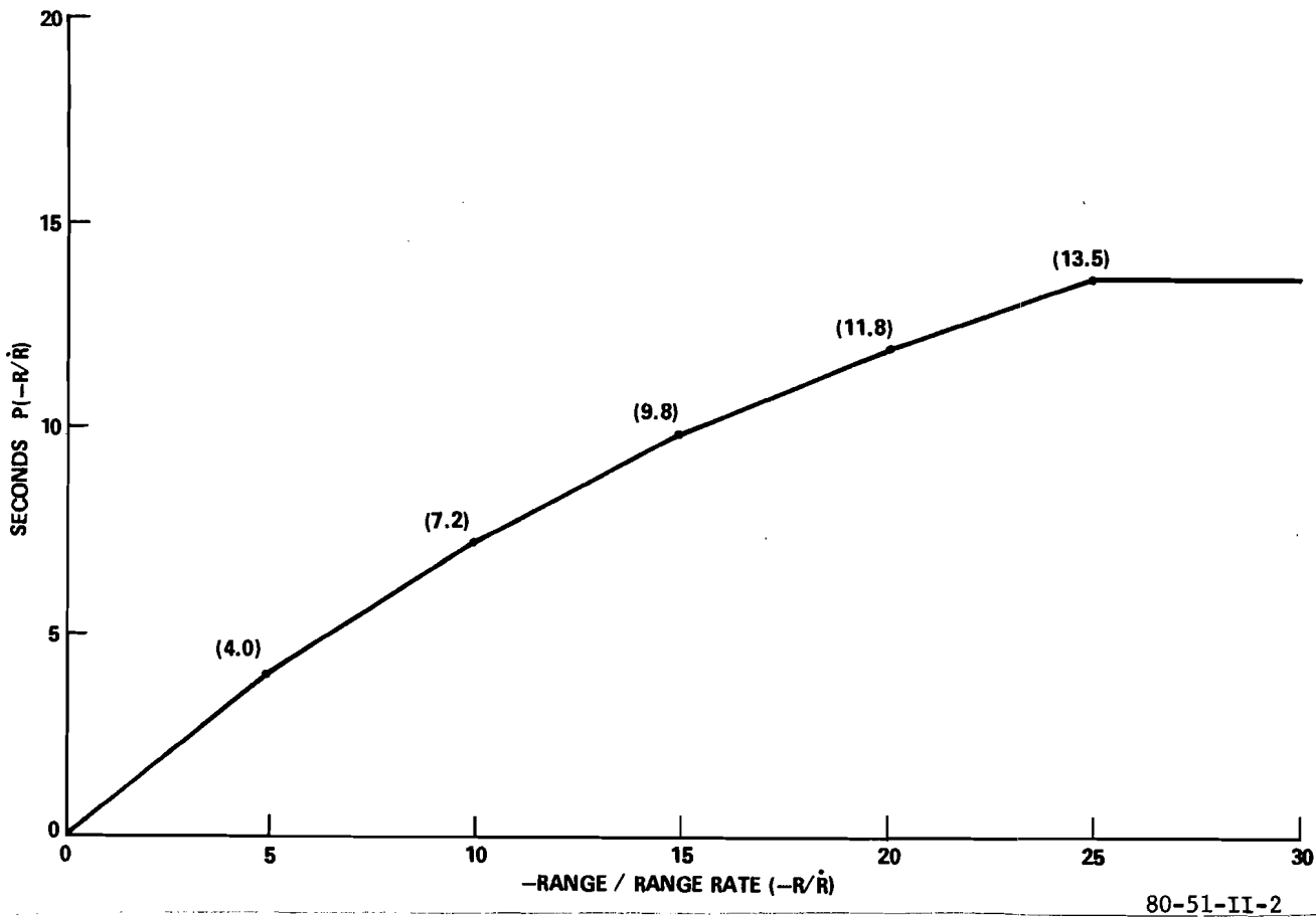
FIGURE 3. VERTICAL DIVERGENCE PROJECTION FUNCTION ( P(-R/\dot{R}) )
