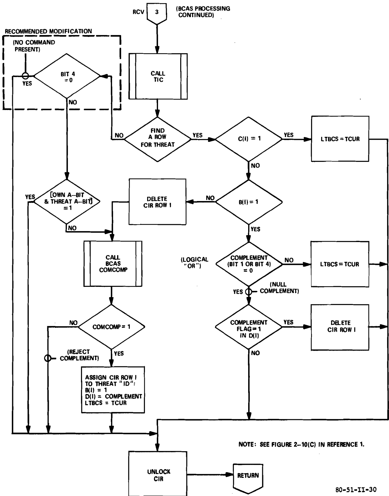
FIGURE 33. RCV MODIFICATION — COMMAND PRESENCE CHECK
