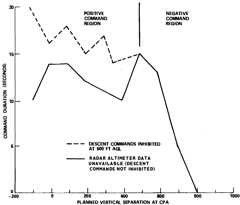
FIGURE 12. COMMAND DURATION COMPARISON
