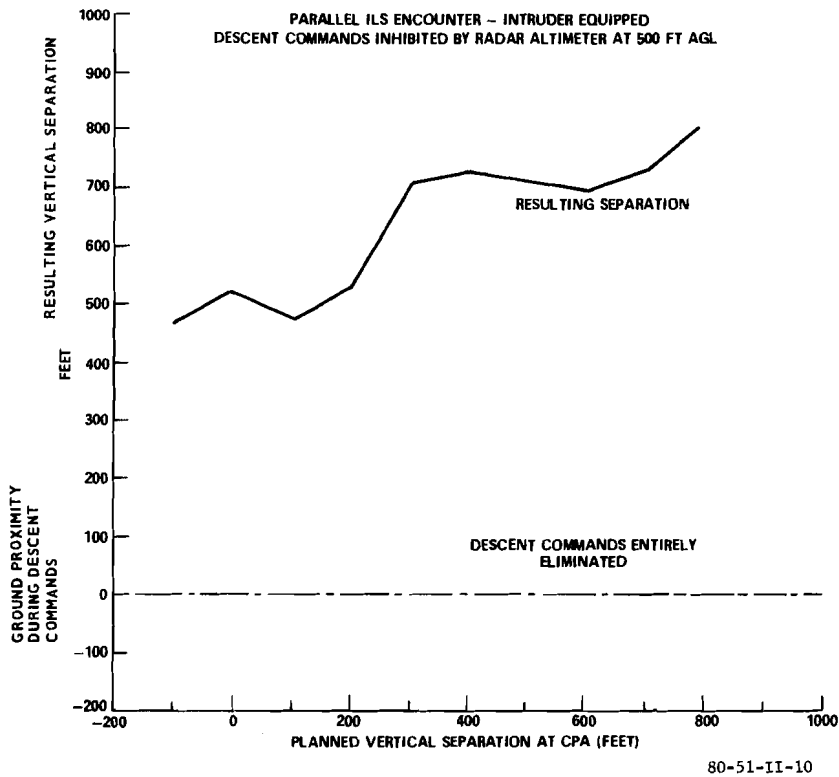
FIGURE 11. DESCENT COMMANDS INHIBITED BY RADAR ALTIMETER (INTRUDER EQUIPPED — PARALLEL ILS)
