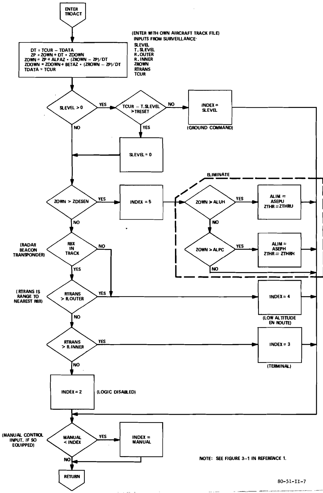
FIGURE 8. TROACT MODIFICATION — ELIMINATION OF THE SETTING OF PARAMETER VALUES
