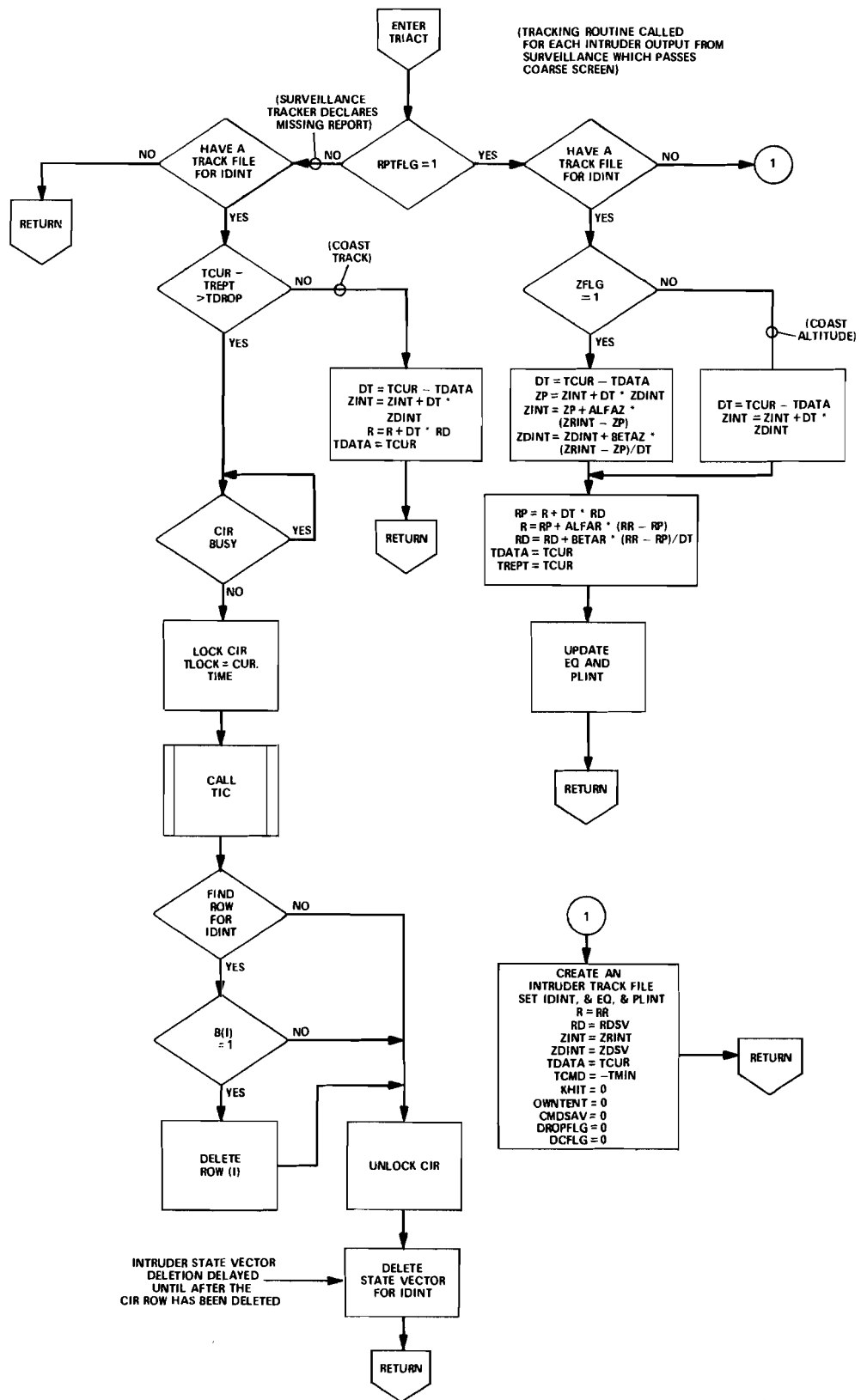
FIGURE 37. TRIACT LOGIC MODIFICATION — DELAY INTRUDER STATE VECTOR DELETION
