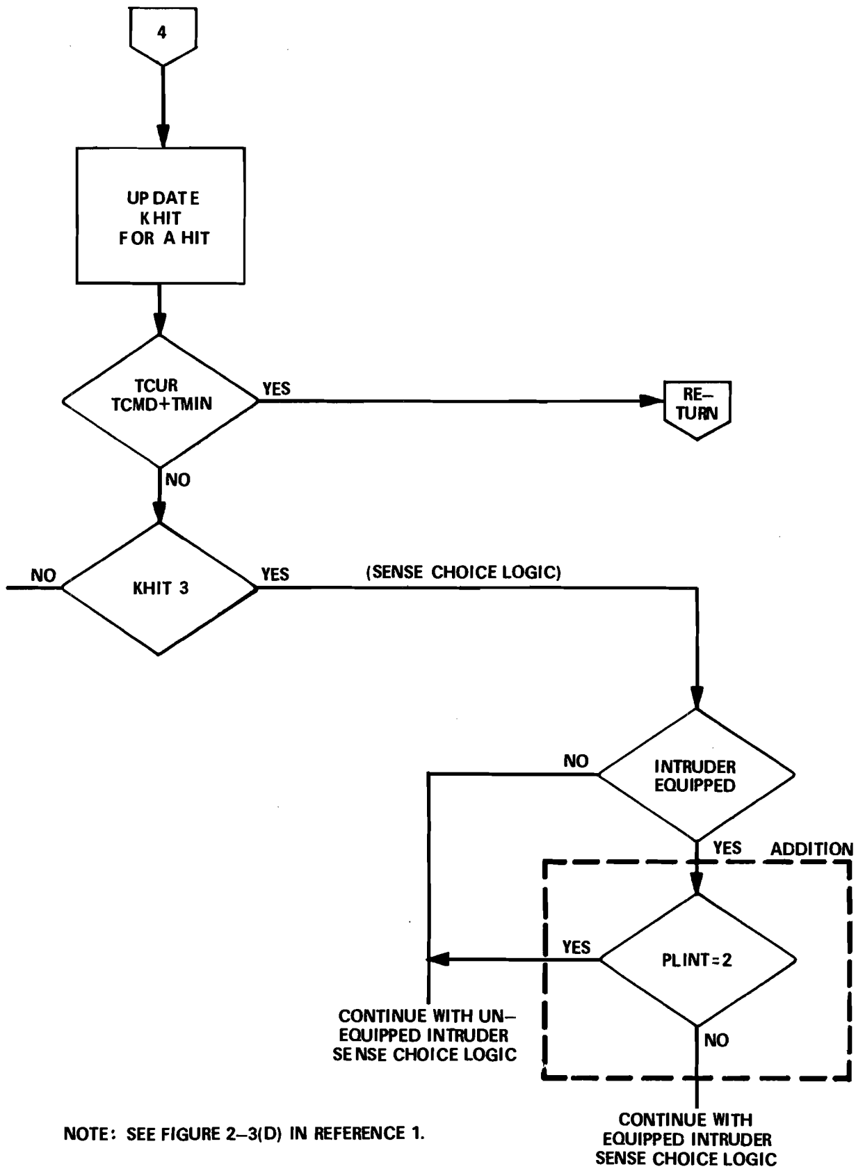
FIGURE 31. DRACT LOGIC MODIFICATION TO PROPERLY SELECT SENSE FOR PERFORMANCE LEVEL 2 EQUIPPED THREATS
