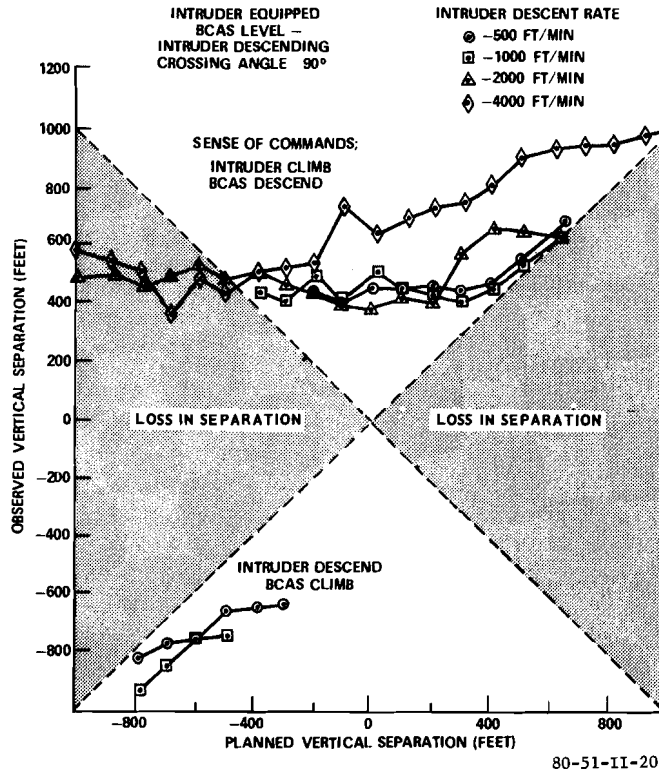
FIGURE 21. PERFORMANCE FOR EQUIPPED DESCENDING INTRUDERS
