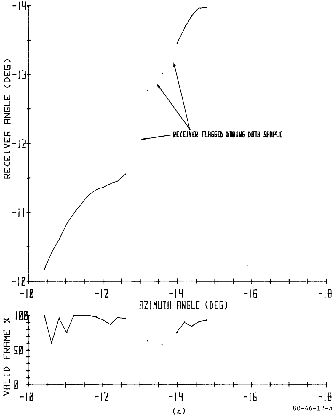
FIGURE 12. AZIMUTH RECEIVER ANGLE VERSUS TRUE AZIMUTH PLOTS USING THE SHAPED CLEARANCE PULSE (SHEET 1 OF 15)
