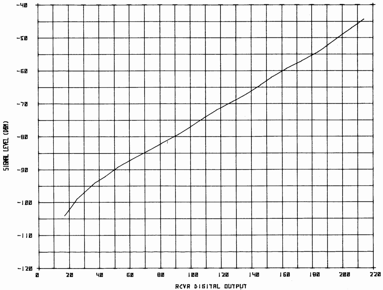
FIGURE 16. RECEIVER CALIBRATION CURVE (S/N SC103)
