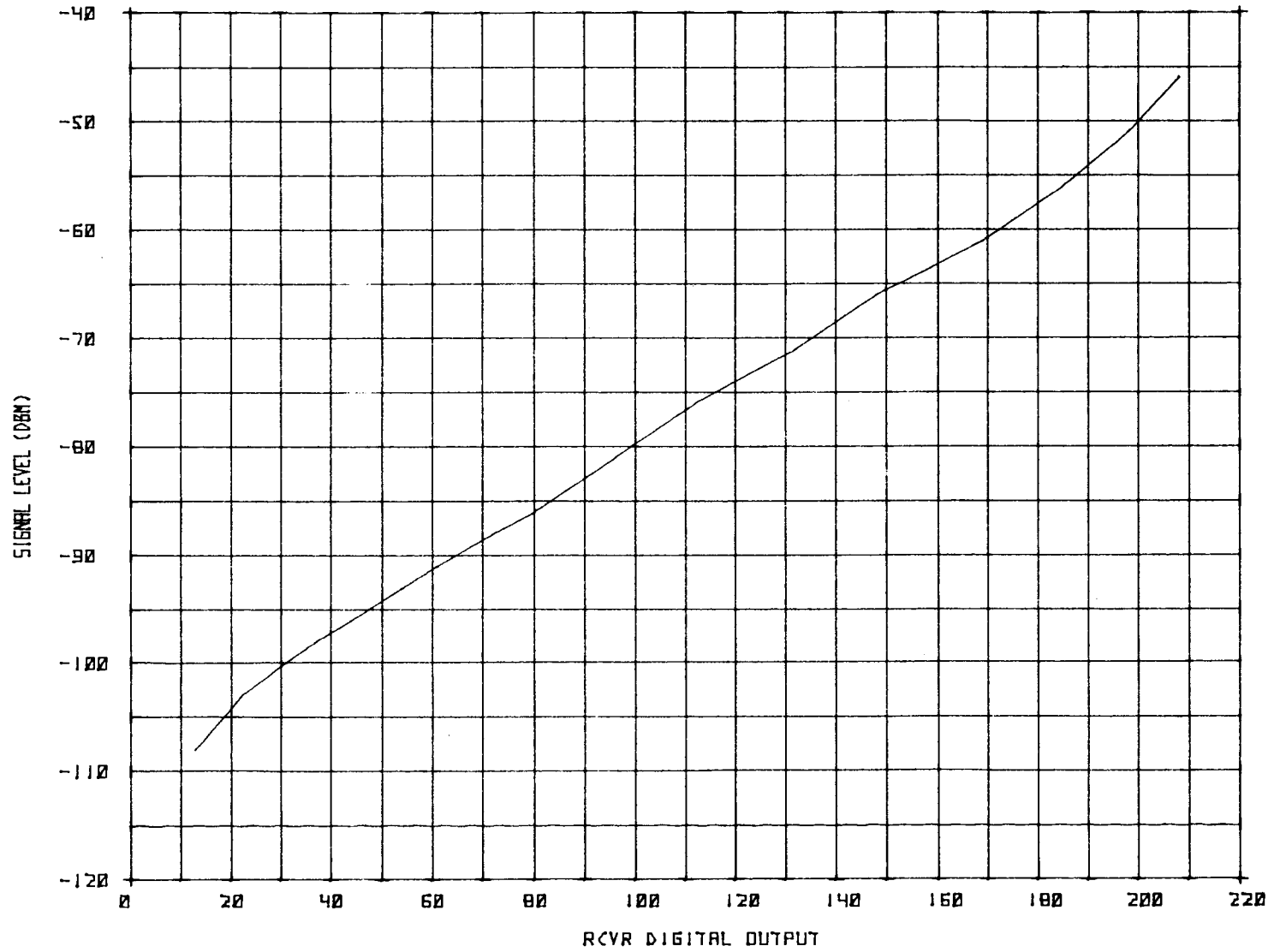
FIGURE 15. RECEIVER CALIBRATION CURVE (S/N SC101)
