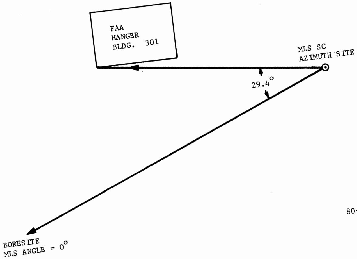
FIGURE 8. SITE 2 (HANGAR) ORIENTATION
