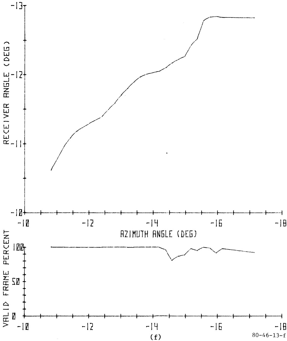
FIGURE 13. AZIMUTH RECEIVER ANGLE VERSUS TRUE AZIMUTH PLOTS USING THE 35 \mu s SQUARE PULSE (SHEET 6 OF 12)
