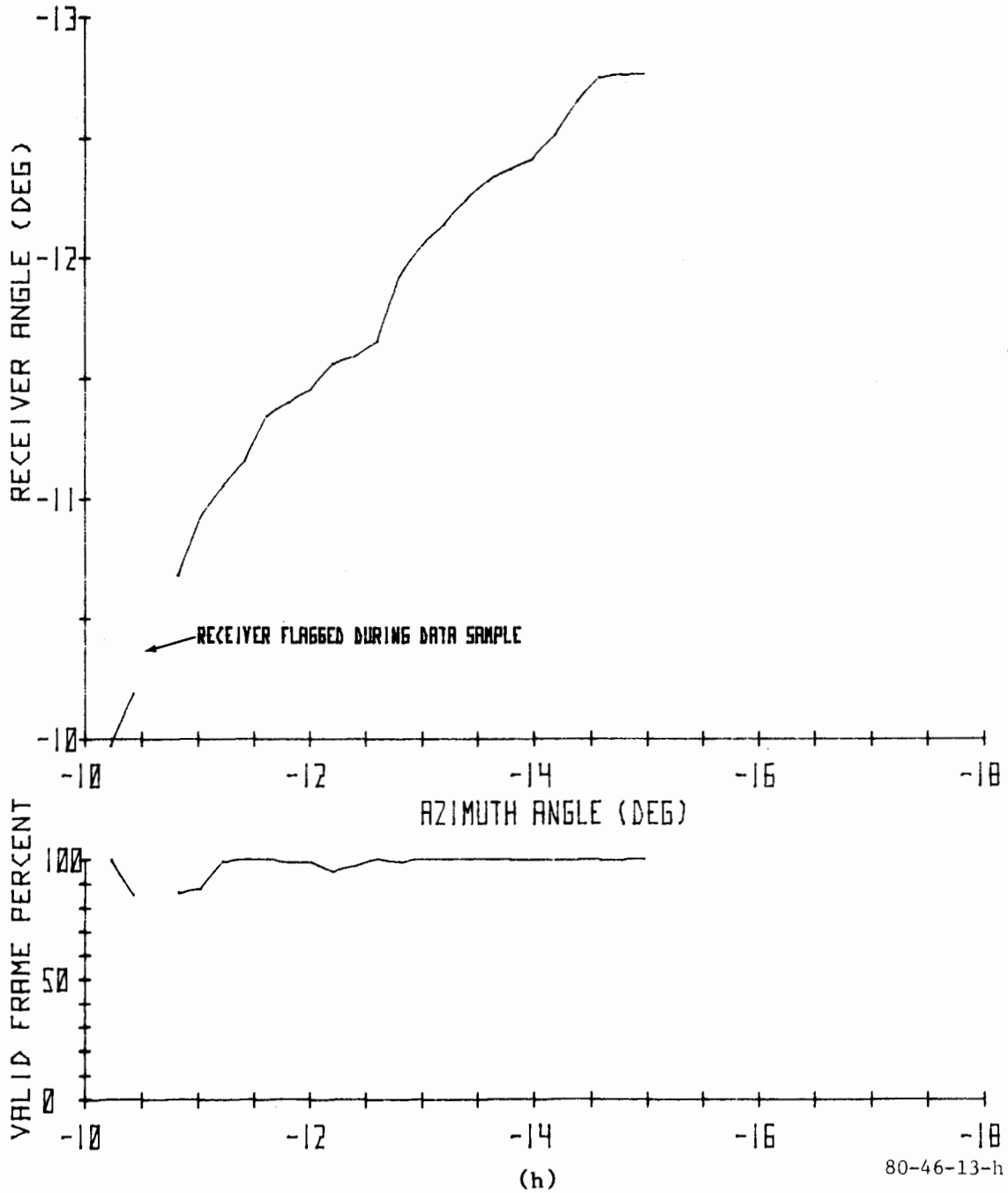
FIGURE 13. AZIMUTH RECEIVER ANGLE VERSUS TRUE AZIMUTH PLOTS USING THE 35 \mu s SQUARE PULSE (SHEET 8 OF 12)
