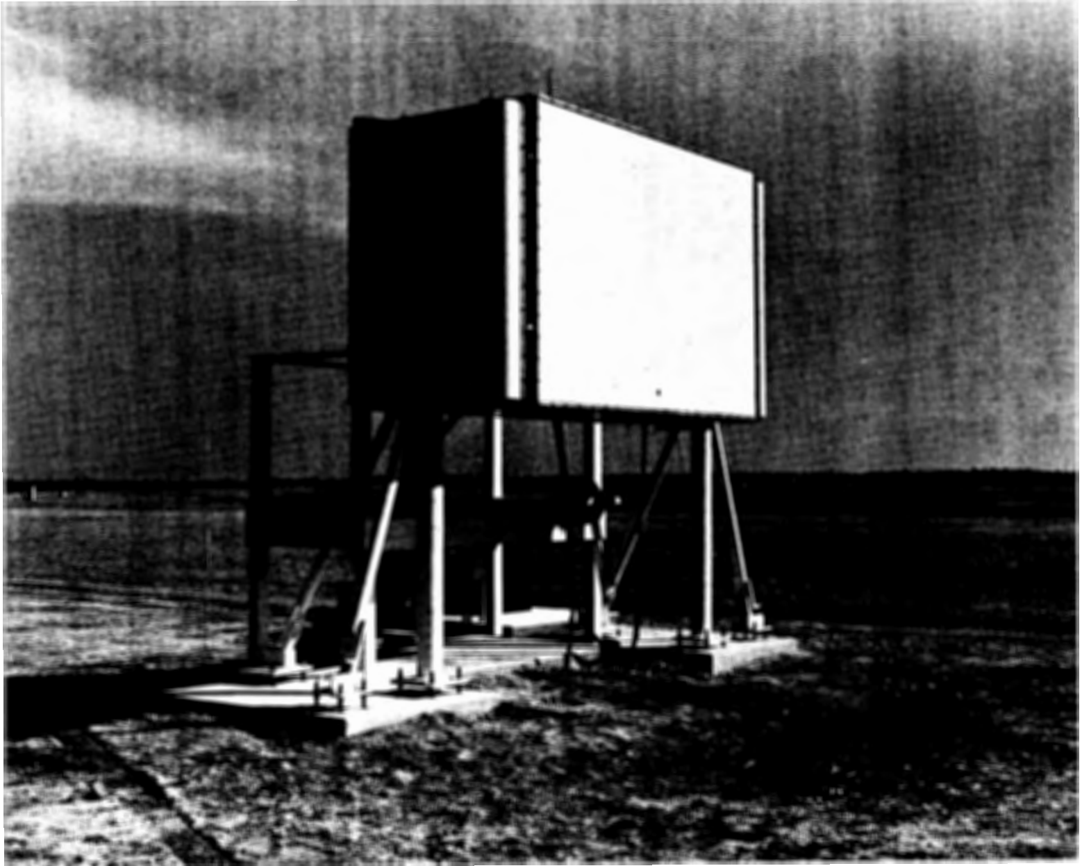
FIGURE 1. BENDIX SMALL COMMUNITY MICROWAVE LANDING SYSTEM AZIMUTH SUBSYSTEM
