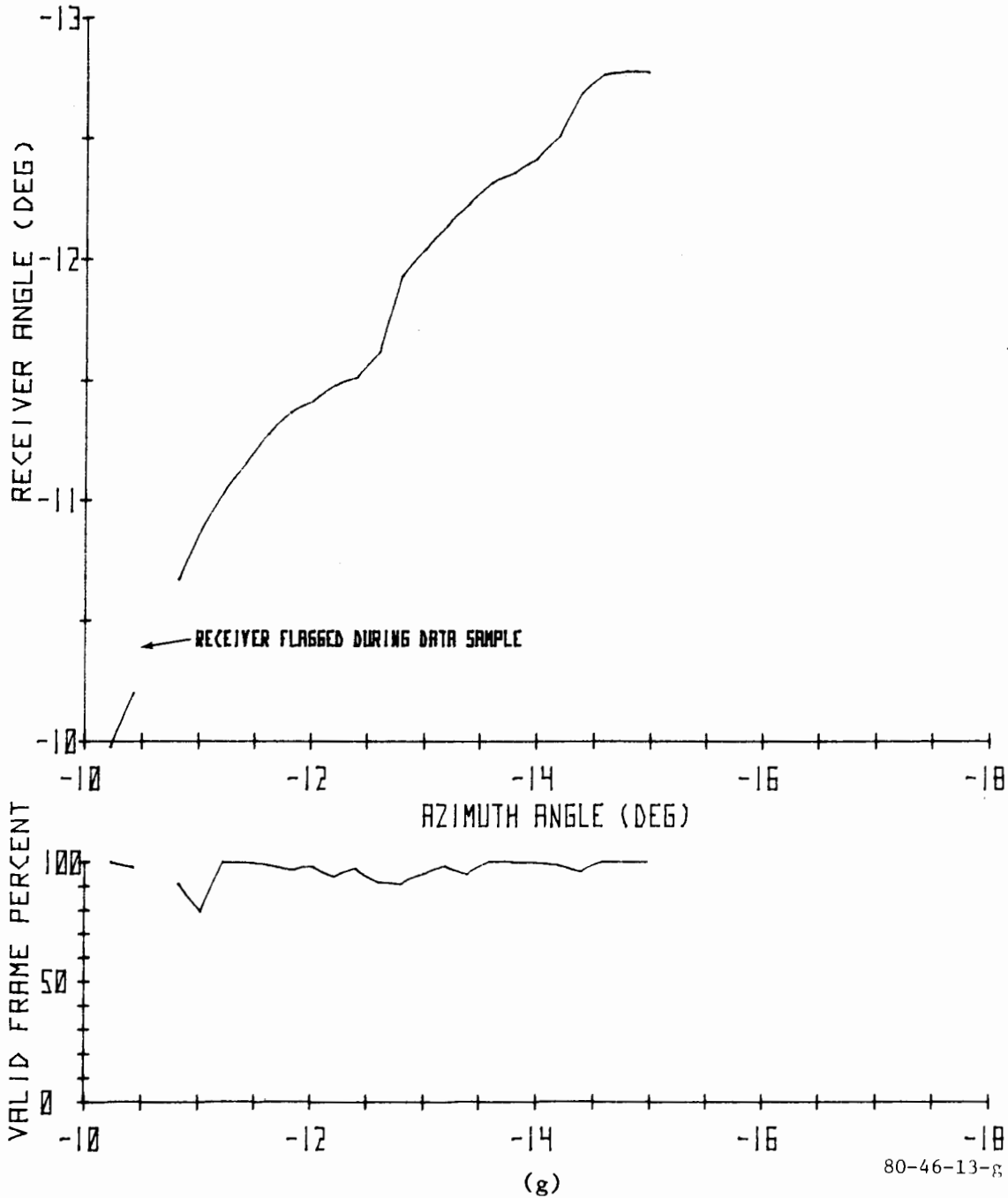
FIGURE 13. AZIMUTH RECEIVER ANGLE VERSUS TRUE AZIMUTH PLOTS USING THE 35 \mu s SQUARE PULSE (SHEET 7 OF 12)
