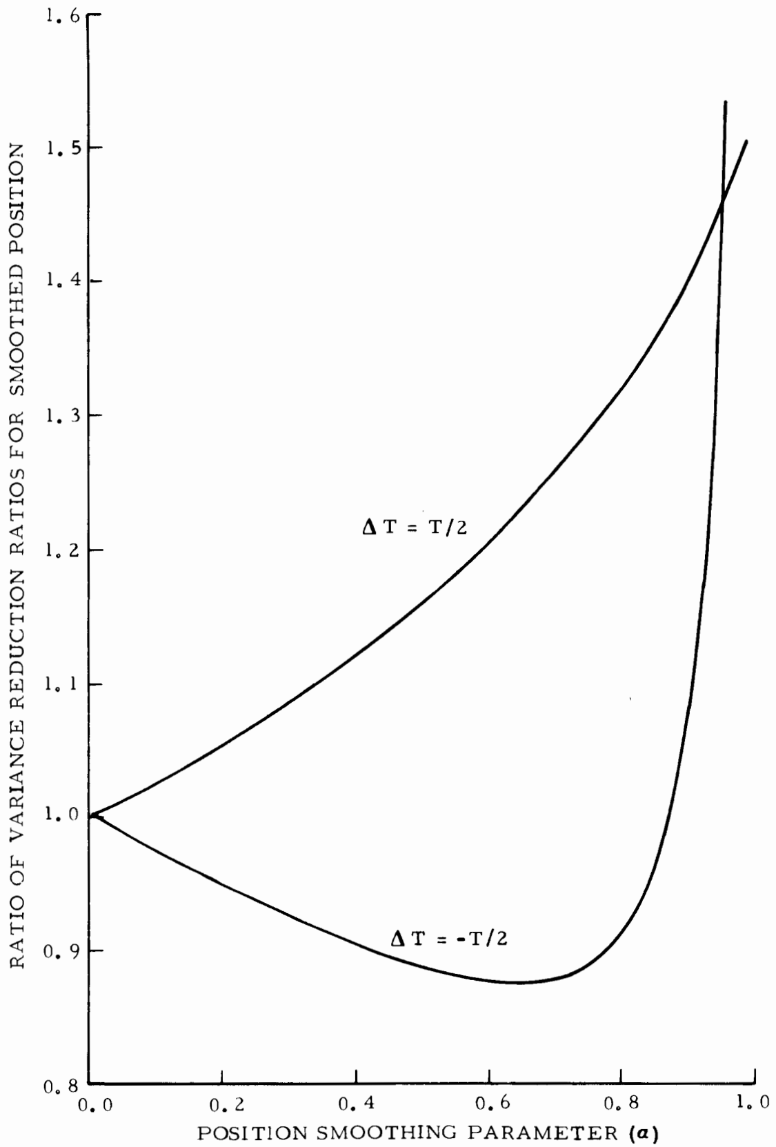
FIGURE 7. PERFORMANCE RATIOS FOR SMOOTHED POSITION
