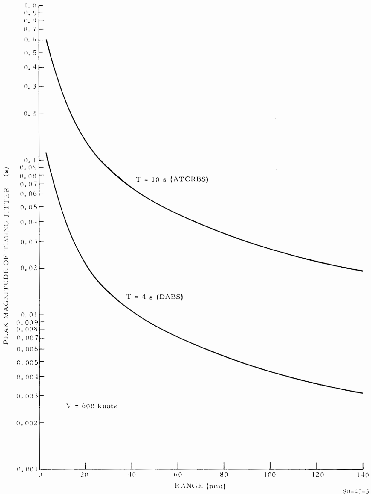
FIGURE 5. PEAK MAGNITUDE OF TIMING JITTER
