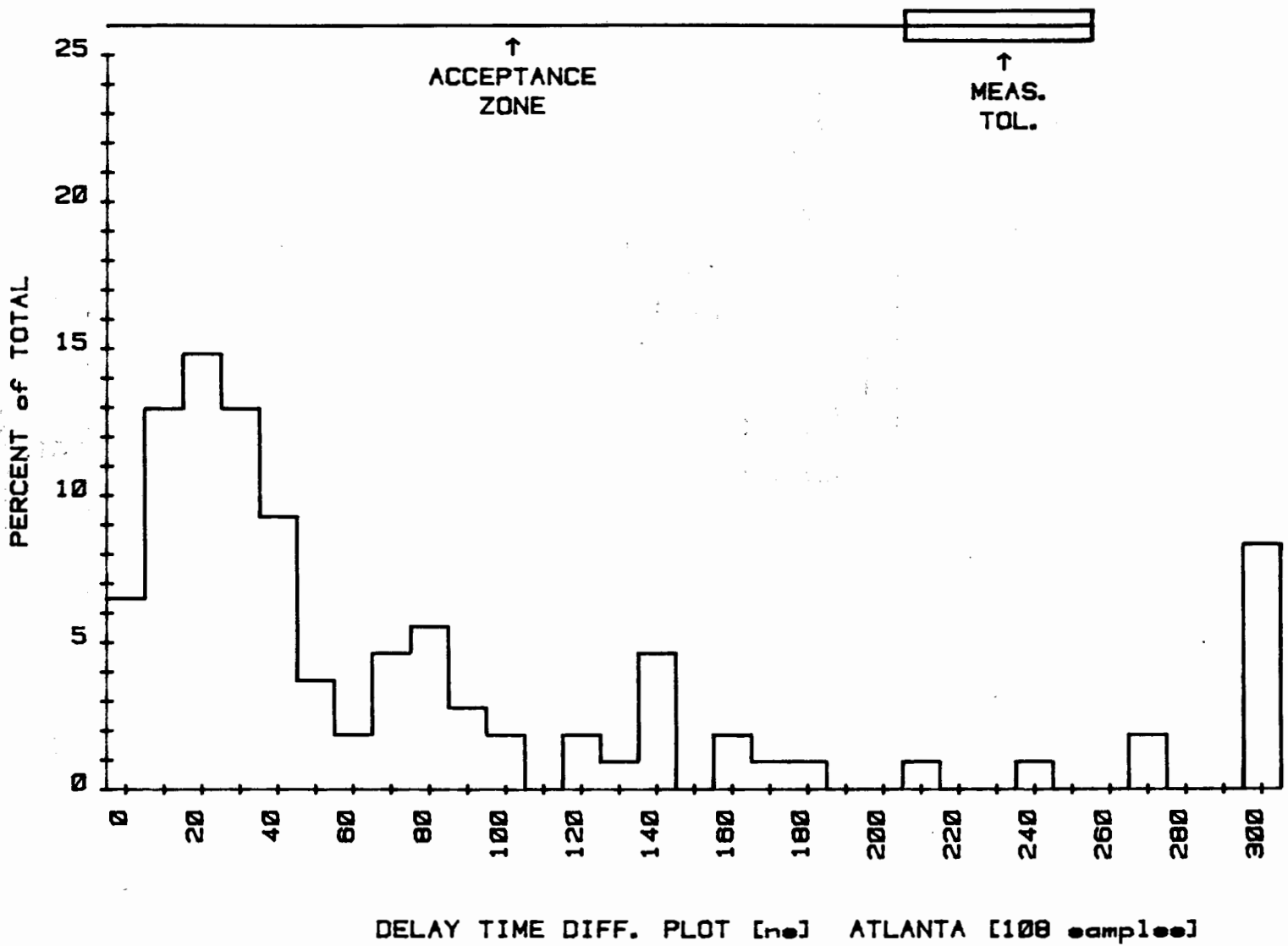
FIGURE 10. BAR GRAPH, DELAY TIME DIFFERENCE PLOT
