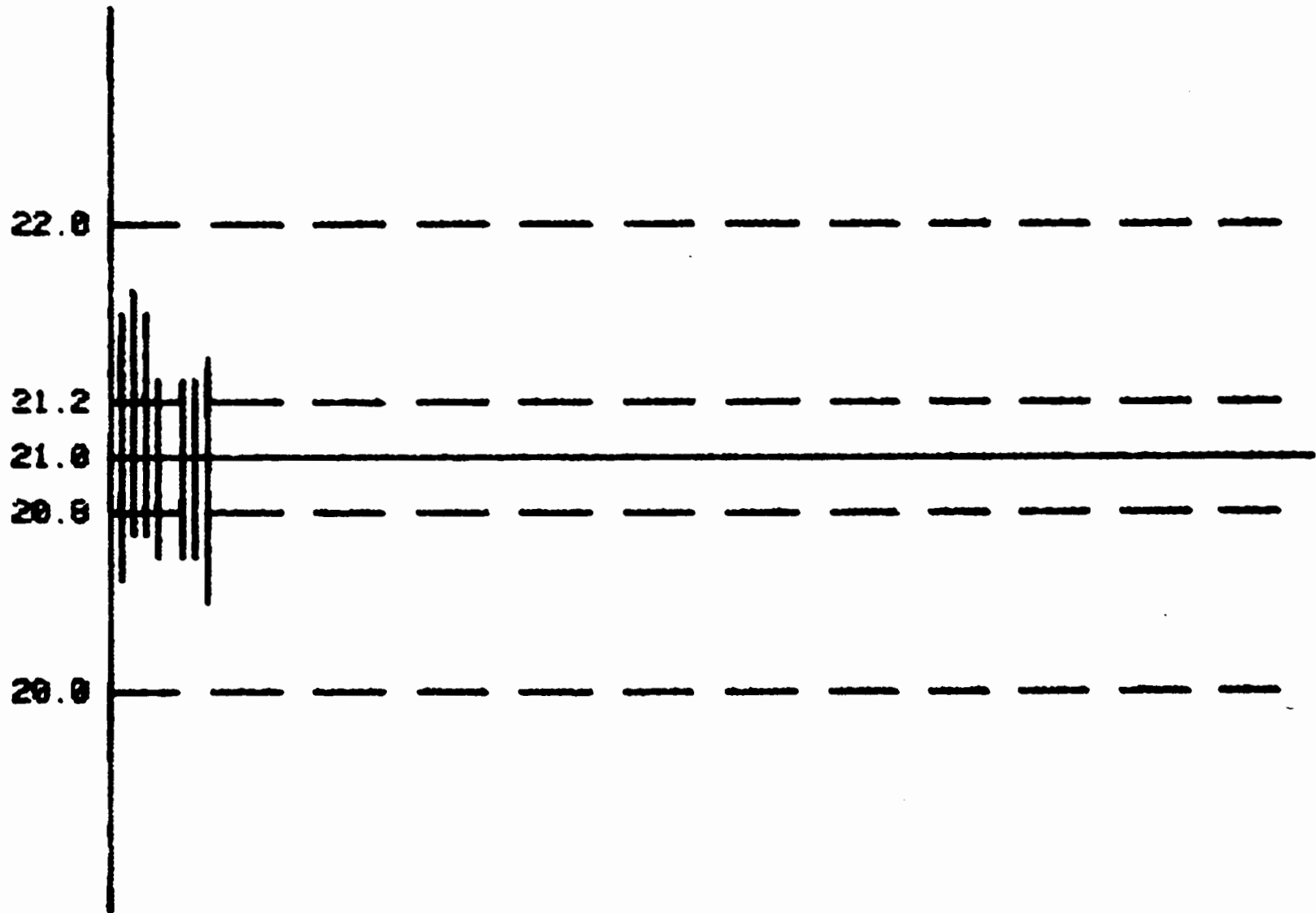
FIGURE 17. MODE C DECODE ACCURACY (Sheet 2 of 2)
