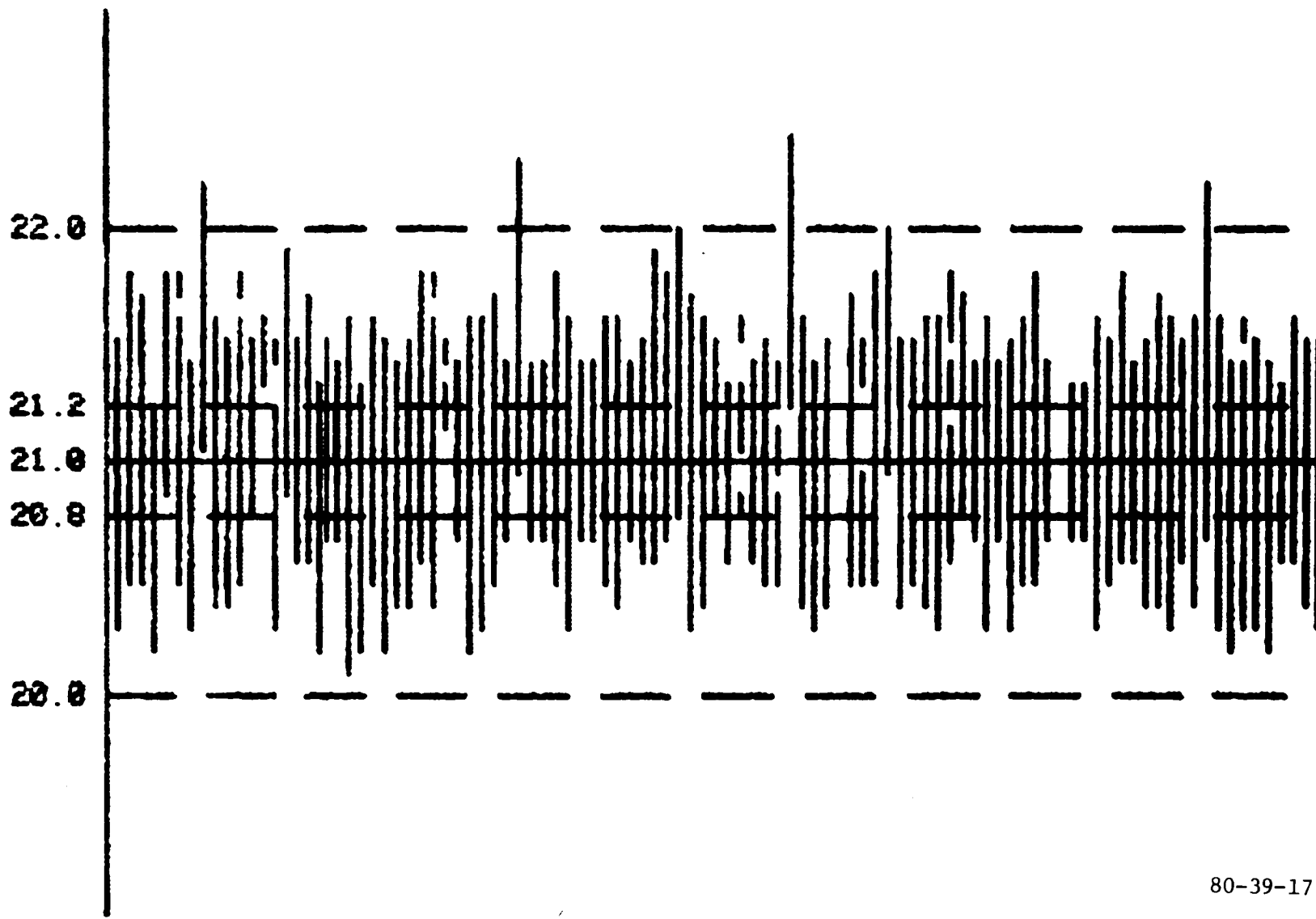
FIGURE 17. MODE C DECODE ACCURACY (Sheet 1 of 2)
