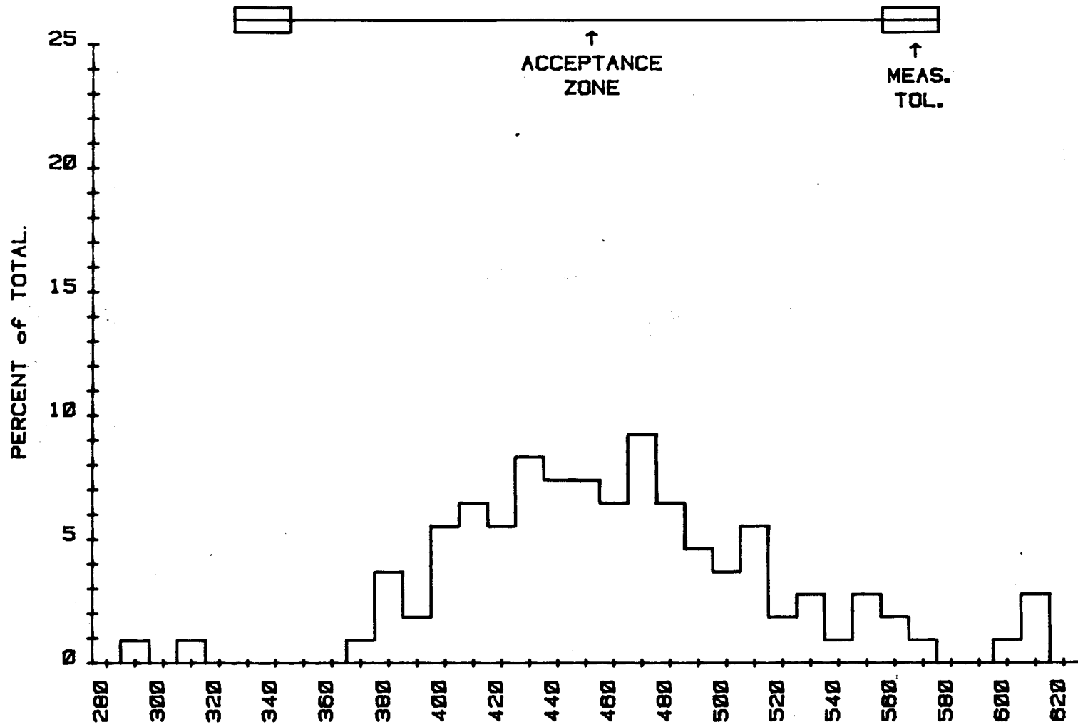
F1 PULSE WIDTH PLOT [ns] ATLANTA [100 samples]
