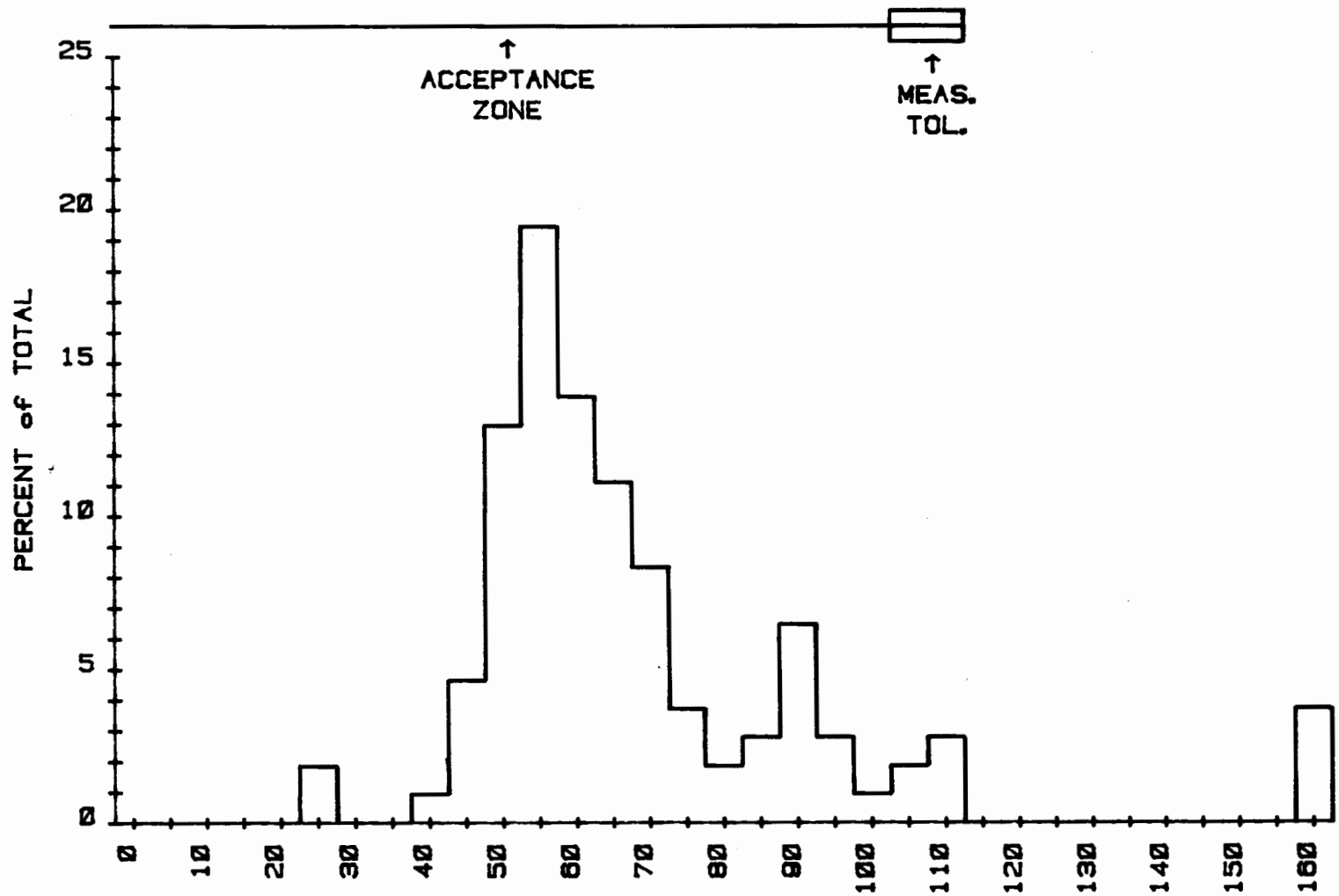
REPLY JITTER PLOT [ns] ATLANTA [100 samples]
