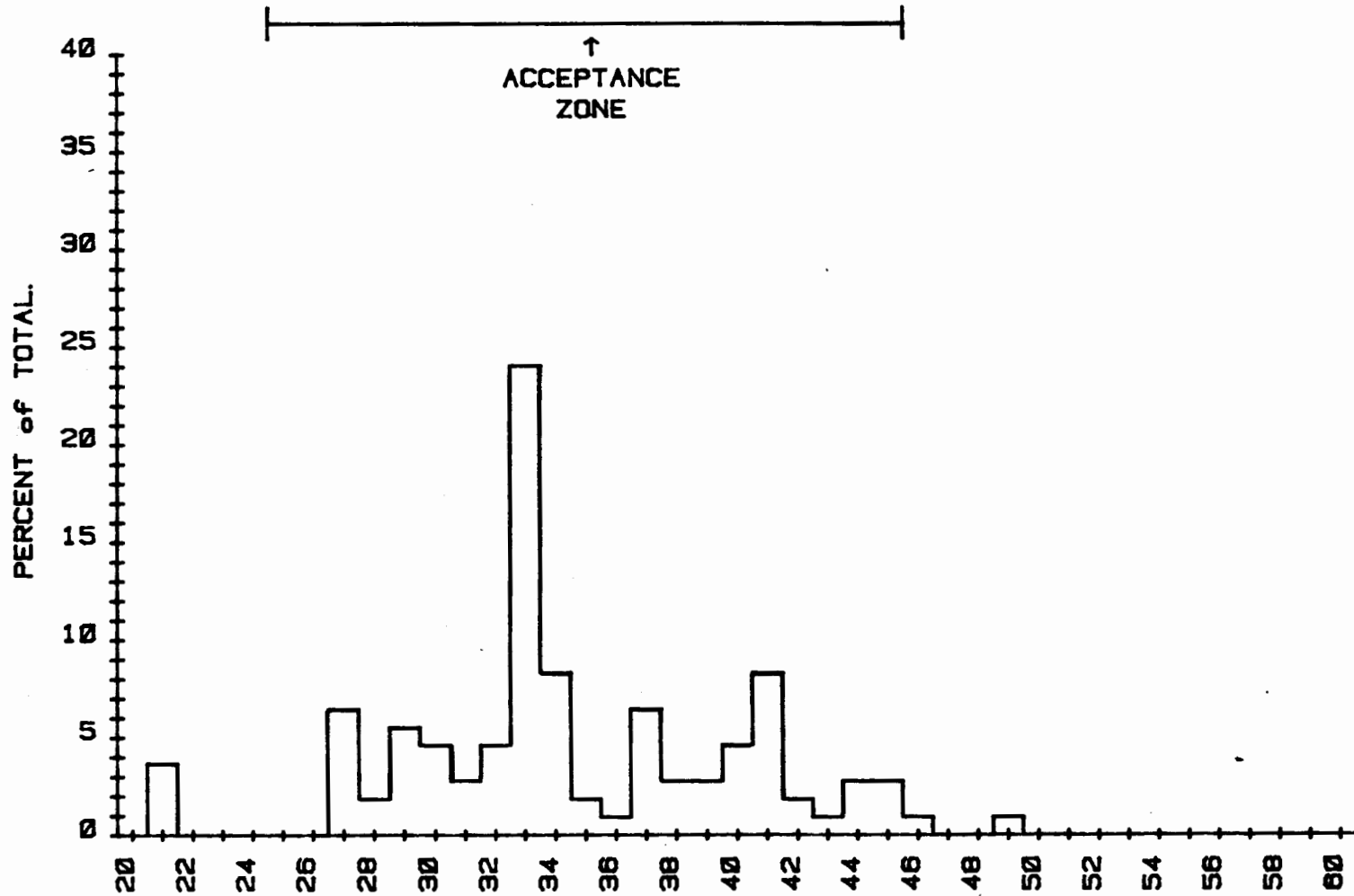
SUPPRESSION TIME PLOT [μs] ATLANTA [108 samples]
