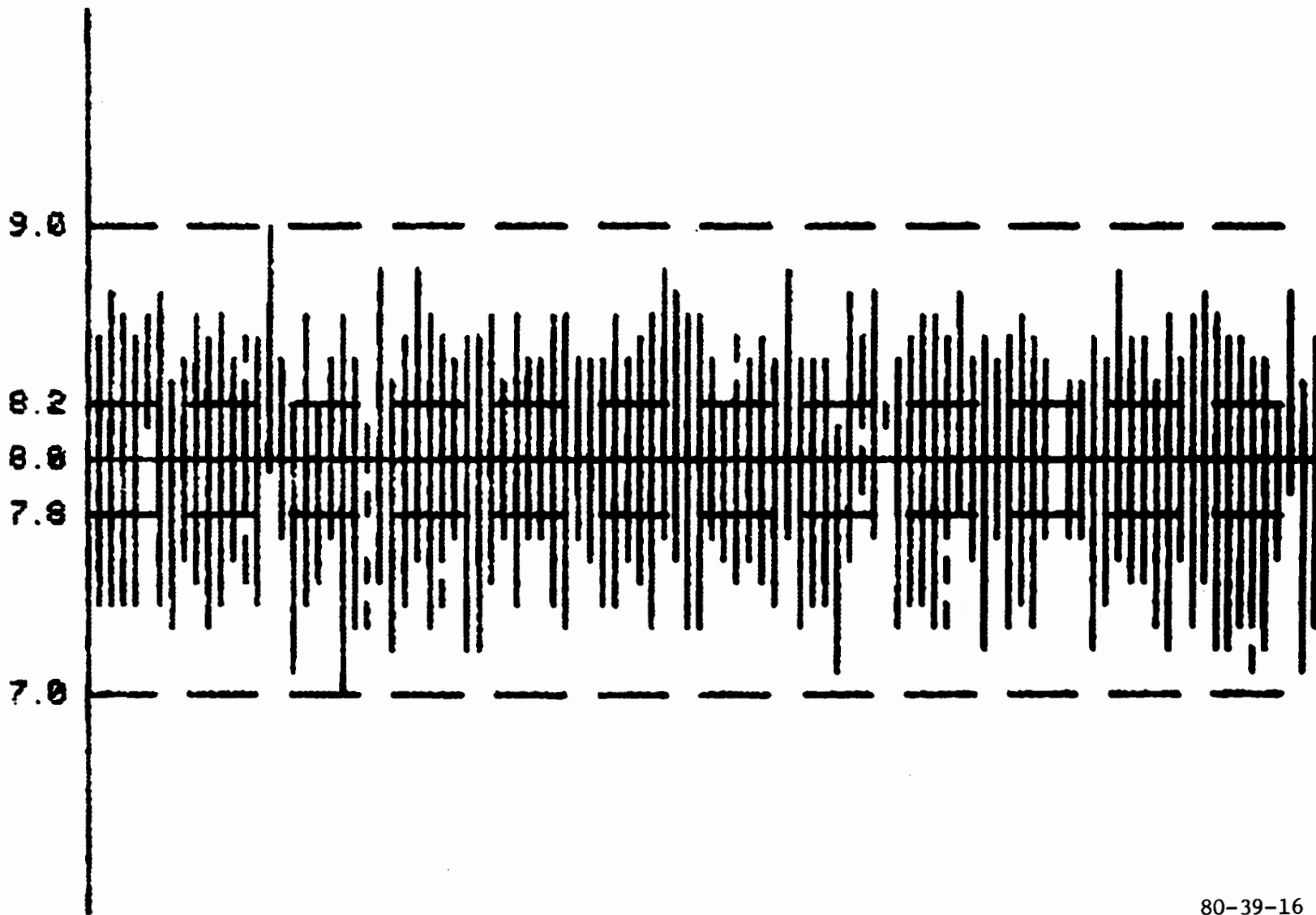
FIGURE 16. MODE 3/A DECODE ACCURACY (Sheet 1 of 2)
