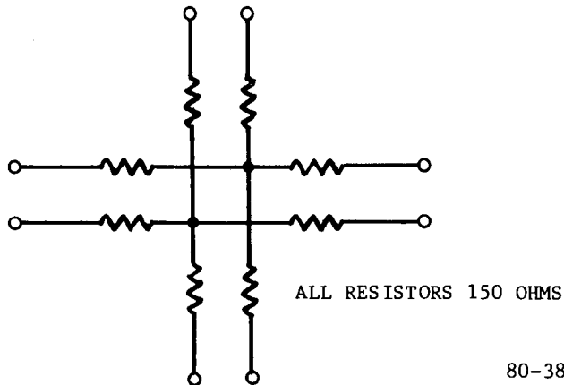
4-WAY COMBINER
