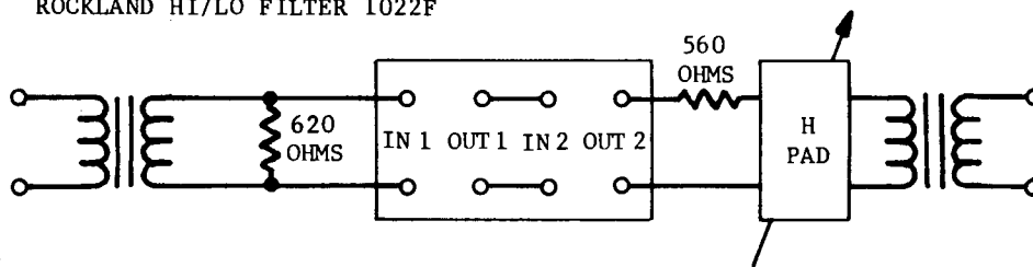
TELEPHONE LINE SIMULATOR
