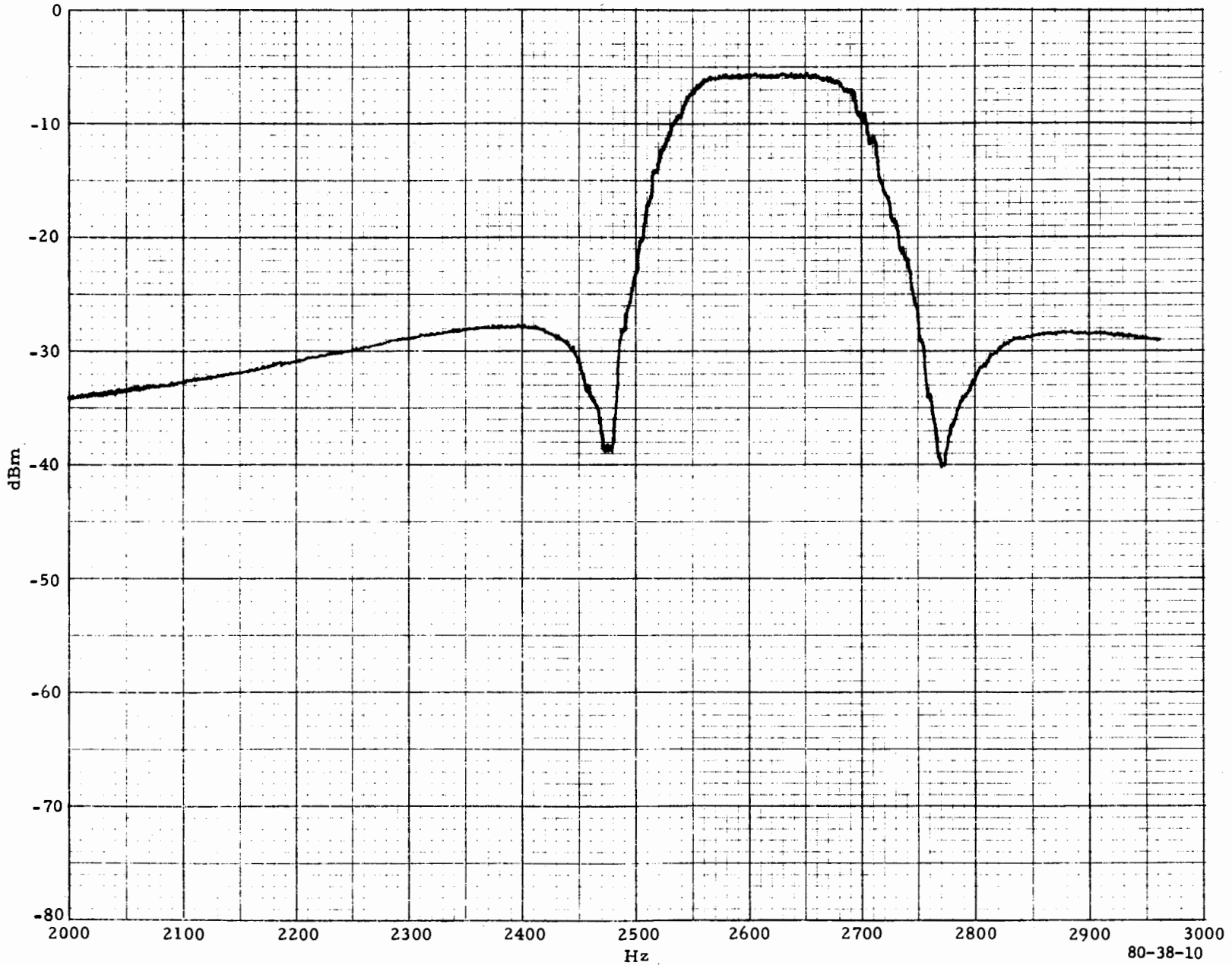
FIGURE 10. RMS MODEM RECEIVE FILTER FREQUENCY RESPONSE (110-BAUD)
