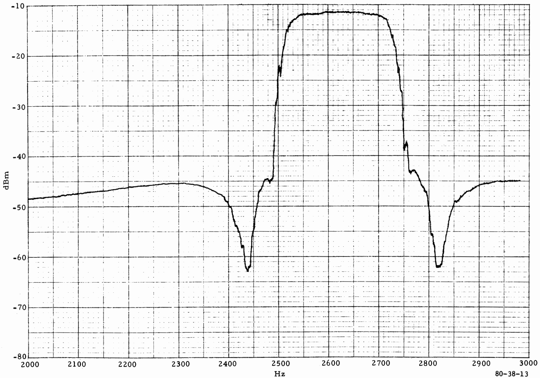
FIGURE 13. BANDPASS FILTER FREQUENCY RESPONSE
