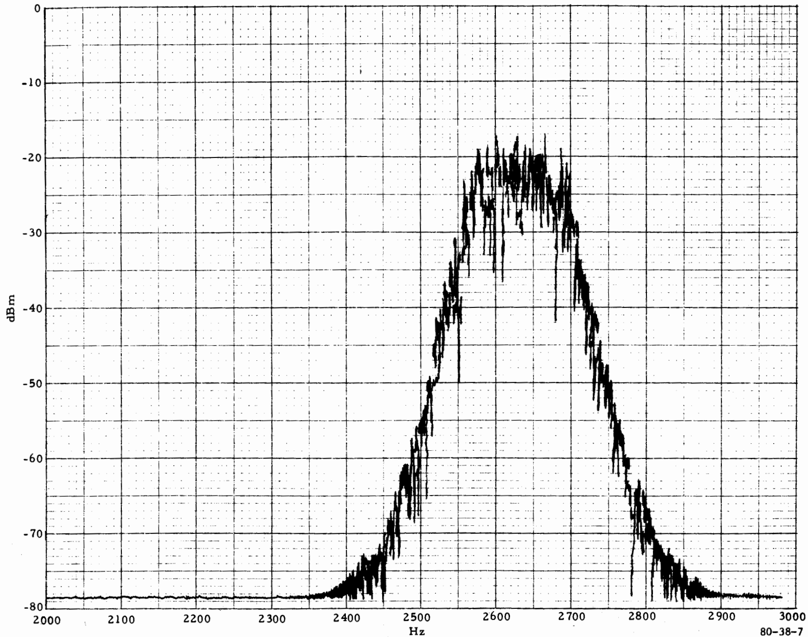
FIGURE 7. SPECTRUM OF 110-BAUD RANDOM RMS DATA
