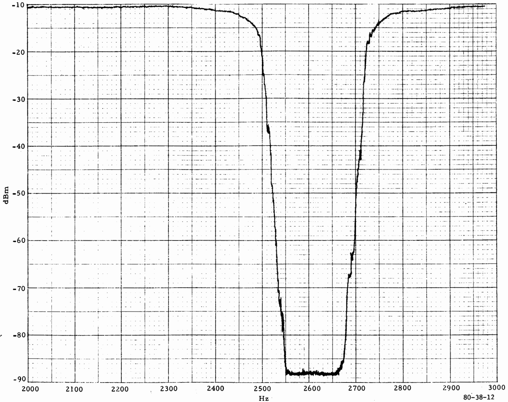
FIGURE 12. NOTCH FILTER FREQUENCY RESPONSE
