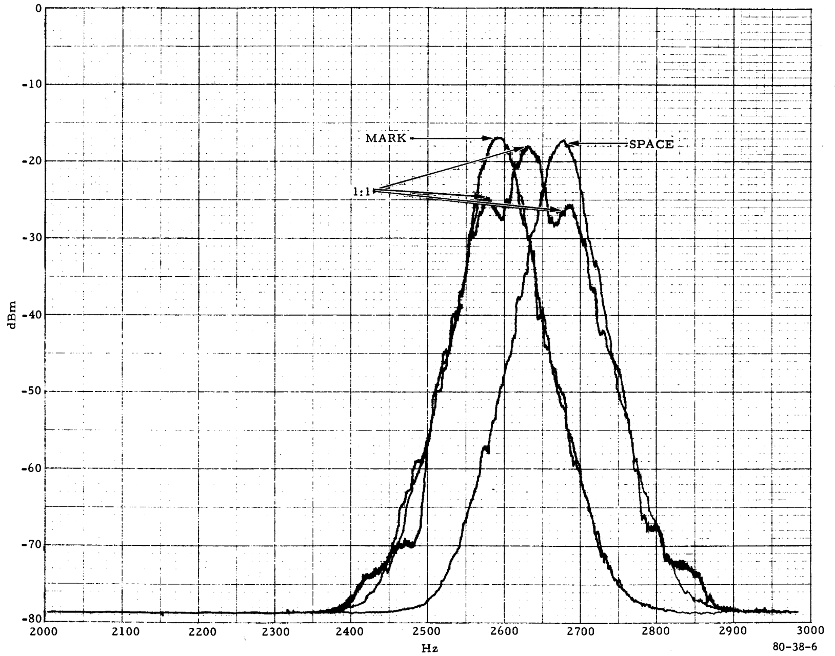
FIGURE 6. SPECTRUM OF 110-BAUD MARK, SPACE, AND 1:1 RMS DATA
