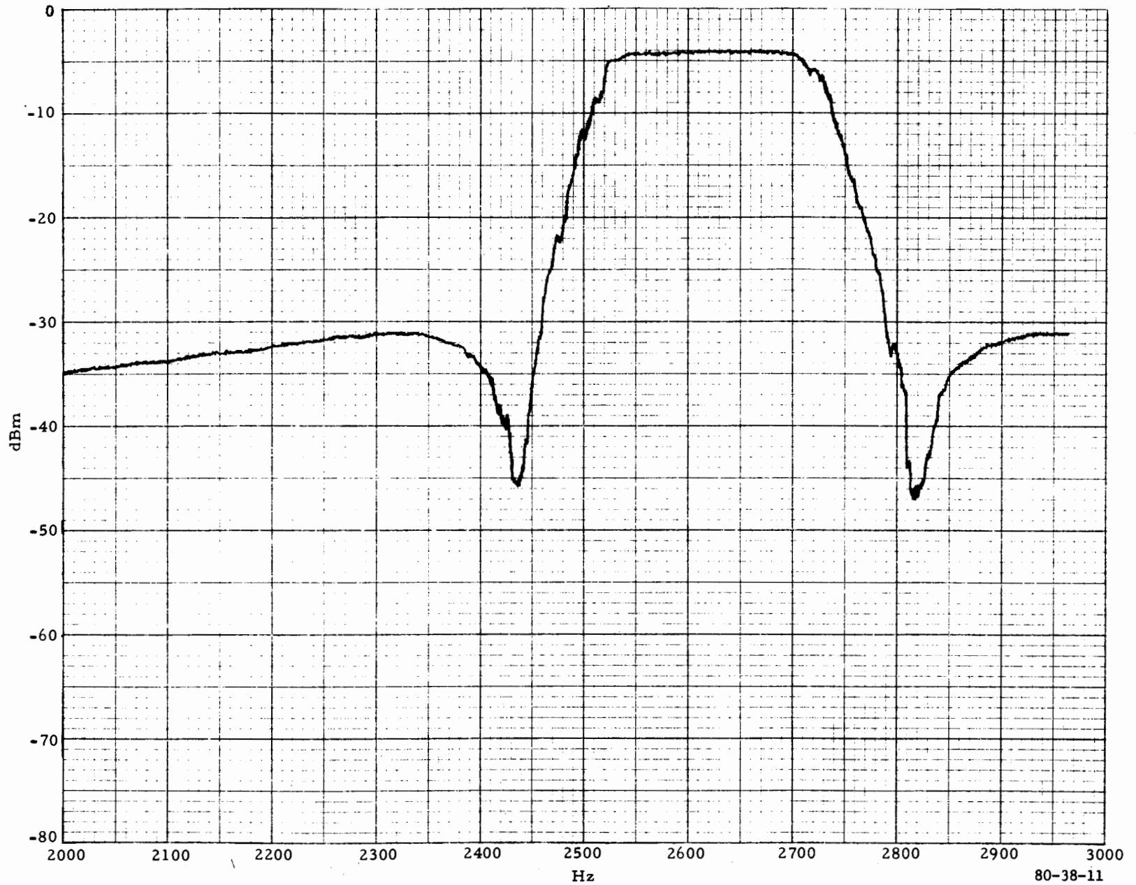
FIGURE 11. RMS MODEM RECEIVE FILTER FREQUENCY RESPONSE (150-BAUD)
