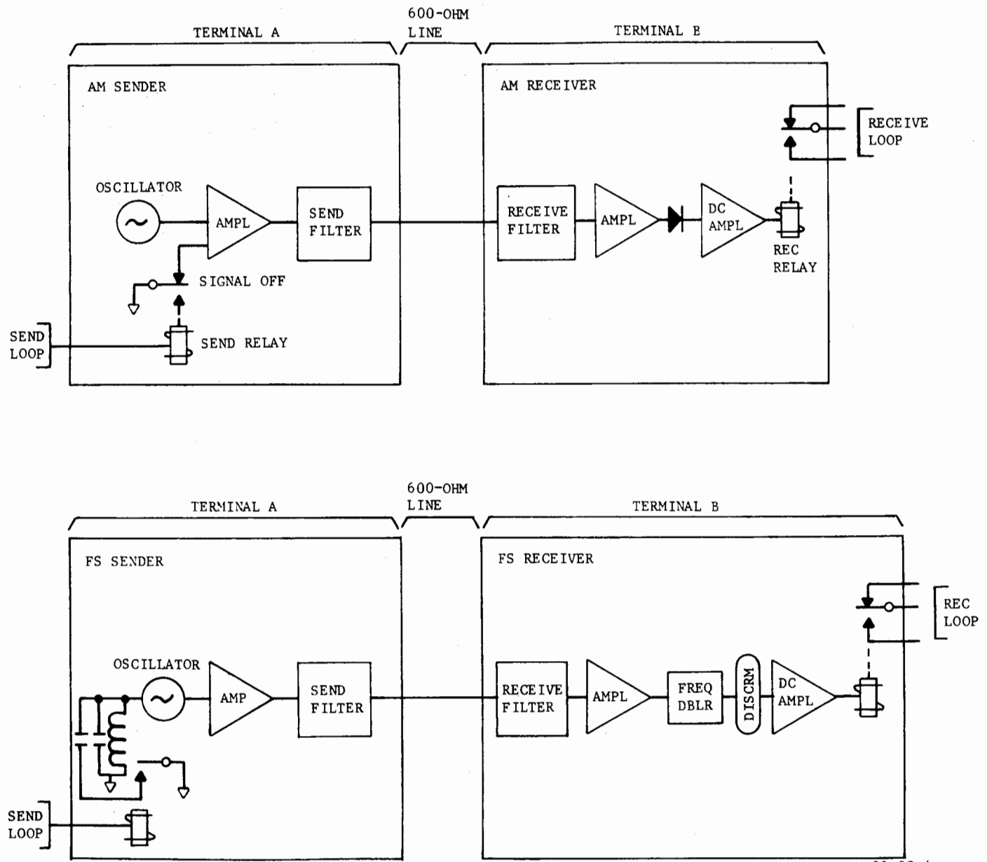
FIGURE 4. FS AND AM SENDER OPERATIONAL DIAGRAM
