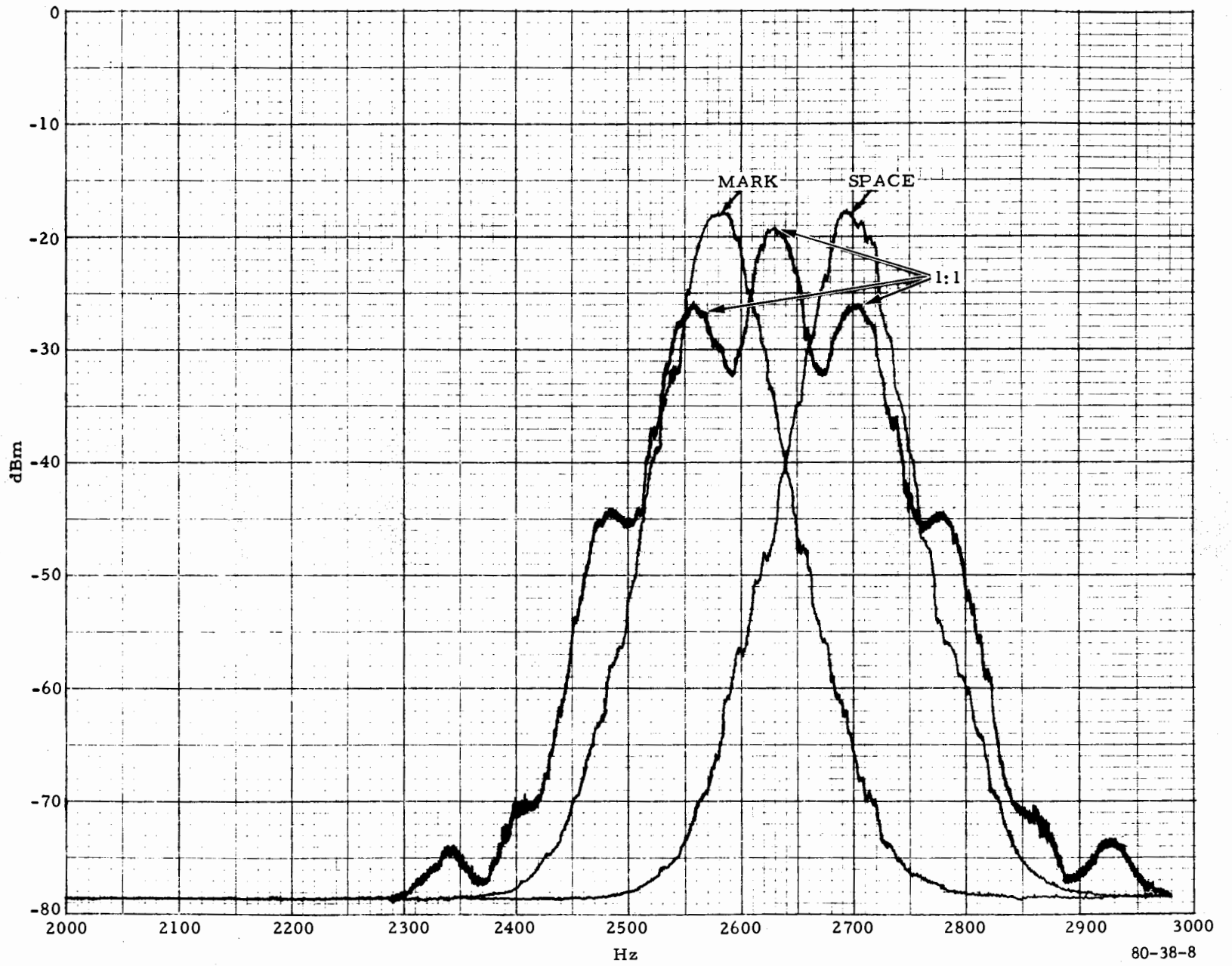
FIGURE 8. SPECTRUM OF 150-BAUD MARK, SPACE, AND 1:1 RMS DATA
