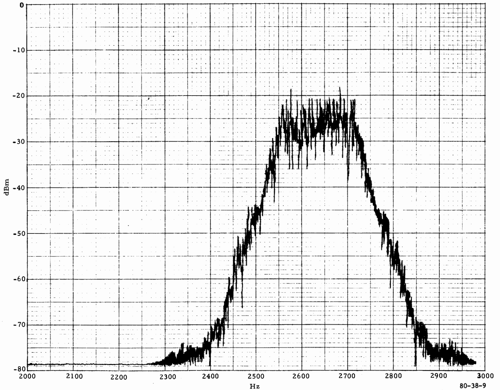
FIGURE 9. SPECTRUM OF 150-BAUD RANDOM RMS DATA
