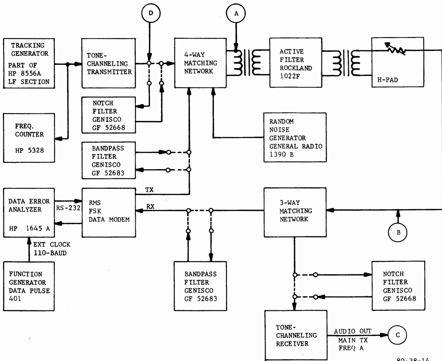
FIGURE 14. TEST SETUP
