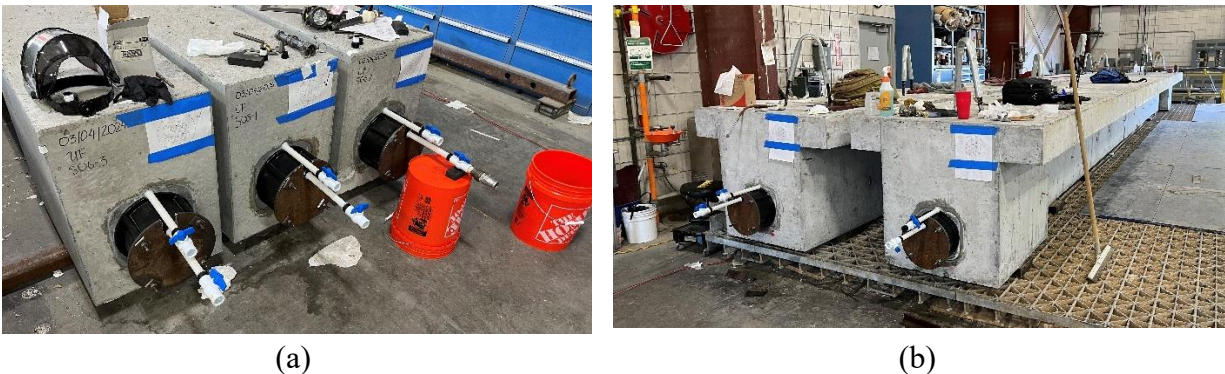
Figure 6.12. Plumbing of beams for injection of grout: (a) S06 beams PT dead end (b) S19 beams PT live end.
