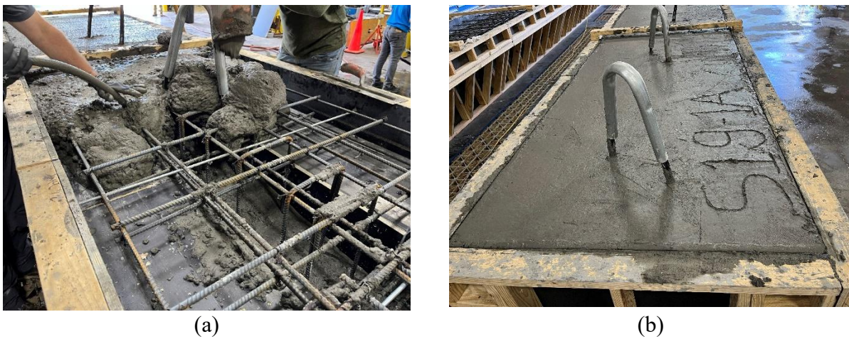
Figure 6.8. Casting of S19 beams: (a) Placement and vibration of second lift; (b) Finished surface after casting.
