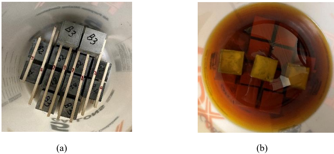
Figure 7.2. Grout cubes soaked in corrosion inhibitor fluid: (a) Stacked for soaking; (b) Immediately after immersion.
