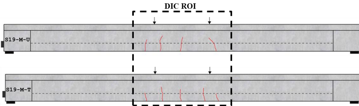
Figure 10.7. Crack map showing the observed cracks on the east face of the S19 beam specimens at the cracking load (concrete tensile stress at 12\sqrt{f'_c} ).
