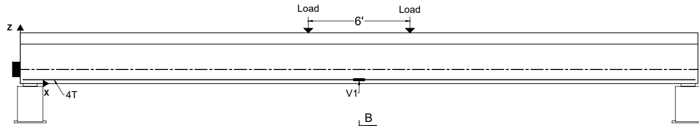
Elevation View (East)
