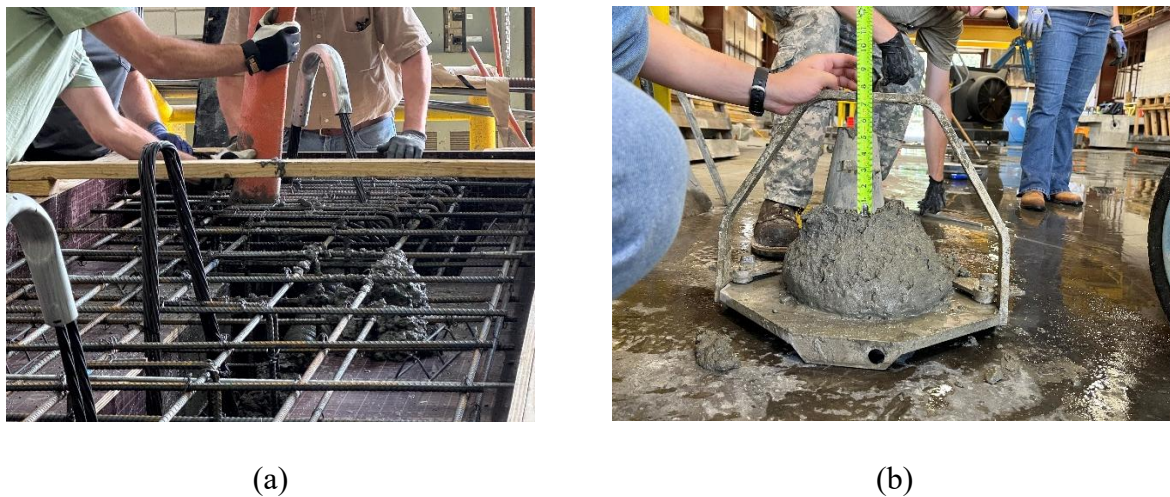
Figure 6.9. Casting of D19 beams: (a) Pumping of concrete in the end-block region of the D19-P-U beam; (b) Slump testing of concrete obtained from the truck before pumping into the S19-M-U beam.
