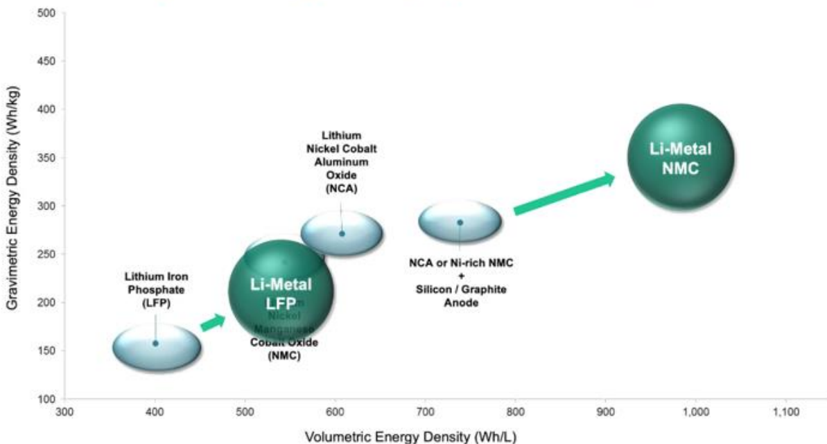
Figure 4. Characteristics of lithium metal, anode-free (QuantumScape, USA [7]).
