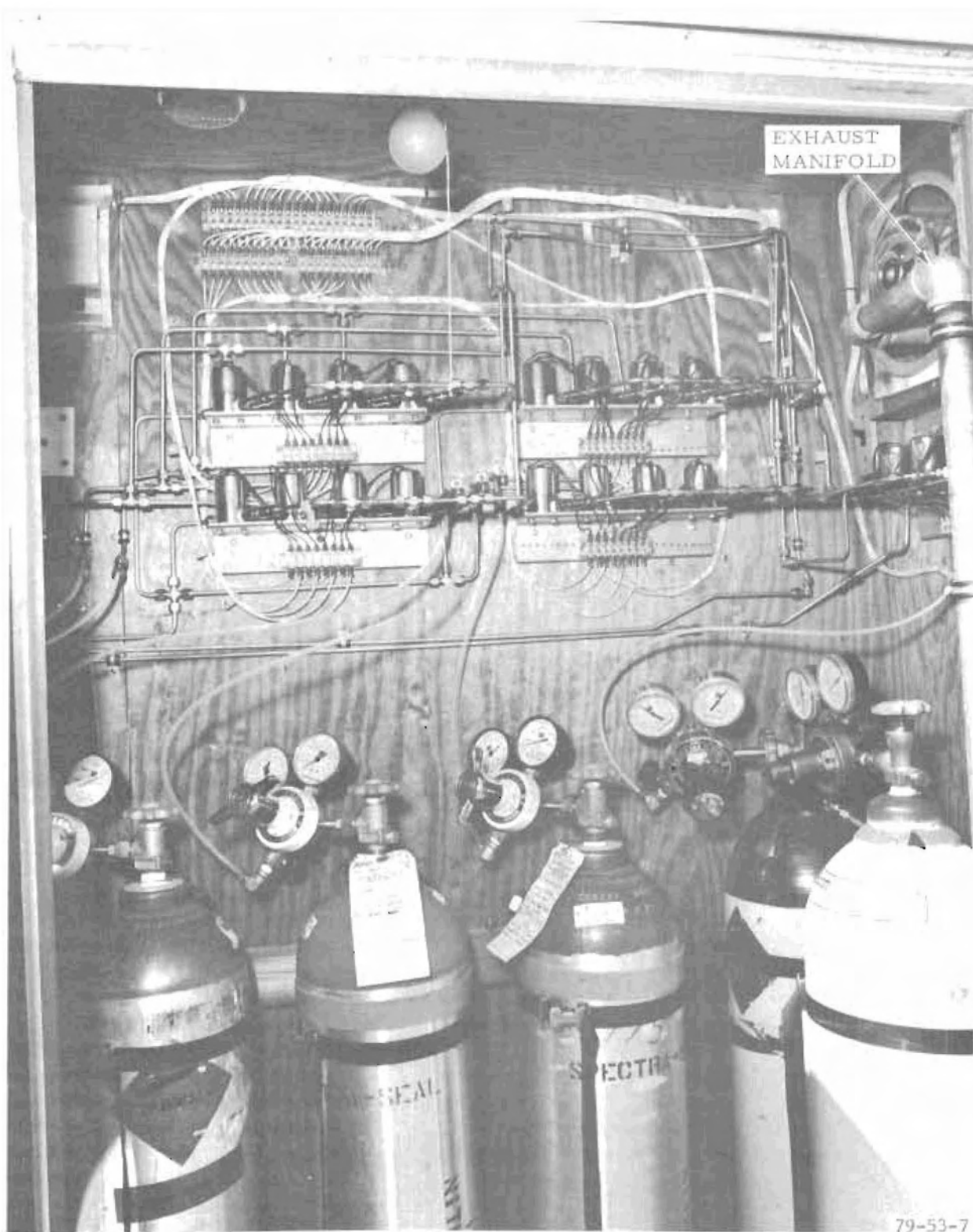
FIGURE D-3. MERF BOTTLE COMPARTMENT--OPERATING/REFERENCE GAS
