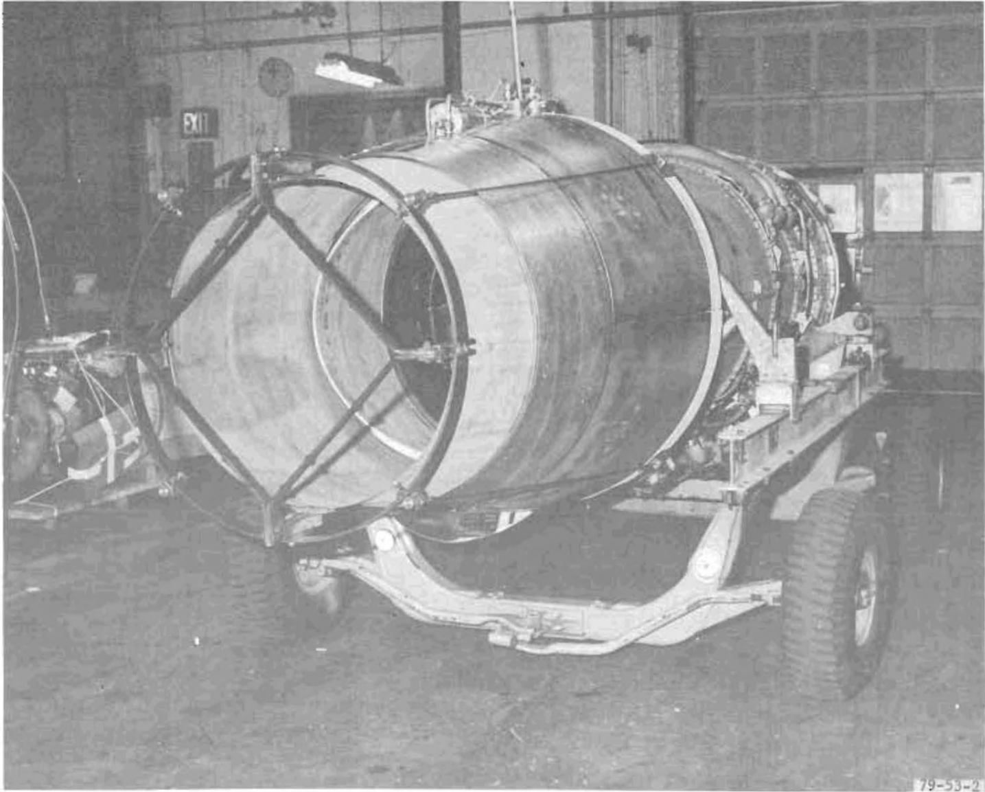
FIGURE 1. QUARTERING VIEW OF FAA EMISSION MEASUREMENT PROBE (DIAMOND SHAPED) INSTALLED ON THE EXHAUST NOZZLE OF A JT8D-7A TURBOFAN ENGINE
