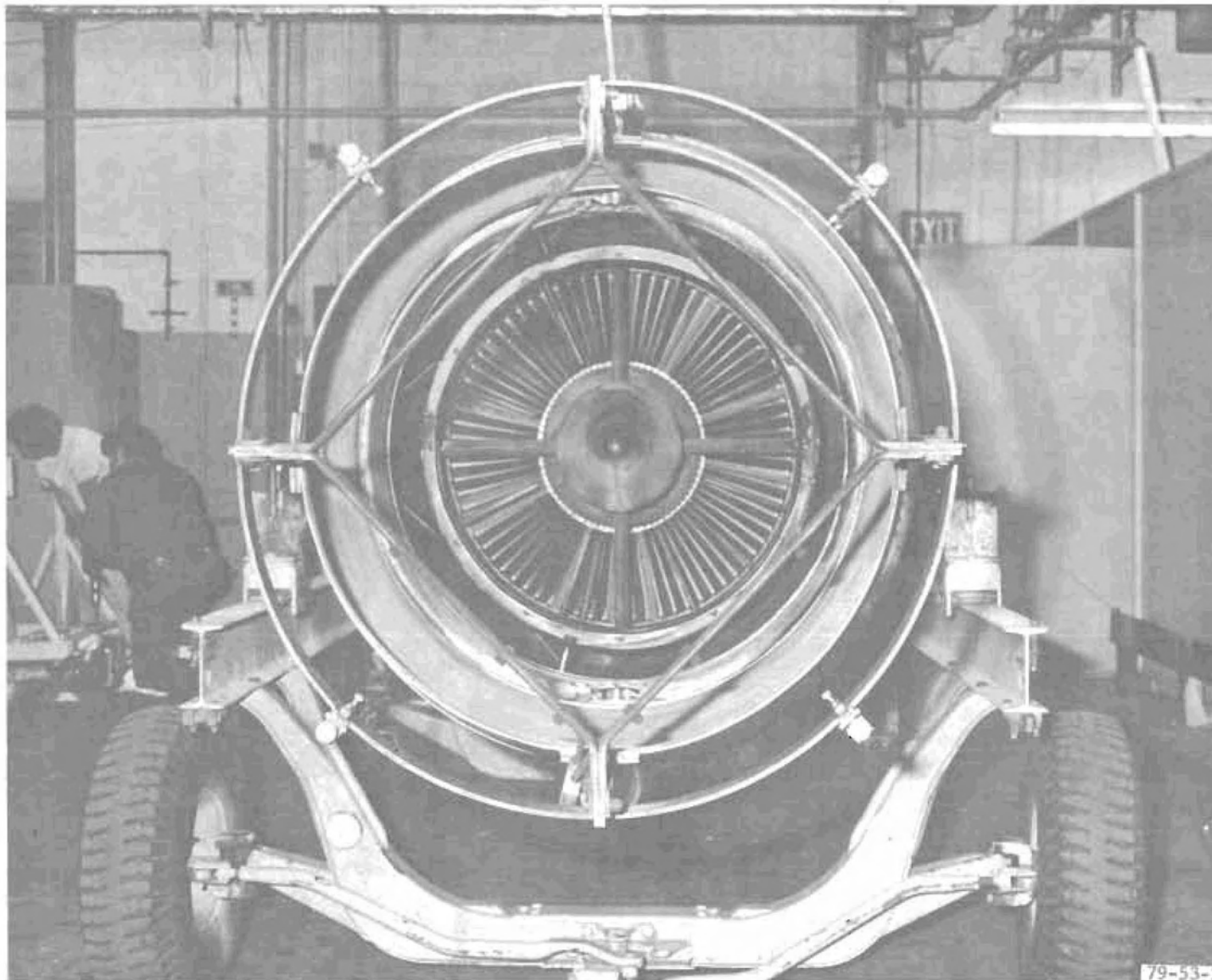
FIGURE 2. VIEW LOOKING FORWARD--INSTALLATION OF FAA EMISSION MEASUREMENT PROBE (DIAMOND SHAPED) INSTALLED ON THE EXHAUST NOZZLE OF A JT8D-7A TURBOFAN ENGINE
