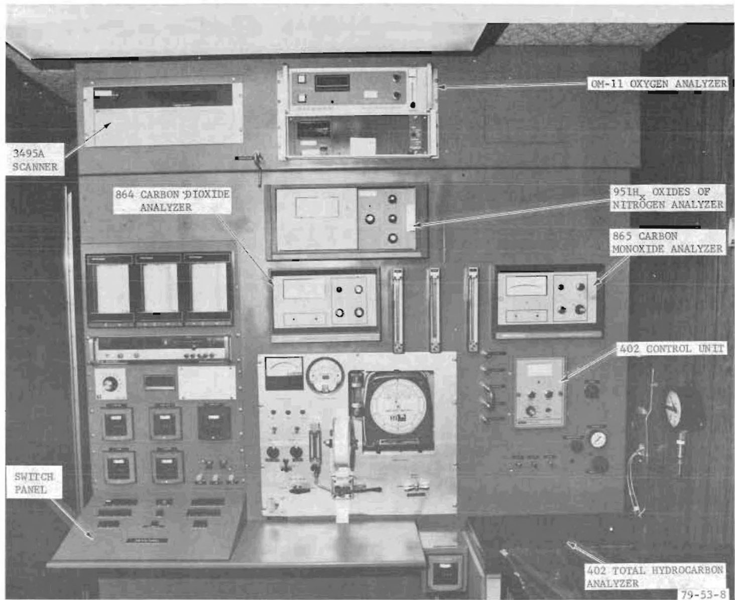
FIGURE D-2. GAS ANALYZERS IN THE MERF OPERATORS COMPARTMENT
