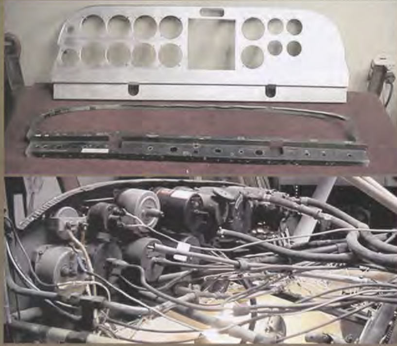
Making Order Out of Chaos: How do you bring a basic VFR 1953 Piper Tripacer panel with its one communications/navigation unit and almost half century old instruments into the 21st Century? An owner-produced part is one answer such as this new IFR instrument panel being designed for a new GPS/comm/nav system and instruments.
