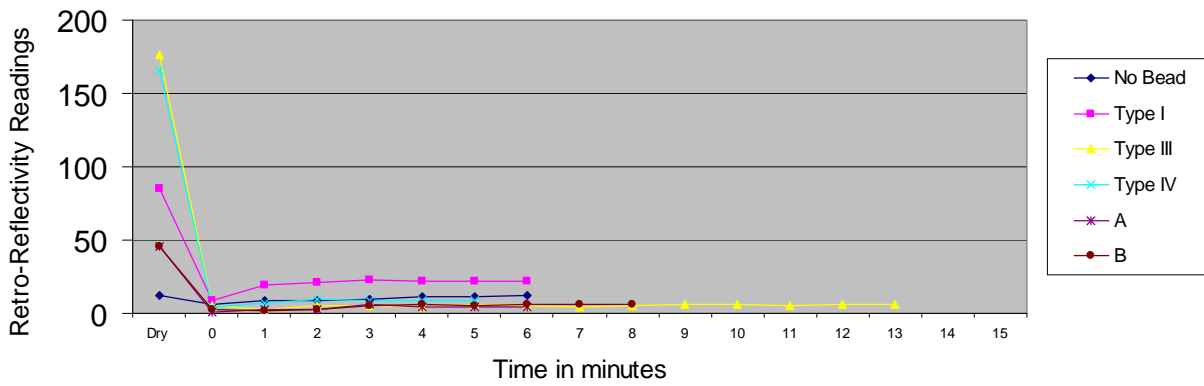
Figure 25. Recovery Test on New HMA
