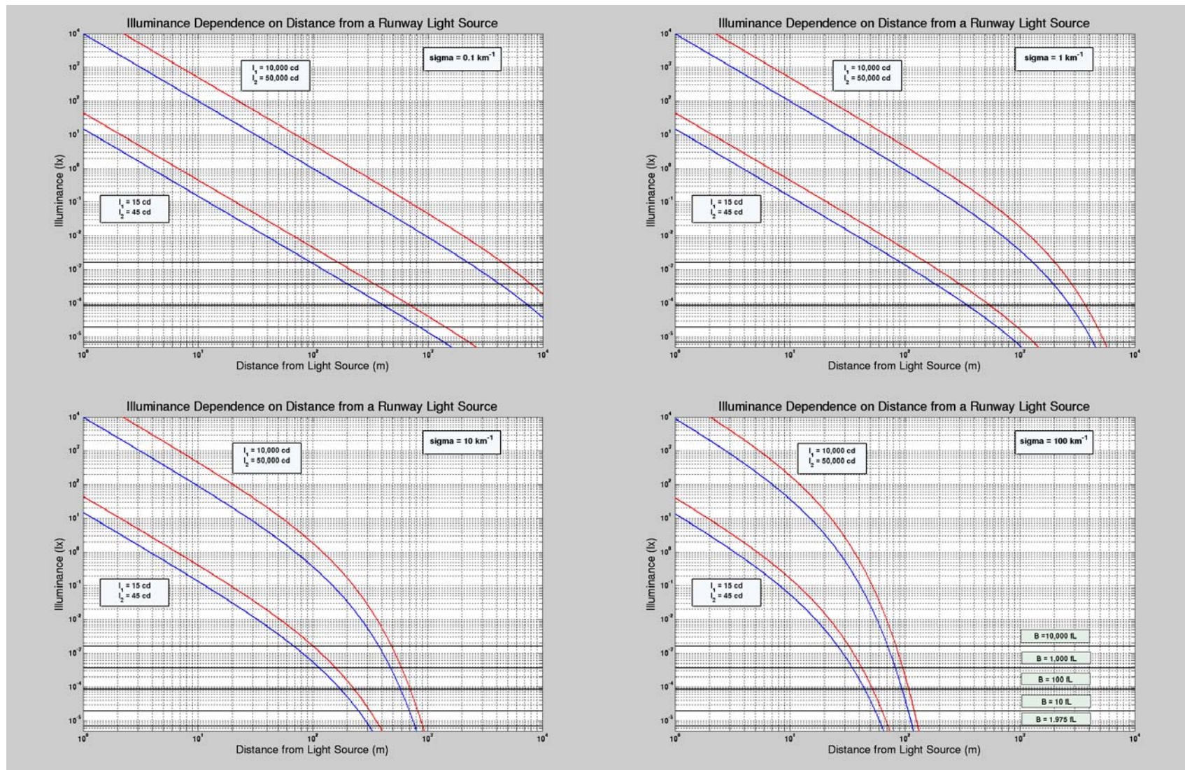
Figure 13. Four Plots of Illuminance Dependence on Distance From a Runway Light Source
