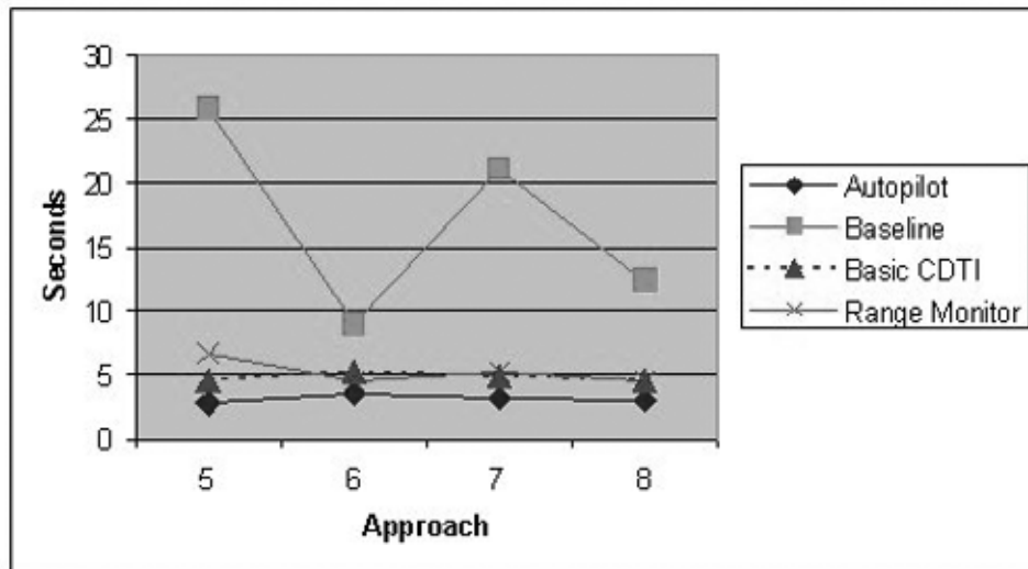
Figure 7. Instrument panel dwell time for IFR approaches.
