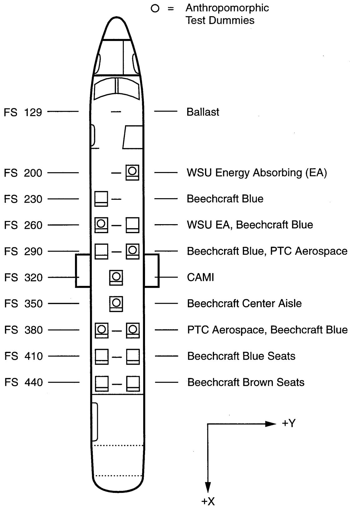
FIGURE 2. BEECHCRAFT 1900C AIRLINER
