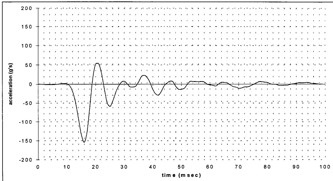
FIGURE 4. FS 290 RIGHT WALL, SEAT TRACK VERTICAL ACCELERATION
