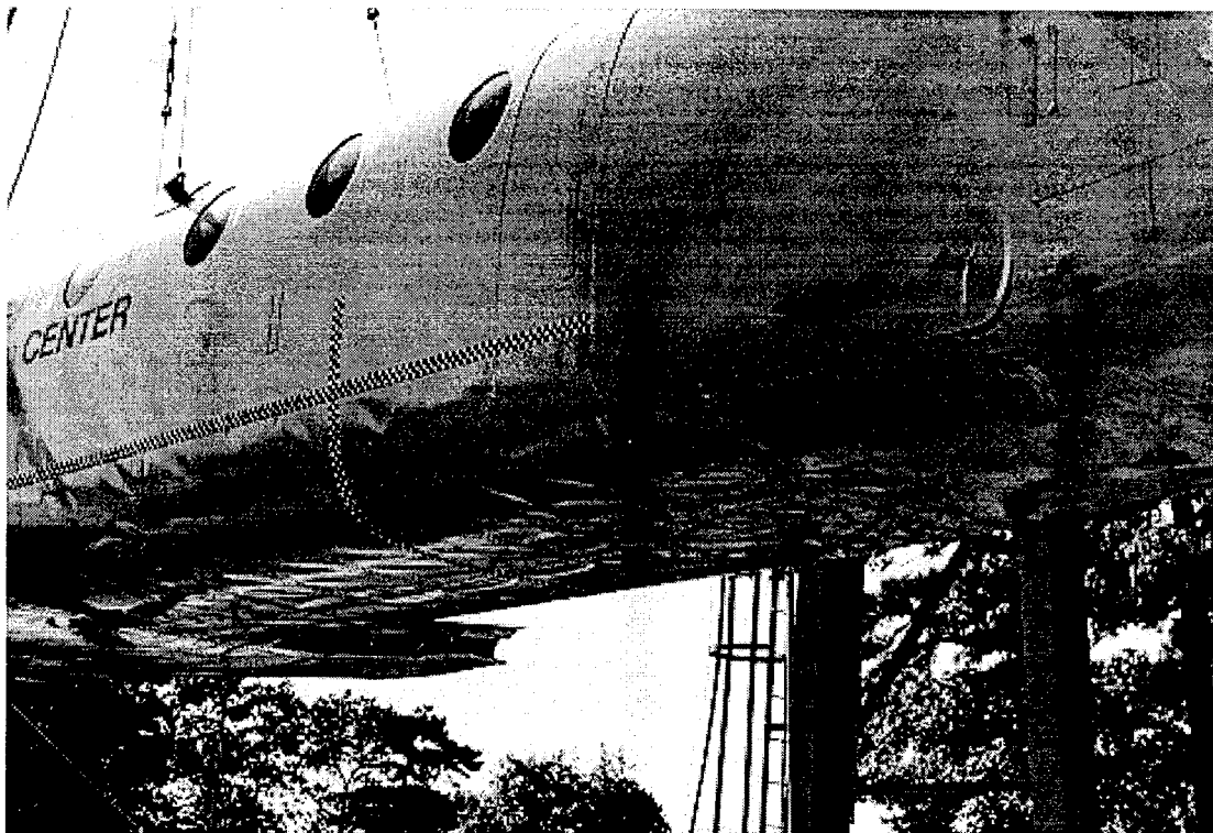
FIGURE 5. UNDERSIDE OF AFT SECTION OF FUSELAGE AFTER IMPACT
