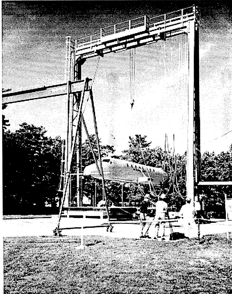
FIGURE 1. DROP TEST FACILITY
