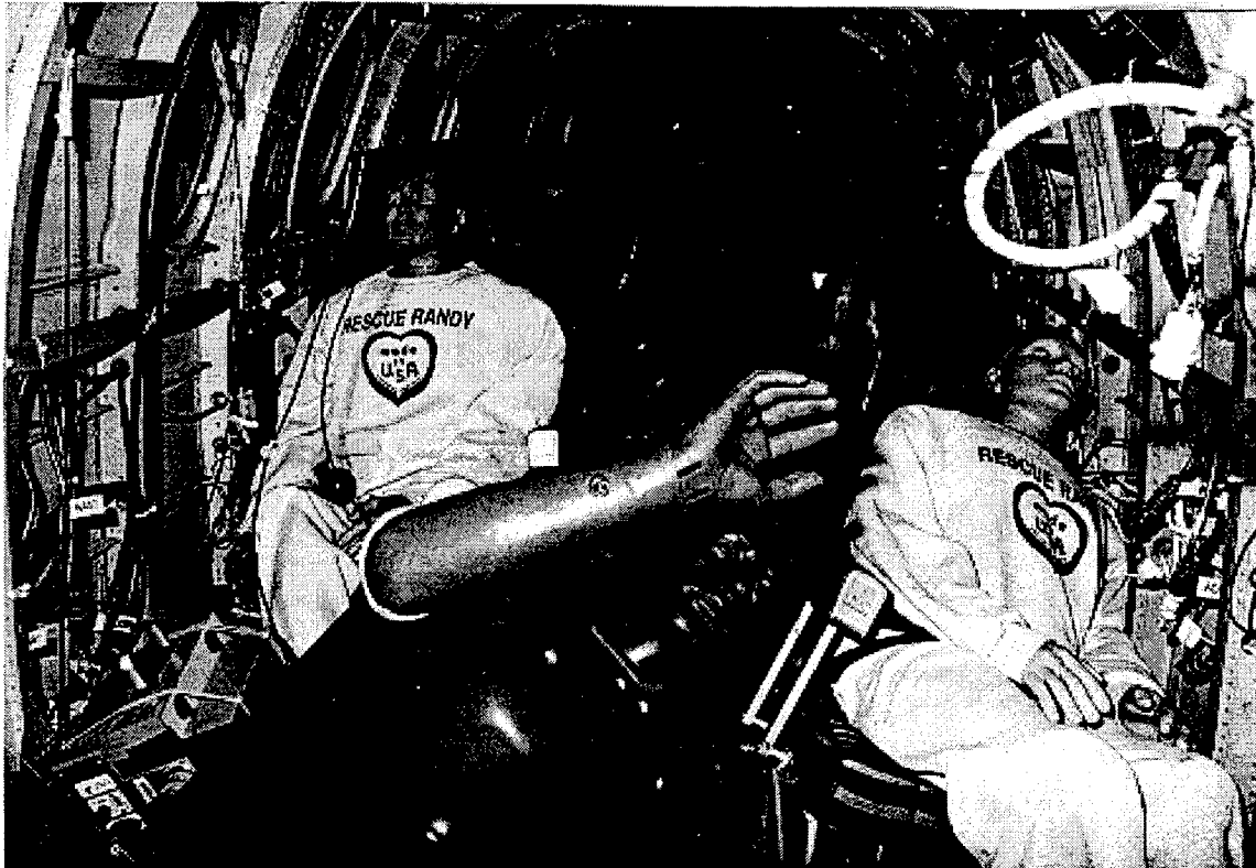
FIGURE 7. FRONT INTERIOR OF TEST ARTICLE AFTER IMPACT
