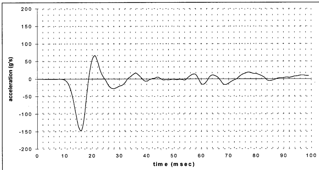
FIGURE 3. FS 260 FLOOR, LEFT SEAT TRACK VERTICAL ACCELERATION
